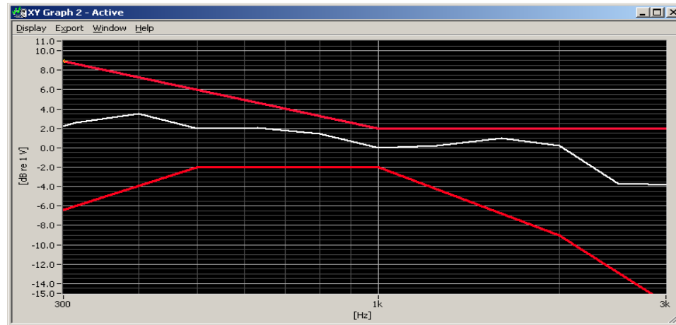
Figure 6-1 Axial Frequency Response
