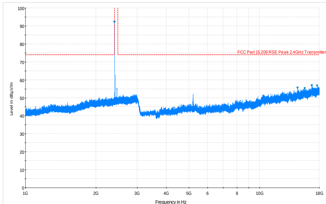
Plot 6-43. Radiated Spurious Plot above 1GHz (BT – Ch. 0, Ant. Pol. V)
