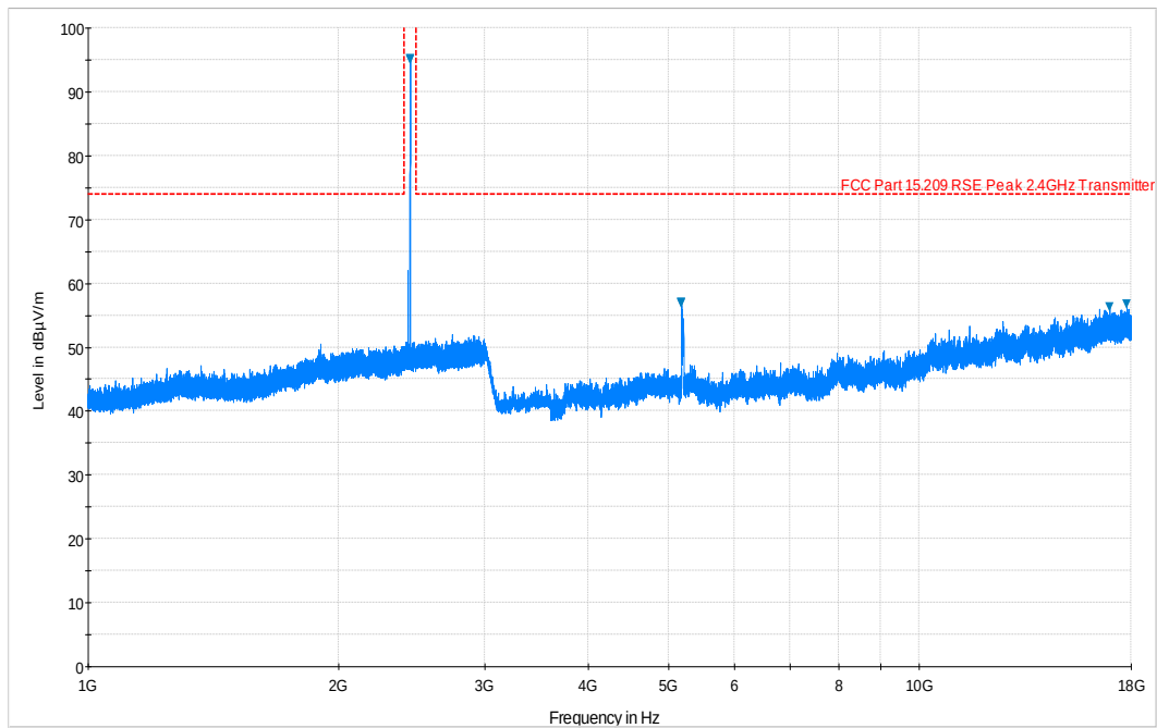
Plot 6-45. Radiated Spurious Plot above 1GHz (BT – Ch. 39, Ant. Pol. V)
