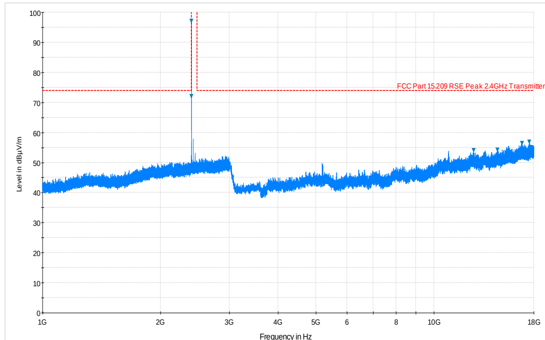
Plot 6-42. Radiated Spurious Plot above 1GHz (BT – Ch. 0, Ant. Pol. H)
