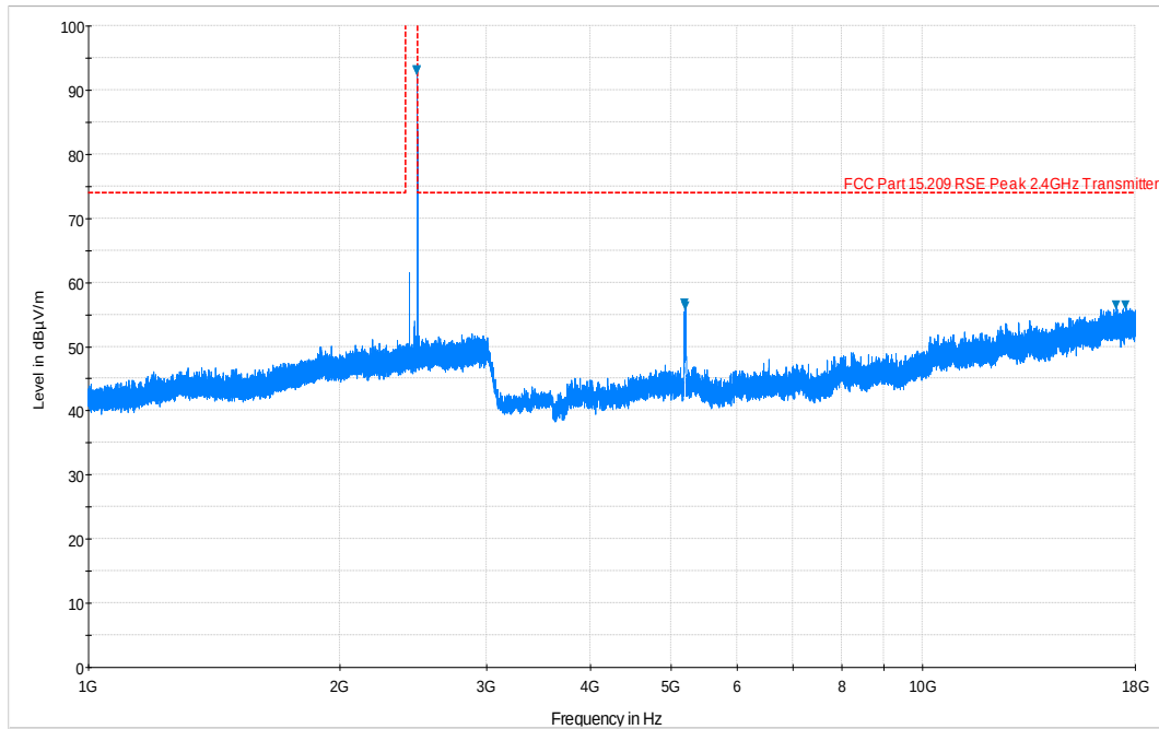
Plot 6-47. Radiated Spurious Plot above 1GHz (BT – Ch. 78, Ant. Pol. V)
