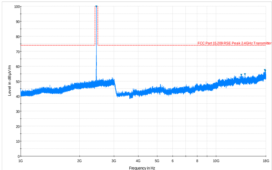
Plot 6-44. Radiated Spurious Plot above 1GHz (BT – Ch. 39, Ant. Pol. H)
