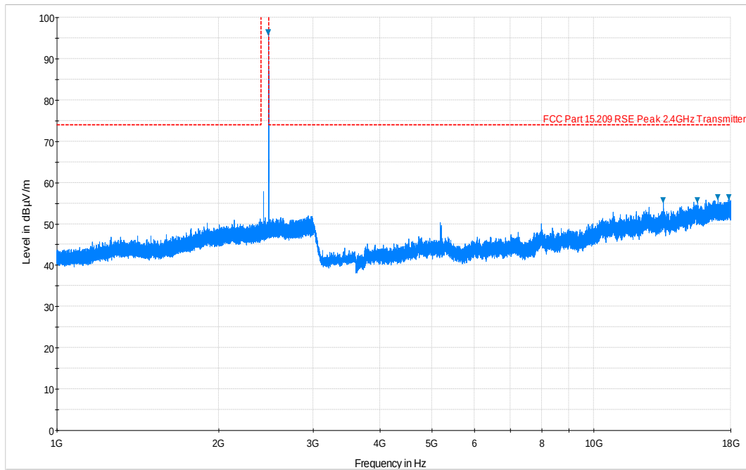
Plot 6-46. Radiated Spurious Plot above 1GHz (BT – Ch. 78, Ant. Pol. H)
