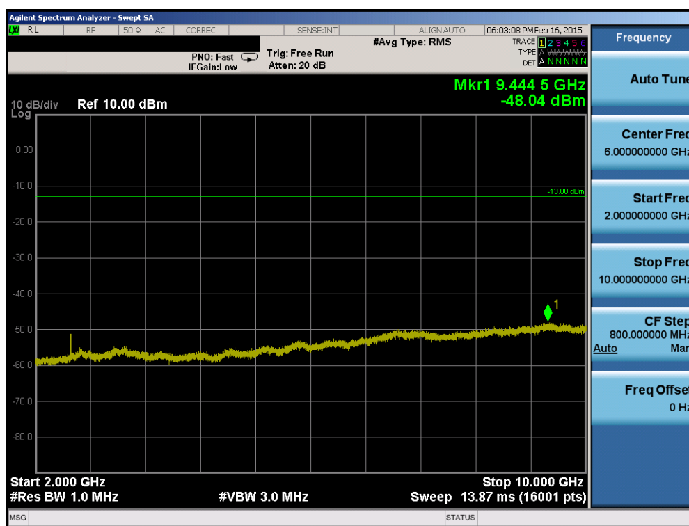
Plot 6-30. Conducted Spurious Plot (Cellular WCDMA Mode - Ch. 4183)
