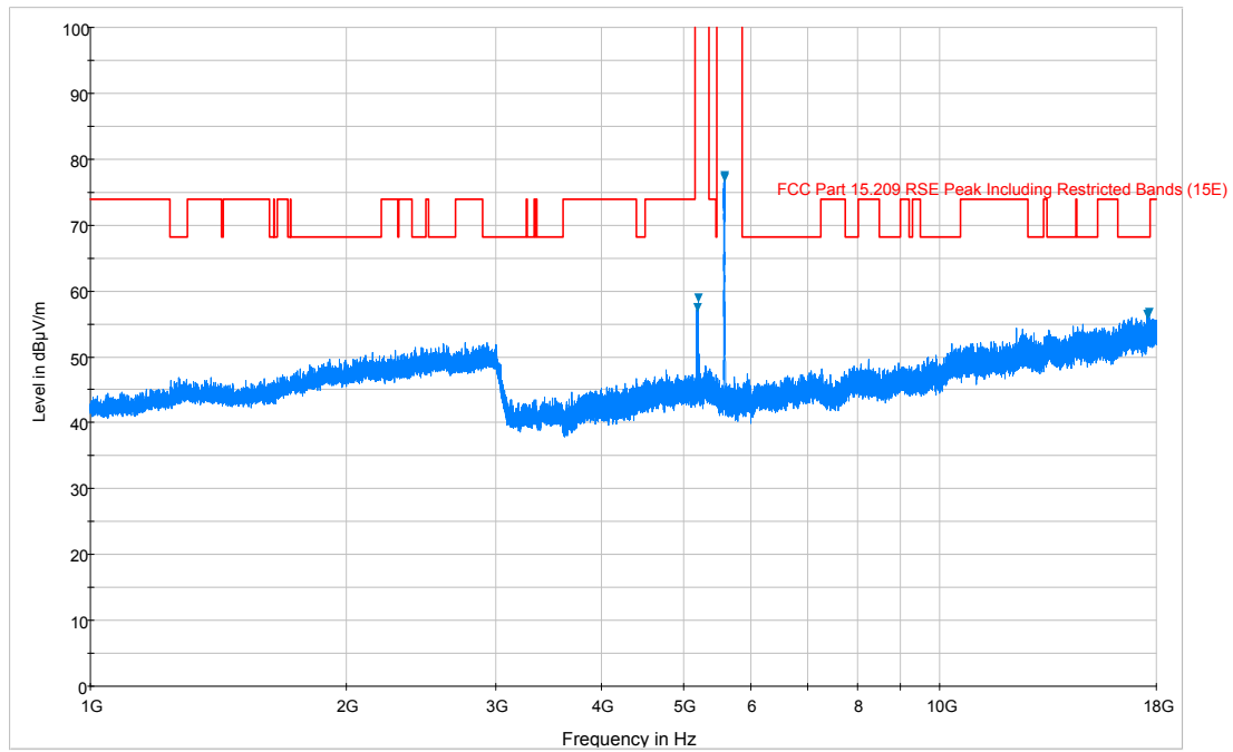
Plot 6-167. Radiated Spurious Plot above 1GHz (802.11a – U2C Ch. 116, Ant. Pol. H)
