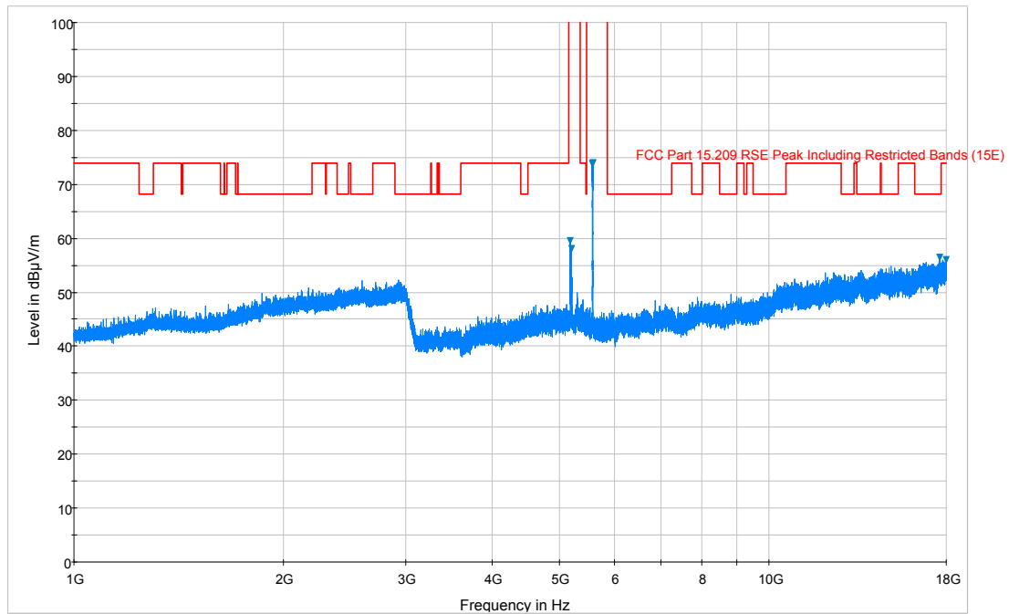
Plot 6-168. Radiated Spurious Plot above 1GHz (802.11a – U2C Ch. 116, Ant. Pol. V)
