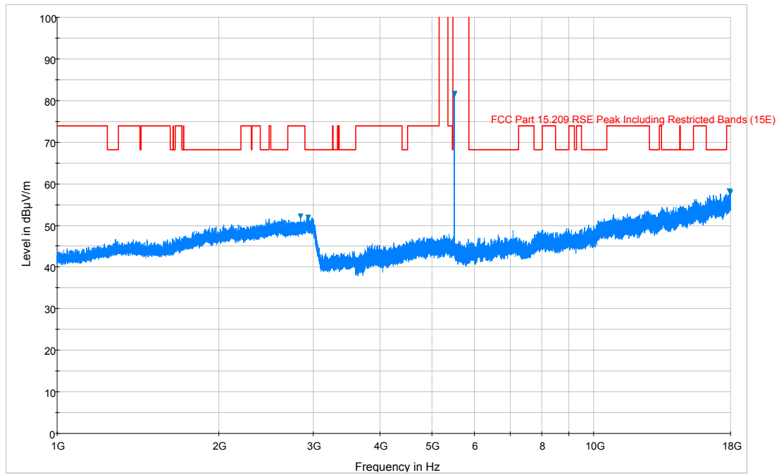
Plot 6-157. Radiated Spurious Plot above 1GHz (802.11a – U2C Ch. 116, Ant. Pol. H)
