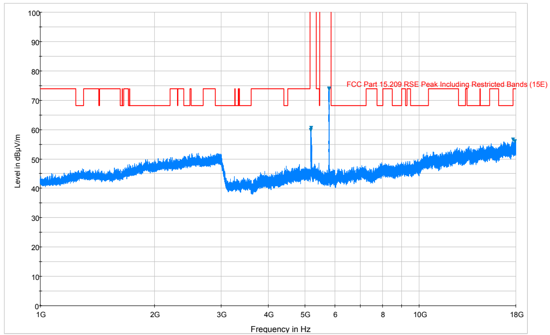
Plot 6-169. Radiated Spurious Plot above 1GHz (802.11a – U3 Ch. 157, Ant. Pol. H)
