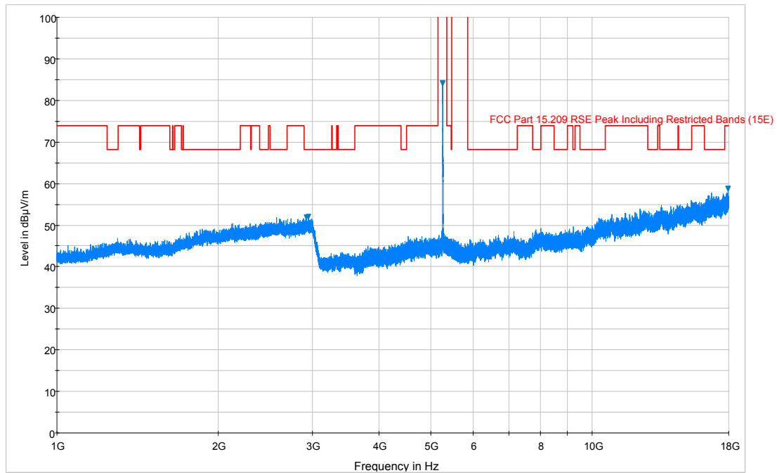
Plot 6-156. Radiated Spurious Plot above 1GHz (802.11a – U2A Ch. 56, Ant. Pol. V)
