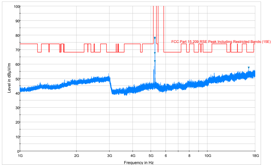
Plot 6-166. Radiated Spurious Plot above 1GHz (802.11a – U2A Ch. 56, Ant. Pol. V)
