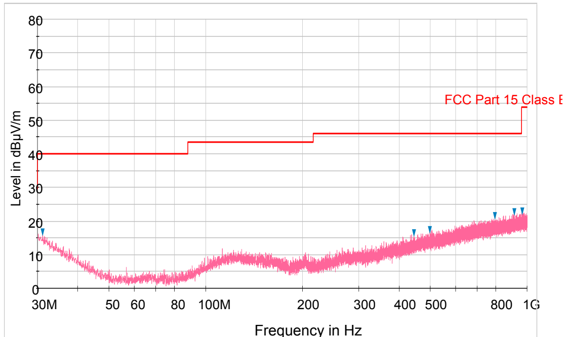
Plot 6-237. Radiated Spurious Plot below 1GHz (802.11a – U3 Ch. 157, Ant. Pol. V)
