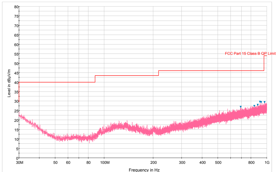
Plot 6-239. Radiated Spurious Plot below 1GHz (802.11a – U3 Ch. 157, Ant. Pol. V)
