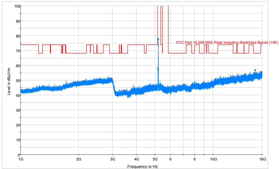
Plot 6-163. Radiated Spurious Plot above 1GHz (802.11a – U1 Ch. 40, Ant. Pol. H)
