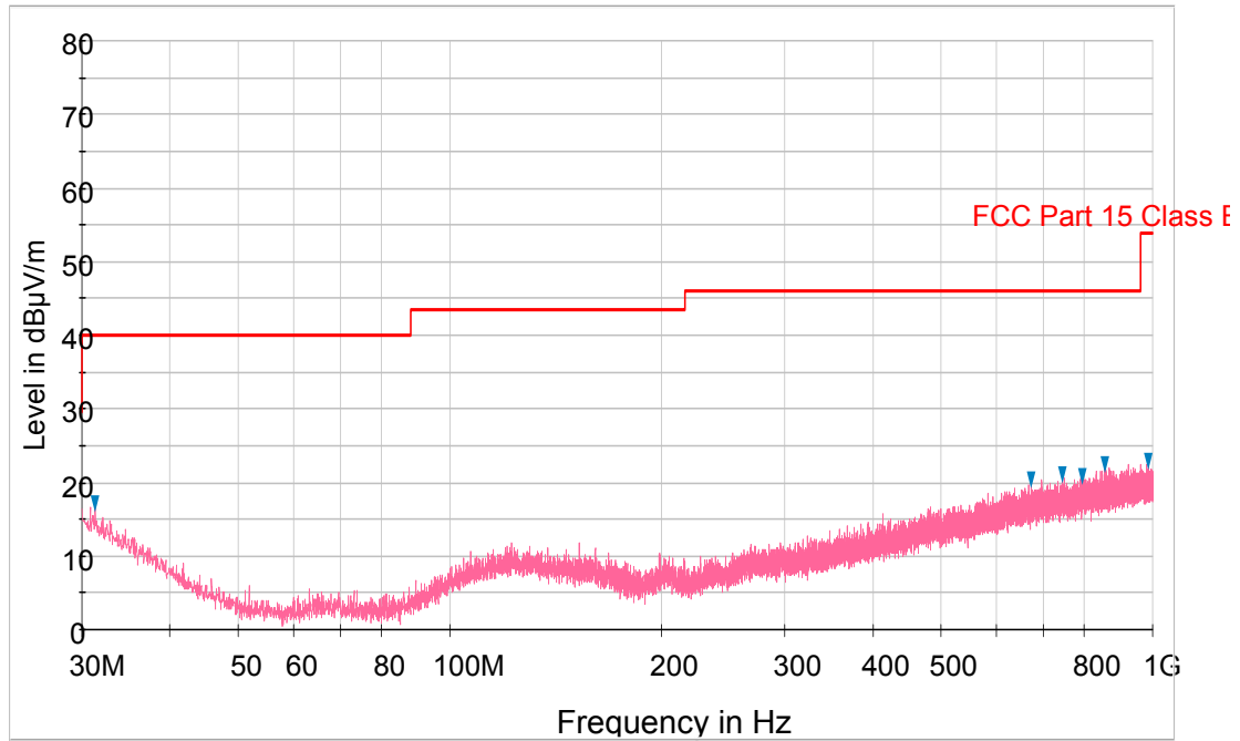
Plot 6-236. Radiated Spurious Plot below 1GHz (802.11a – U3 Ch. 157, Ant. Pol. H)
