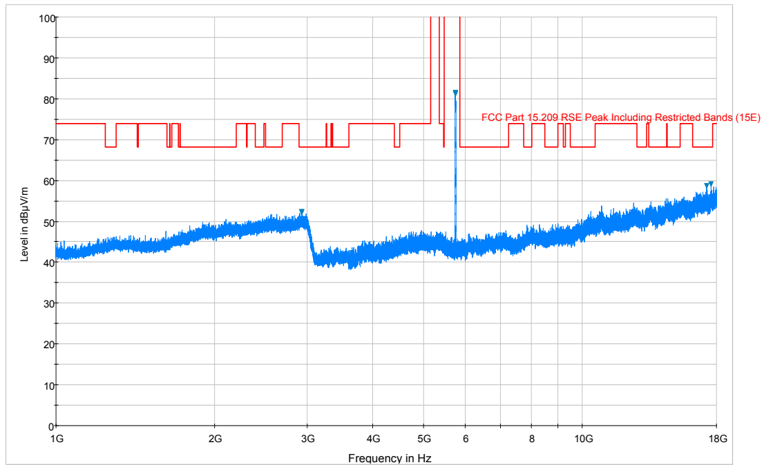
Plot 6-160. Radiated Spurious Plot above 1GHz (802.11a – U3 Ch. 157, Ant. Pol. V)
