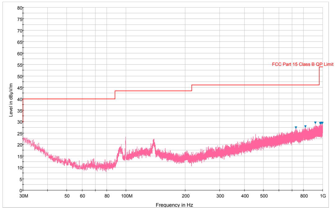
Plot 6-238. Radiated Spurious Plot below 1GHz (802.11a – U3 Ch. 157, Ant. Pol. H)
