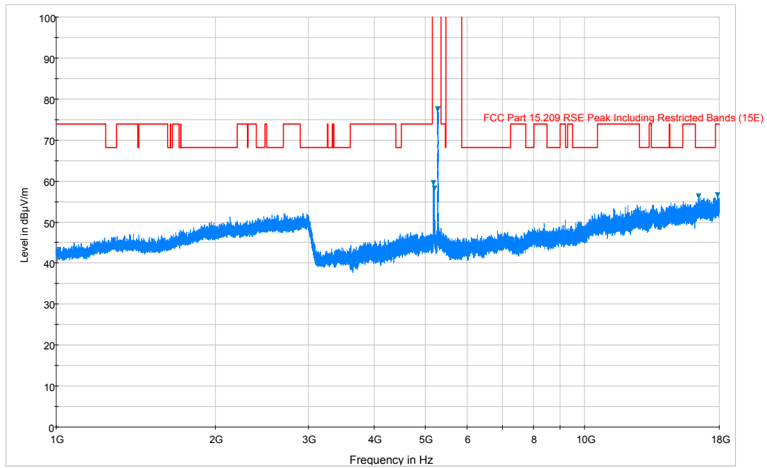
Plot 6-165. Radiated Spurious Plot above 1GHz (802.11a – U2A Ch. 56, Ant. Pol. H)
