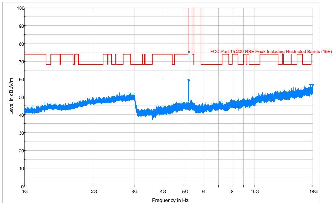
Plot 6-164. Radiated Spurious Plot above 1GHz (802.11a – U1 Ch. 40, Ant. Pol. V)
