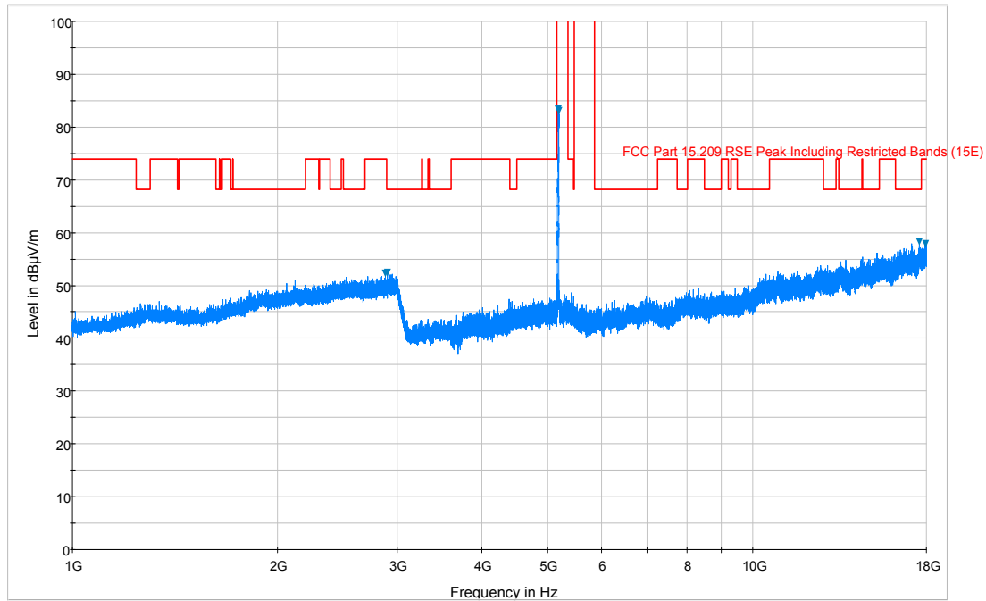
Plot 6-153. Radiated Spurious Plot above 1GHz (802.11a – U1 Ch. 40, Ant. Pol. H)
