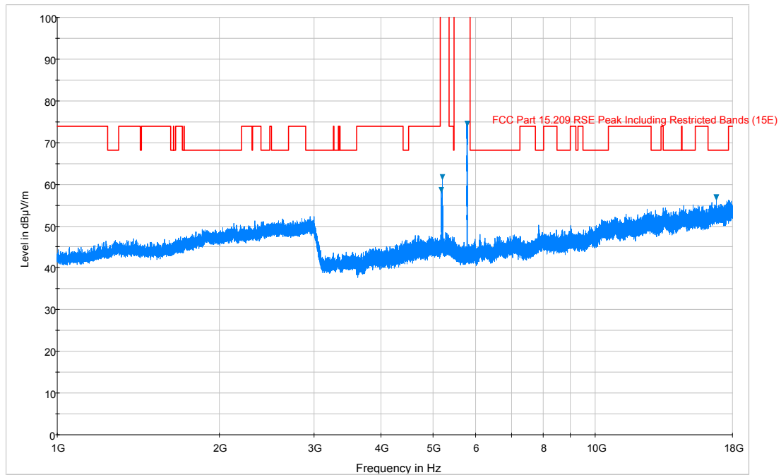
Plot 6-170. Radiated Spurious Plot above 1GHz (802.11a – U3 Ch. 157, Ant. Pol. V)
