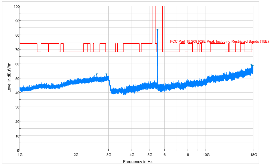
Plot 6-158. Radiated Spurious Plot above 1GHz (802.11a – U2C Ch. 116, Ant. Pol. V)
