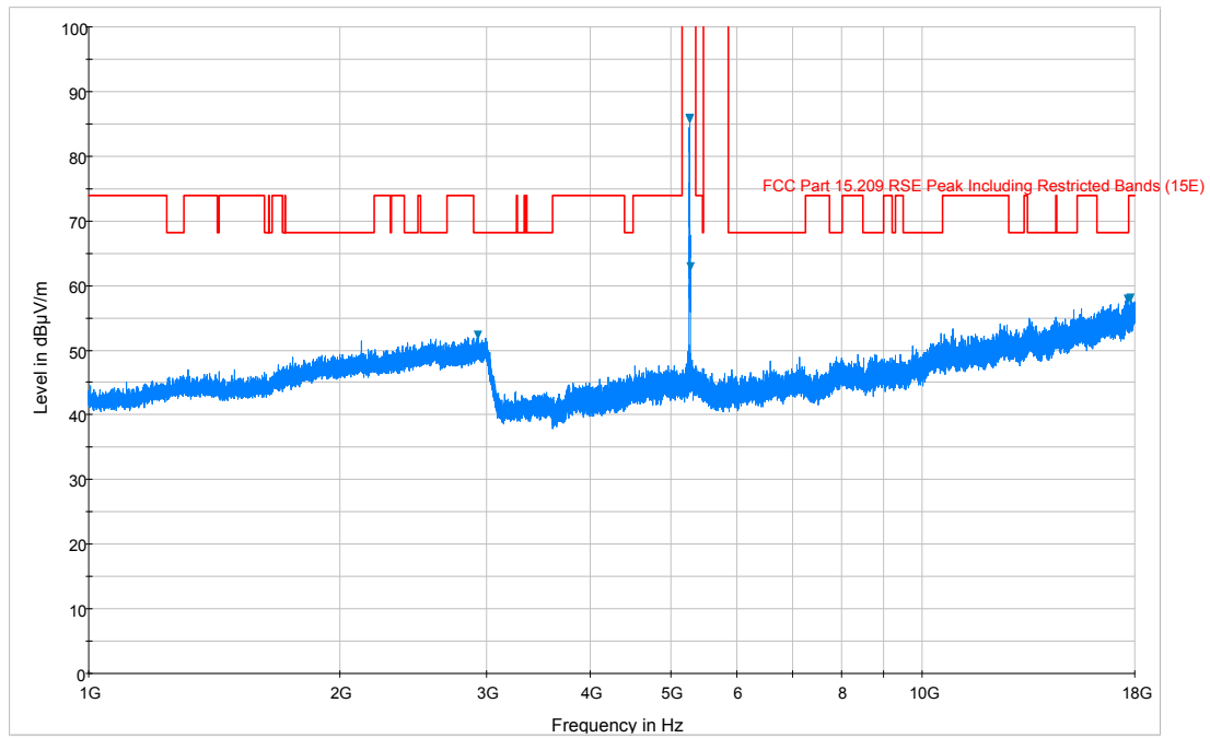
Plot 6-155. Radiated Spurious Plot above 1GHz (802.11a – U2A Ch. 56, Ant. Pol. H)
