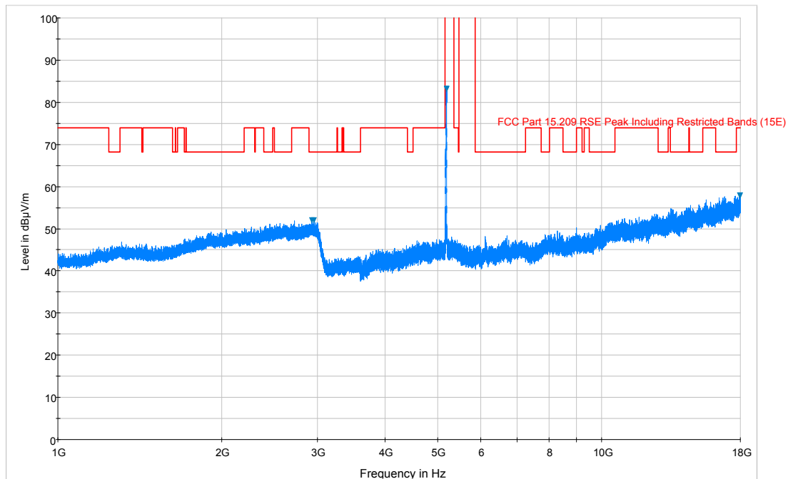
Plot 6-154. Radiated Spurious Plot above 1GHz (802.11a – U1 Ch. 40, Ant. Pol. V)
