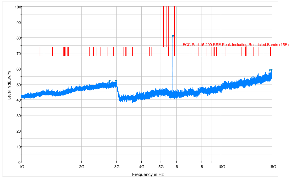
Plot 6-159. Radiated Spurious Plot above 1GHz (802.11a – U3 Ch. 157, Ant. Pol. H)
