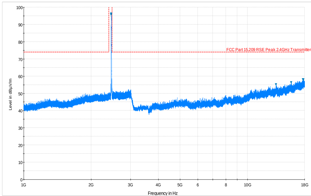
Plot 6-71. Radiated Spurious Plot above 1GHz (802.11b – Ch. 11, Ant. Pol. H)
