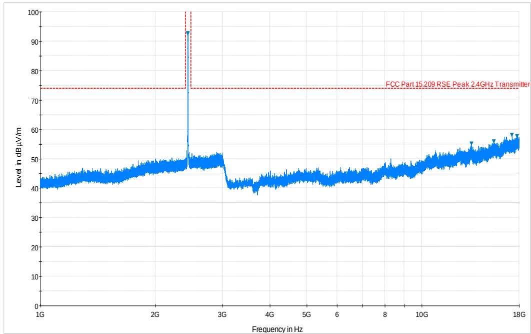
Plot 6-64. Radiated Spurious Plot above 1GHz (802.11b – Ch. 6, Ant. Pol. V)
