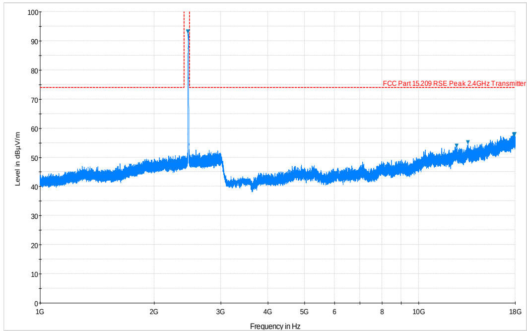
Plot 6-66. Radiated Spurious Plot above 1GHz (802.11b – Ch. 11, Ant. Pol. V)
