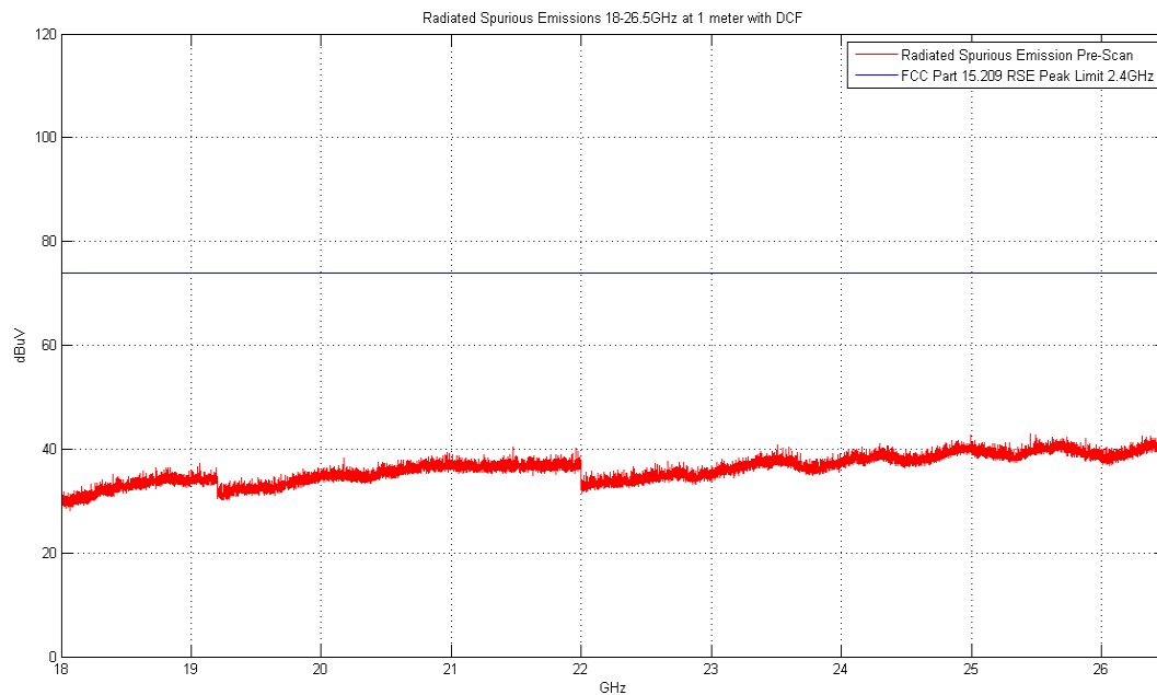
Plot 6-74. Radiated Spurious Plot above 18GHz (Pol. V)
