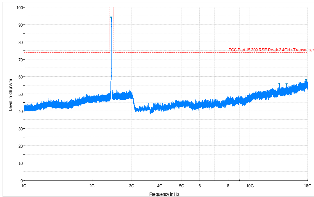
Plot 6-69. Radiated Spurious Plot above 1GHz (802.11b – Ch. 6, Ant. Pol. H)
