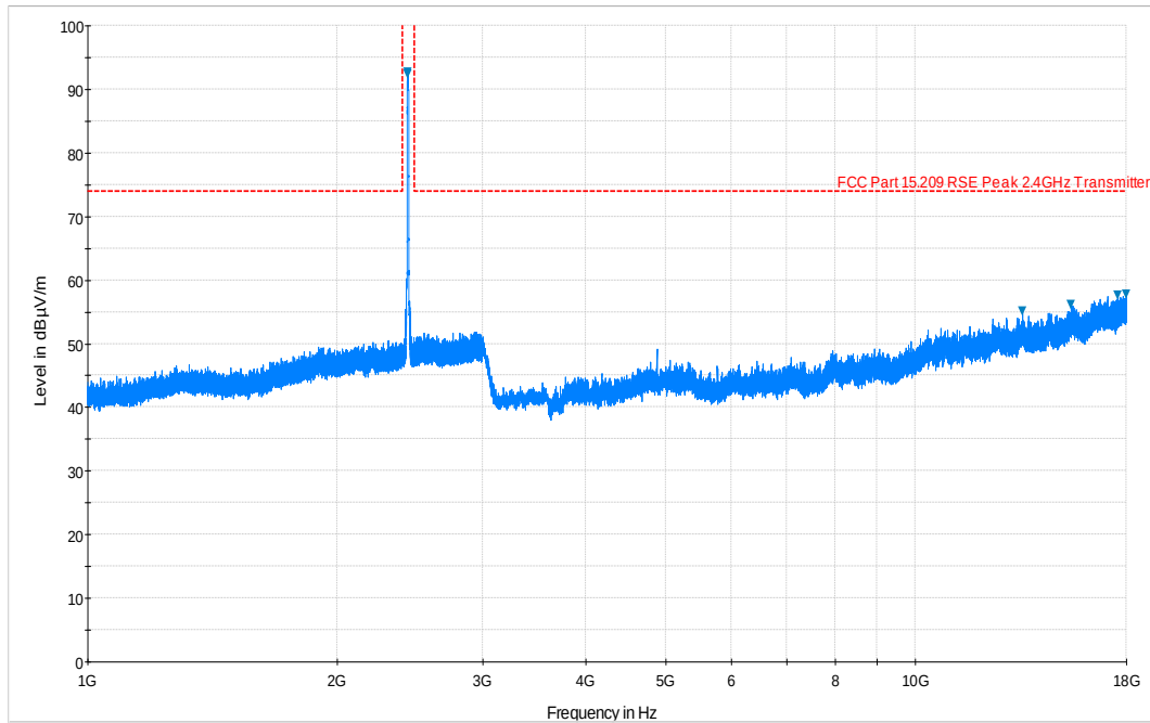
Plot 6-70. Radiated Spurious Plot above 1GHz (802.11b – Ch. 6, Ant. Pol. V)
