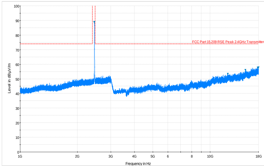
Plot 6-72. Radiated Spurious Plot above 1GHz (802.11b – Ch. 11, Ant. Pol. V)
