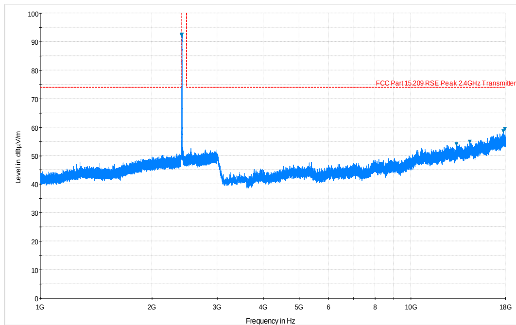
Plot 6-62. Radiated Spurious Plot above 1GHz (802.11b – Ch. 1, Ant. Pol. V)
