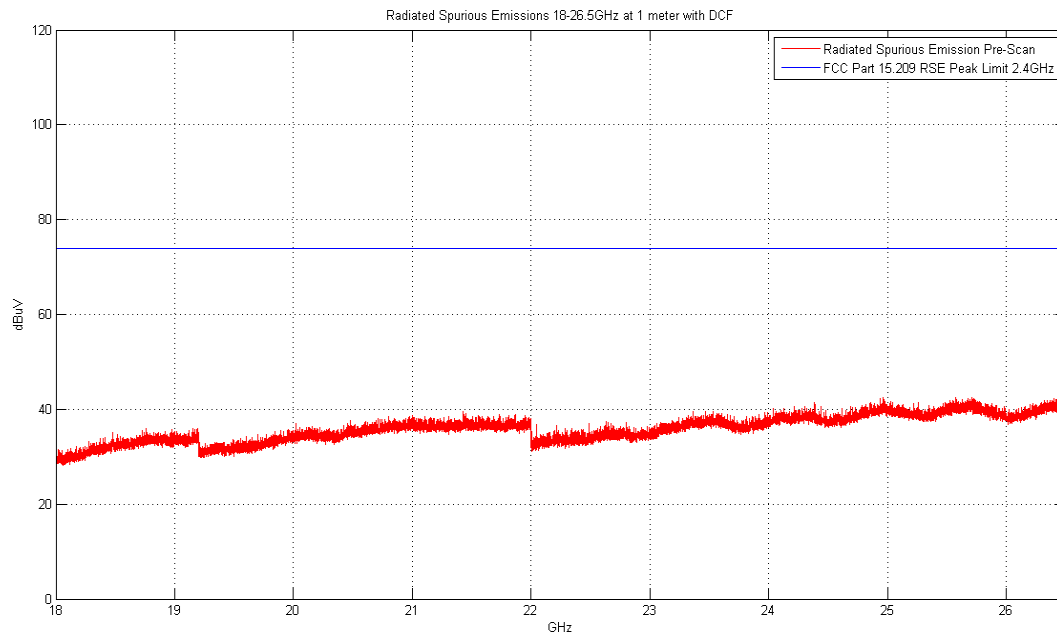
Plot 6-73. Radiated Spurious Plot above 18GHz (Pol. H)
