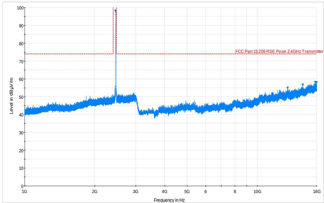
Plot 6-65. Radiated Spurious Plot above 1GHz (802.11b – Ch. 11, Ant. Pol. H)
