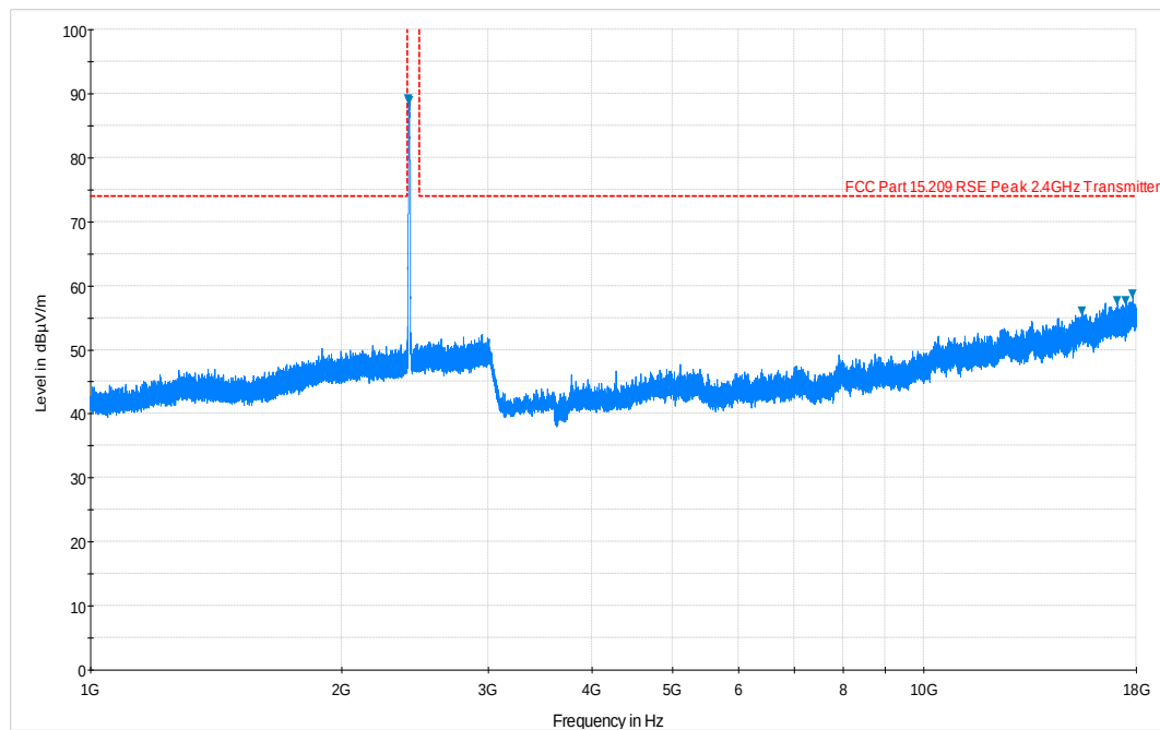
Plot 6-68. Radiated Spurious Plot above 1GHz (802.11b – Ch. 1, Ant. Pol. V)
