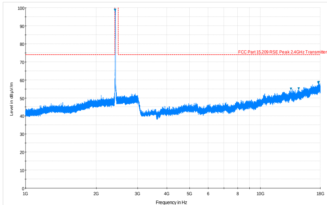
Plot 6-61. Radiated Spurious Plot above 1GHz (802.11b – Ch. 1, Ant. Pol. H)
