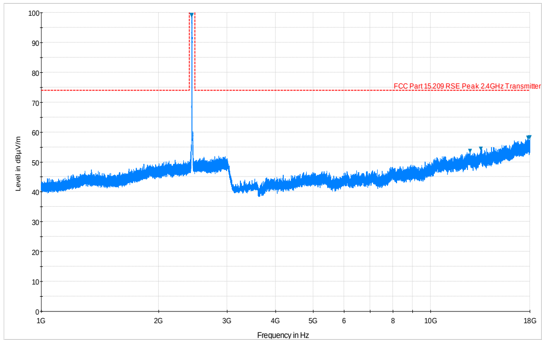
Plot 6-63. Radiated Spurious Plot above 1GHz (802.11b – Ch. 6, Ant. Pol. H)
