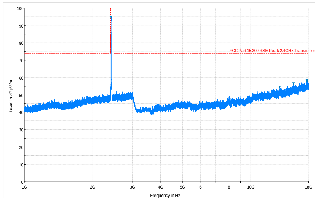
Plot 6-67. Radiated Spurious Plot above 1GHz (802.11b – Ch. 1, Ant. Pol. H)
