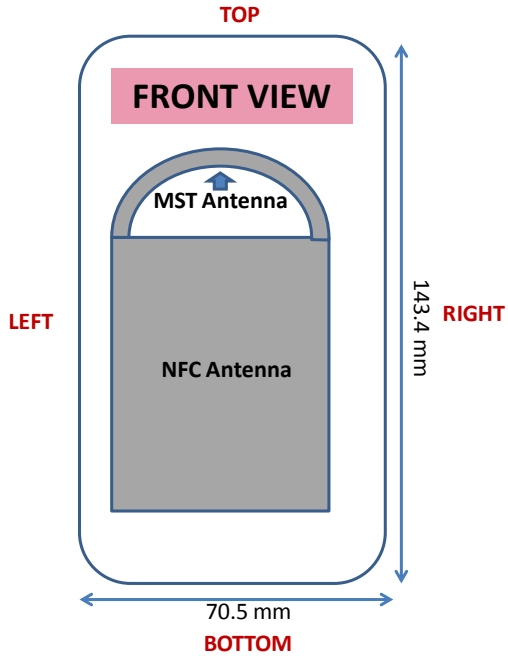
Figure F-1 DUT Antenna Locations
