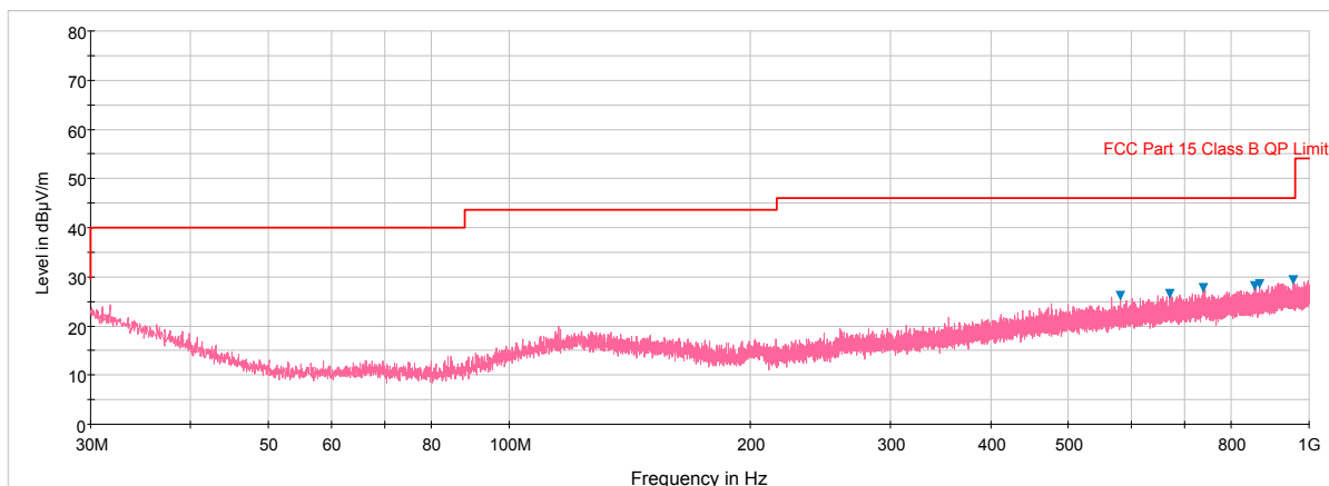
Plot 6-29. Radiated Spurious Plot below 1GHz (Pol. V)
