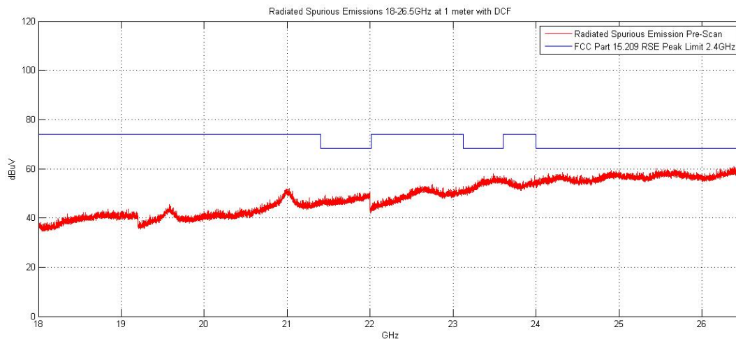
Plot 6-24. Radiated Spurious Plot above 18GHz (Pol. H)
