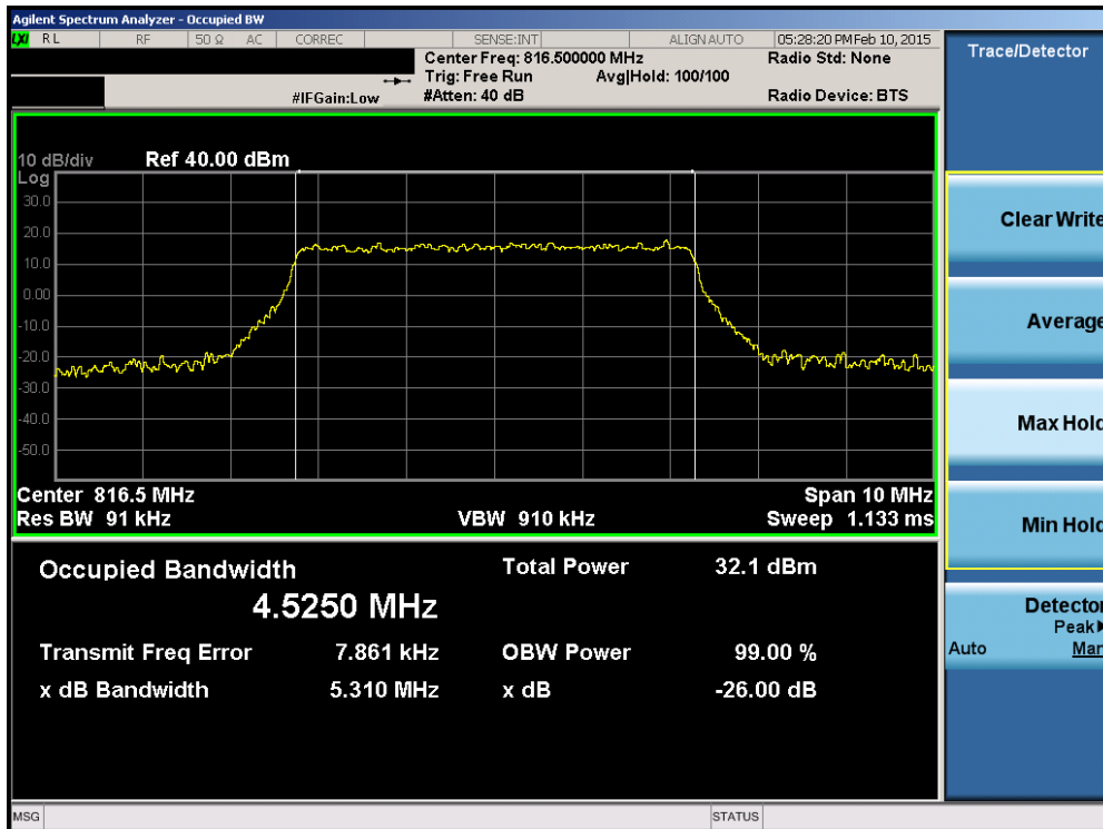
Plot 7-16. Occupied Bandwidth Plot (5MHz QPSK – RB Size 25– Low Channel)
