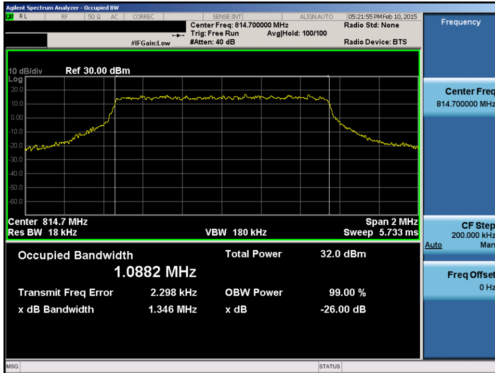
Plot 7-5. Occupied Bandwidth Plot (1.4MHz QPSK – RB Size 6– Low Channel)
