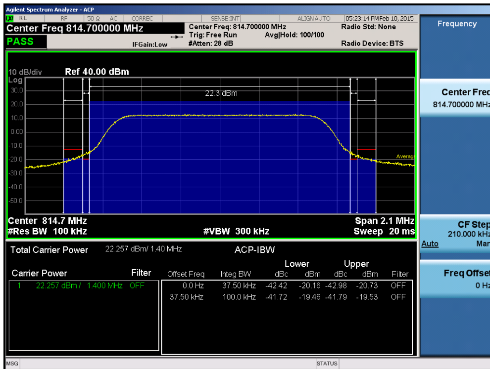
Plot 7-4. Channel Edge Plot (1.4MHz QPSK – RB Size 6– Low Channel)
