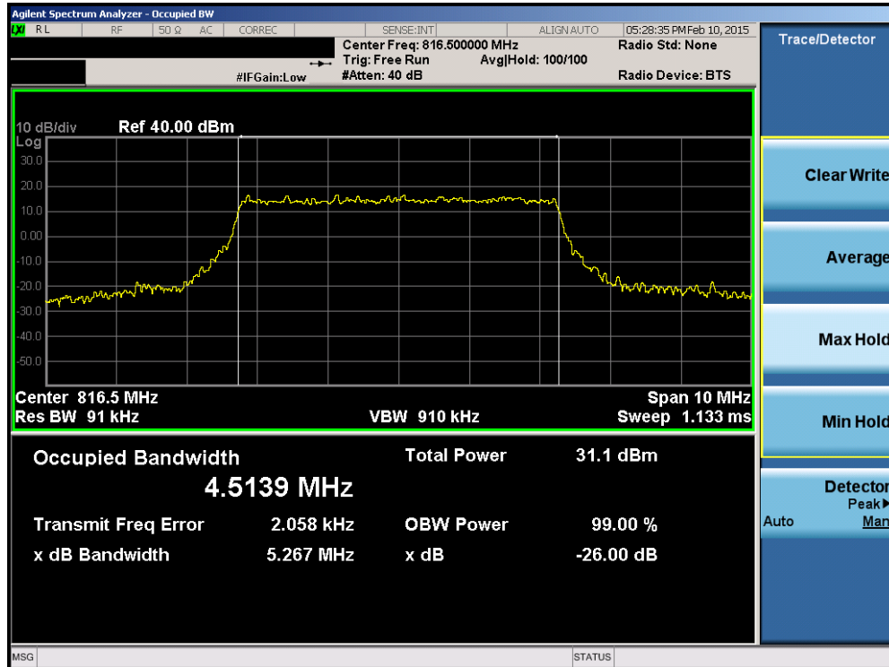
Plot 7-17. Occupied Bandwidth Plot (5MHz 16-QAM – RB Size 25– Low Channel)
