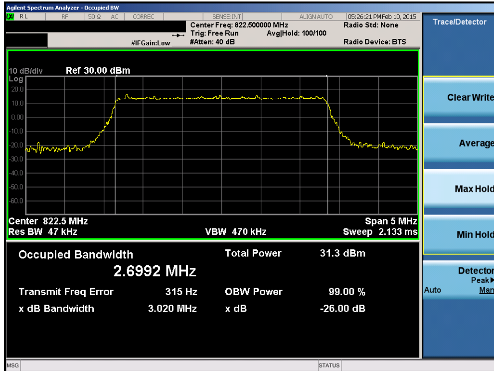
Plot 7-13. Occupied Bandwidth Plot (3MHz 16-QAM – RB Size 15– High Channel))
