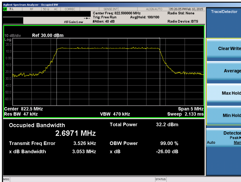
Plot 7-12. Occupied Bandwidth Plot (3MHz QPSK – RB Size 15– High Channel)
