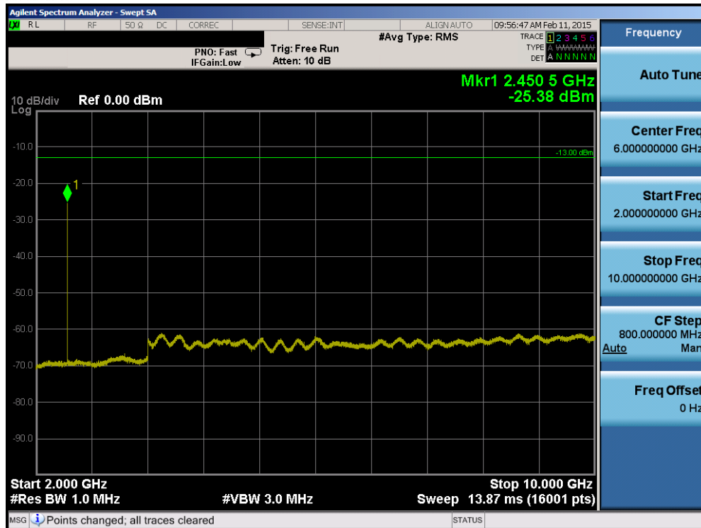
Plot 7-3. Conducted Spurious Plot (1.4MHz QPSK – RB Size 1, RB Offset 0 – Low Channel)
