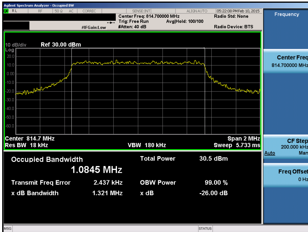
Plot 7-6. Occupied Bandwidth Plot (1.4MHz 16-QAM – RB Size 6– Low Channel)
