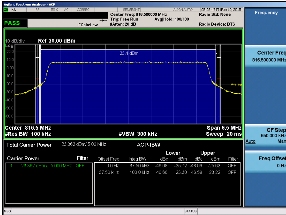
Plot 7-15. Channel Edge Plot (5MHz QPSK – RB Size 25– Low Channel)
