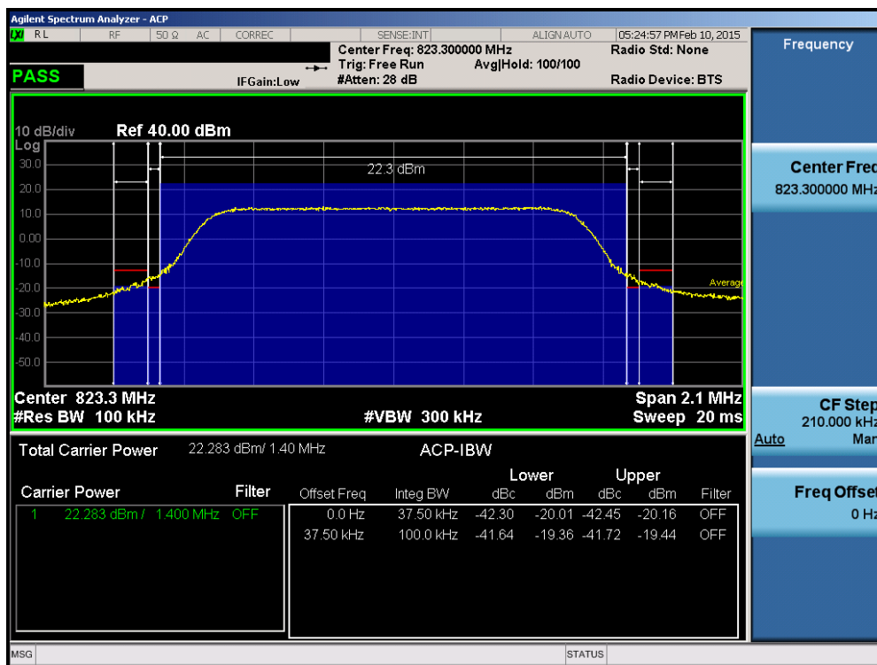
Plot 7-10. Channel Edge Plot (1.4MHz QPSK – RB Size 6 – High Channel)
