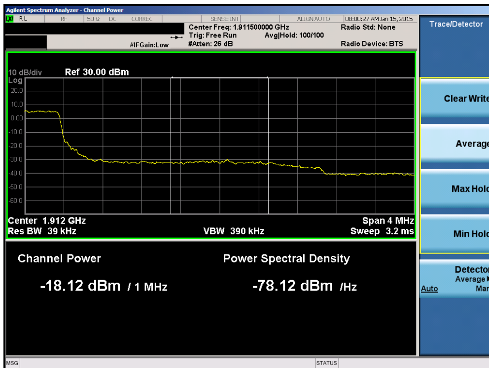
Plot 6-142. Upper Extended Band Edge Plot (Band 2 – 3.0MHz QPSK – RB Size 15)
