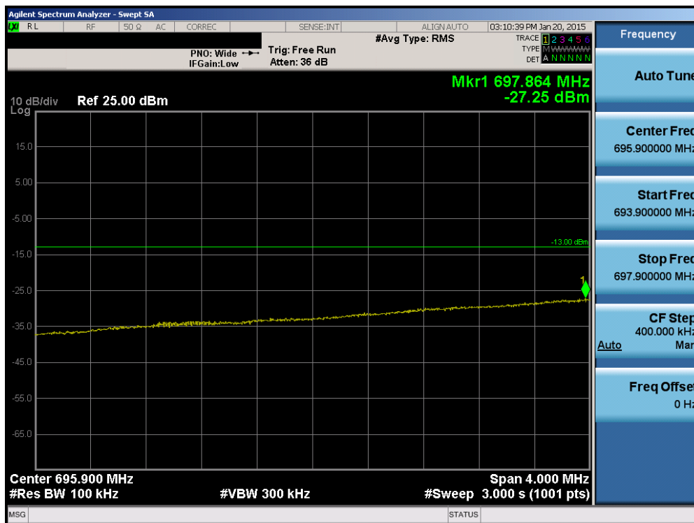
Plot 6-92. Lower Extended Band Edge Plot (Band 12 - 10.0MHz QPSK - RB Size 50)
