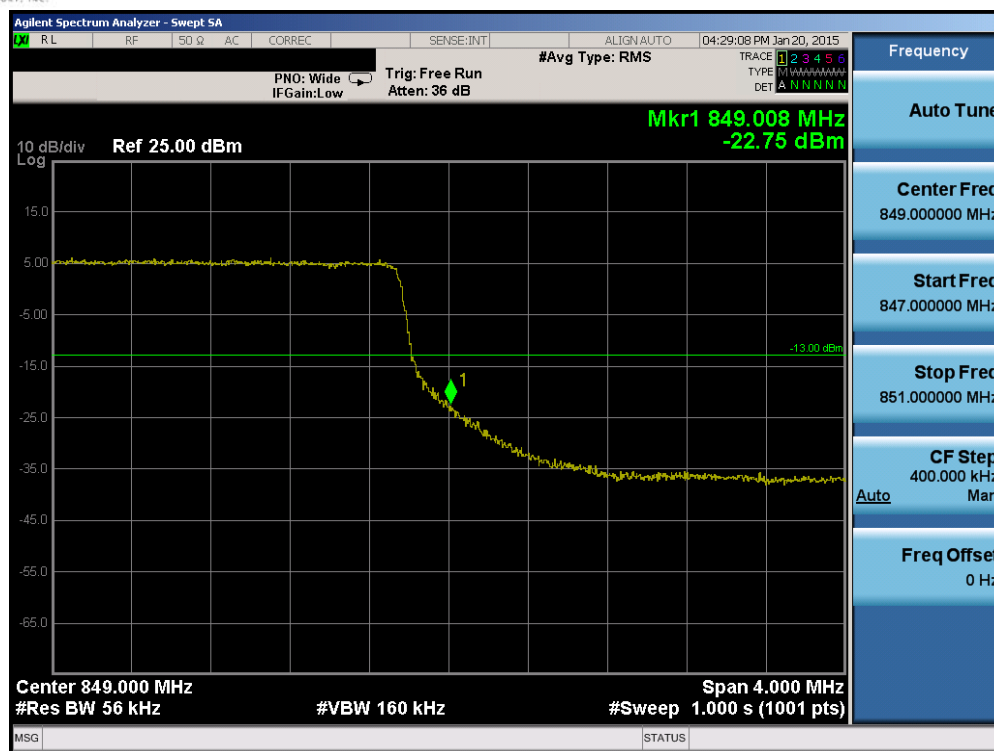
Plot 6-105. Upper Band Edge Plot (Band 5/26 – 5.0MHz QPSK – RB Size 25)
