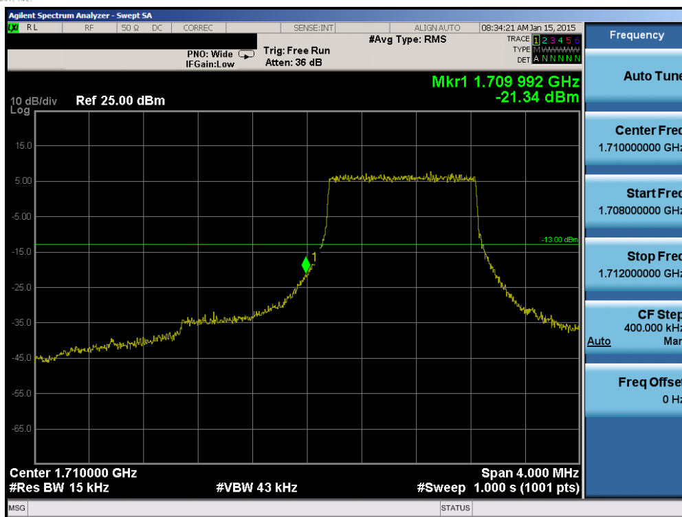
Plot 6-111. Lower Band Edge Plot (Band 4 – 1.4MHz QPSK – RB Size 6)
