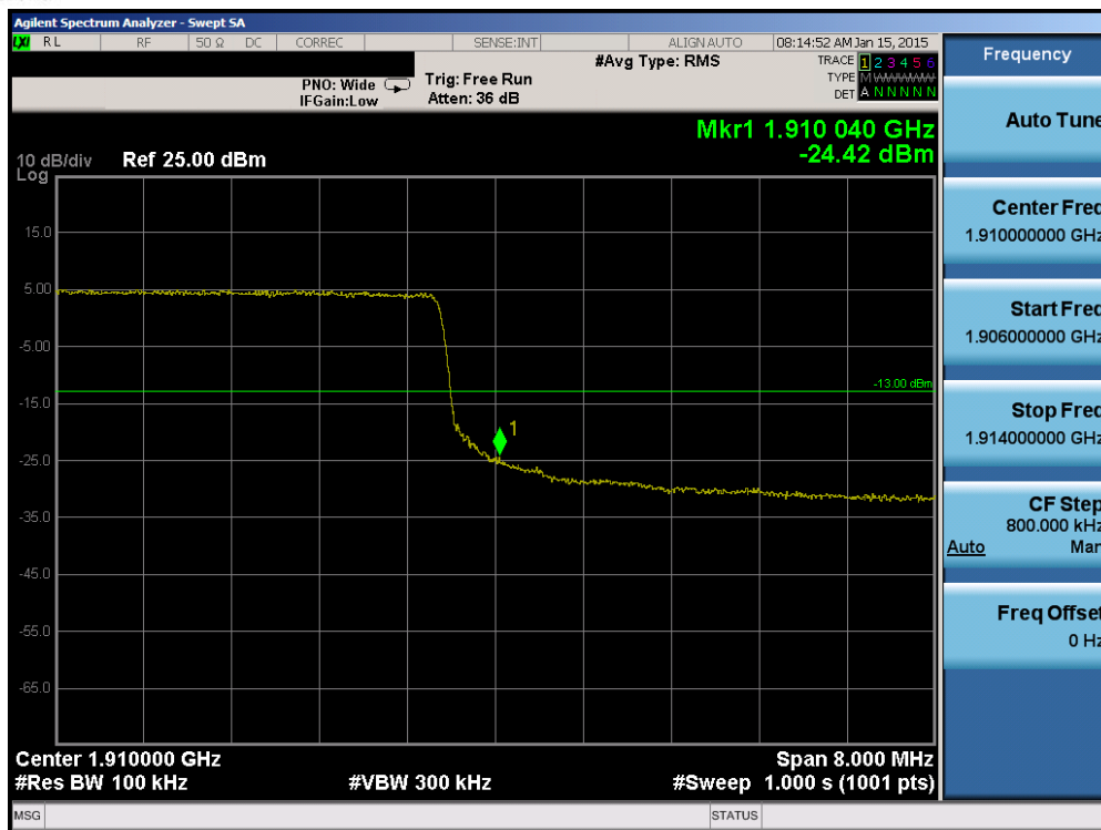
Plot 6-149. Upper Band Edge Plot (Band 2 – 10.0MHz QPSK – RB Size 50)
