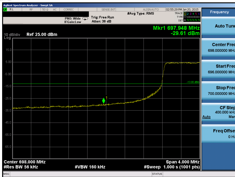
Plot 6-87. Lower Band Edge Plot (Band 12 – 5.0MHz QPSK – RB Size 25)
