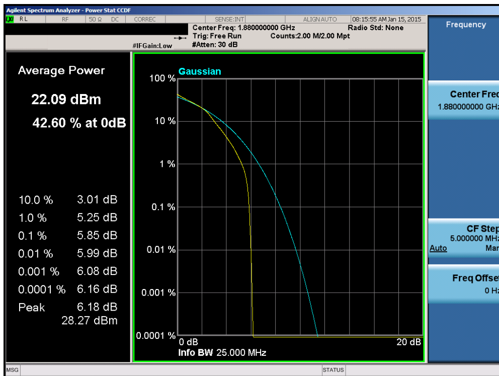
Plot 6-168. PAR Plot (Band 2 – 15.0MHz 16-QAM – RB Size 75)
