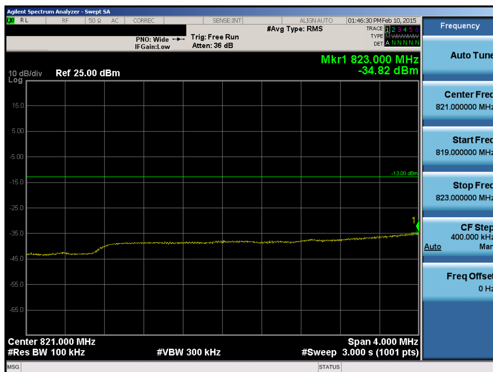
Plot 6-104. Lower Extended Band Edge Plot (Band 5/26 - 5.0MHz QPSK - RB Size 25)
