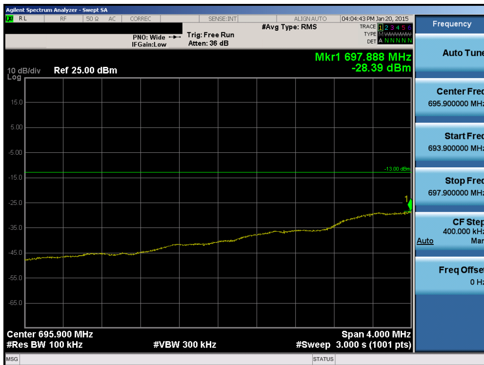
Plot 6-80. Lower Extended Band Edge Plot (Band 12 – 1.4MHz QPSK – RB Size 6)
