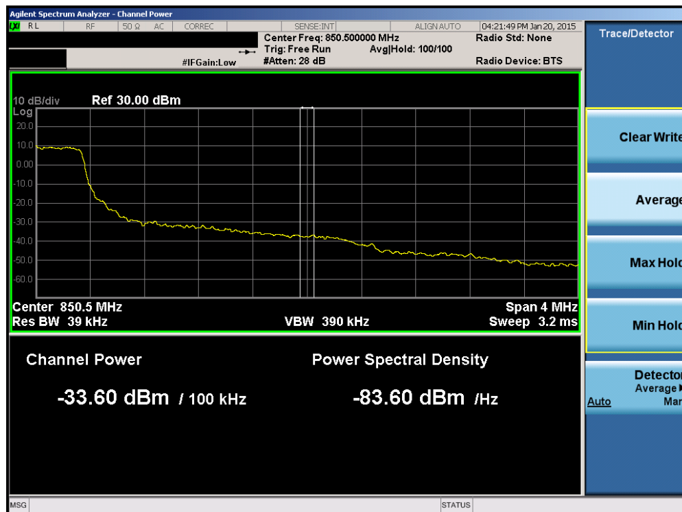
Plot 6-98. Upper Extended Band Edge Plot (Band 5/26 – 1.4MHz QPSK – RB Size 6)
