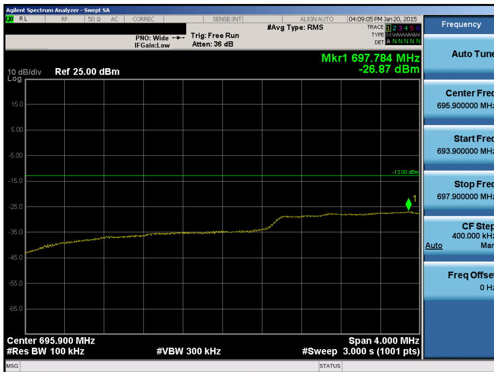
Plot 6-84. Lower Extended Band Edge Plot (Band 12 – 3.0MHz QPSK – RB Size 15)
