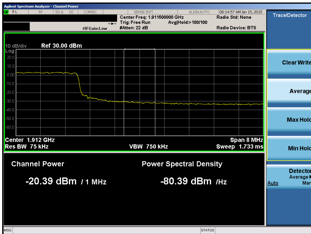
Plot 6-150. Upper Extended Band Edge Plot (Band 2 – 10.0MHz QPSK – RB Size 50)
