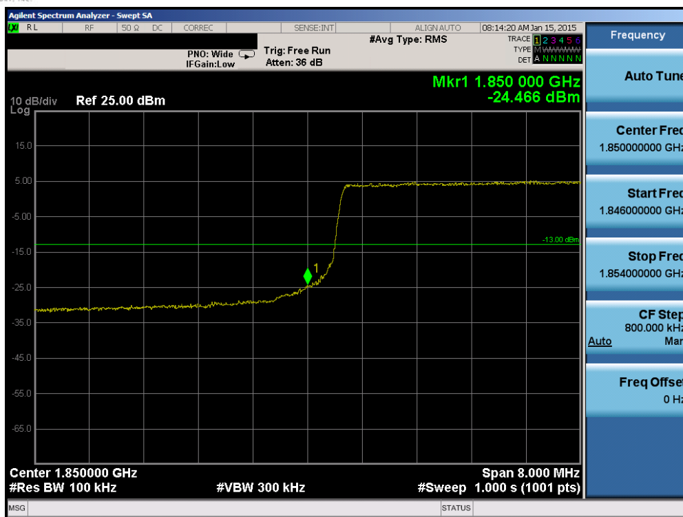
Plot 6-147. Lower Band Edge Plot (Band 2 – 10.0MHz QPSK – RB Size 50)
