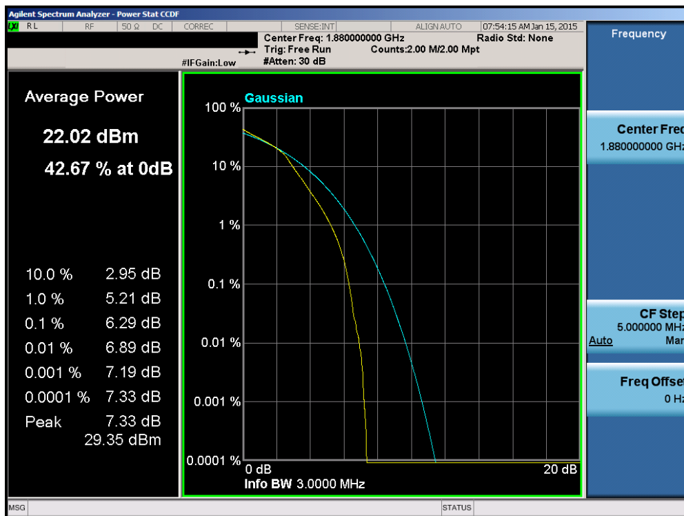
Plot 6-162. PAR Plot (Band 2 – 3.0MHz 16-QAM – RB Size 15)
