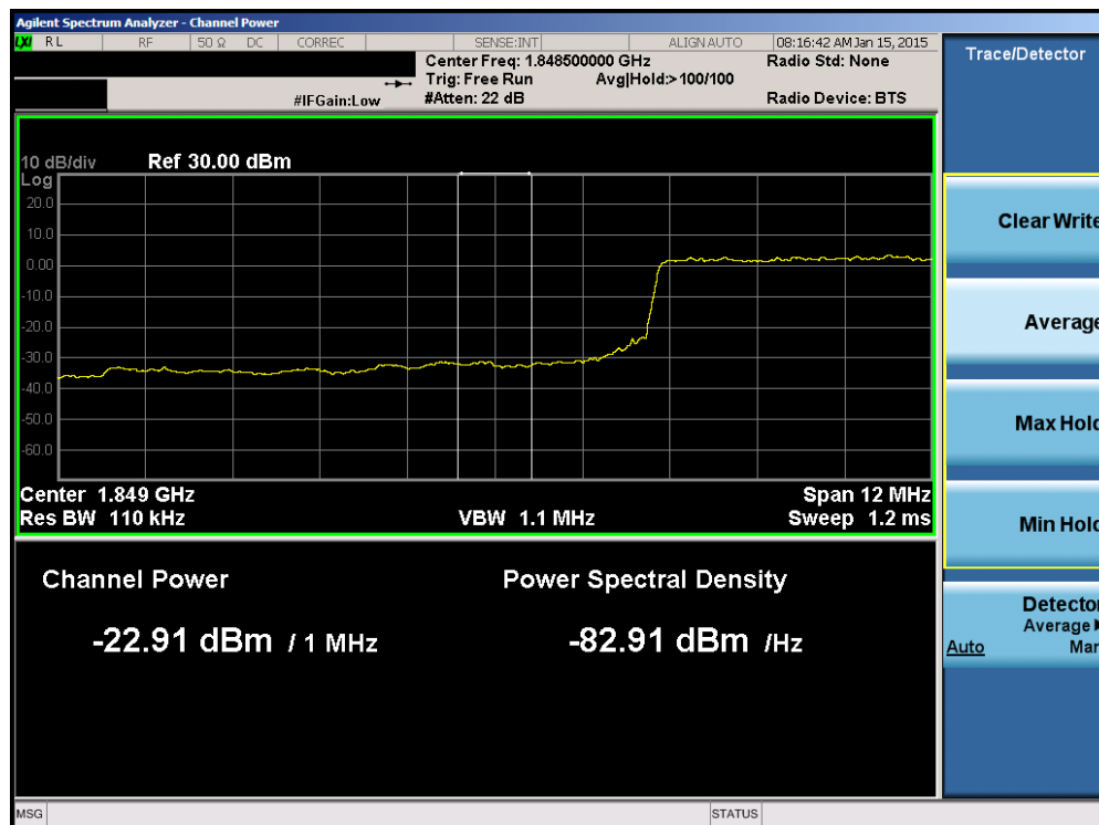
Plot 6-152. Lower Extended Band Edge Plot (Band 2 – 15.0MHz QPSK – RB Size 75)
