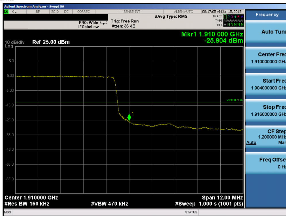
Plot 6-153. Upper Band Edge Plot (Band 2 – 15.0MHz QPSK – RB Size 75)
