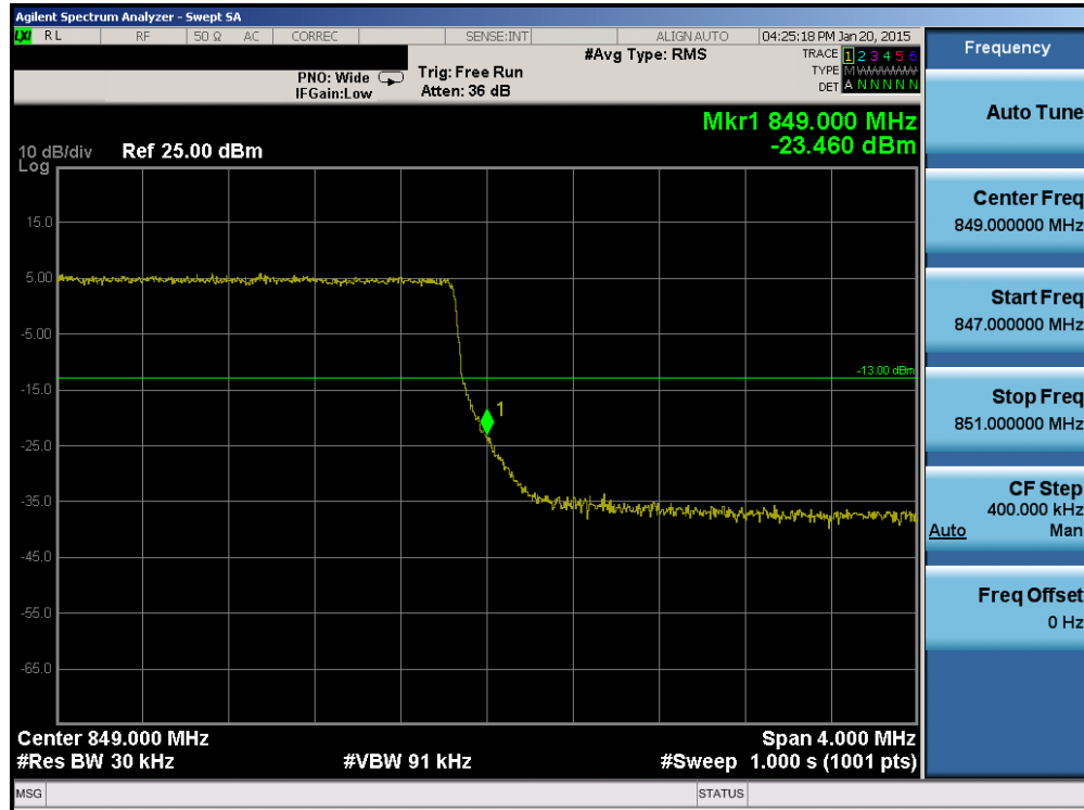
Plot 6-101. Upper Band Edge Plot (Band 5/26 – 3.0MHz QPSK – RB Size 15)
