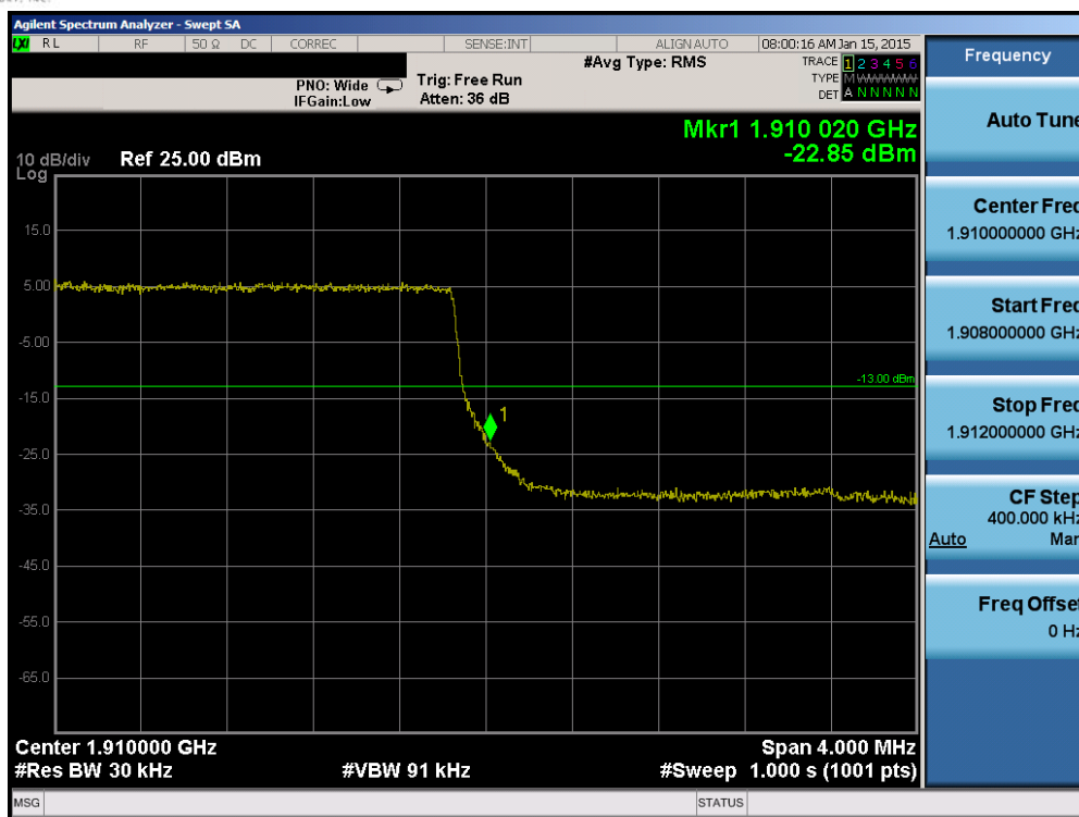
Plot 6-141. Upper Band Edge Plot (Band 2 – 3.0MHz QPSK – RB Size 15)
