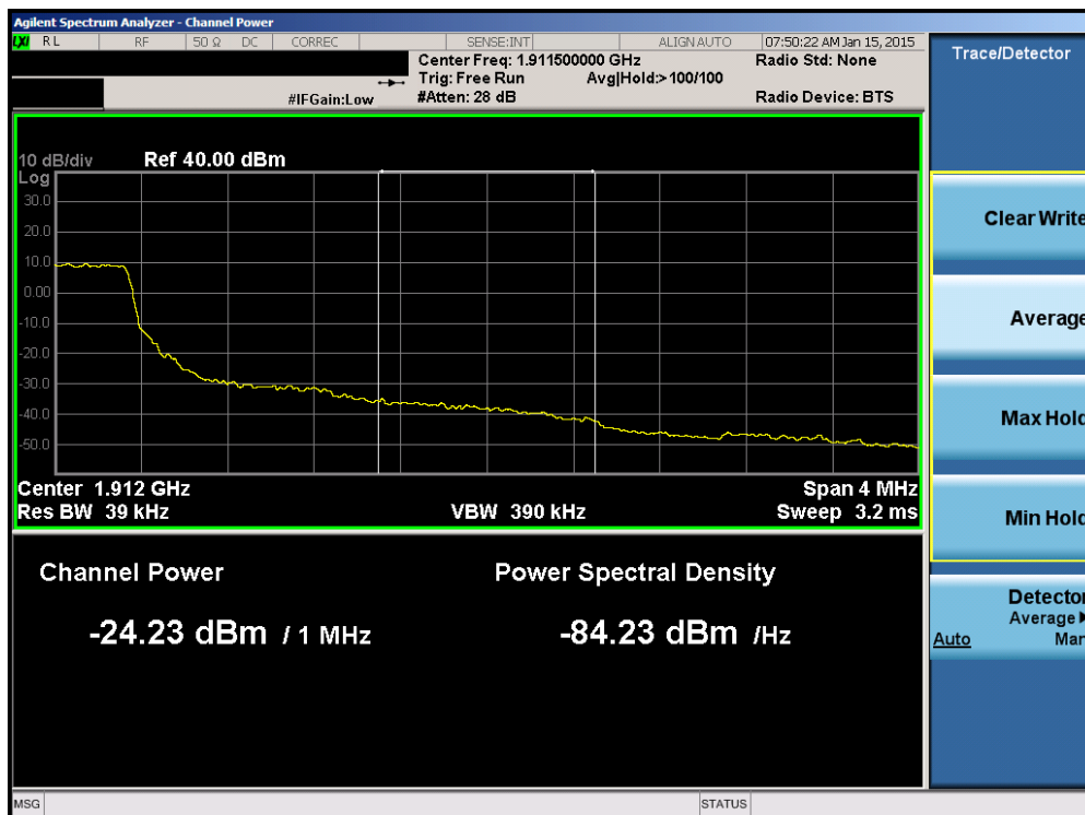
Plot 6-138. Upper Extended Band Edge Plot (Band 2 – 1.4MHz QPSK – RB Size 6)
