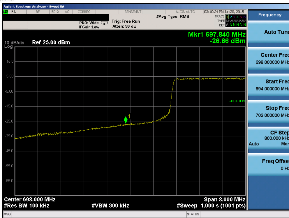
Plot 6-91. Lower Band Edge Plot (Band 12 - 10.0MHz QPSK - RB Size 50)
