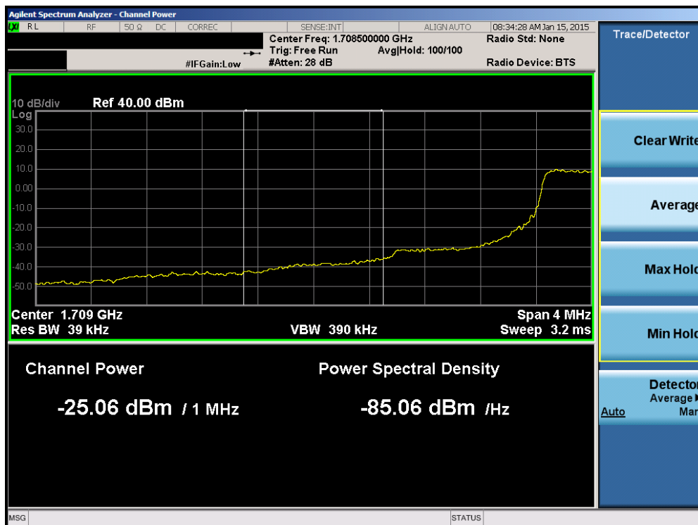
Plot 6-112. Lower Extended Band Edge Plot (Band 4 – 1.4MHz QPSK – RB Size 6)
