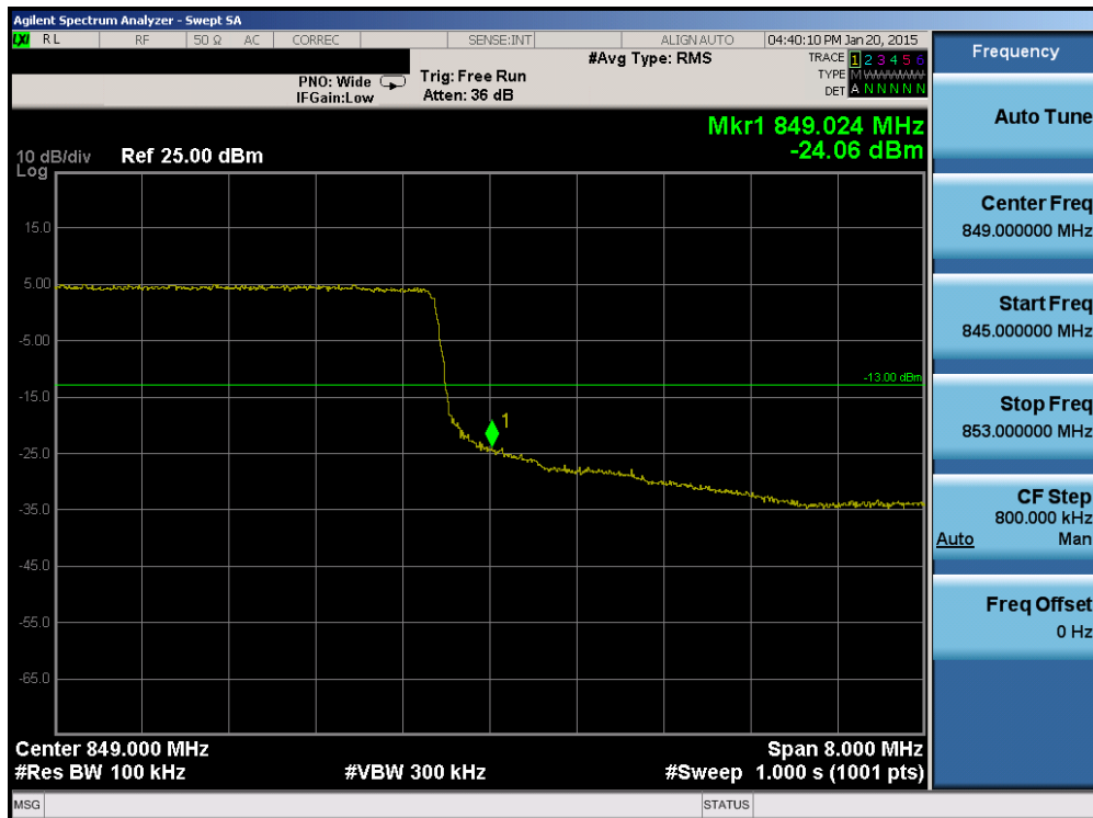
Plot 6-108. Upper Band Edge Plot (Band 5/26 – 10.0MHz QPSK – RB Size 50)
