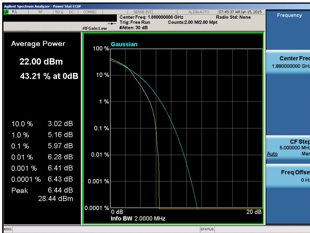
Plot 6-160. PAR Plot (Band 2 – 1.4MHz 16-QAM – RB Size 6)
