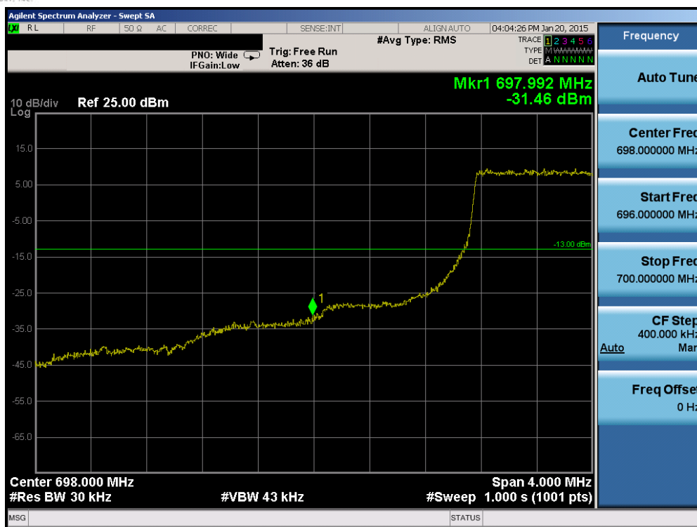
Plot 6-79. Lower Band Edge Plot (Band 12 – 1.4MHz QPSK – RB Size 6)
