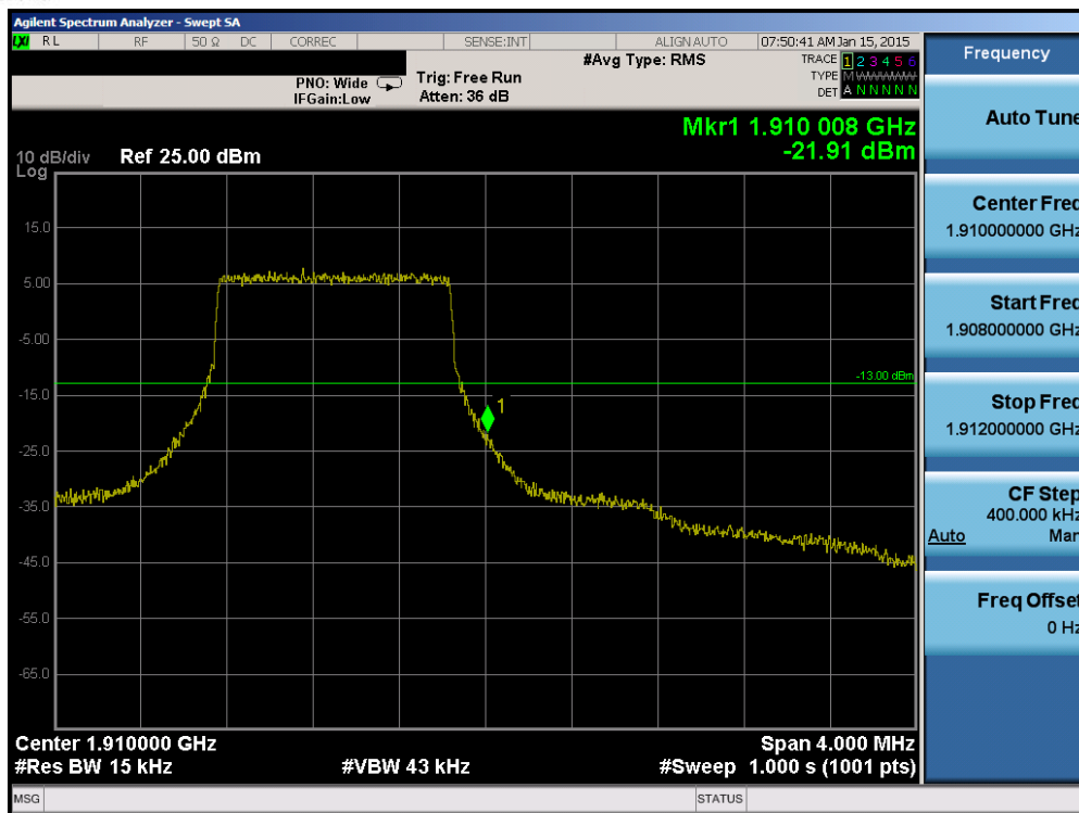
Plot 6-137. Upper Band Edge Plot (Band 2 – 1.4MHz QPSK – RB Size 6)
