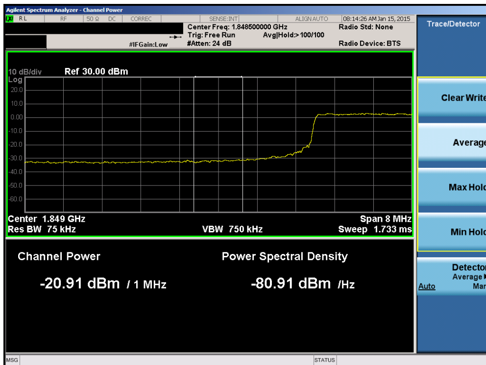
Plot 6-148. Lower Extended Band Edge Plot (Band 2 – 10.0MHz QPSK – RB Size 50)
