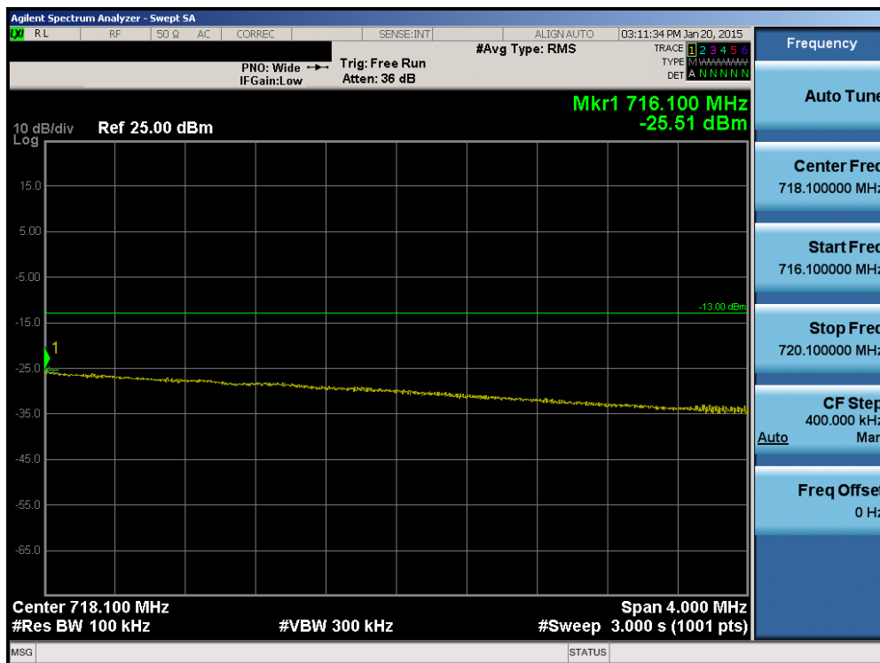
Plot 6-94. Upper Extended Band Edge Plot (Band 12 – 10.0MHz QPSK – RB Size 50)
