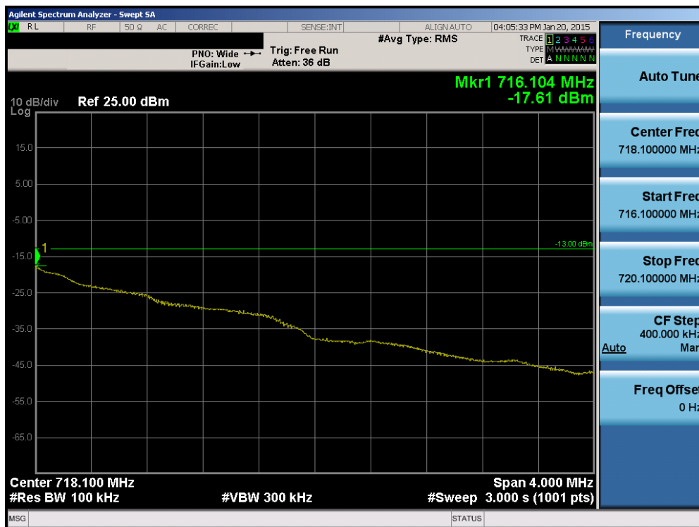
Plot 6-82. Upper Extended Band Edge Plot (Band 12 – 1.4MHz QPSK – RB Size 6)
