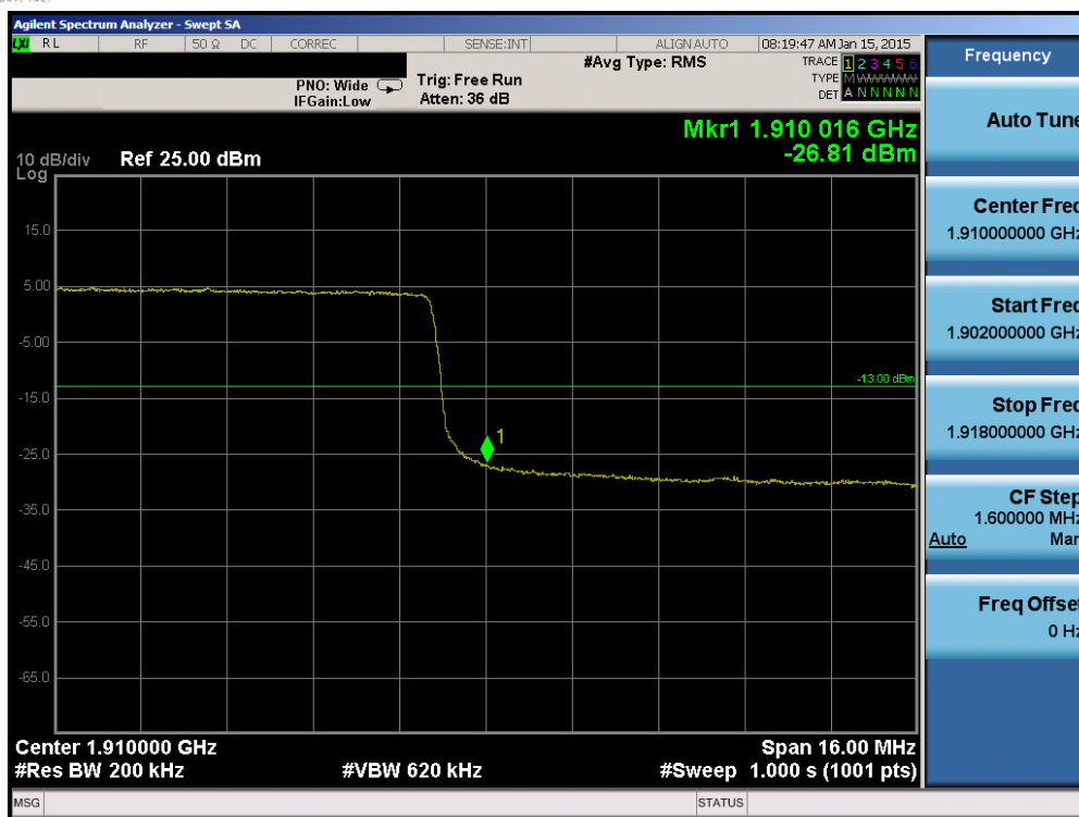
Plot 6-157. Upper Band Edge Plot (Band 2 – 20.0MHz QPSK – RB Size 100)
