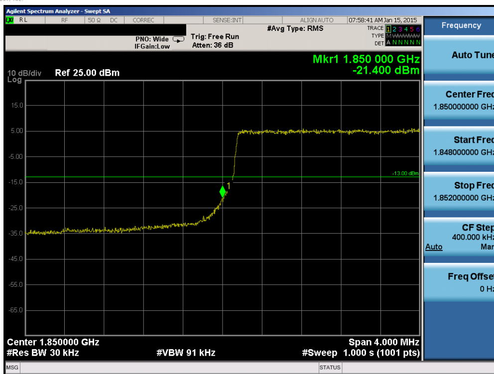
Plot 6-139. Lower Band Edge Plot (Band 2 – 3.0MHz QPSK – RB Size 15)
