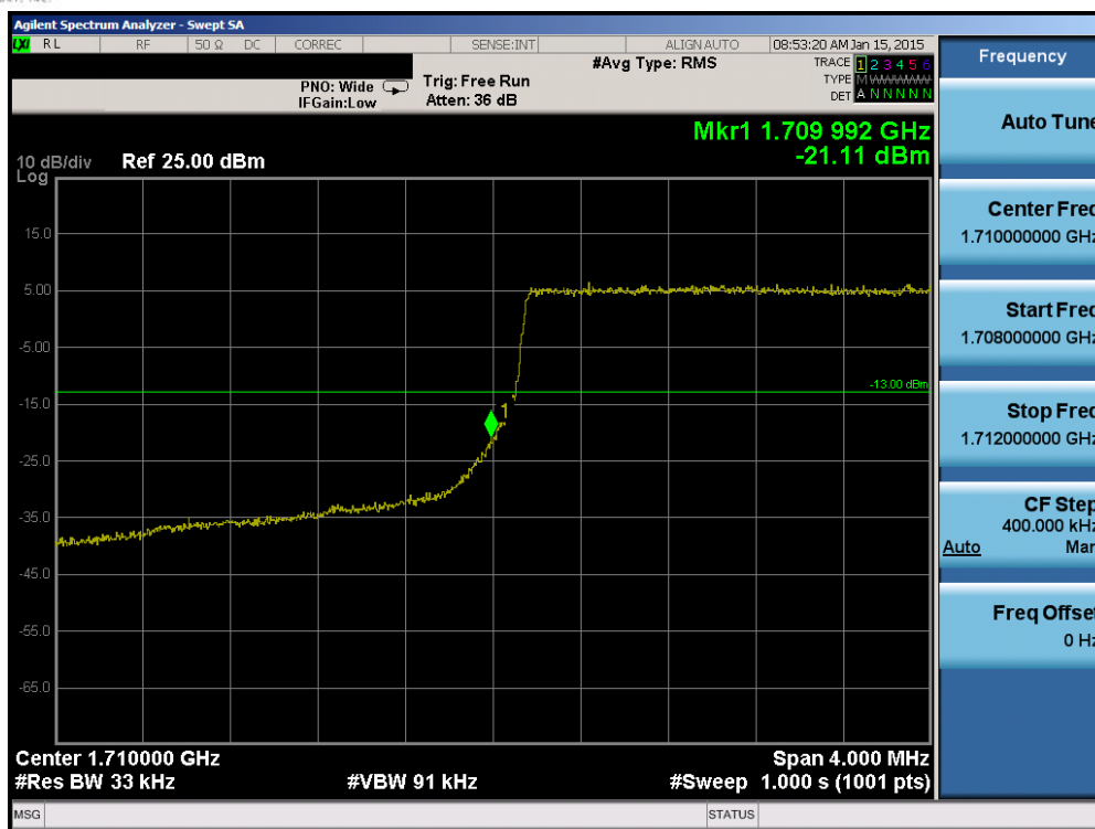
Plot 6-115. Lower Band Edge Plot (Band 4 – 3.0MHz QPSK – RB Size 15)
