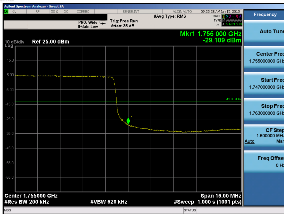
Plot 6-133. Upper Band Edge Plot (Band 4 – 20.0MHz QPSK – RB Size 100)
