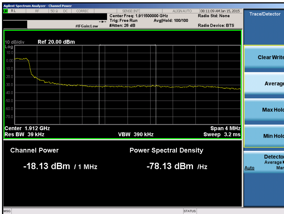
Plot 6-146. Upper Extended Band Edge Plot (Band 2 – 5.0MHz QPSK – RB Size 25)
