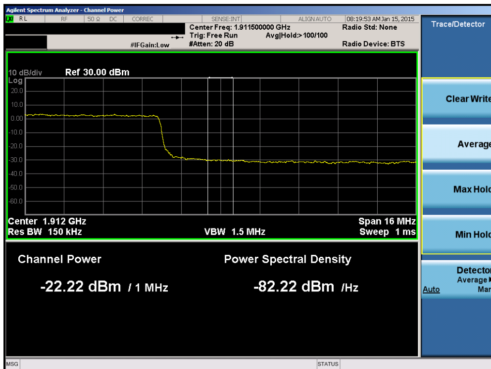
Plot 6-158. Upper Extended Band Edge Plot (Band 2 – 20.0MHz QPSK – RB Size 100)
