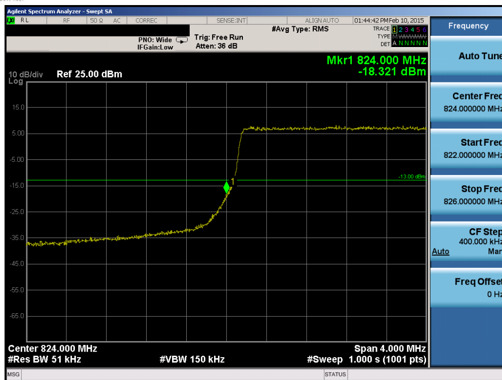
Plot 6-99. Lower Band Edge Plot (Band 5/26 – 3.0MHz QPSK – RB Size 15)
