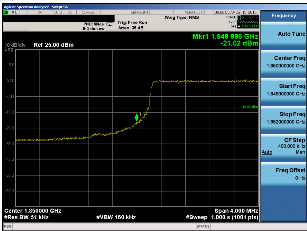
Plot 6-143. Lower Band Edge Plot (Band 2 – 5.0MHz QPSK – RB Size 25)
