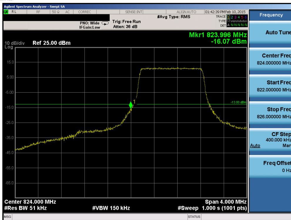
Plot 6-95. Lower Band Edge Plot (Band 5/26 – 1.4MHz QPSK – RB Size 6)
