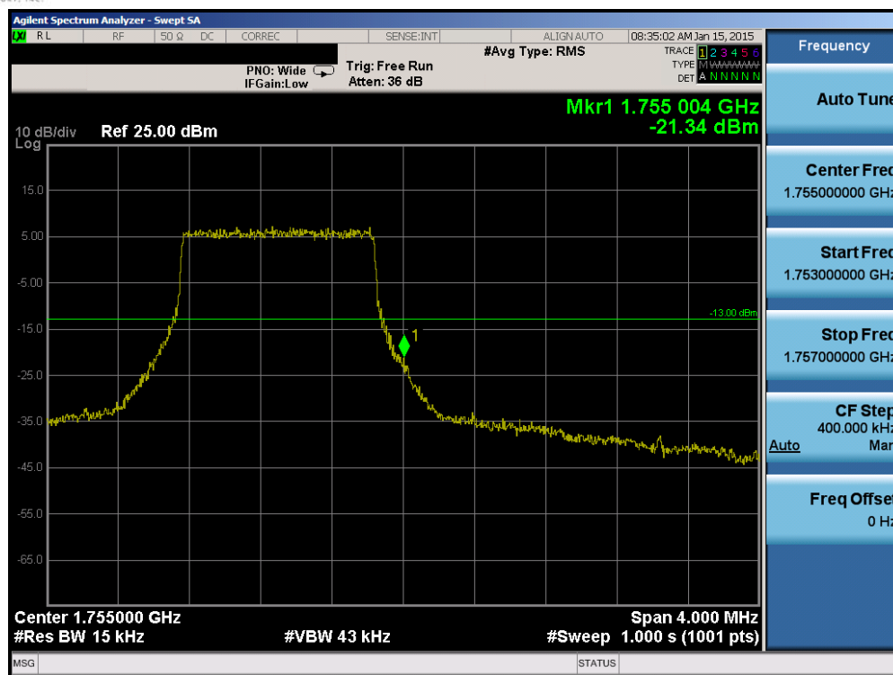
Plot 6-113. Upper Band Edge Plot (Band 4 – 1.4MHz QPSK – RB Size 6)
