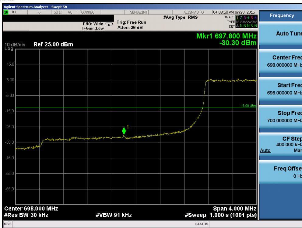
Plot 6-83. Lower Band Edge Plot (Band 12 – 3.0MHz QPSK – RB Size 15)
