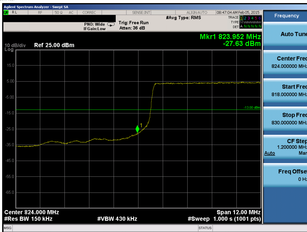
Plot 6-109. Lower Band Edge Plot (Band 26 – 15.0MHz QPSK – RB Size 75)
