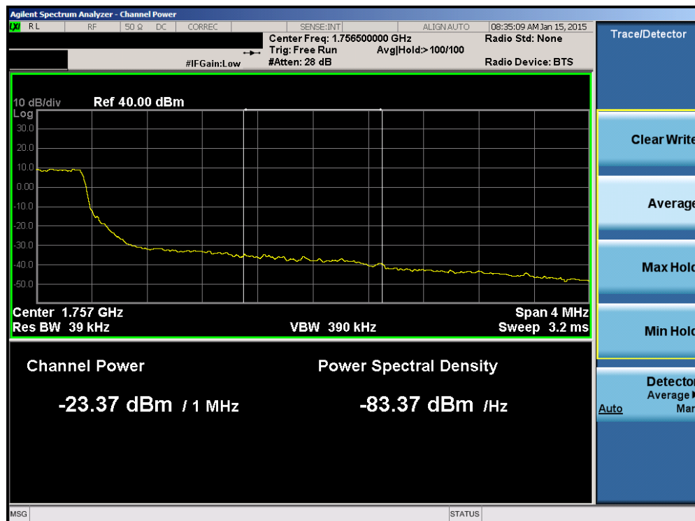
Plot 6-114. Upper Extended Band Edge Plot (Band 4 – 1.4MHz QPSK – RB Size 6)
