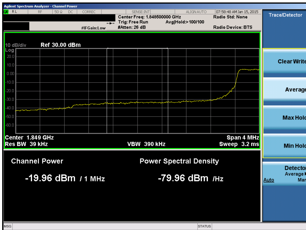
Plot 6-140. Lower Extended Band Edge Plot (Band 2 – 3.0MHz QPSK – RB Size 15)
