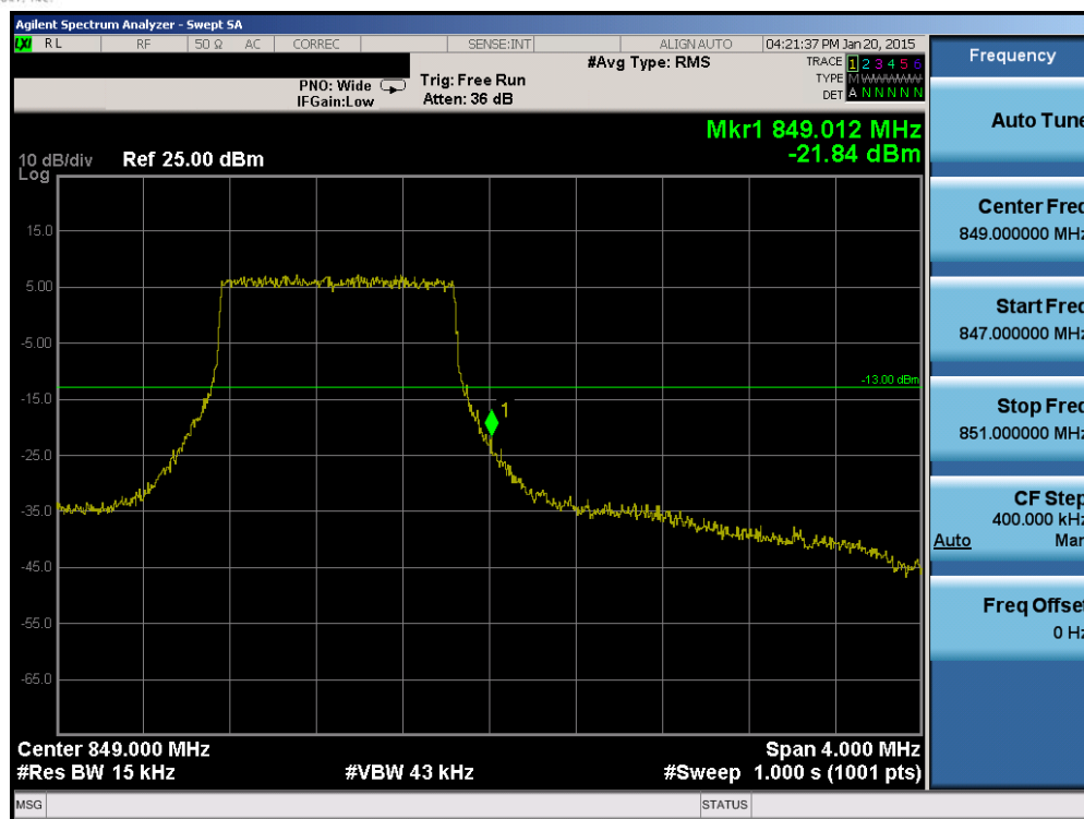
Plot 6-97. Upper Band Edge Plot (Band 5/26 – 1.4MHz QPSK – RB Size 6)
