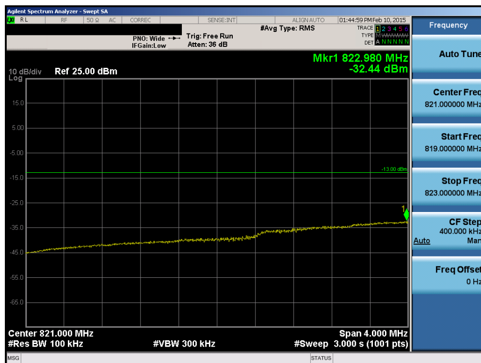
Plot 6-100. Lower Extended Band Edge Plot (Band 5/26 – 3.0MHz QPSK – RB Size 15)
