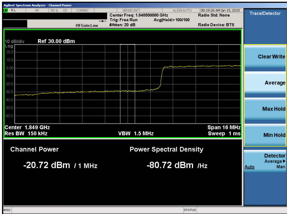
Plot 6-156. Lower Extended Band Edge Plot (Band 2 – 20.0MHz QPSK – RB Size 100)
