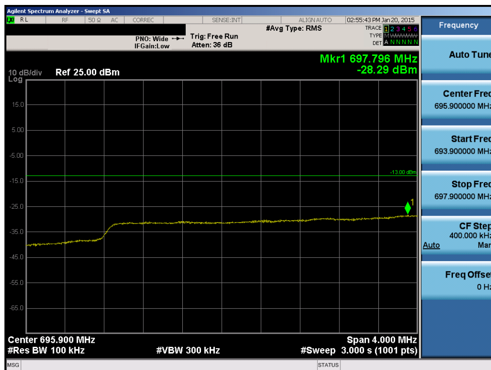
Plot 6-88. Lower Extended Band Edge Plot (Band 12 – 5.0MHz QPSK – RB Size 25)
