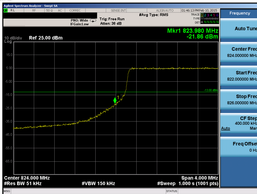
Plot 6-103. Lower Band Edge Plot (Band 5/26 - 5.0MHz QPSK - RB Size 25)
