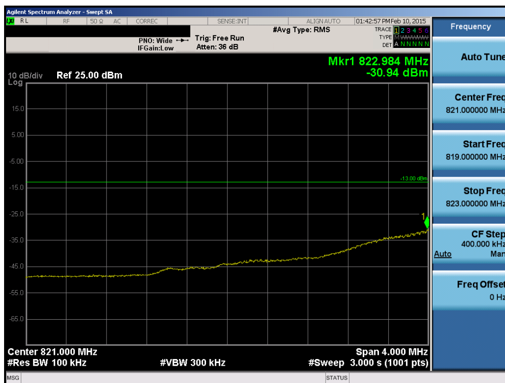
Plot 6-96. Lower Extended Band Edge Plot (Band 5/26 – 1.4MHz QPSK – RB Size 6)
