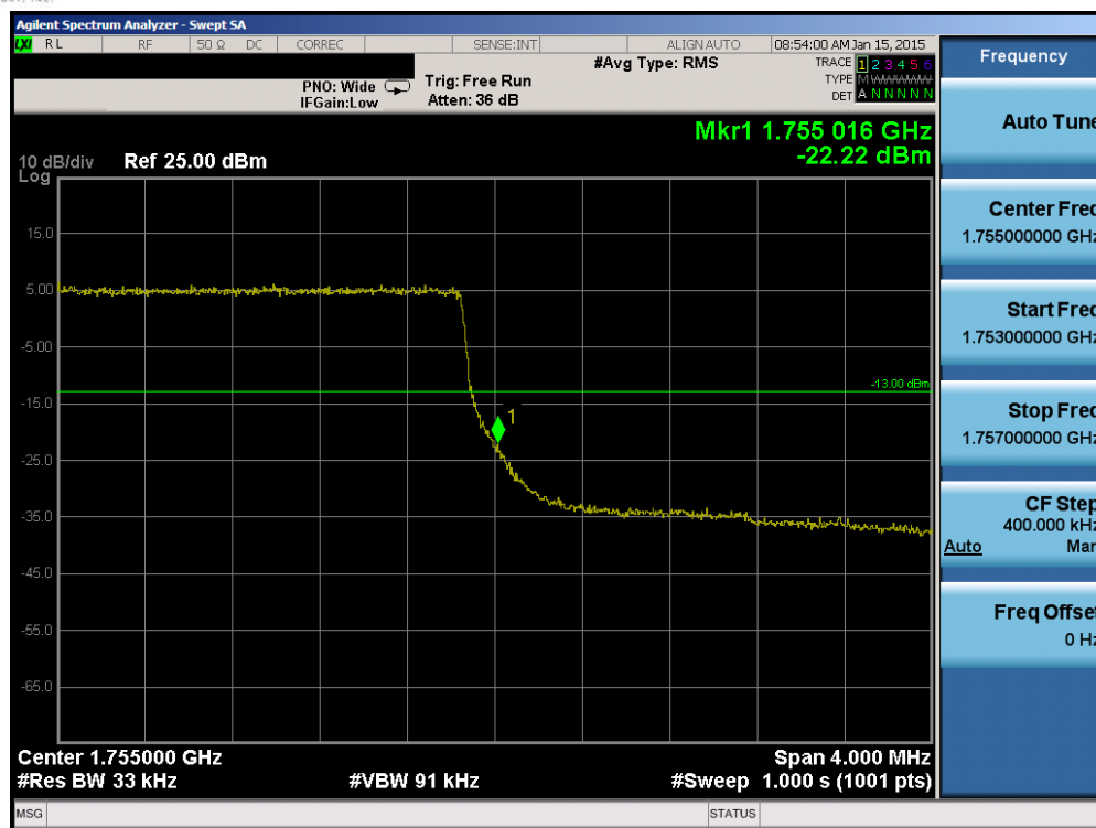
Plot 6-117. Upper Band Edge Plot (Band 4 – 3.0MHz QPSK – RB Size 15)
