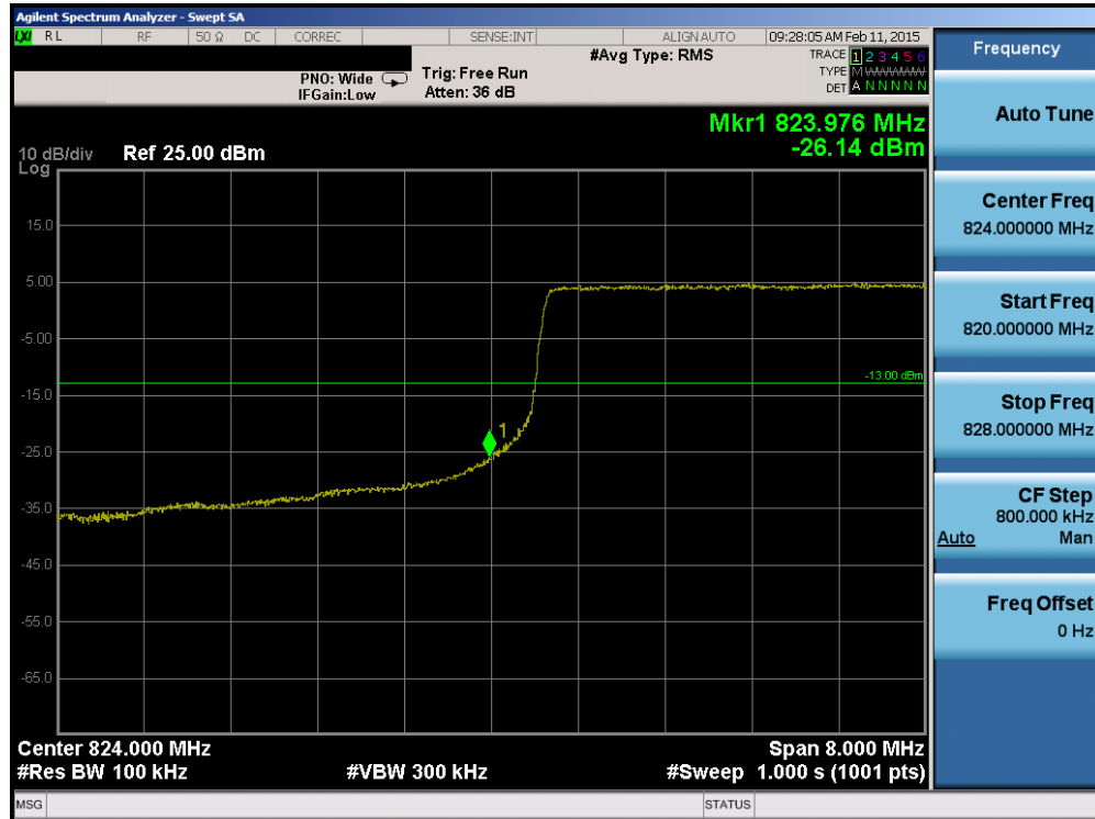
Plot 6-107. Lower Band Edge Plot (Band 5/26 – 10.0MHz QPSK – RB Size 50)
