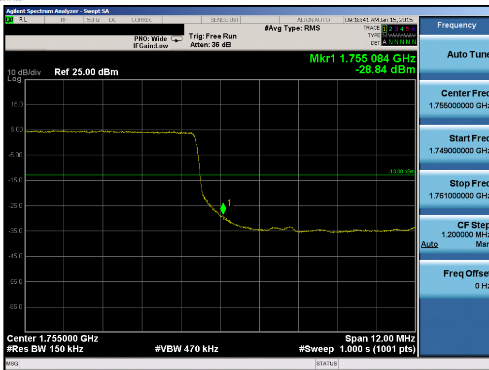
Plot 6-129. Upper Band Edge Plot (Band 4 – 15.0MHz QPSK – RB Size 75)
