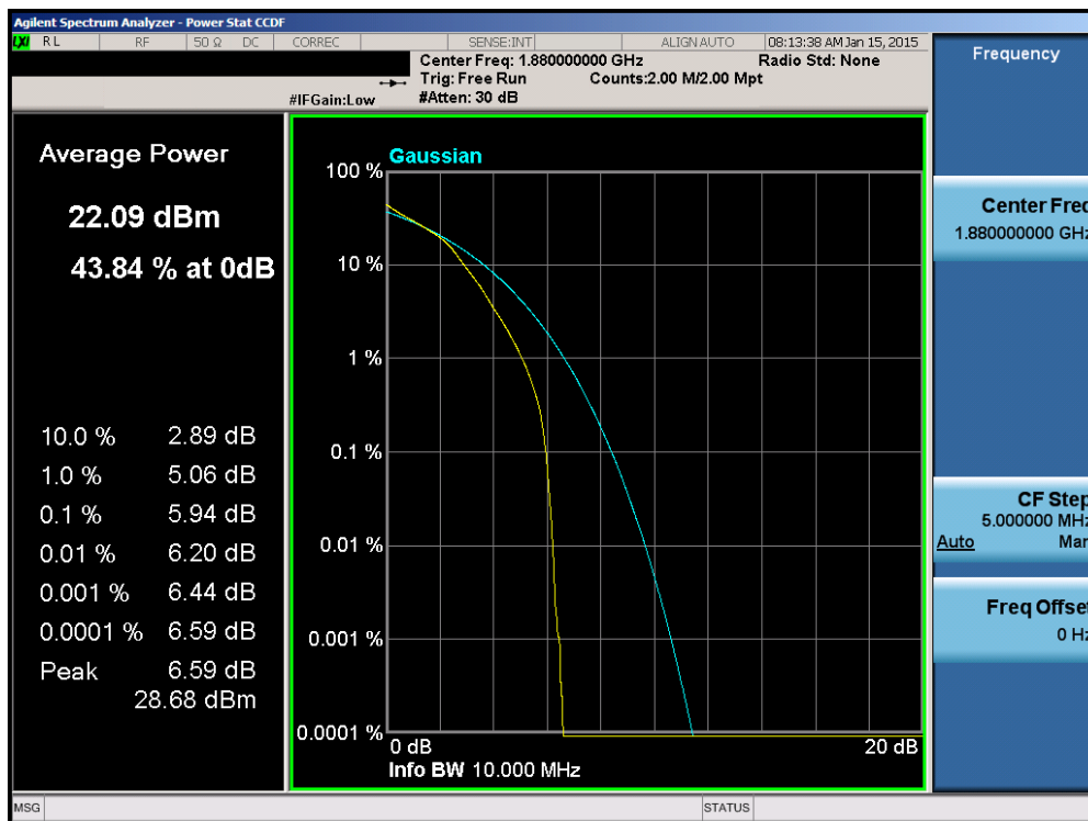
Plot 6-166. PAR Plot (Band 2 – 10.0MHz 16-QAM – RB Size 50)
