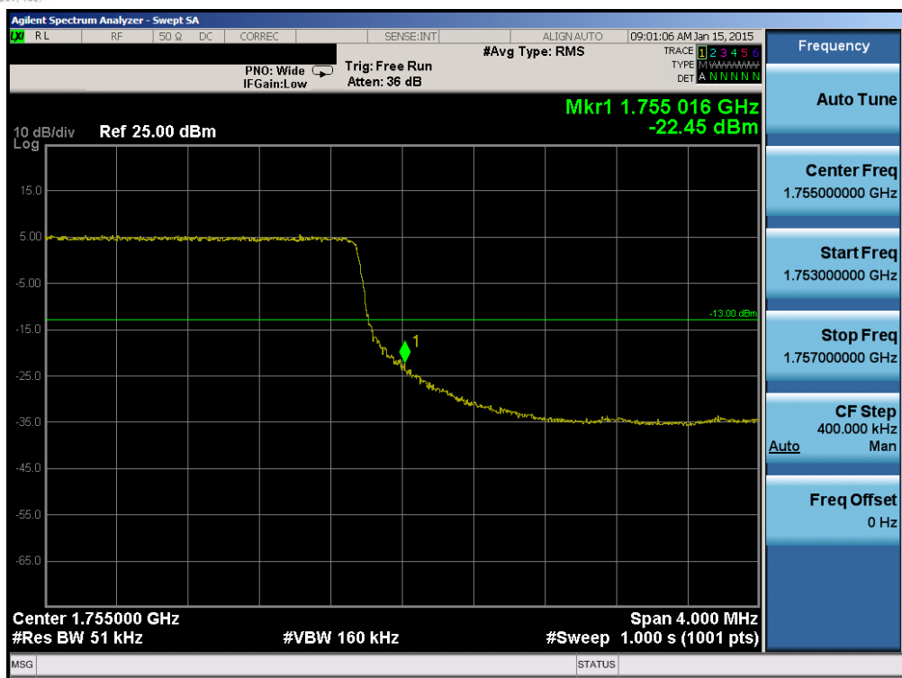
Plot 6-121. Upper Band Edge Plot (Band 4 – 5.0MHz QPSK – RB Size 25)
