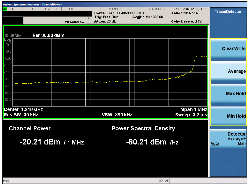
Plot 6-144. Lower Extended Band Edge Plot (Band 2 – 5.0MHz QPSK – RB Size 25)
