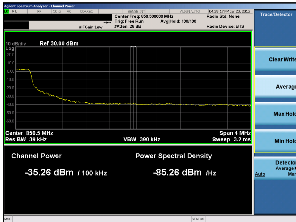
Plot 6-106. Upper Extended Band Edge Plot (Band 5/26 – 5.0MHz QPSK – RB Size 25)
