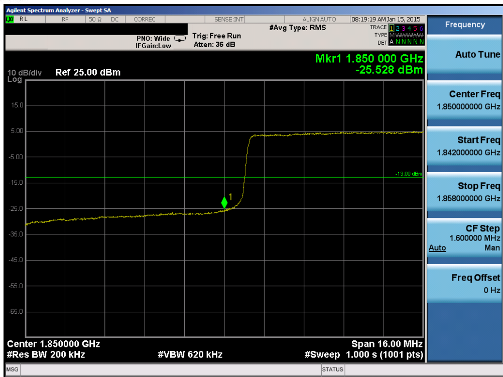
Plot 6-155. Lower Band Edge Plot (Band 2 – 20.0MHz QPSK – RB Size 100)
