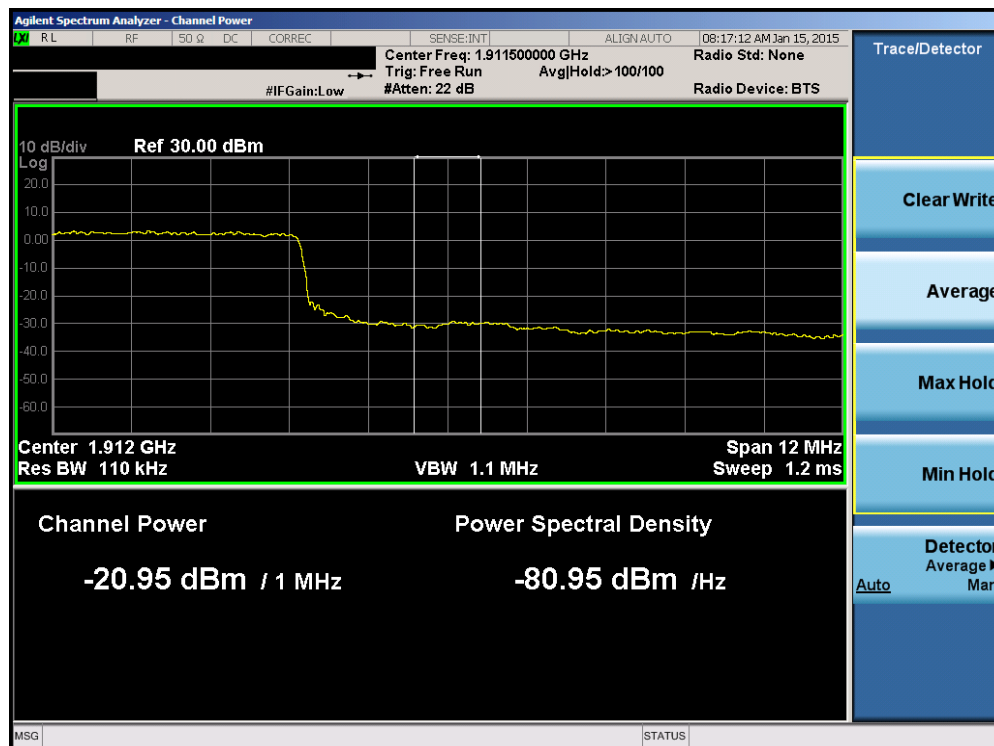
Plot 6-154. Upper Extended Band Edge Plot (Band 2 – 15.0MHz QPSK – RB Size 75)
