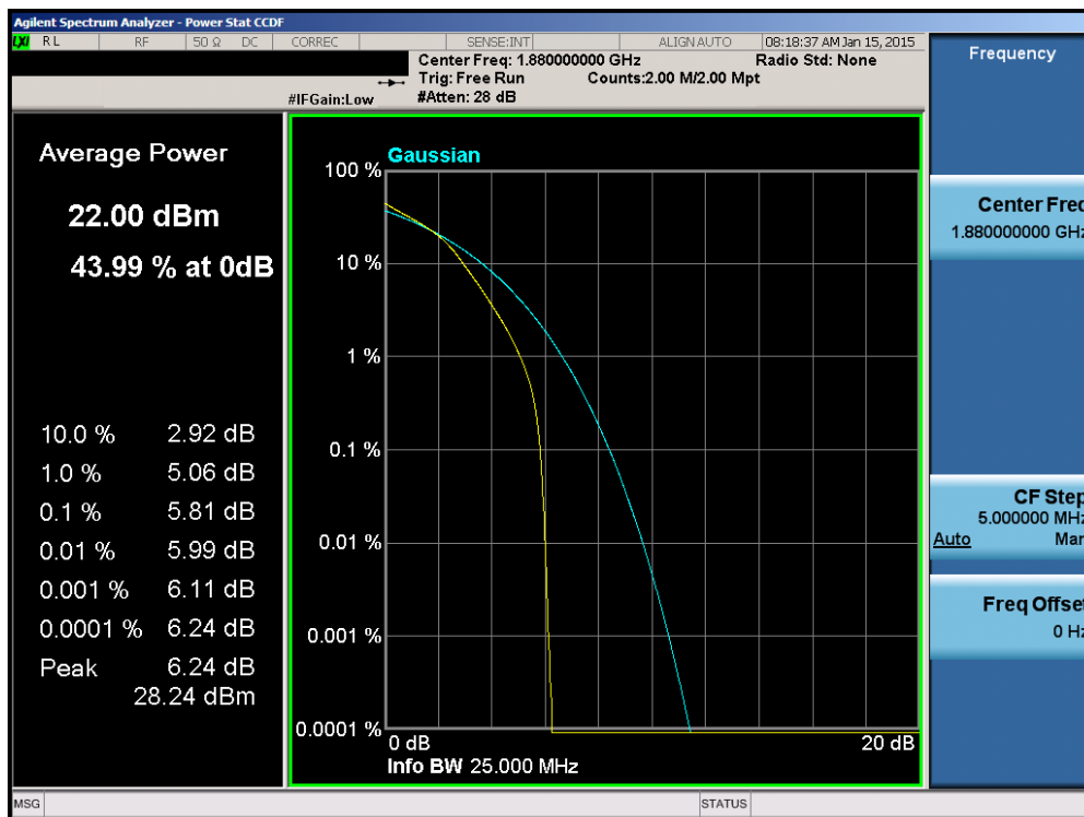
Plot 6-170. PAR Plot (Band 2 – 20.0MHz 16-QAM – RB Size 100)
