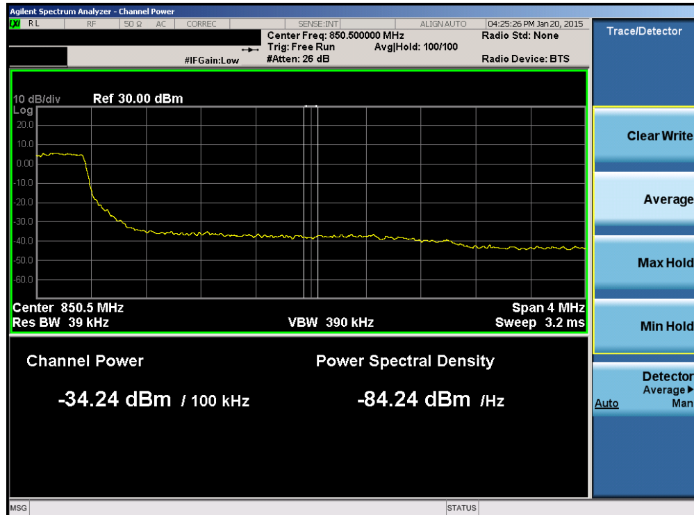
Plot 6-102. Upper Extended Band Edge Plot (Band 5/26 – Band 5 – 3.0MHz QPSK – RB Size 15)
