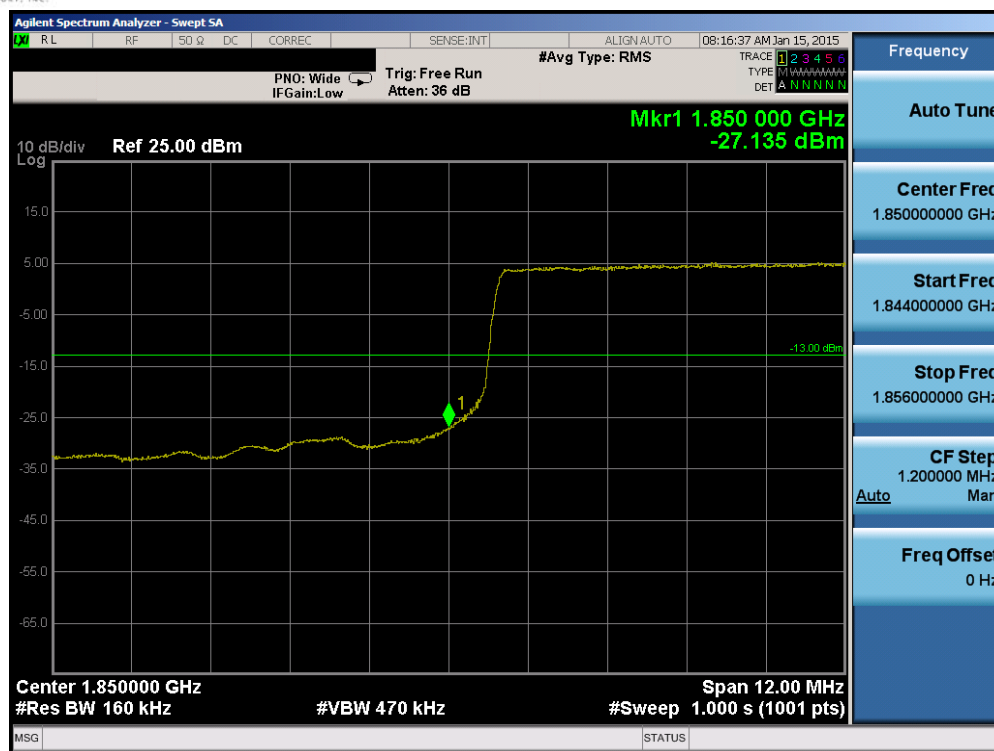
Plot 6-151. Lower Band Edge Plot (Band 2 – 15.0MHz QPSK – RB Size 75)
