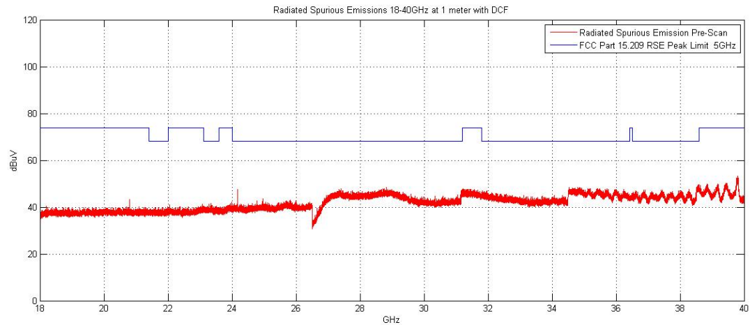
Plot 6-162. Radiated Spurious Plot above 18GHz (802.11a – Ant. Pol. V)
