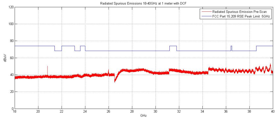
Plot 6-161. Radiated Spurious Plot above 18GHz (802.11a – Ant. Pol. H)
