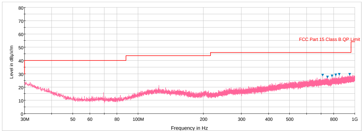
Plot 6-237. Radiated Spurious Plot below 1GHz (802.11a – U3 Ch. 157, Ant. Pol. V)
