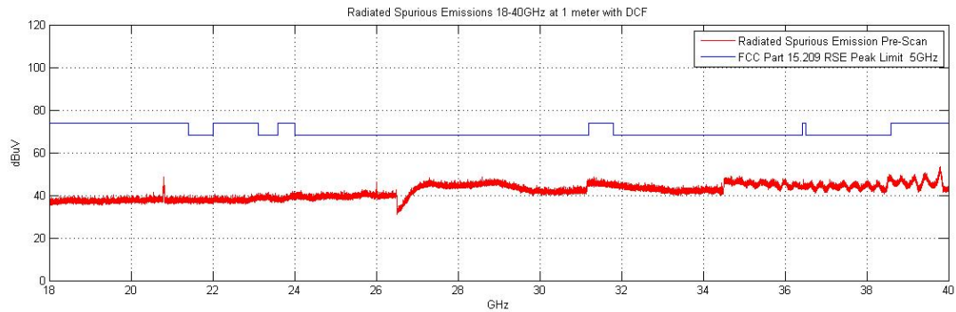
Plot 6-171. Radiated Spurious Plot above 18GHz (802.11a – Ant. Pol. H)
