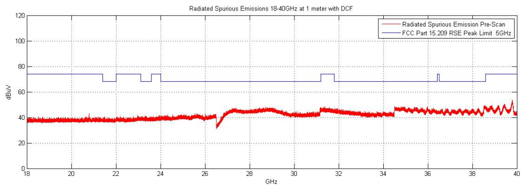
Plot 6-172. Radiated Spurious Plot above 18GHz (802.11a – Ant. Pol. V)
