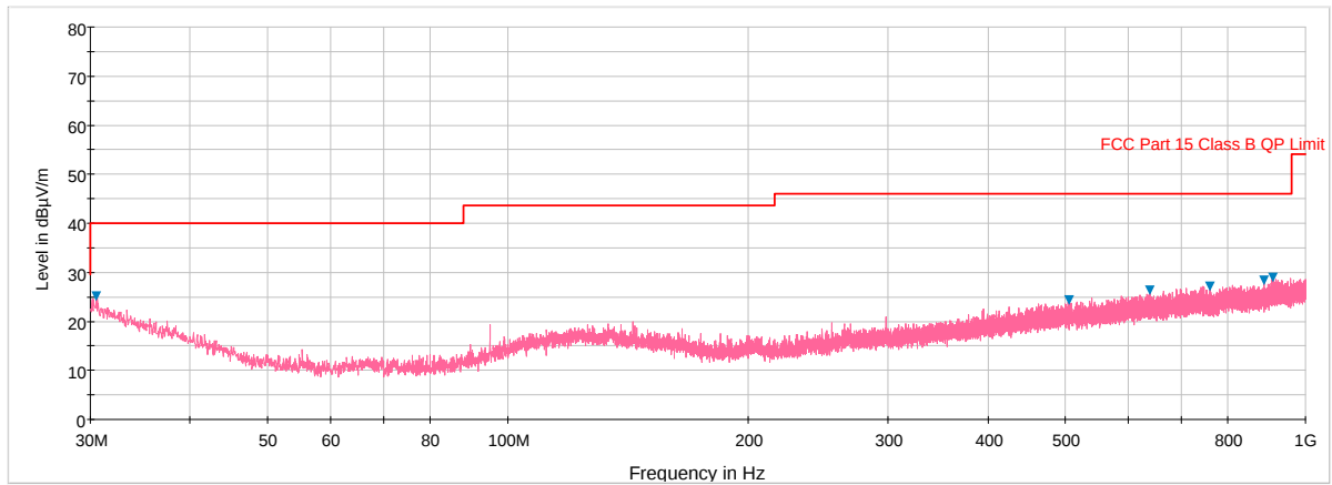
Plot 6-236. Radiated Spurious Plot below 1GHz (802.11a – U3 Ch. 157, Ant. Pol. H)
