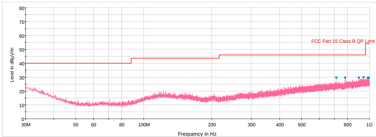
Plot 6-239. Radiated Spurious Plot below 1GHz (802.11a – U3 Ch. 157, Ant. Pol. V)
