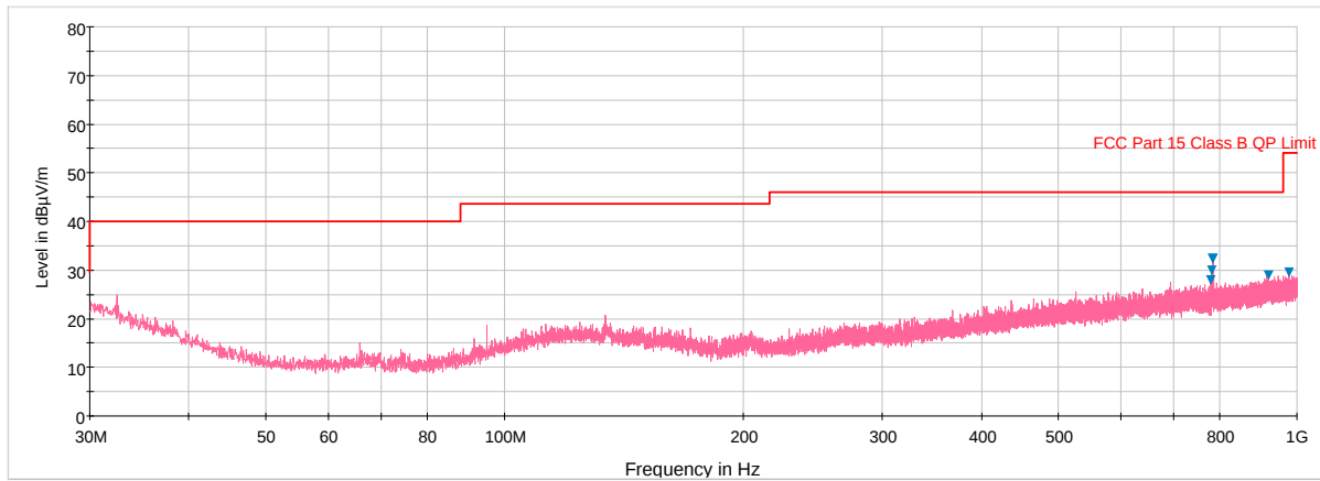
Plot 6-238. Radiated Spurious Plot below 1GHz (802.11a – U3 Ch. 157, Ant. Pol. H)
