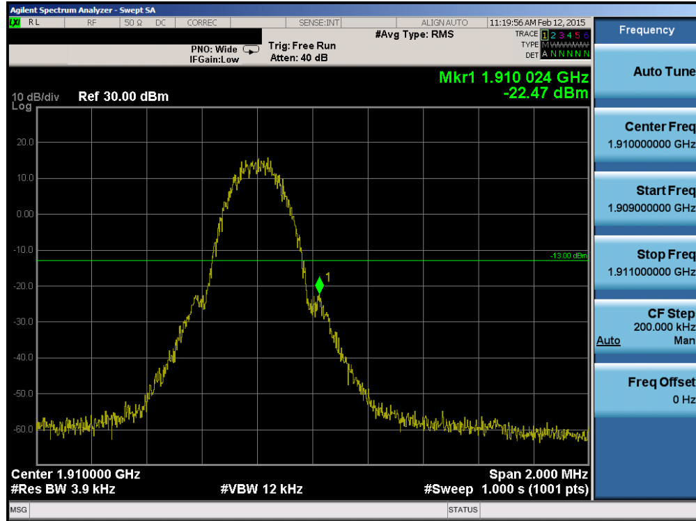
Plot 6-57. Band Edge Plot (PCS GSM Mode – Ch. 810)
