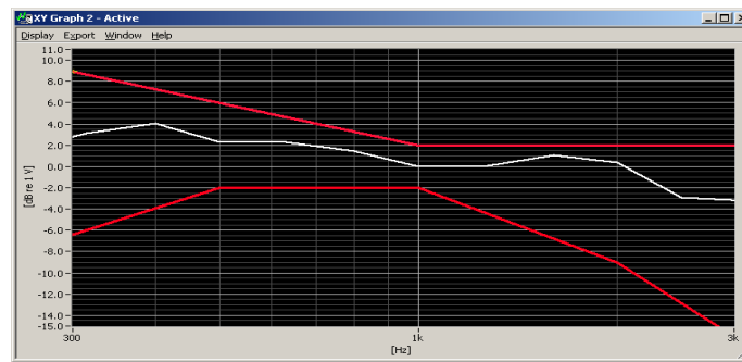
Figure 6-1 Axial Frequency Response
