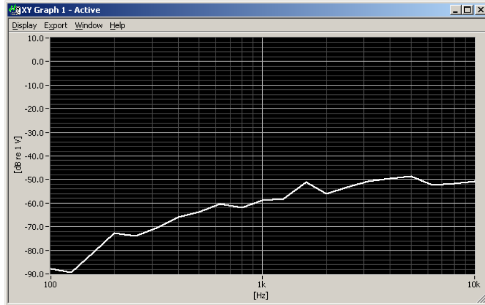
Figure 6-3 Worst-case ABM2 Plot for UMTS
