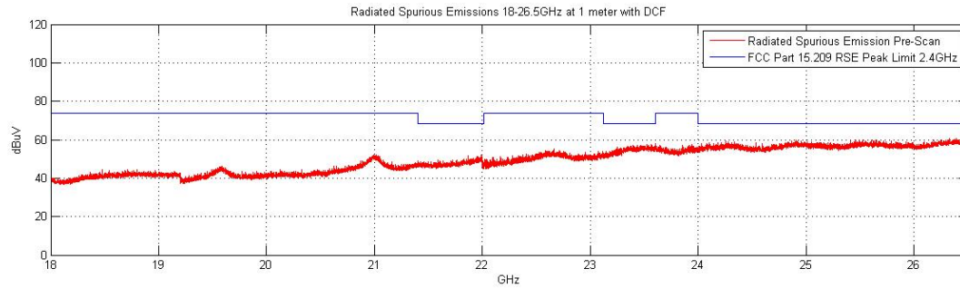
Plot 6-48. Radiated Spurious Plot above 18GHz (Pol. H)
