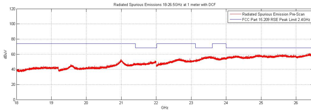
Plot 6-49. Radiated Spurious Plot above 18GHz (Pol. V)
