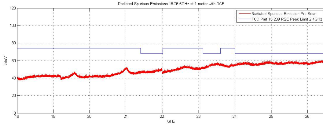
Plot 6-75. Radiated Spurious Plot above 18GHz (Pol. H)
