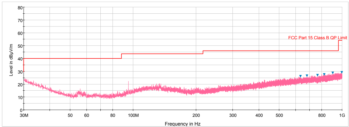
Plot 6-91. Radiated Spurious Plot below 1GHz (Pol. H)
