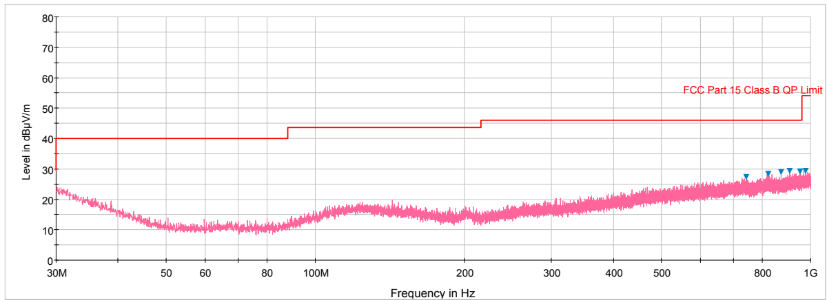
Plot 6-92. Radiated Spurious Plot below 1GHz (Pol. V)
