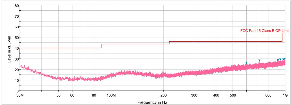
Plot 6-89. Radiated Spurious Plot below 1GHz (Pol. H)
