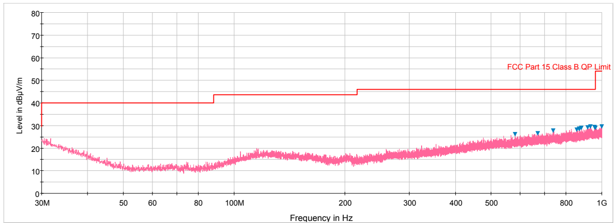
Plot 6-90. Radiated Spurious Plot below 1GHz (Pol. V)
