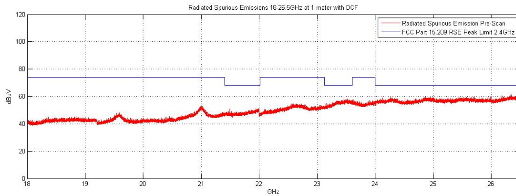
Plot 6-68. Radiated Spurious Plot above 18GHz (Pol. V)
