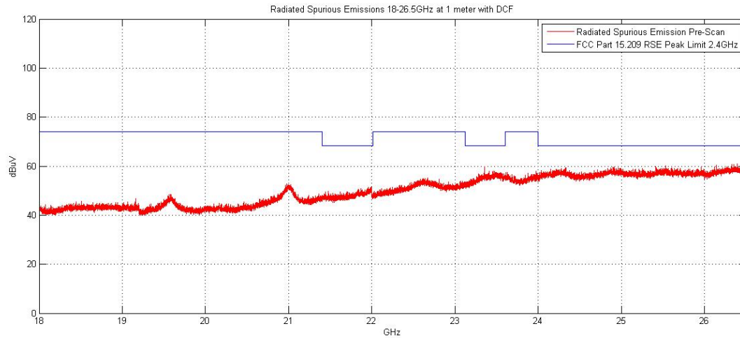
Plot 6-67. Radiated Spurious Plot above 18GHz (Pol. H)
