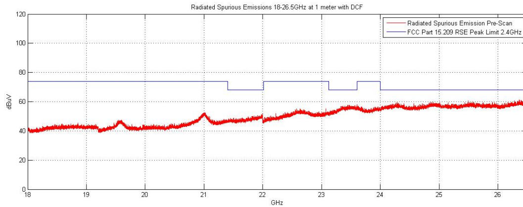
Plot 6-76. Radiated Spurious Plot above 18GHz (Pol. V)
