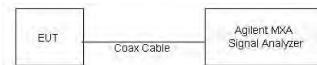
Figure 9-4 Power Measurement Setup for Bandwidths > 50 MHz
