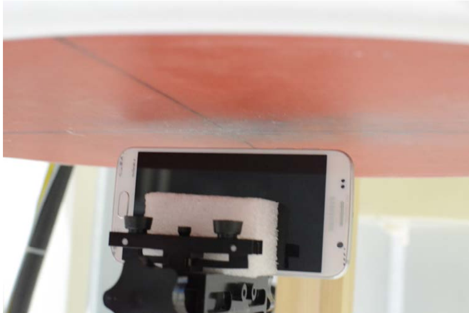
SAR Test Setup Photo 11: Left at 1.0 cm
