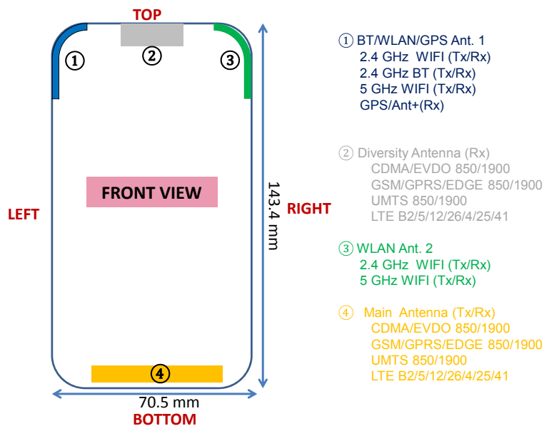
Figure F-1 DUT Antenna Locations
