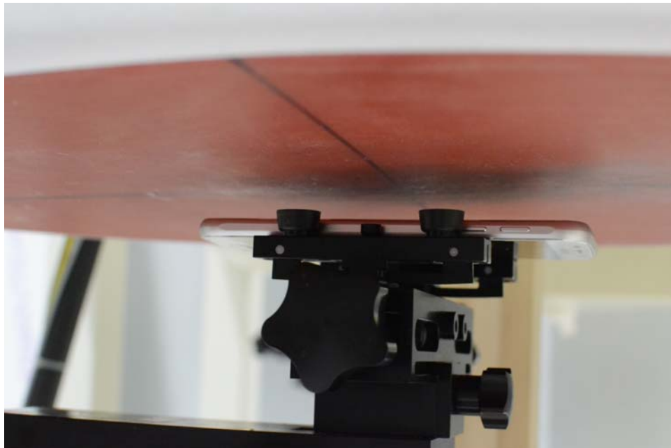
SAR Test Setup Photo 6: Back at 1.5 cm
