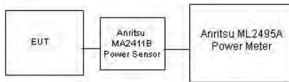
Figure 9-4 Power Measurement Setup
