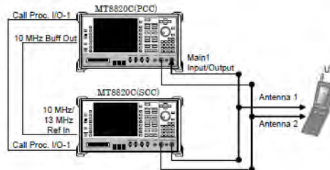
Figure 9-3 Power Measurement Setup
