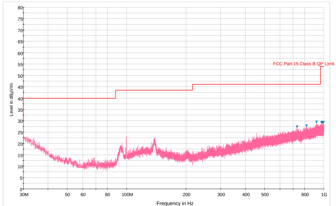
Plot 6-238. Radiated Spurious Plot below 1GHz (802.11a – U3 Ch. 157, Ant. Pol. H)
