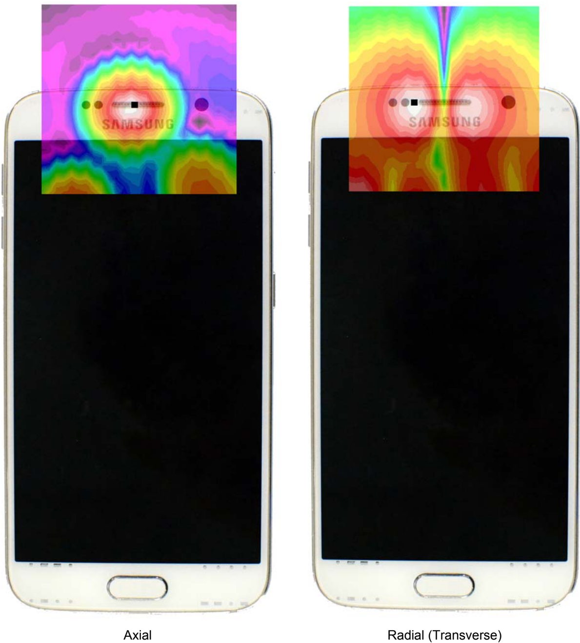
Figure 12-3 T-Coil Scan Overlay Magnetic Field Distributions
