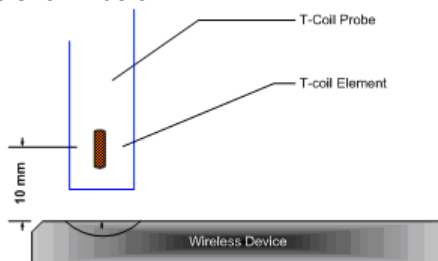
Figure 4-10 Measurement Distance
