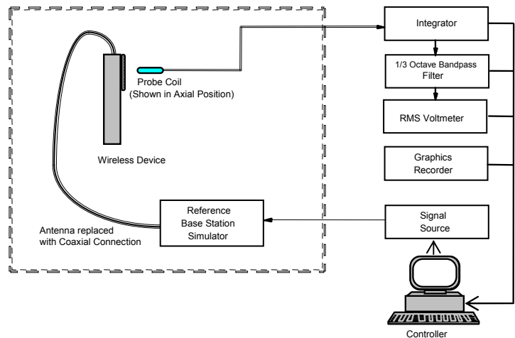
Figure 4-13 Audio Magnetic Field Test Setup
