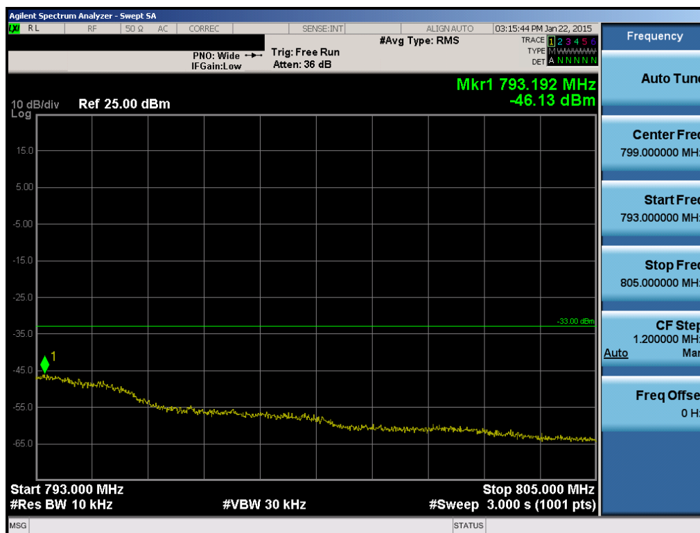
Plot 6-72. Upper Extended Band Edge Plot (Band 13 – 5.0MHz QPSK – RB Size 25)
