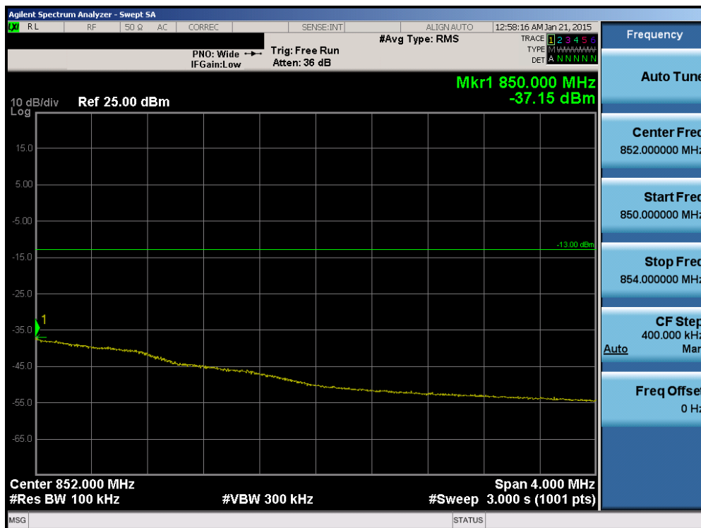
Plot 6-79. Upper Extended Band Edge Plot (Band 5 – 1.4MHz QPSK – RB Size 6)
