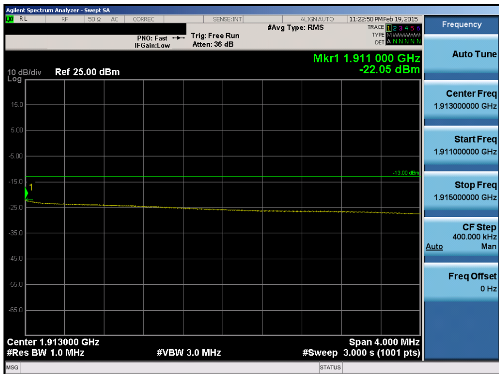
Plot 6-121. Upper Extended Band Edge Plot (Band 2 – 10.0MHz QPSK – RB Size 50)
