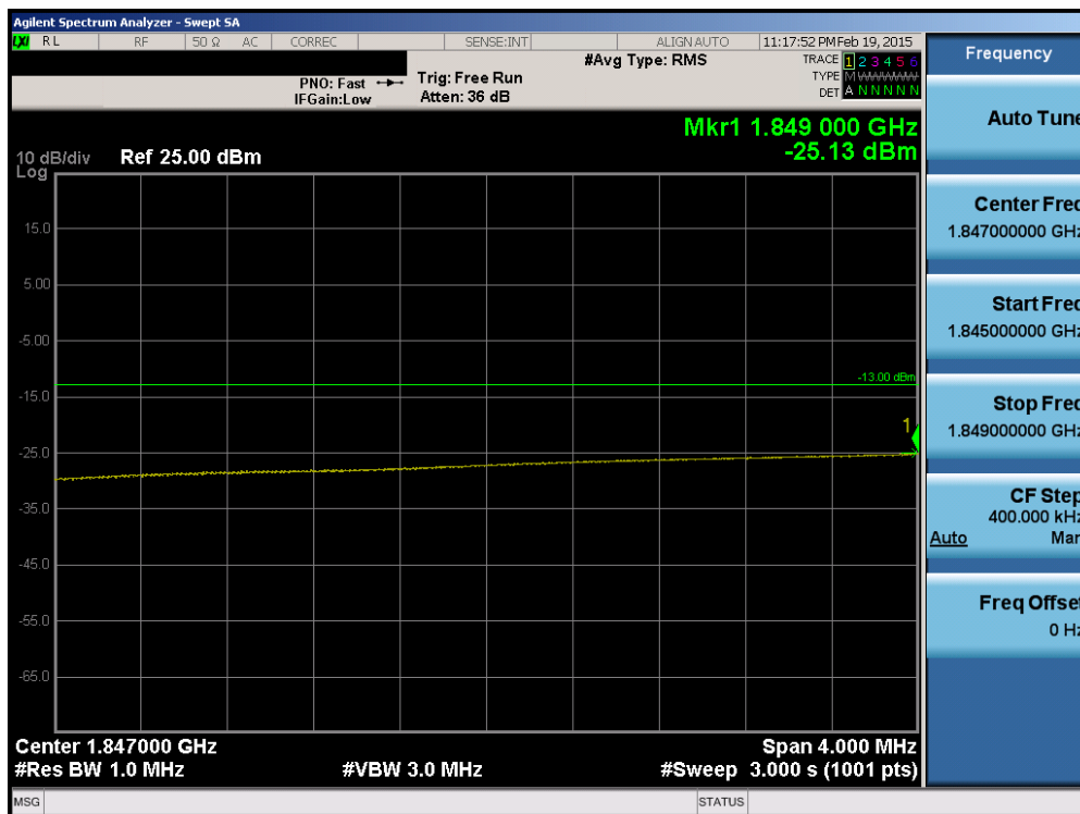
Plot 6-123. Lower Extended Band Edge Plot (Band 2 – 15.0MHz QPSK – RB Size 75)
