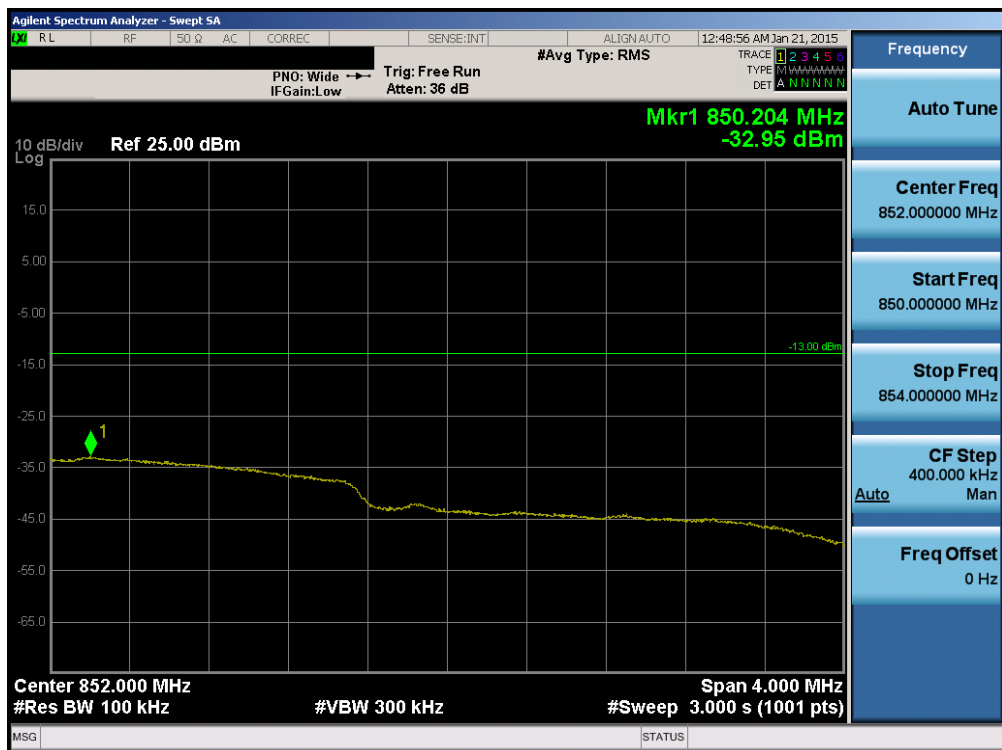
Plot 6-83. Upper Extended Band Edge Plot (Band 5 – Band 5 – 3.0MHz QPSK – RB Size 15)
