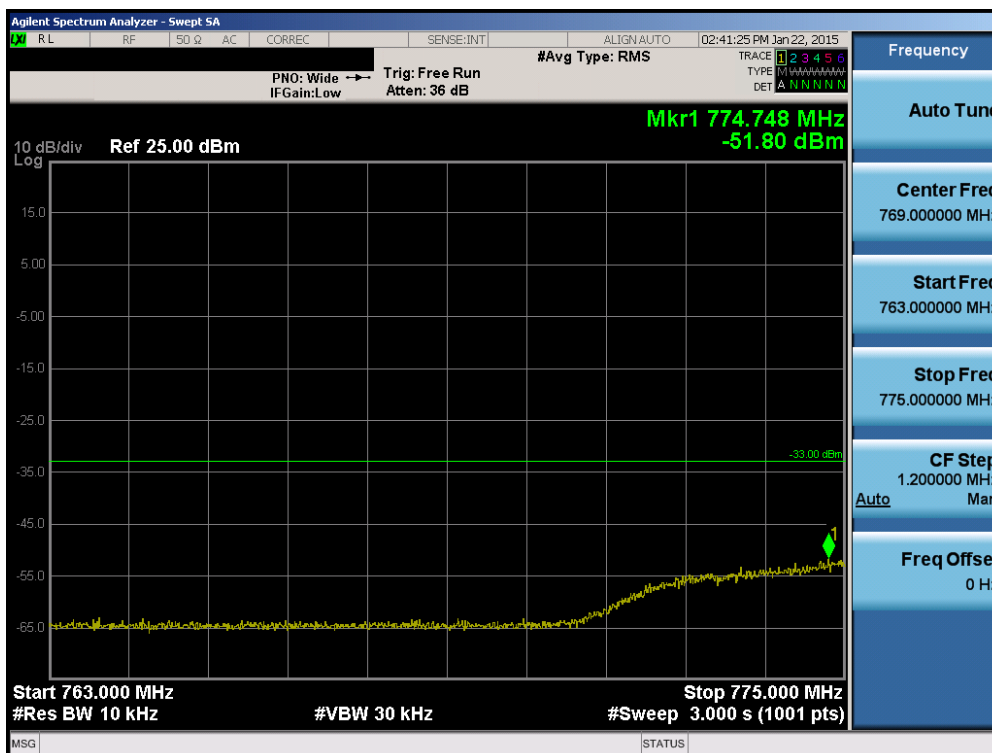
Plot 6-70. Lower Extended Band Edge Plot (Band 13 – 5.0MHz QPSK – RB Size 25)
