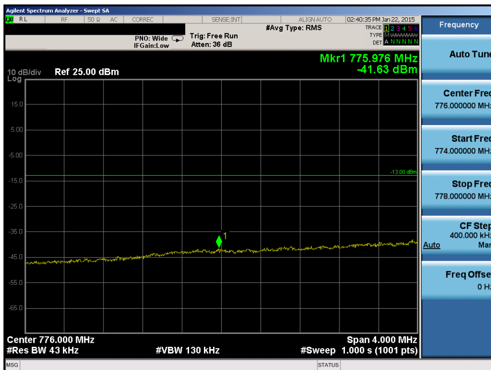
Plot 6-69. Lower Band Edge Plot (Band 13 – 5.0MHz QPSK – RB Size 25)
