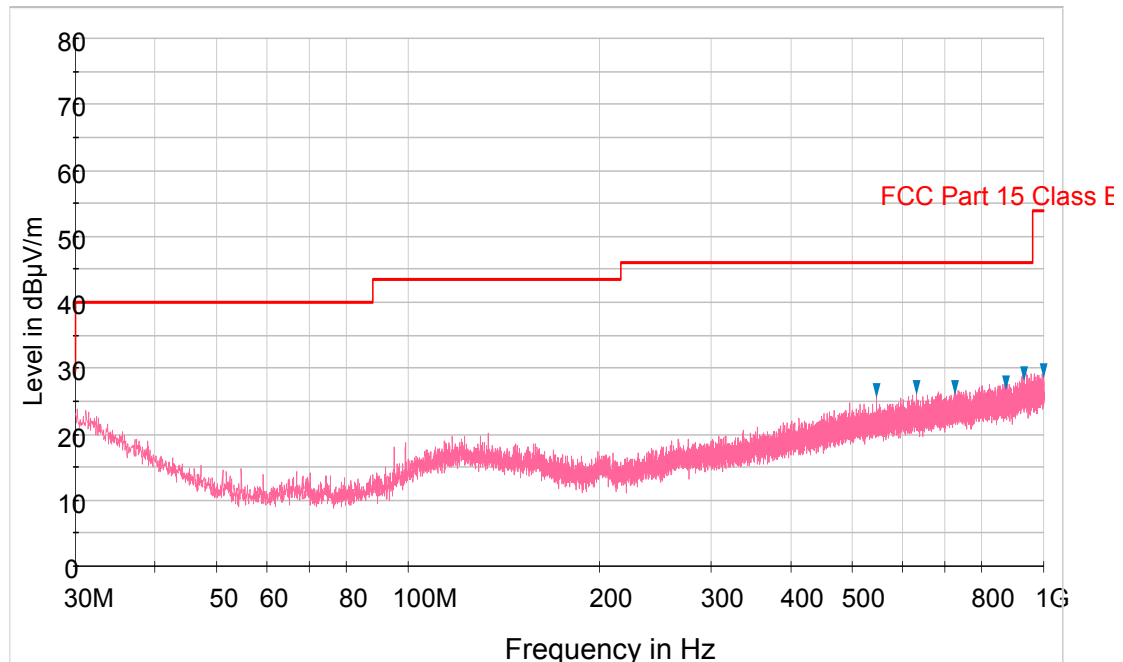
Plot 6-52. Radiated Spurious Plot below 1GHz (Pol. H)
