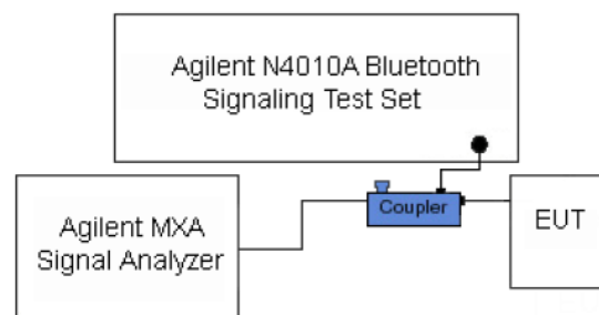
Figure 8-2 Power Measurement Setup
