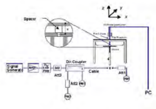
Figure 10-1 System Verification Setup Diagram
