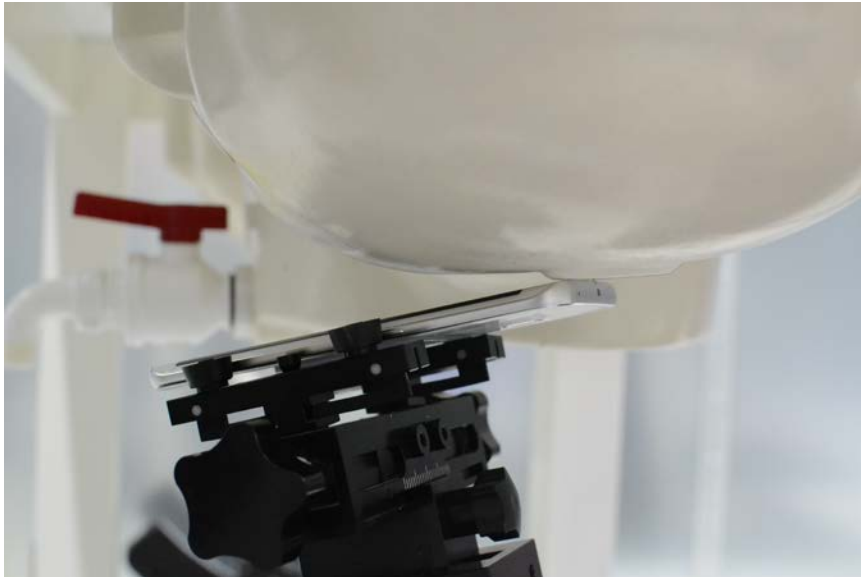
SAR Test Setup Photo 4: Left Tilt
