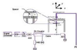
Figure 10-1 System Verification Setup Diagram
