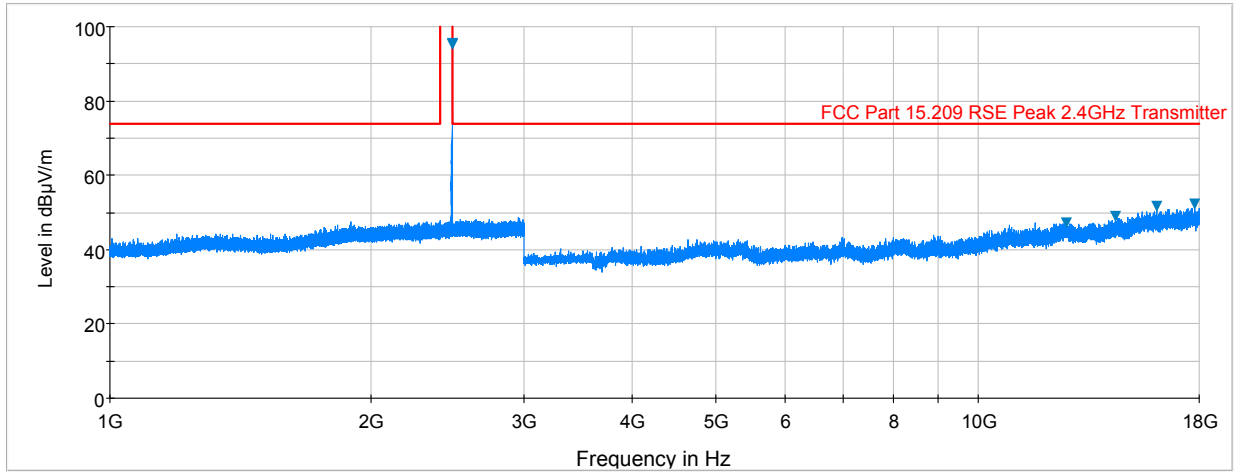
Plot 6-23. Radiated Spurious Plot above 1GHz (BTLE – Ch. 39, Ant. Pol. V)
