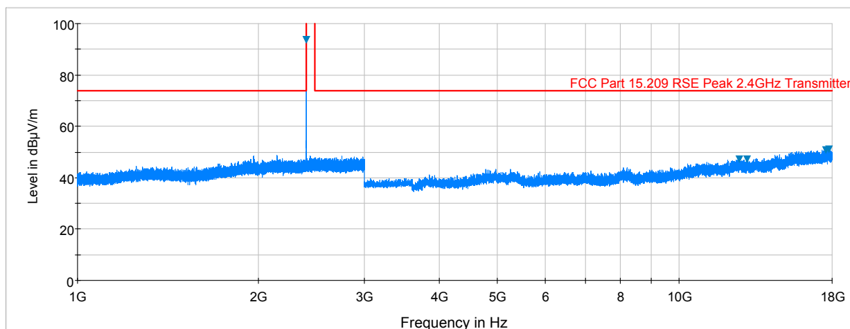
Plot 6-19. Radiated Spurious Plot above 1GHz (BTLE – Ch. 0, Ant. Pol. V)
