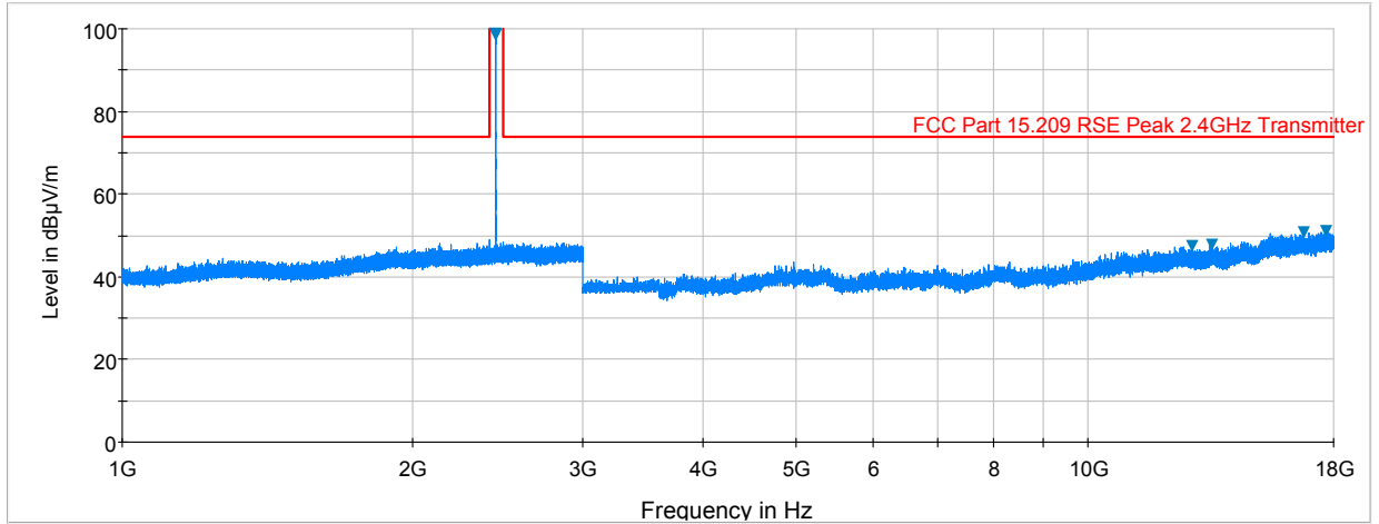
Plot 6-20. Radiated Spurious Plot above 1GHz (BTLE – Ch. 19, Ant. Pol. H)
