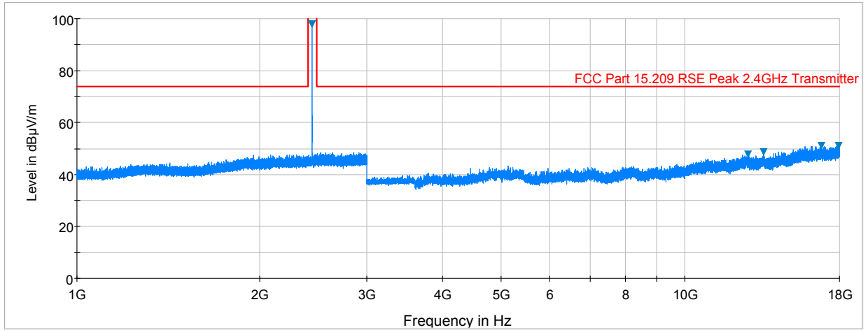
Plot 6-21. Radiated Spurious Plot above 1GHz (BTLE – Ch. 19, Ant. Pol. V)
