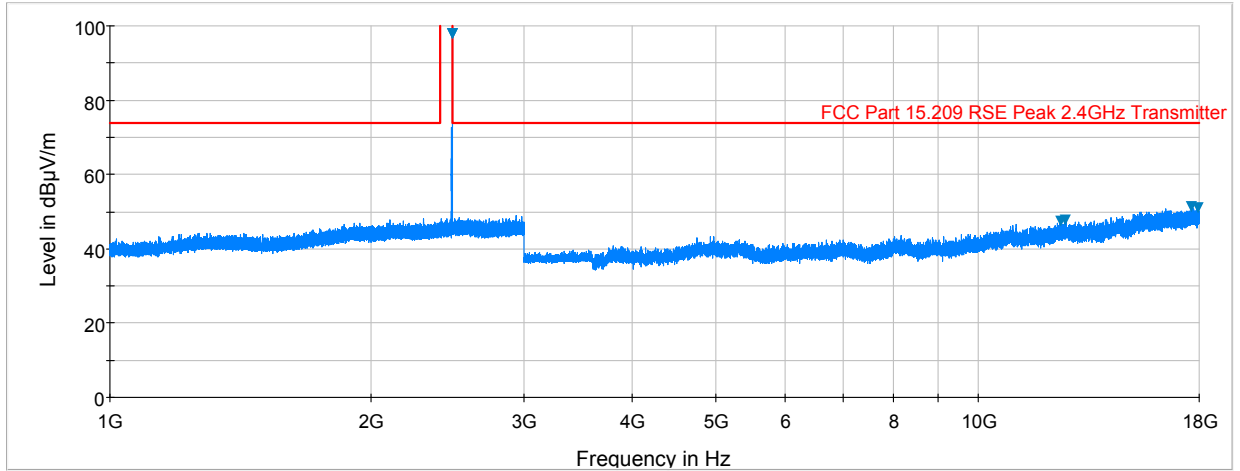
Plot 6-22. Radiated Spurious Plot above 1GHz (BTLE – Ch. 39, Ant. Pol. H)
