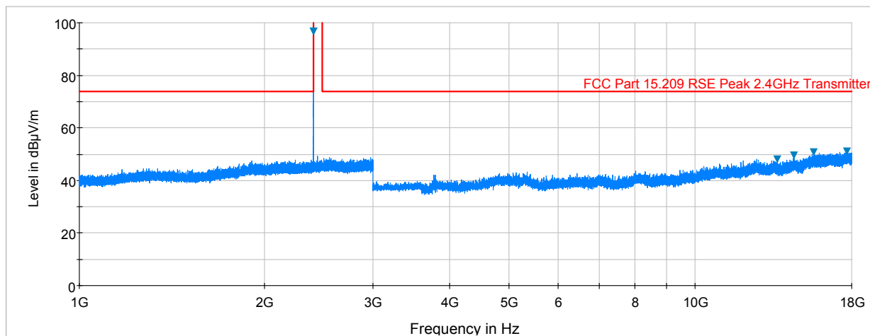
Plot 6-18. Radiated Spurious Plot above 1GHz (BTLE – Ch. 0, Ant. Pol. H)
