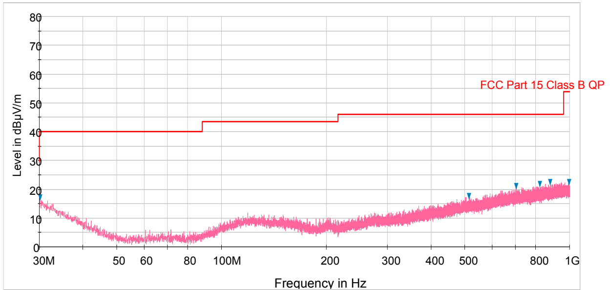
Plot 6-52. Radiated Spurious Plot below 1GHz (Pol. H)
