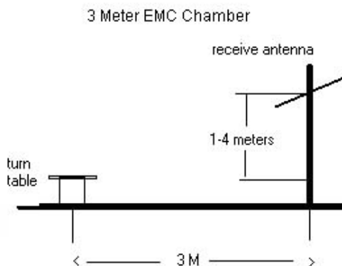
Figure 6-3. Test Instrument & Measurement Setup
