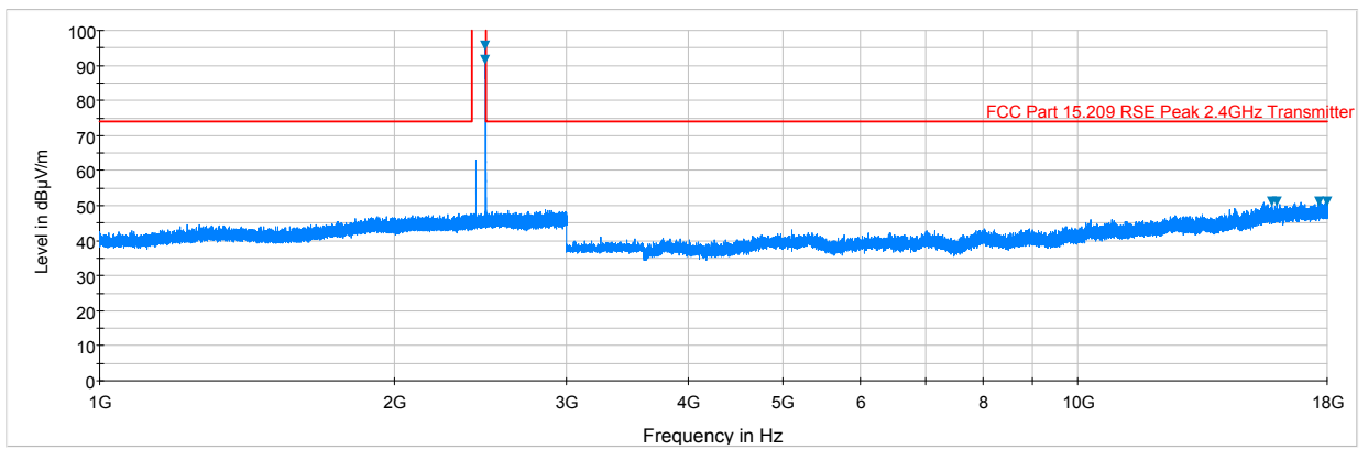
Plot 6-47. Radiated Spurious Plot above 1GHz (BT – Ch. 78, Ant. Pol. V)
