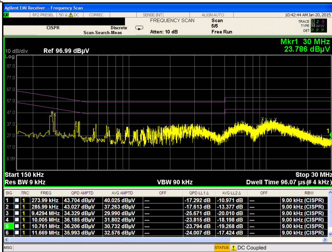
Plot 6-55. Line-Conducted Test Plot (N)
