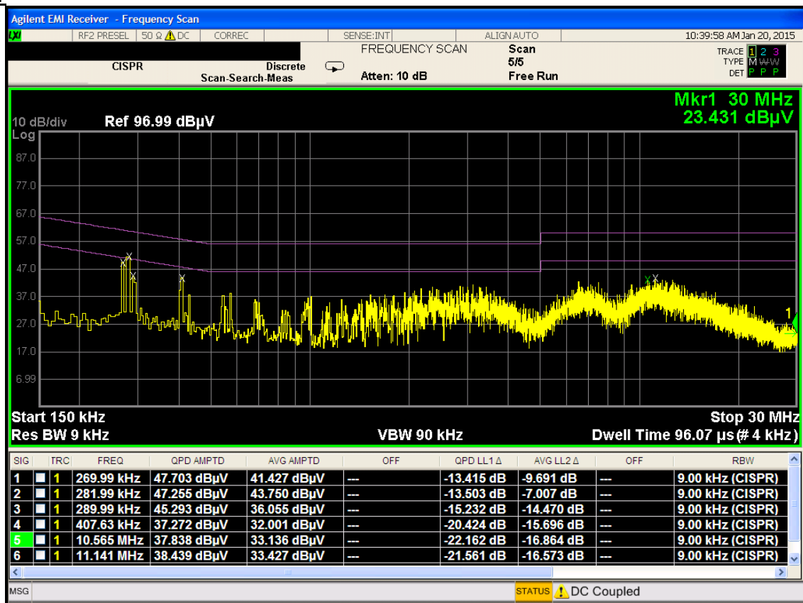
Plot 6-54. Line-Conducted Test Plot (L1)
