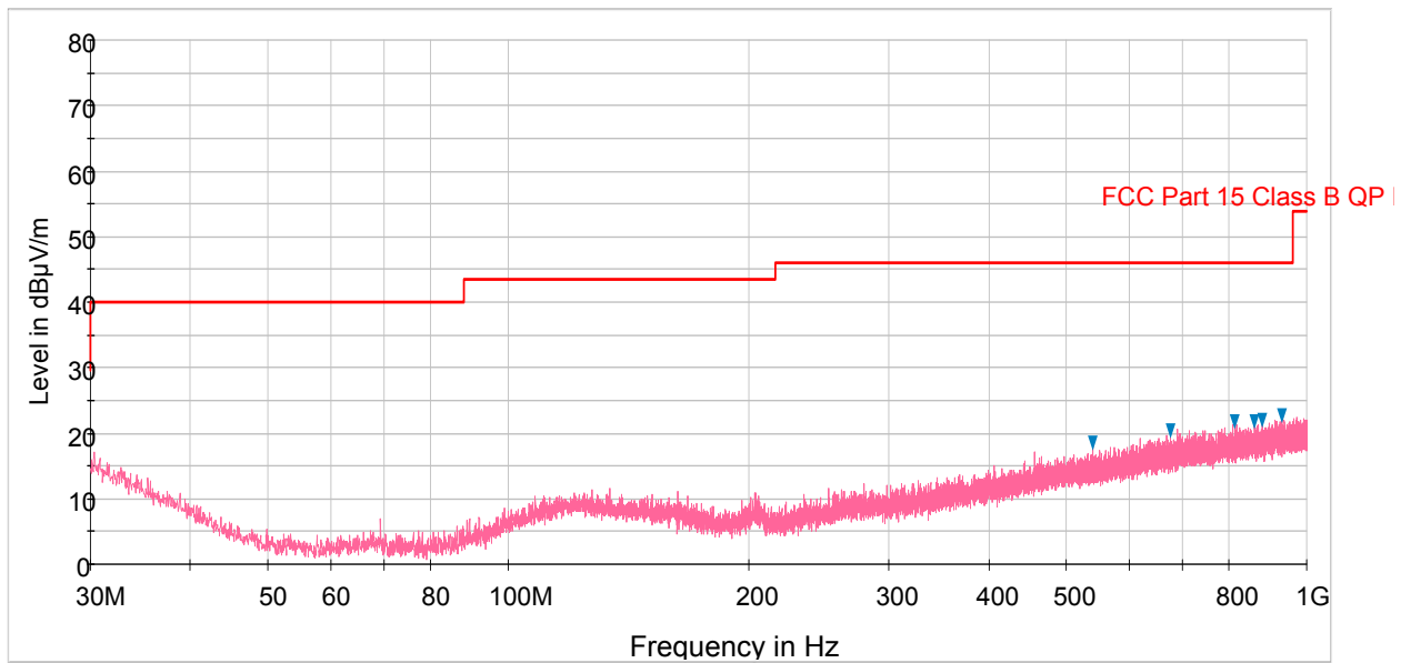
Plot 6-53. Radiated Spurious Plot below 1GHz (Pol. V)
