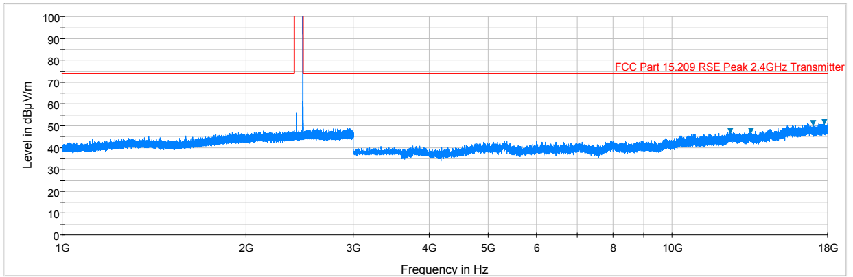
Plot 6-46. Radiated Spurious Plot above 1GHz (BT – Ch. 78, Ant. Pol. H)
