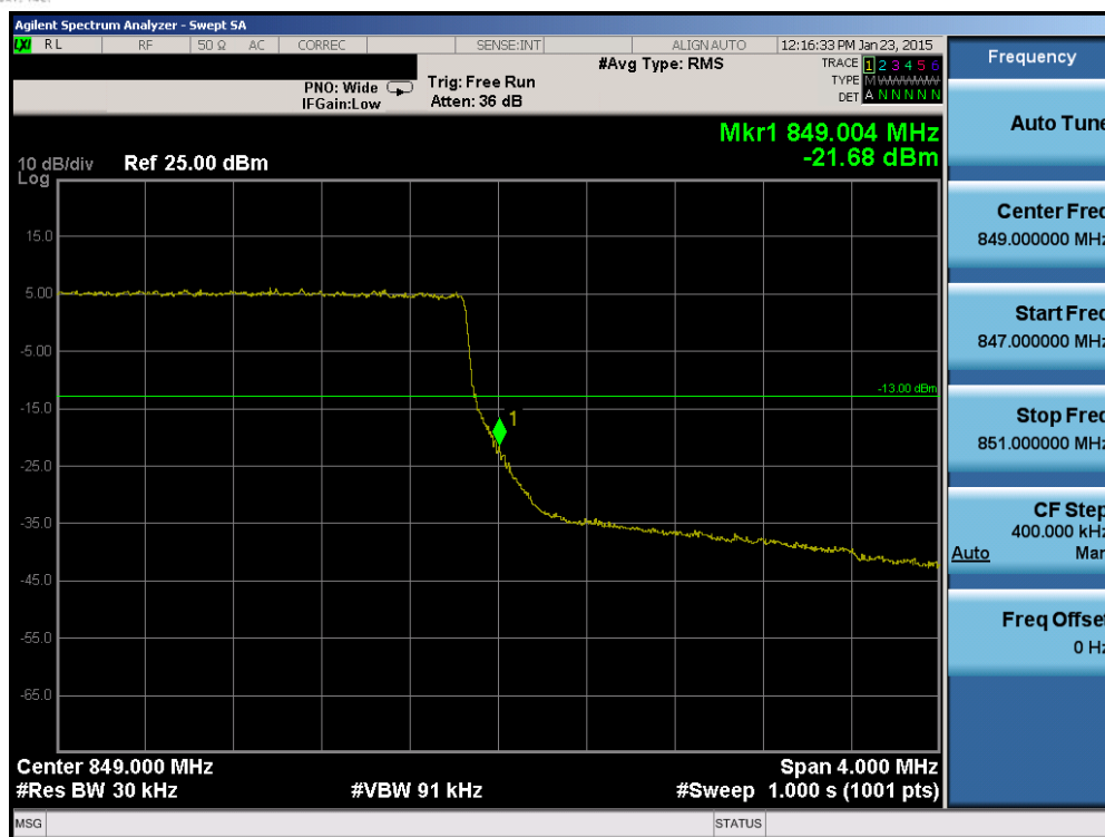
Plot 6-110. Upper Band Edge Plot (Band 5 – 3.0MHz QPSK – RB Size 15)
