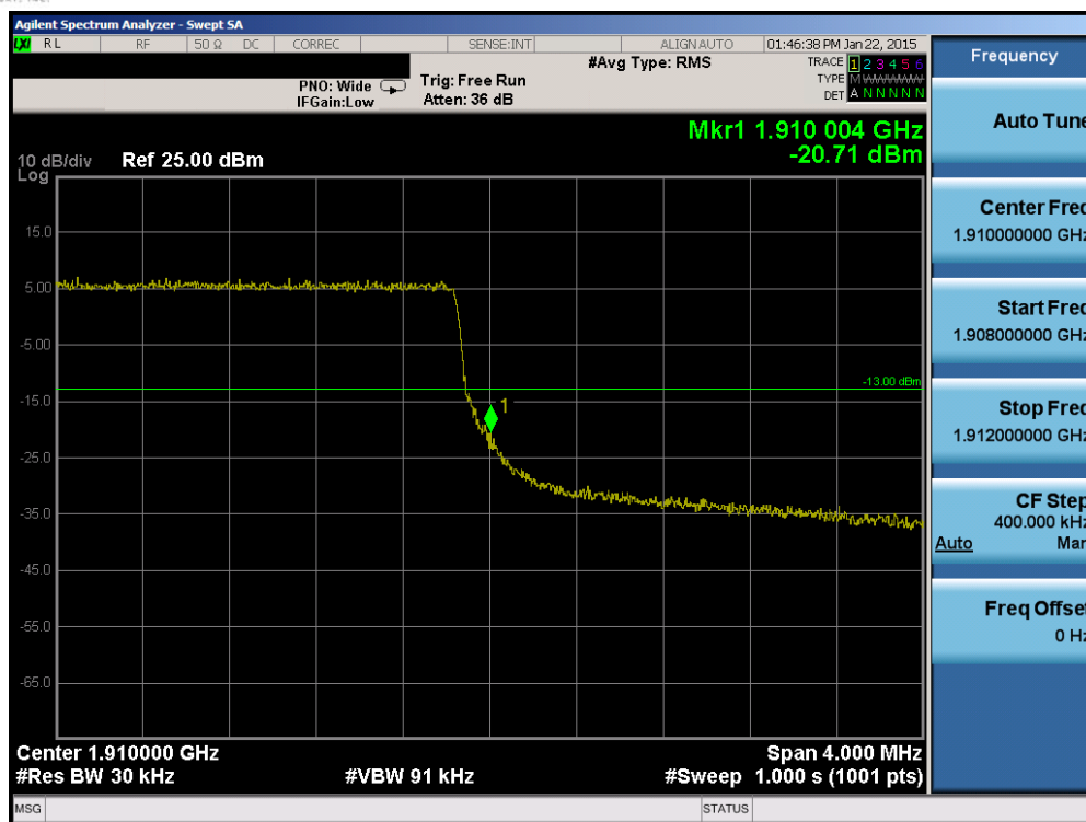
Plot 6-148. Upper Band Edge Plot (Band 2 – 3.0MHz QPSK – RB Size 15)
