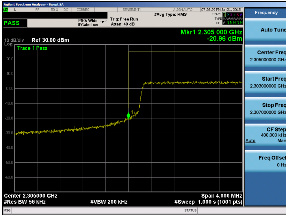
Plot 6-166. Lower Band Edge Plot (Band 30 – 5.0MHz QPSK – RB Size 25)
