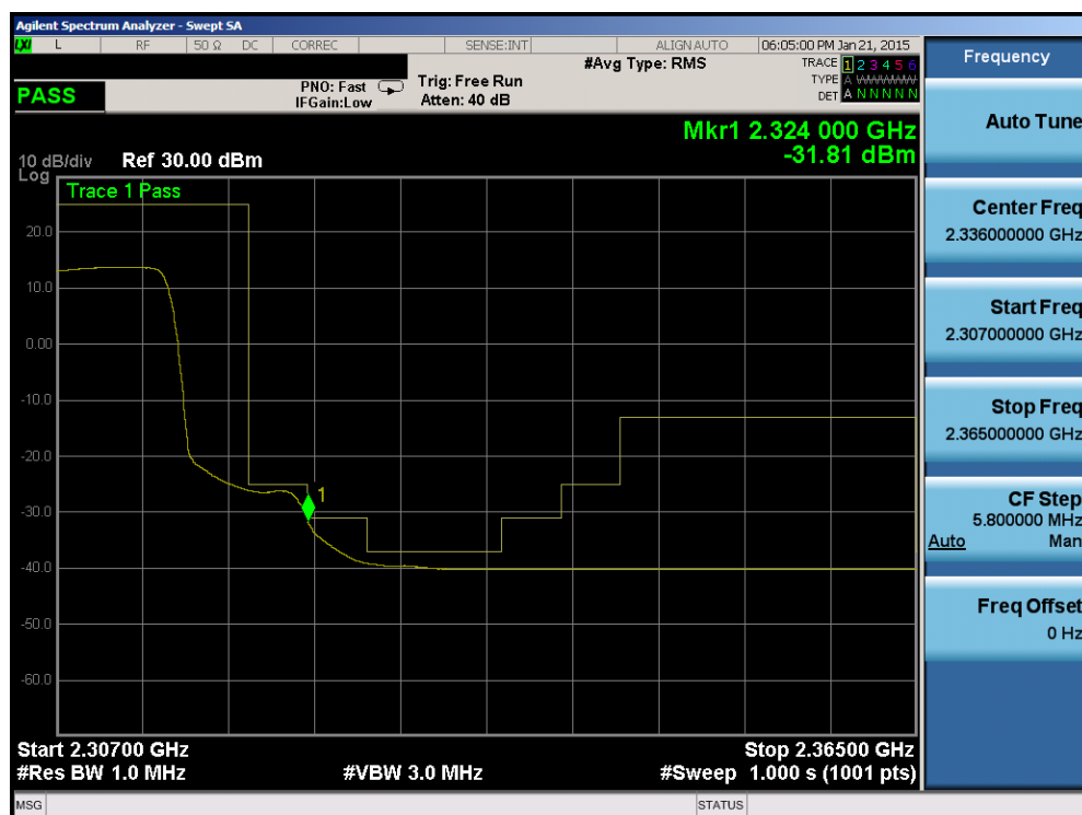
Plot 6-173. Upper Band Edge Plot (Band 30 – 10.0MHz QPSK – RB Size 50)
