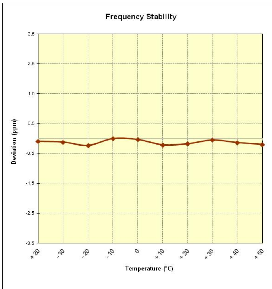
Figure 6-11. Frequency Stability Graph (Band 30)
