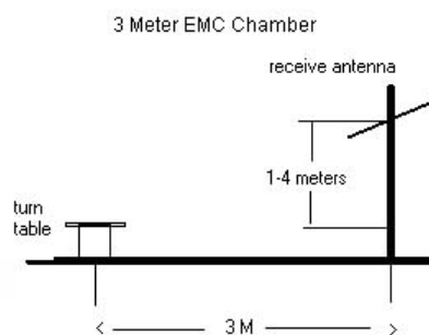
Figure 6-6. Test Instrument & Measurement Setup
