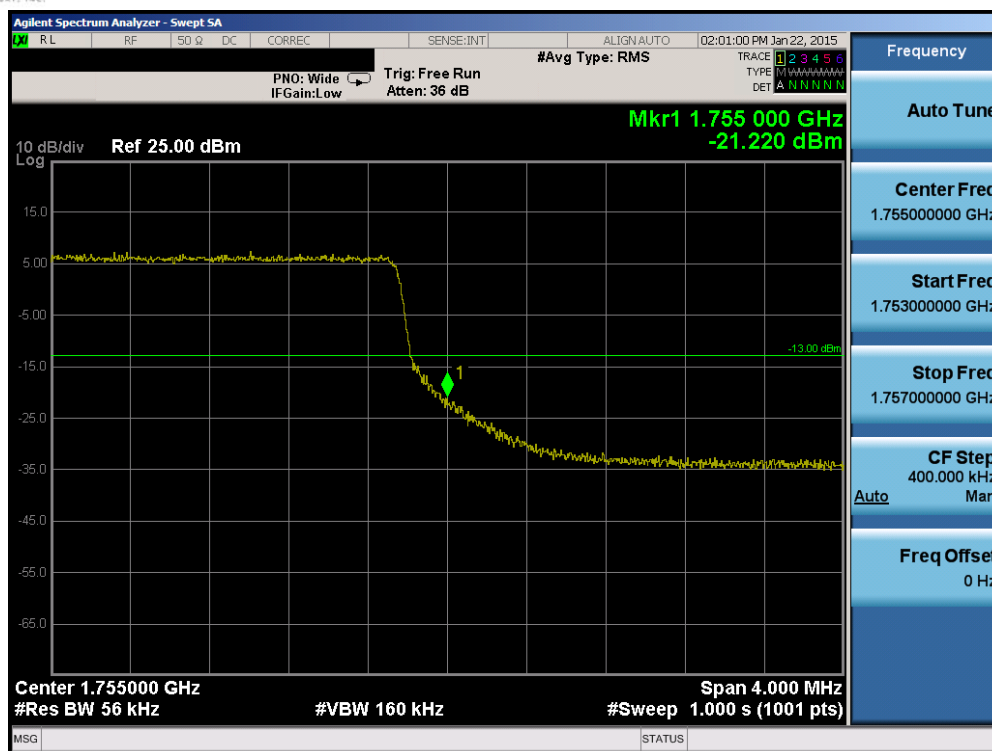
Plot 6-128. Upper Band Edge Plot (Band 4 – 5.0MHz QPSK – RB Size 25)
