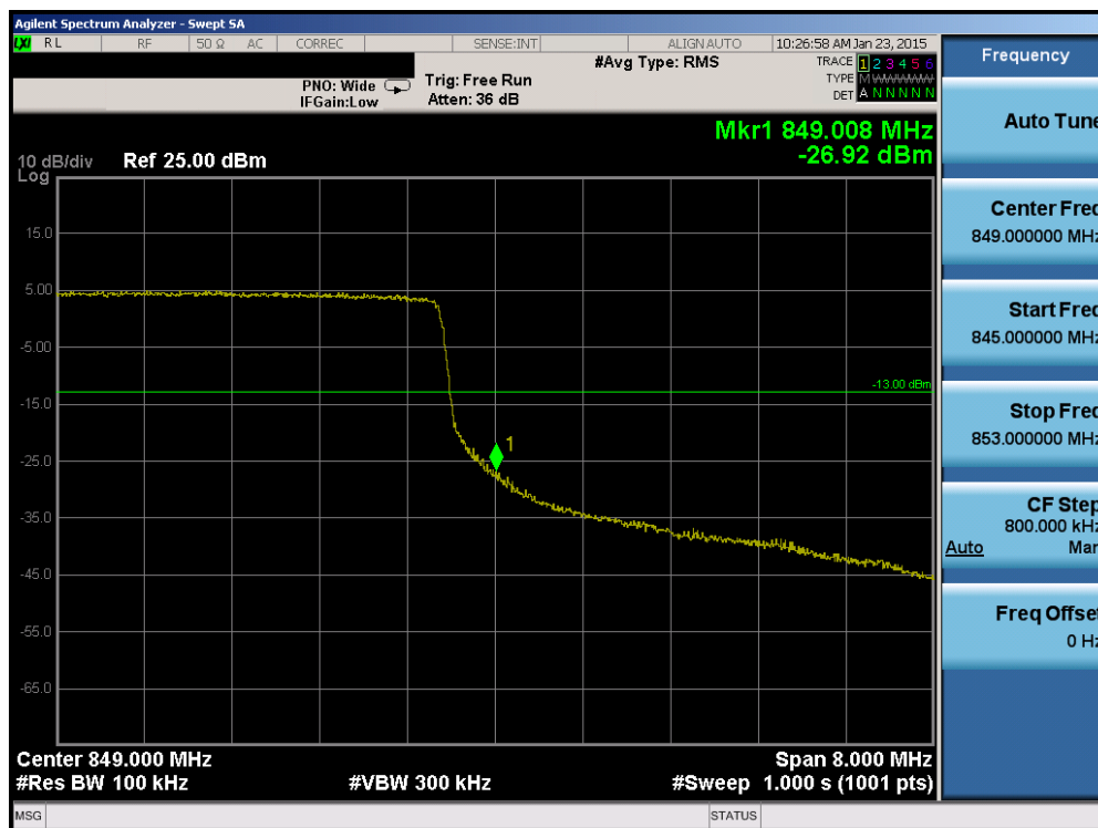
Plot 6-117. Upper Band Edge Plot (Band 5 – 10.0MHz QPSK – RB Size 50)
