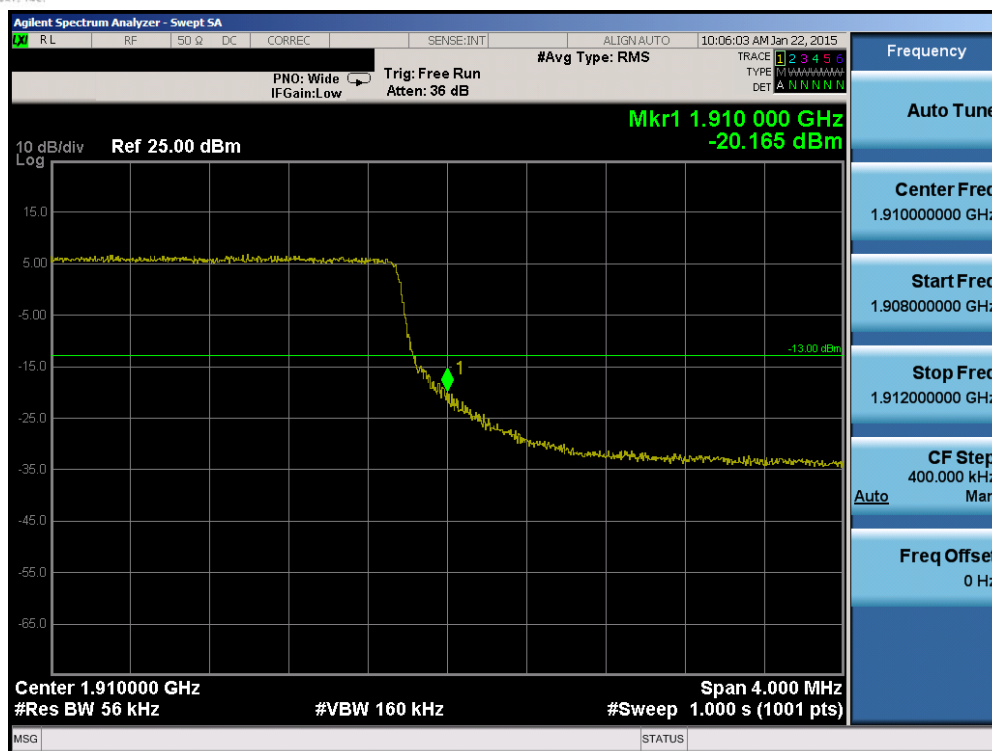
Plot 6-152. Upper Band Edge Plot (Band 2 – 5.0MHz QPSK – RB Size 25)
