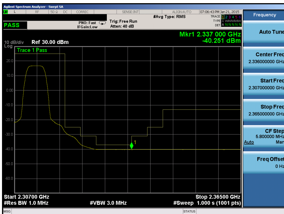
Plot 6-169. Upper Extended Band Edge Plot (Band 30 – 5.0MHz QPSK – RB Size 50)
