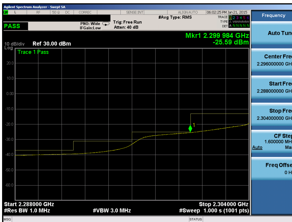
Plot 6-171. Lower Extended Band Edge Plot (Band 30 – 10.0MHz QPSK – RB Size 25)
