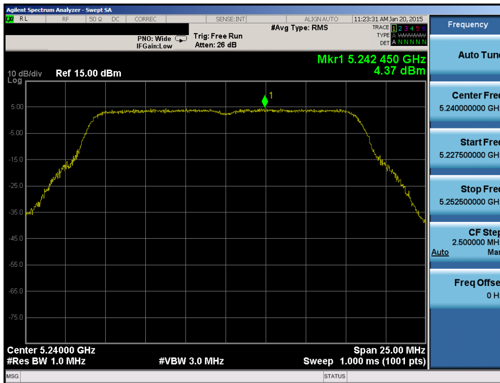
Plot 6-117. Power Spectral Density Plot (802.11a (UNII Band 1) – Ch. 48)
