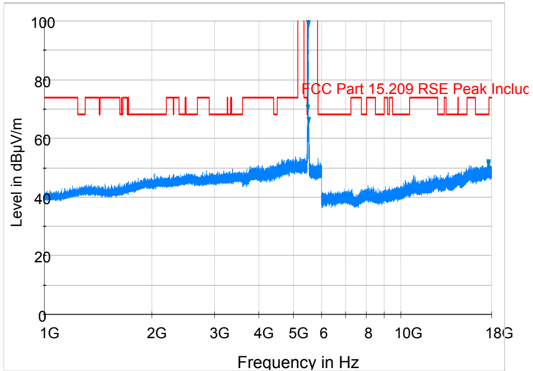
Plot 6-168. Radiated Spurious Plot above 1GHz (802.11a – U2C Ch. 116, Ant. Pol. V)
