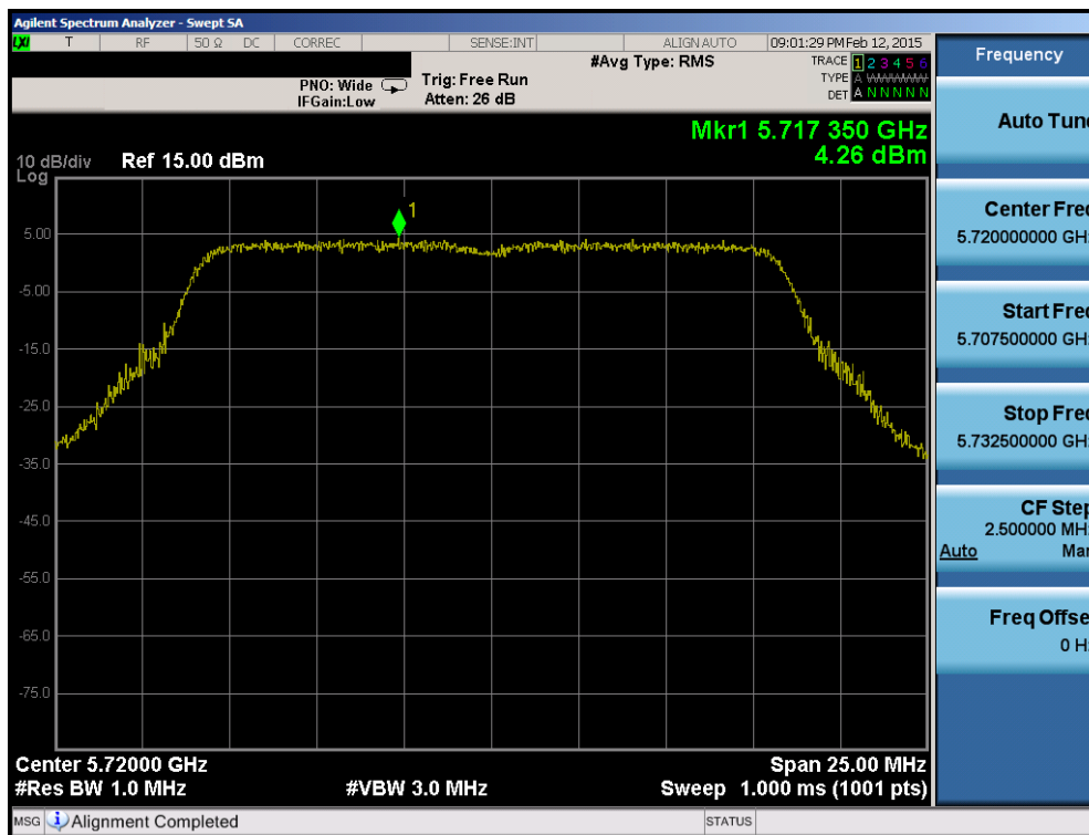
Plot 6-97. Power Spectral Density Plot (20MHz BW 802.11a (UNII Band 2C) – Ch. 144)
