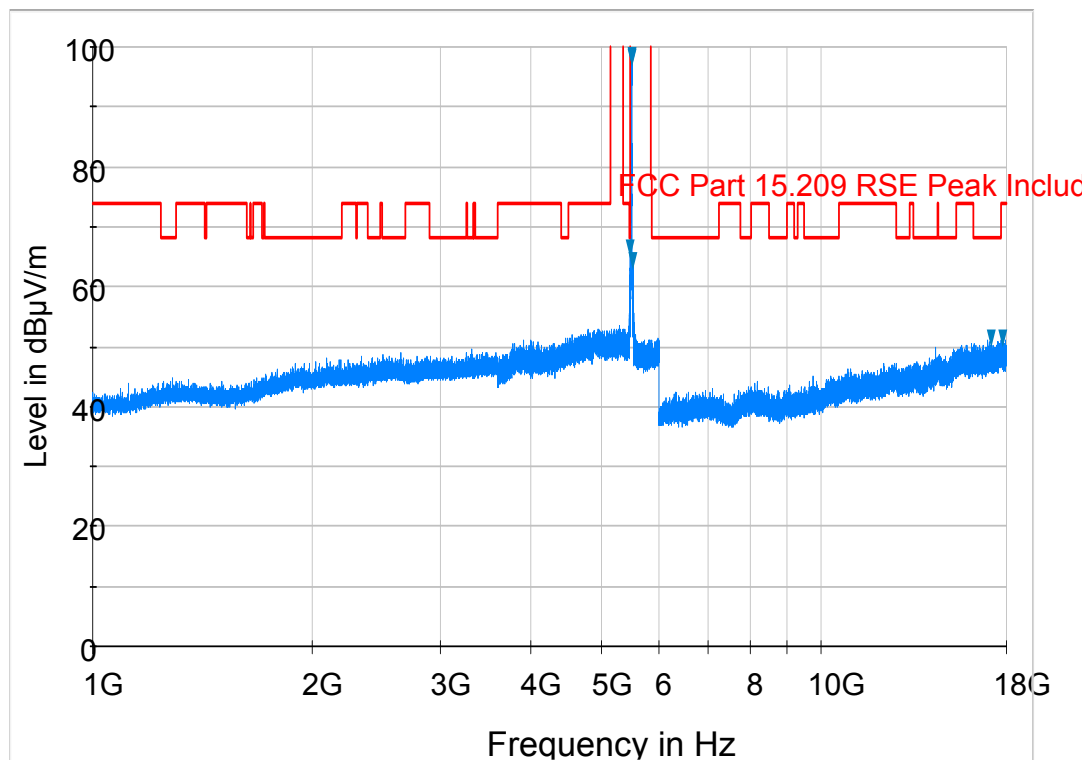
Plot 6-158. Radiated Spurious Plot above 1GHz (802.11a – U2C Ch. 116, Ant. Pol. V)
