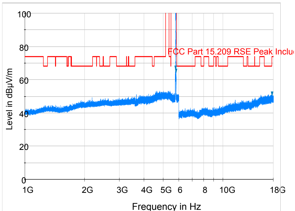
Plot 6-159. Radiated Spurious Plot above 1GHz (802.11a – U3 Ch. 157, Ant. Pol. H)
