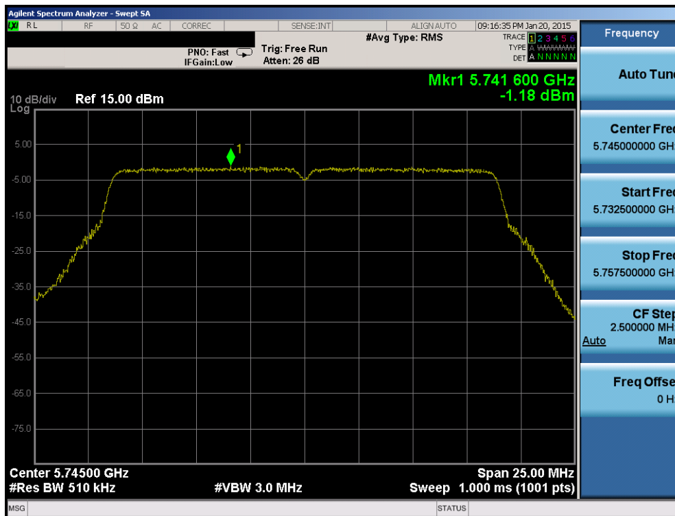
Plot 6-147. Power Spectral Density Plot (20MHz BW 802.11n (UNII Band 3) – Ch. 149)
