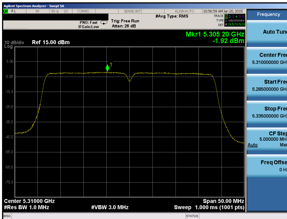
Plot 6-93. Power Spectral Density Plot (40MHz BW 802.11n (UNII Band 2A) – Ch. 62)
