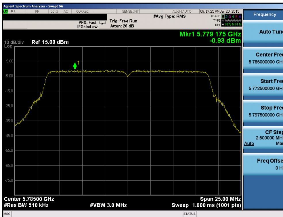
Plot 6-148. Power Spectral Density Plot (20MHz BW 802.11n (UNII Band 3) – Ch. 157)
