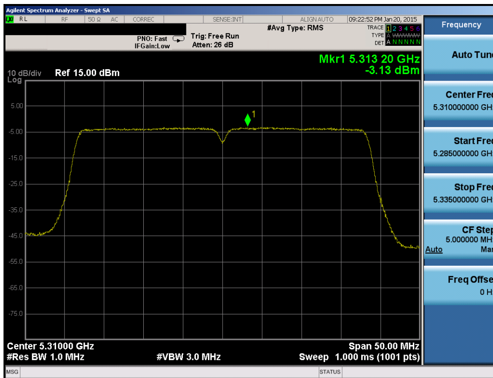
Plot 6-131. Power Spectral Density Plot (40MHz BW 802.11n (UNII Band 2A) – Ch. 62)
