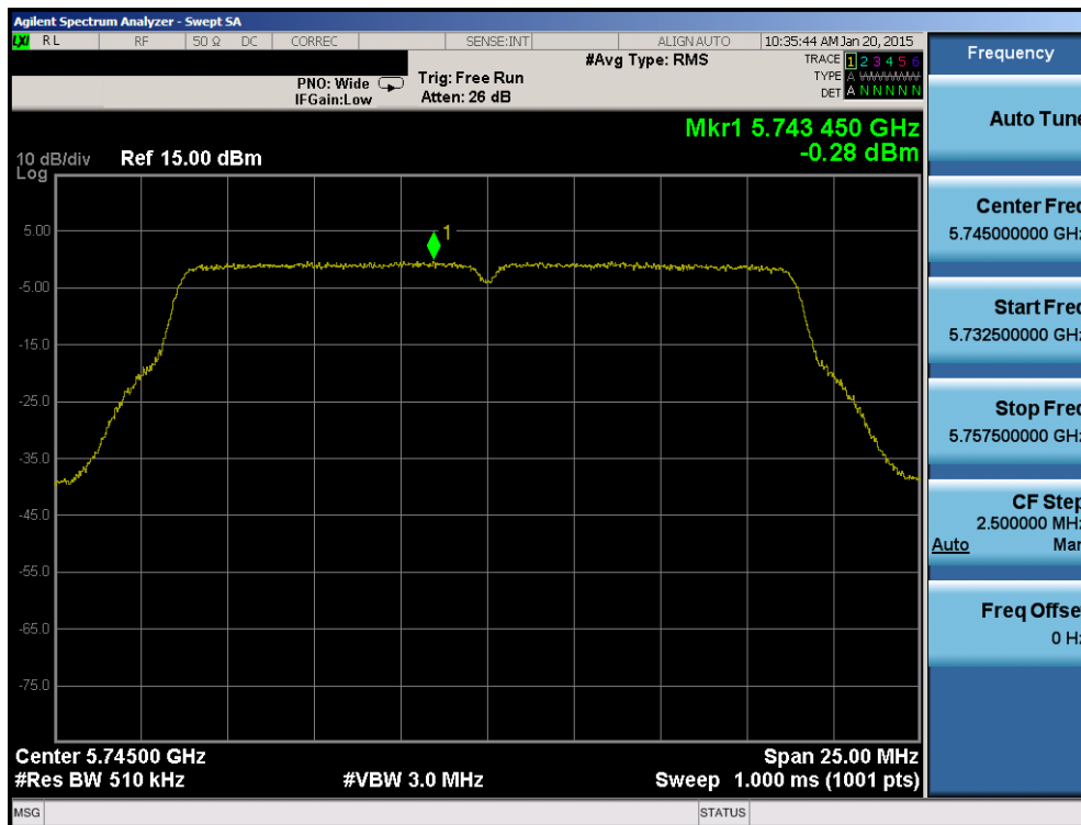
Plot 6-109. Power Spectral Density Plot (20MHz BW 802.11n (UNII Band 3) – Ch. 149)
