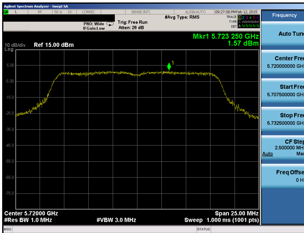
Plot 6-135. Power Spectral Density Plot (20MHz BW 802.11a UNII Band 2C) – Ch. 144)
