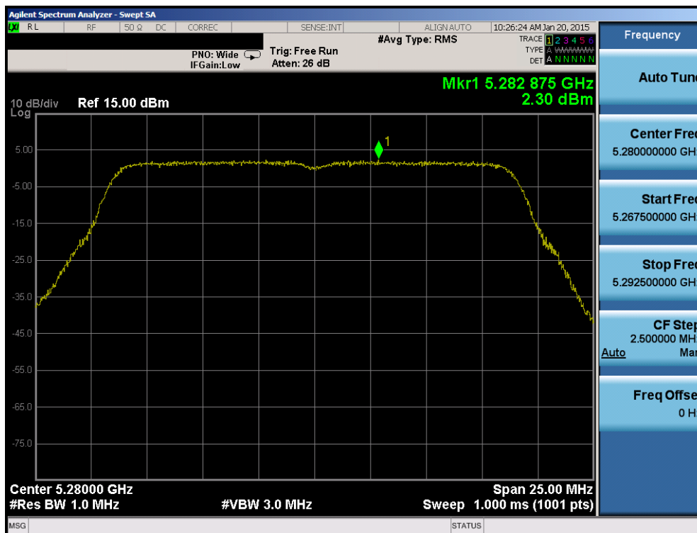
Plot 6-90. Power Spectral Density Plot (20MHz BW 802.11n (UNII Band 2A) – Ch. 56)
