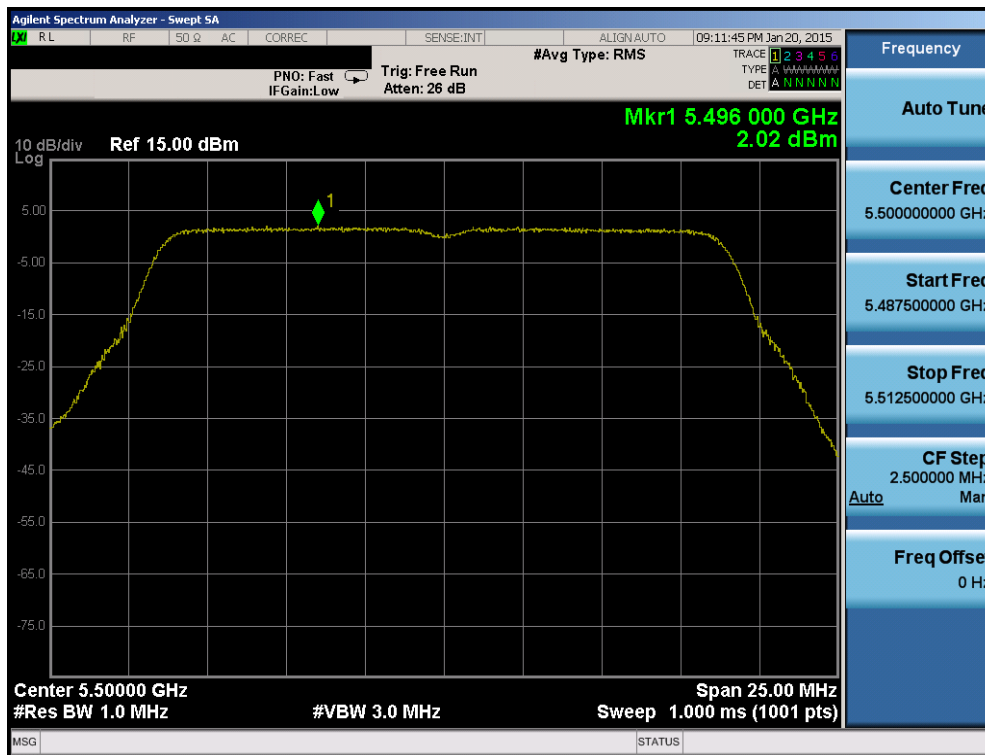
Plot 6-136. Power Spectral Density Plot (20MHz BW 802.11n (UNII Band 2C) – Ch. 100)
