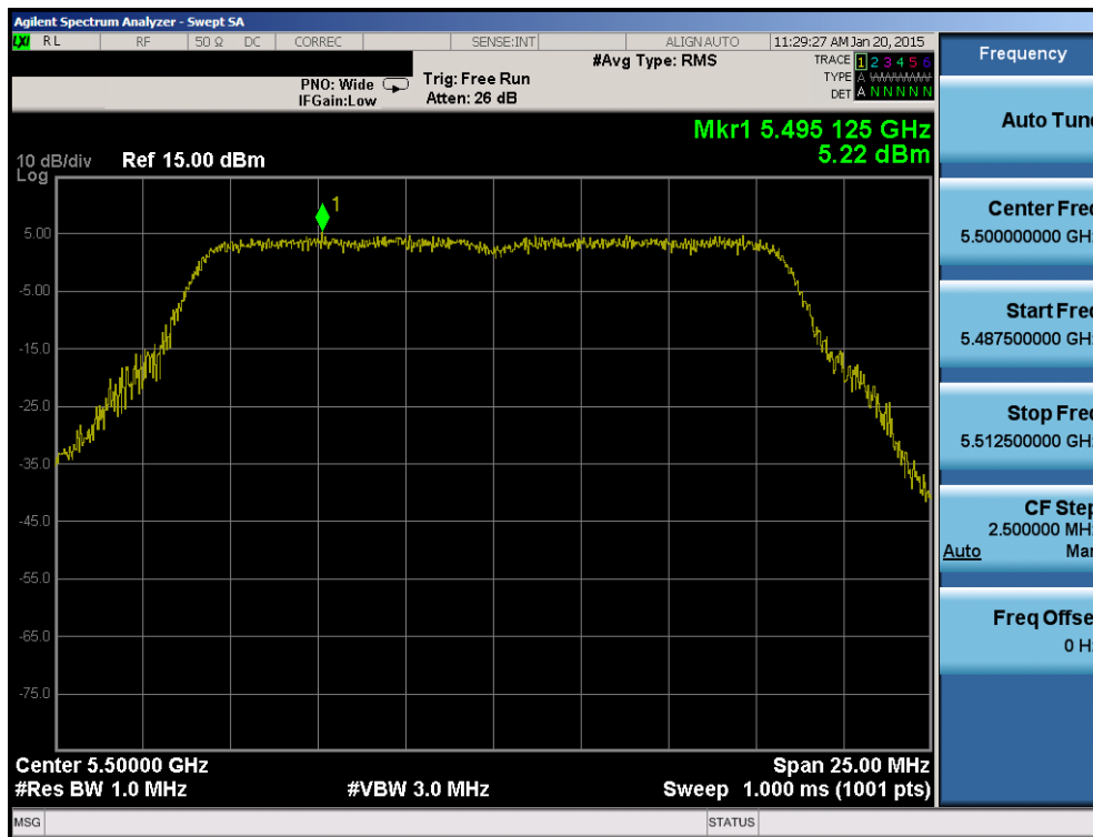
Plot 6-133. Power Spectral Density Plot (802.11a (UNII Band 2C) – Ch. 100)
