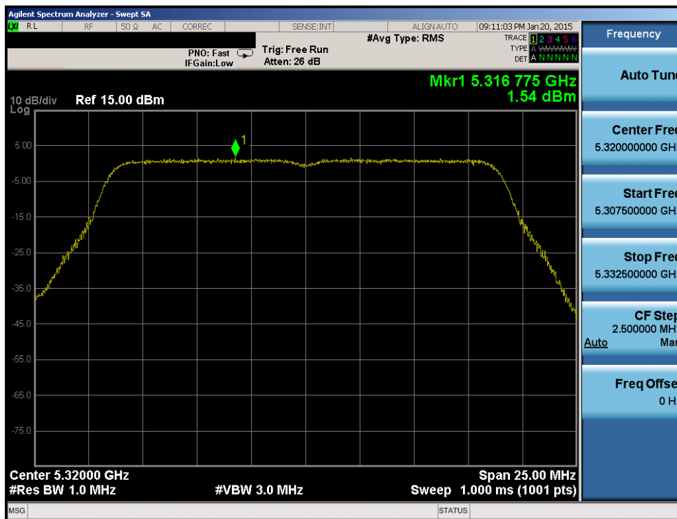
Plot 6-129. Power Spectral Density Plot (20MHz BW 802.11n (UNII Band 2A) – Ch. 64)
