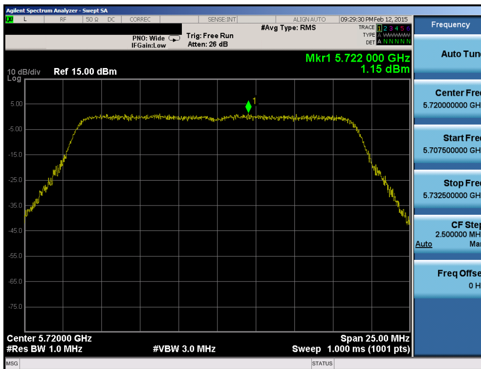
Plot 6-138. Power Spectral Density Plot (20MHz BW 802.11n (UNII Band 2C) – Ch. 144)
