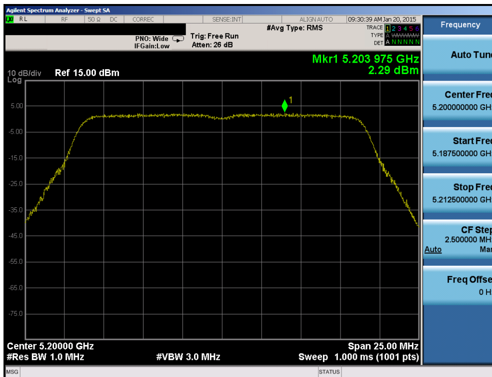
Plot 6-81. Power Spectral Density Plot (20MHz BW 802.11n (UNII Band 1) – Ch. 40)
