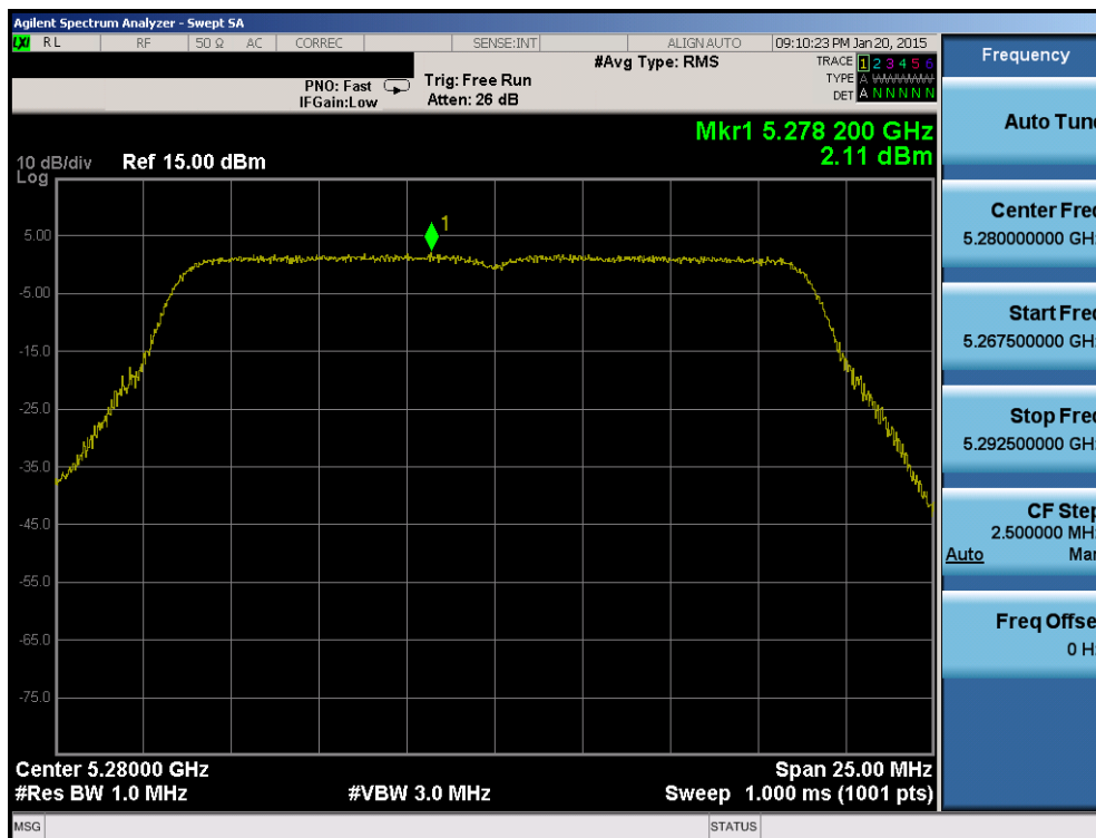
Plot 6-128. Power Spectral Density Plot (20MHz BW 802.11n (UNII Band 2A) – Ch. 56)
