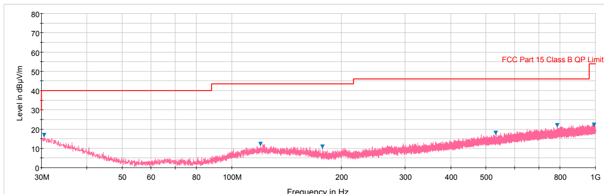
Plot 6-238. Radiated Spurious Plot below 1GHz (802.11a – U3 Ch. 157, Ant. Pol. H)
