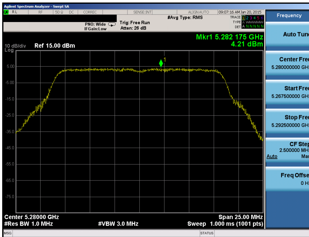
Plot 6-87. Power Spectral Density Plot (802.11a (UNII Band 2A) – Ch. 56)
