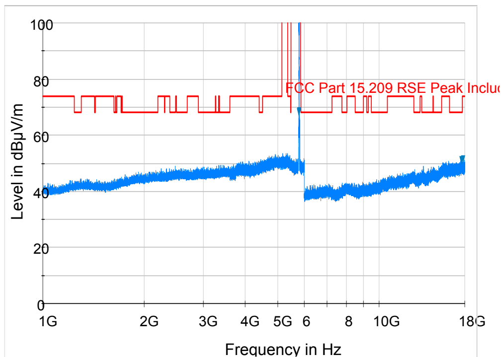
Plot 6-169. Radiated Spurious Plot above 1GHz (802.11a – U3 Ch. 157, Ant. Pol. H)
