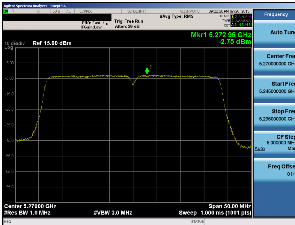
Plot 6-130. Power Spectral Density Plot (40MHz BW 802.11n (UNII Band 2A) – Ch. 54)
