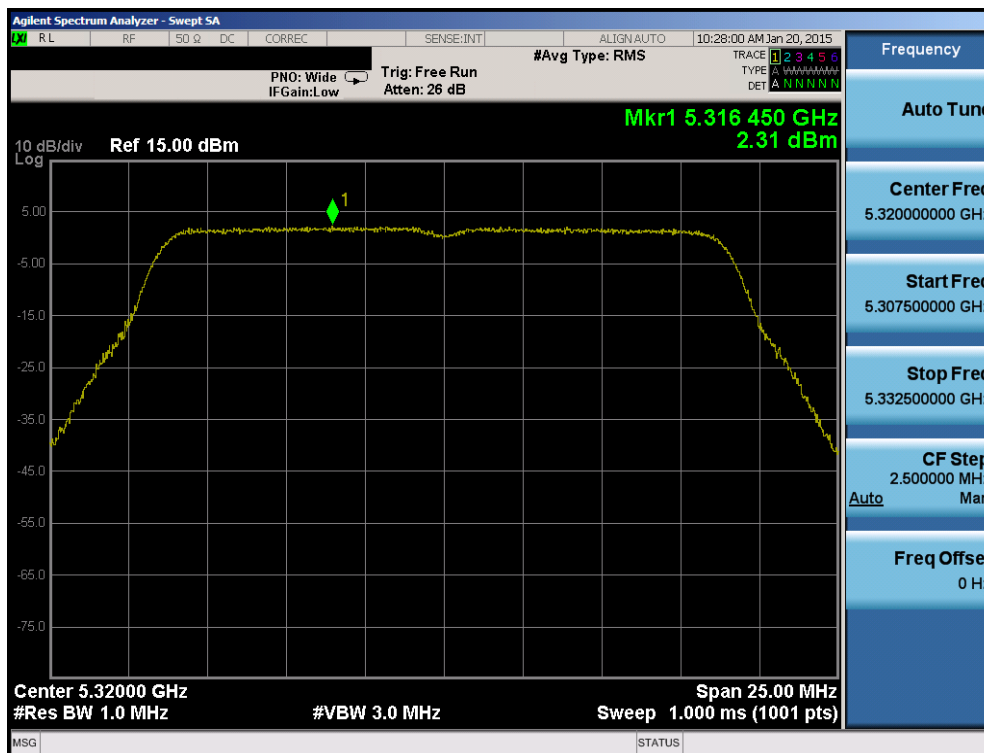
Plot 6-91. Power Spectral Density Plot (20MHz BW 802.11n (UNII Band 2A) – Ch. 64)
