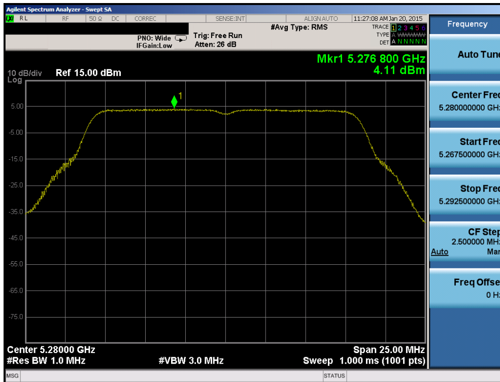
Plot 6-125. Power Spectral Density Plot (802.11a (UNII Band 2A) – Ch. 56)
