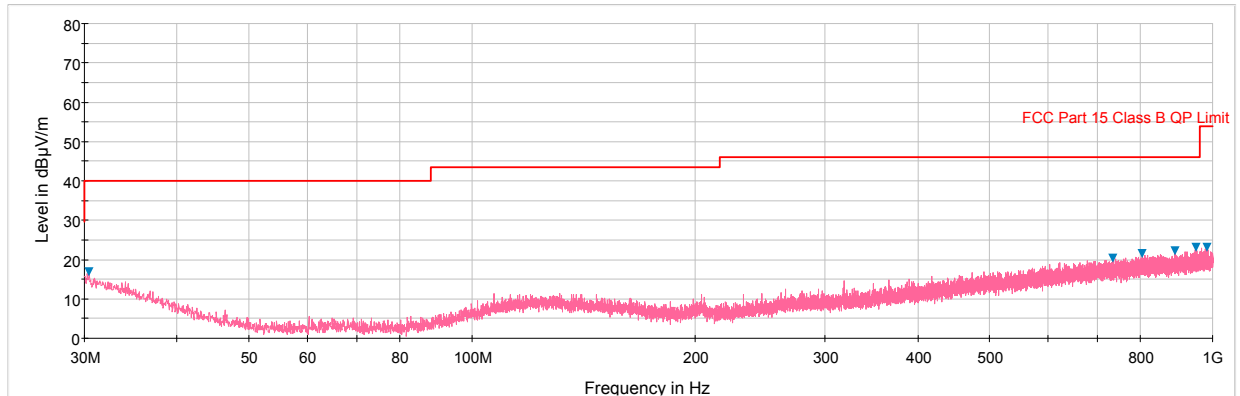
Plot 6-236. Radiated Spurious Plot below 1GHz (802.11a – U3 Ch. 157, Ant. Pol. H)
