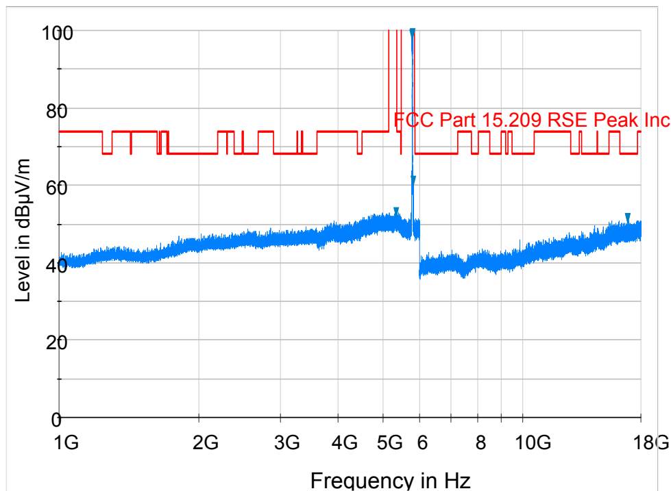
Plot 6-170. Radiated Spurious Plot above 1GHz (802.11a – U3 Ch. 157, Ant. Pol. V)
