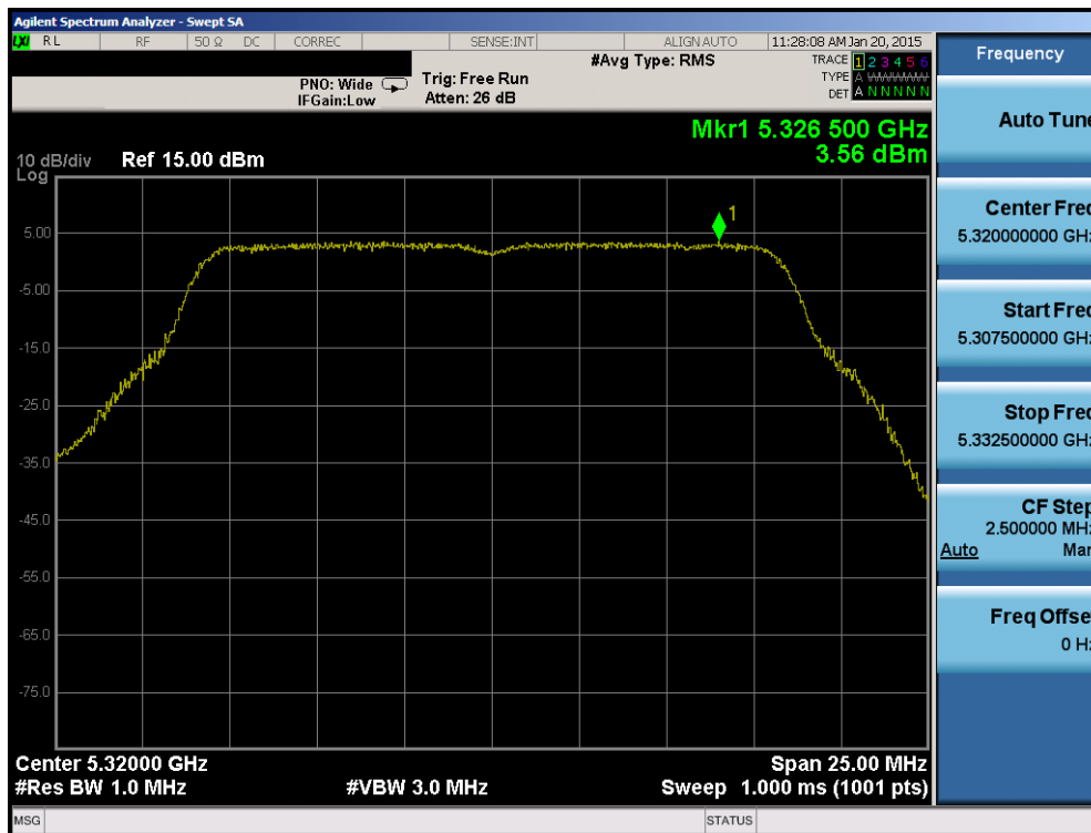
Plot 6-126. Power Spectral Density Plot (802.11a (UNII Band 2A) – Ch. 64)
