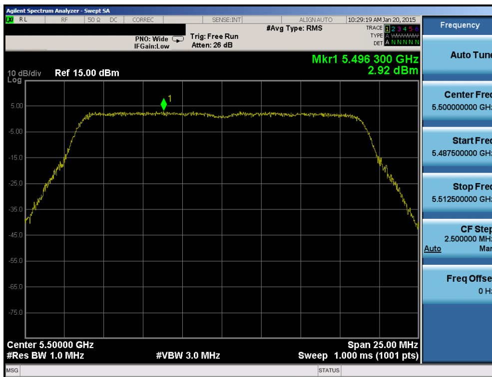
Plot 6-98. Power Spectral Density Plot (20MHz BW 802.11n (UNII Band 2C) – Ch. 100)
