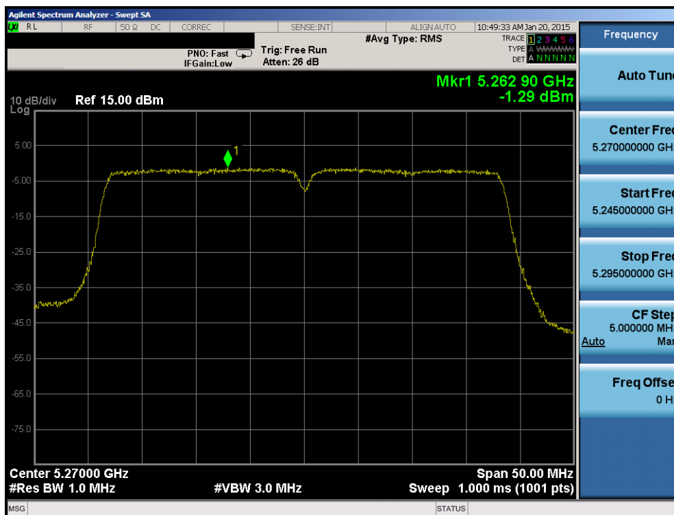
Plot 6-92. Power Spectral Density Plot (40MHz BW 802.11n (UNII Band 2A) – Ch. 54)
