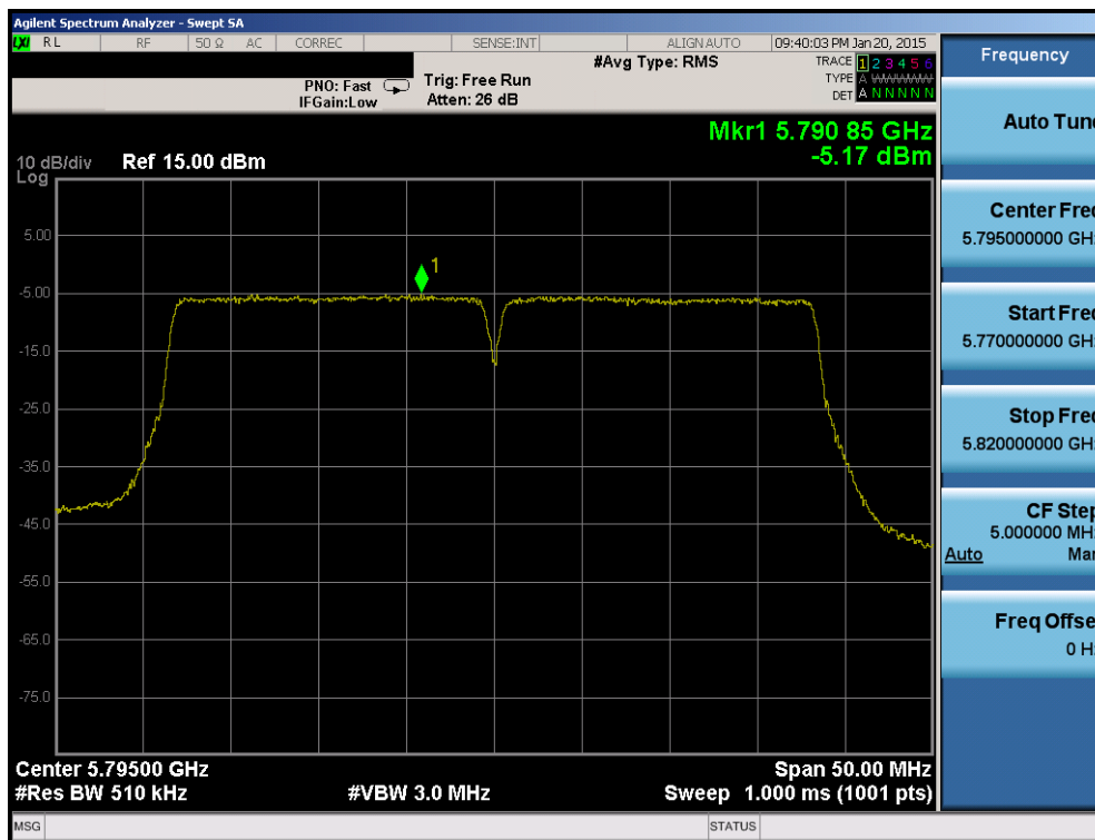
Plot 6-151. Power Spectral Density Plot (40MHz BW 802.11n (UNII Band 3) – Ch. 159)
