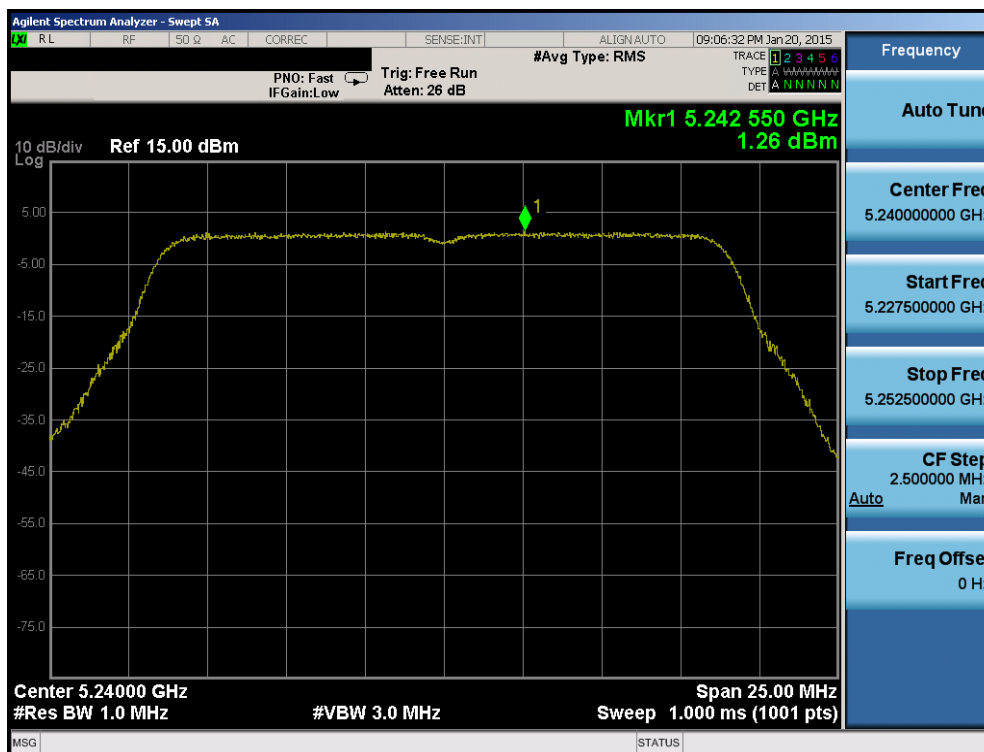
Plot 6-120. Power Spectral Density Plot (20MHz BW 802.11n (UNII Band 1) – Ch. 48)
