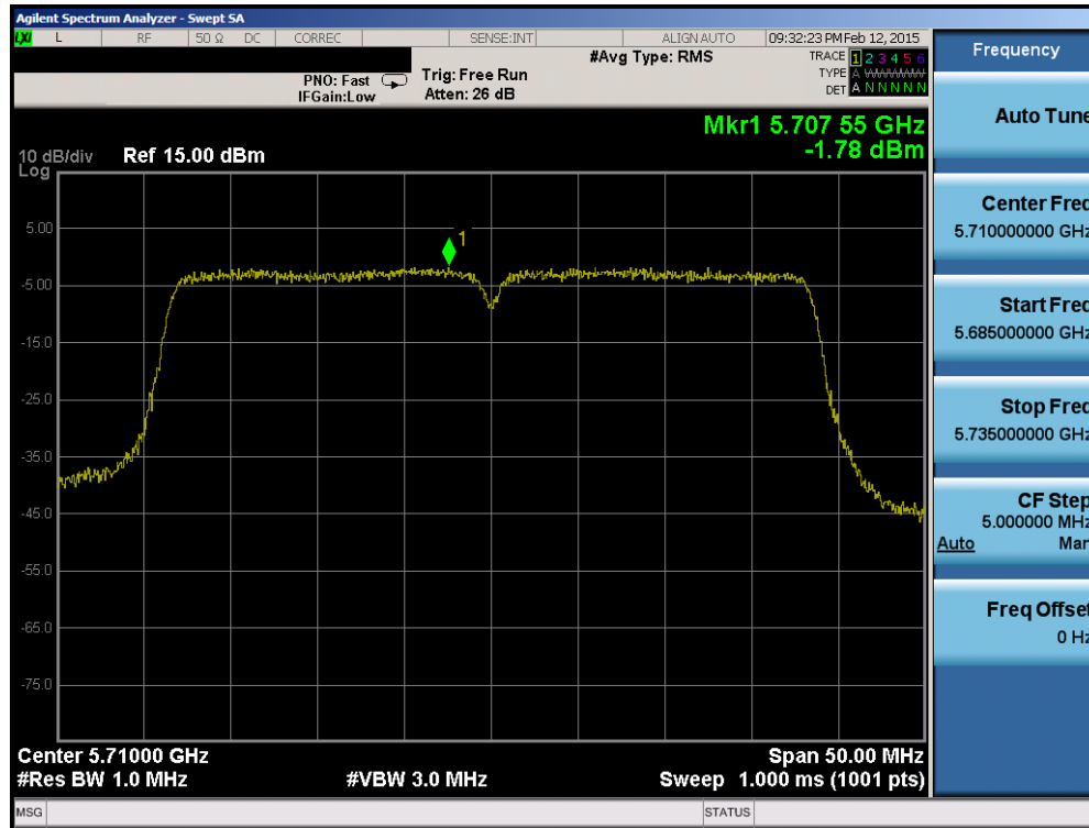
Plot 6-141. Power Spectral Density Plot (40MHz BW 802.11n (UNII Band 2C) – Ch. 142)
