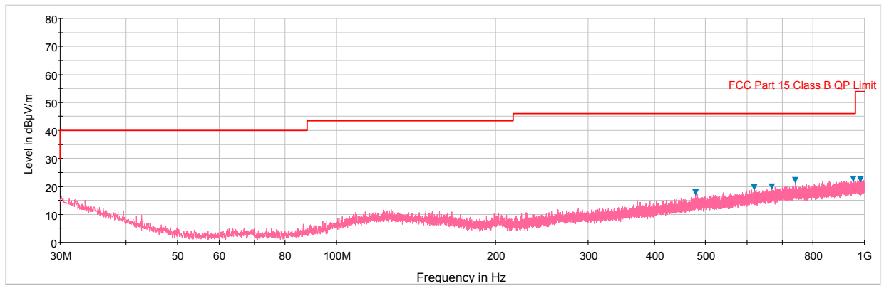
Plot 6-237. Radiated Spurious Plot below 1GHz (802.11a – U3 Ch. 157, Ant. Pol. V)
