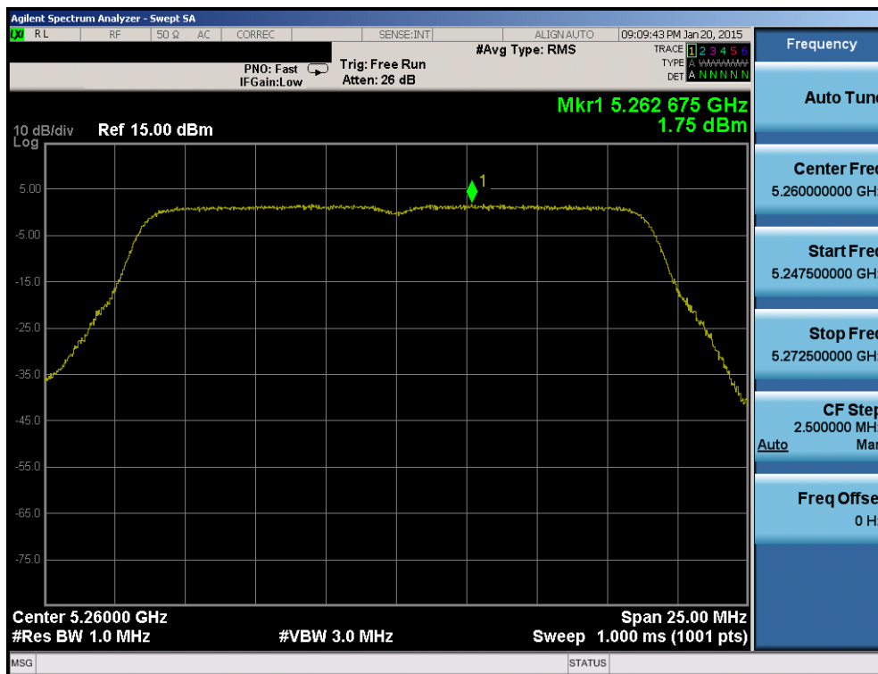
Plot 6-127. Power Spectral Density Plot (20MHz BW 802.11n (UNII Band 2A) – Ch. 52)
