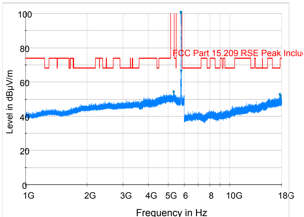
Plot 6-160. Radiated Spurious Plot above 1GHz (802.11a – U3 Ch. 157, Ant. Pol. V)
