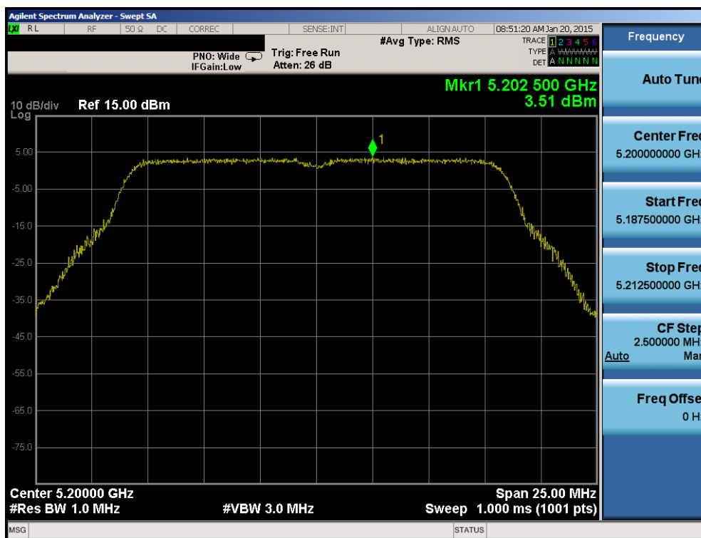
Plot 6-78. Power Spectral Density Plot (802.11a (UNII Band 1) – Ch. 40)
