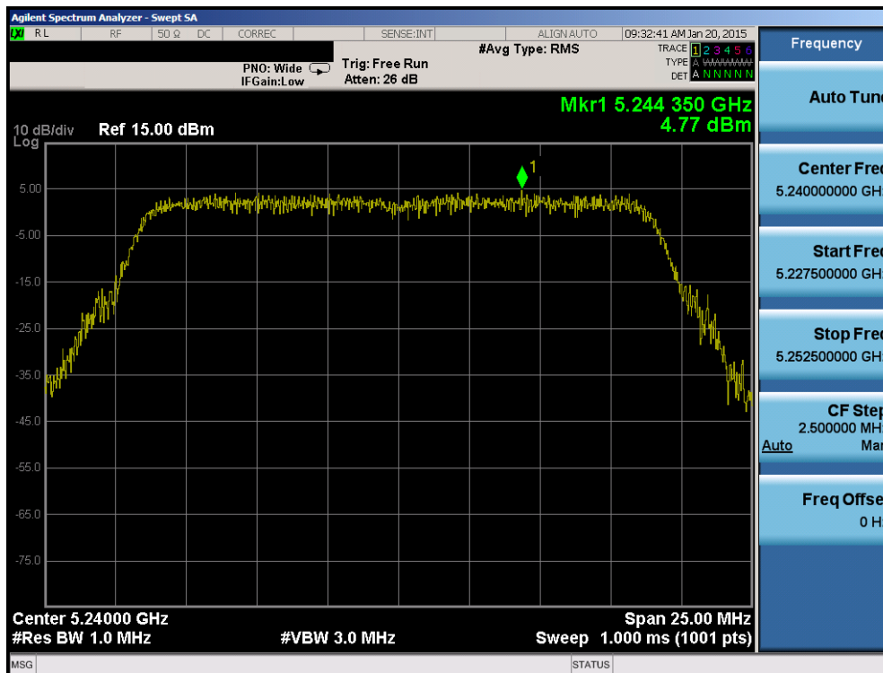
Plot 6-82. Power Spectral Density Plot (20MHz BW 802.11n (UNII Band 1) – Ch. 48)
