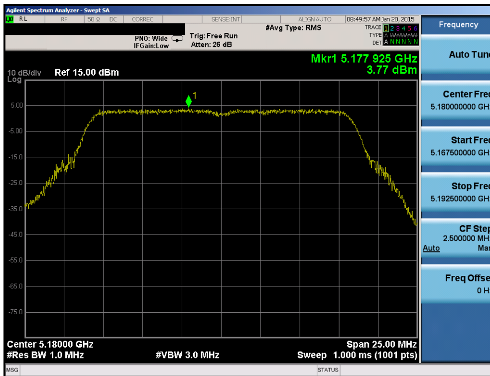
Plot 6-77. Power Spectral Density Plot (802.11a (UNII Band 1) – Ch. 36)
