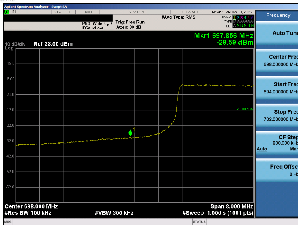
Plot 6-75. Lower Band Edge Plot (Band 12 – 10.0MHz QPSK – RB Size 50)
