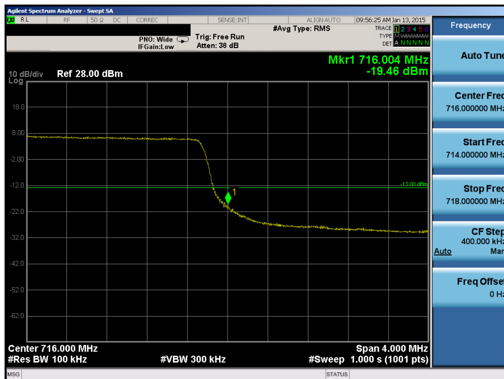
Plot 6-74. Upper Band Edge Plot (Band 12 – 5.0MHz QPSK – RB Size 25)
