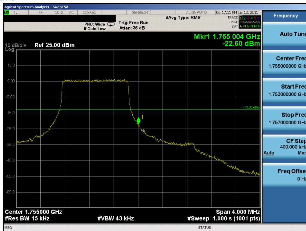
Plot 6-95. Upper Band Edge Plot (Band 4 – 1.4MHz QPSK – RB Size 6)
