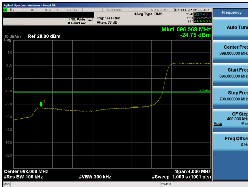
Plot 6-70. Lower Band Edge Plot (Band 12 – 3.0MHz QPSK – RB Size 15)
