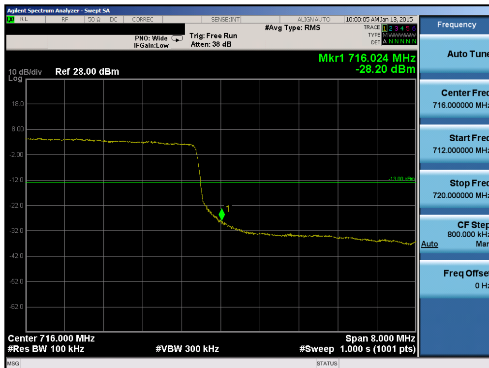
Plot 6-76. Upper Band Edge Plot (Band 12 – 10.0MHz QPSK – RB Size 50)
