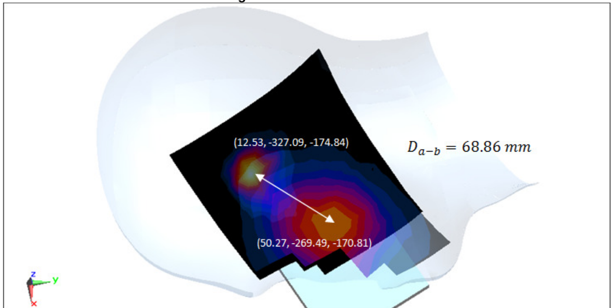
Figure 12-1 Peak SAR Locations for Right Cheek 5GHz WLAN MIMO and GSM 850 MHz
