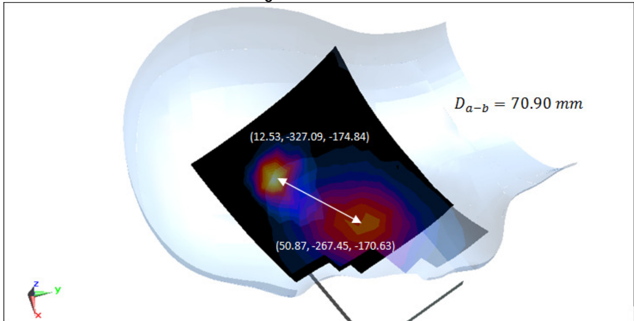
Figure 12-2 Peak SAR Locations for Right Cheek 5GHz WLAN MIMO and LTE B26
