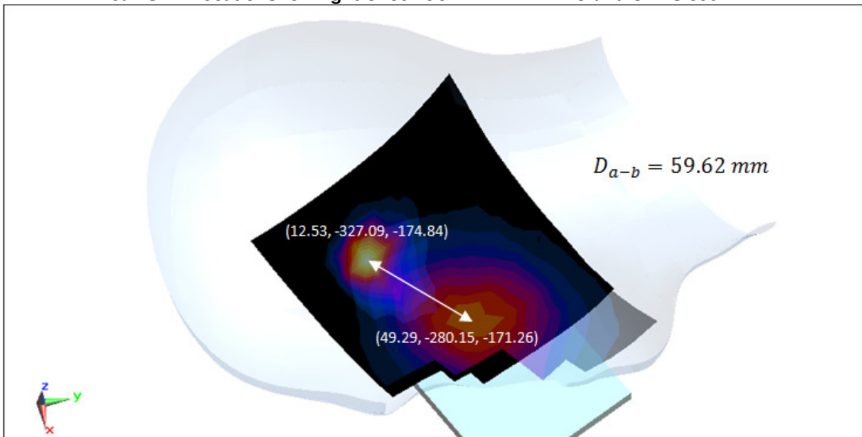
Figure 12-2 Peak SAR Locations for Right Cheek 5GHz WLAN MIMO and UMTS 850 MHz
