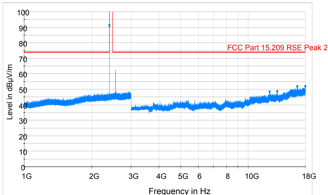
Plot 6-18. Radiated Spurious Plot above 1GHz (BTLE – Ch. 0, Ant. Pol. H)
