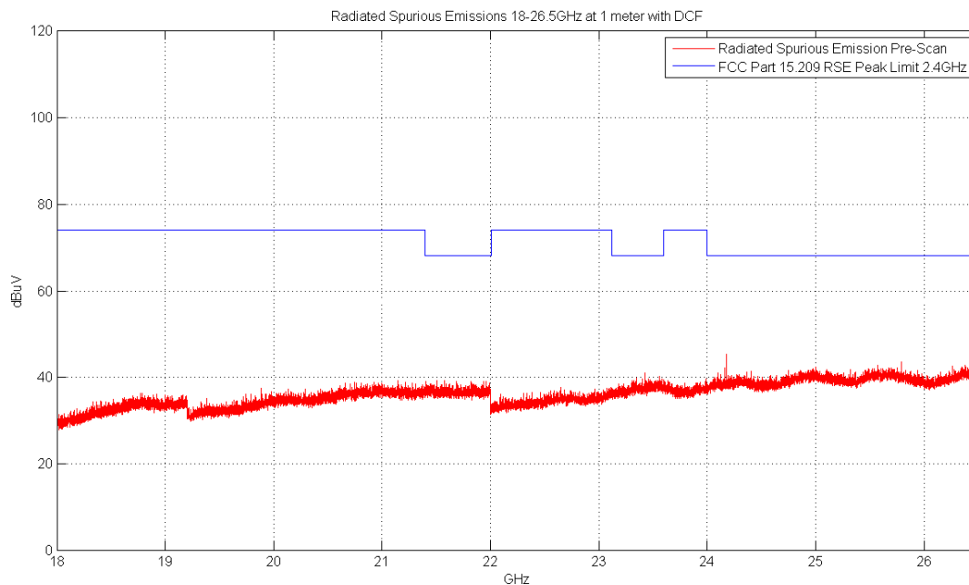
Plot 6-25. Radiated Spurious Plot above 18GHz (Pol. V)
