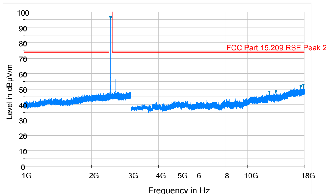
Plot 6-20. Radiated Spurious Plot above 1GHz (BTLE – Ch. 19, Ant. Pol. H)
