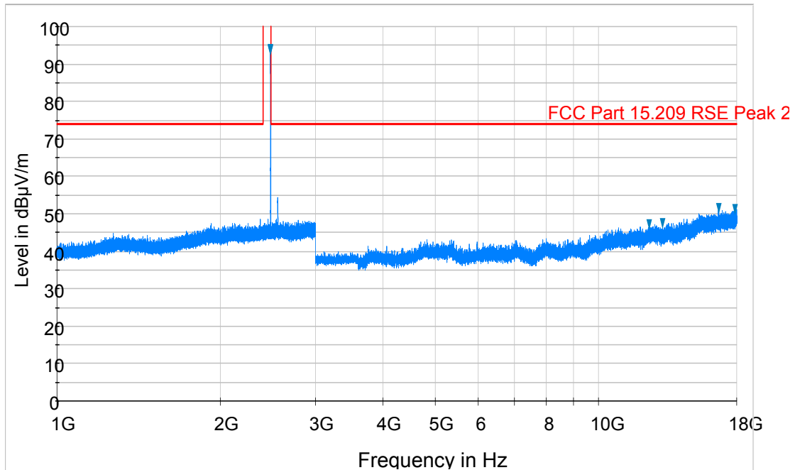
Plot 6-23. Radiated Spurious Plot above 1GHz (BTLE – Ch. 39, Ant. Pol. V)
