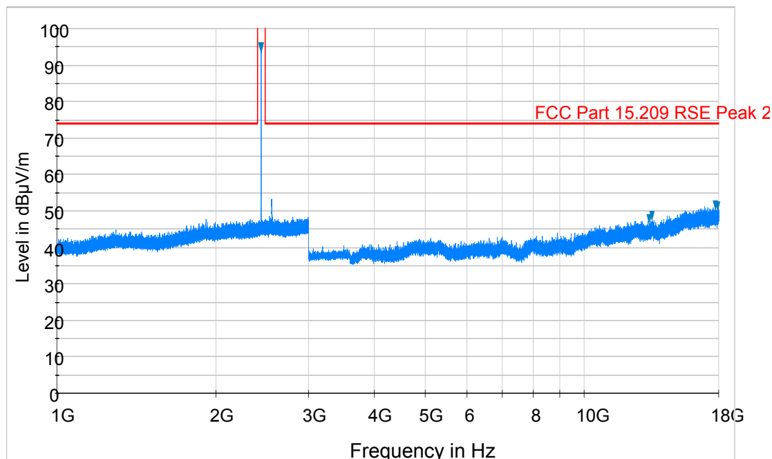
Plot 6-21. Radiated Spurious Plot above 1GHz (BTLE – Ch. 19, Ant. Pol. V)
