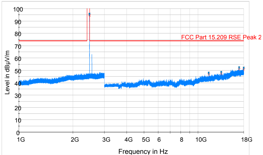
Plot 6-22. Radiated Spurious Plot above 1GHz (BTLE – Ch. 39, Ant. Pol. H)
