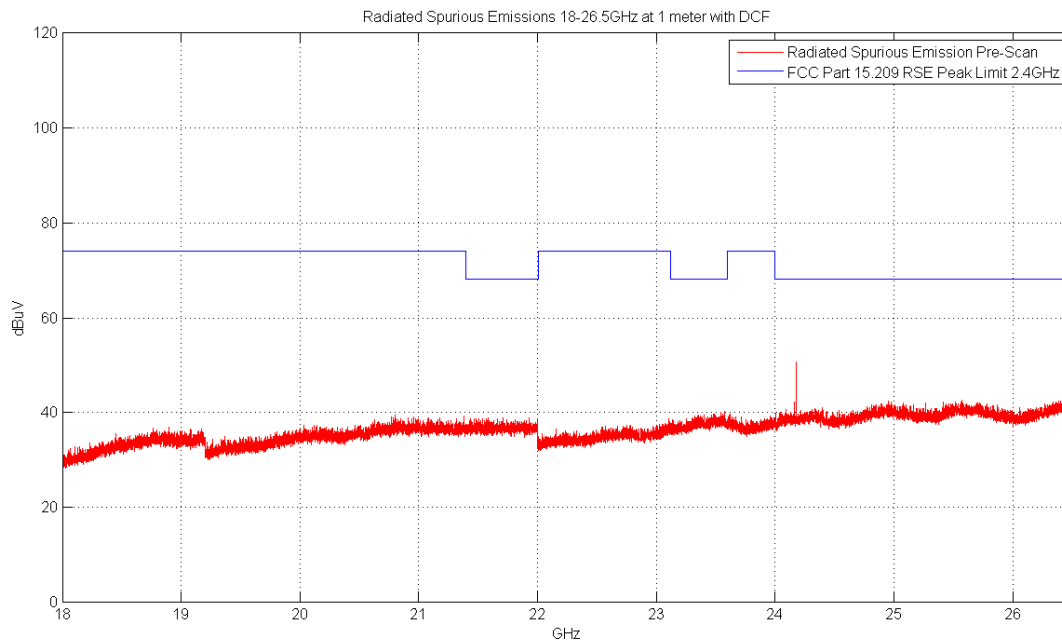
Plot 6-24. Radiated Spurious Plot above 18GHz (Pol. H)
