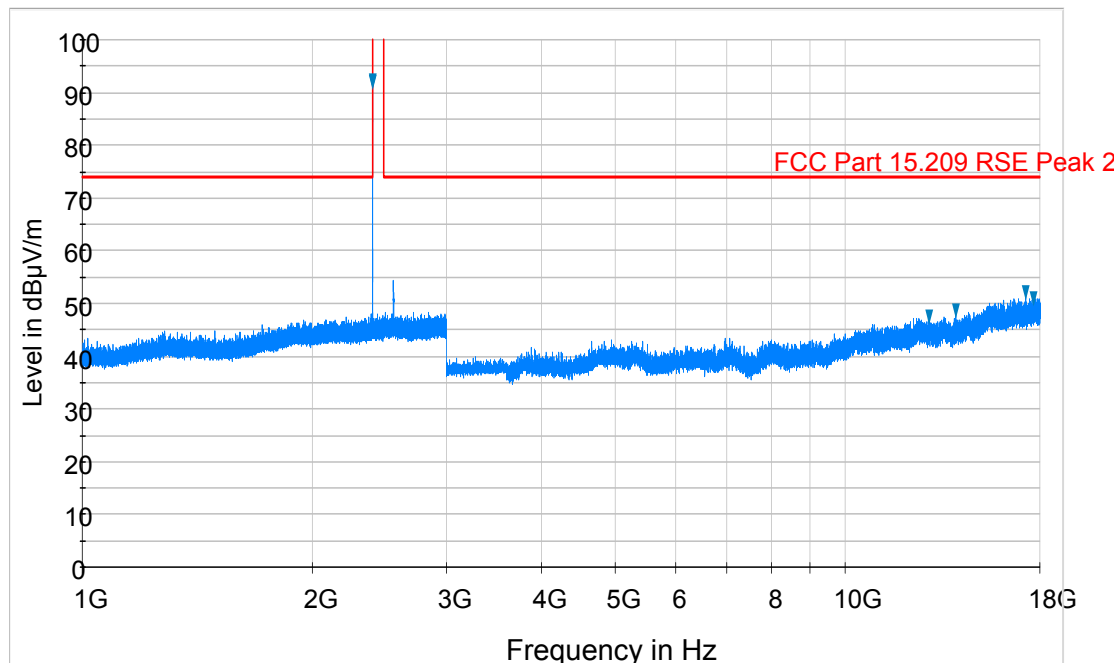
Plot 6-19. Radiated Spurious Plot above 1GHz (BTLE – Ch. 0, Ant. Pol. V)
