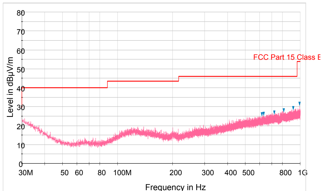
Plot 6-29. Radiated Spurious Plot below 1GHz (Pol. V)
