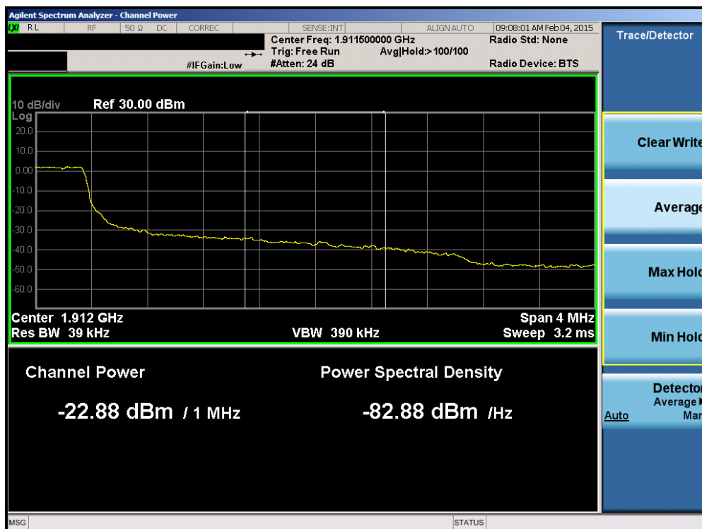
Plot 6-130. Upper Extended Band Edge Plot (Band 2 – 3.0MHz QPSK – RB Size 15)
