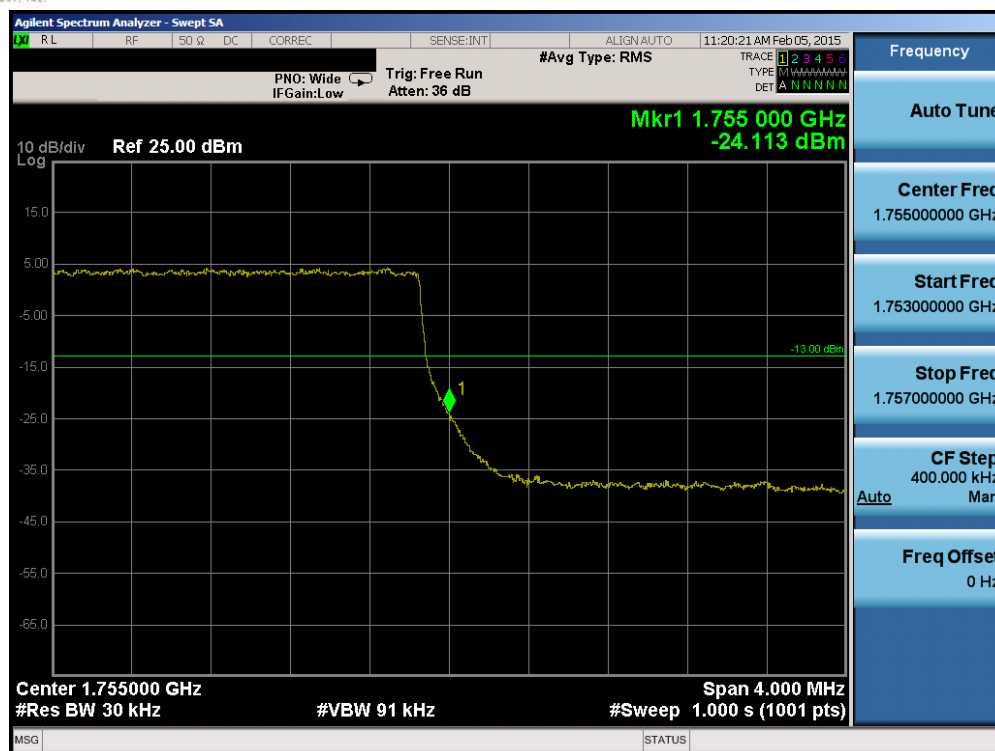
Plot 6-105. Upper Band Edge Plot (Band 4 – 3.0MHz QPSK – RB Size 15)
