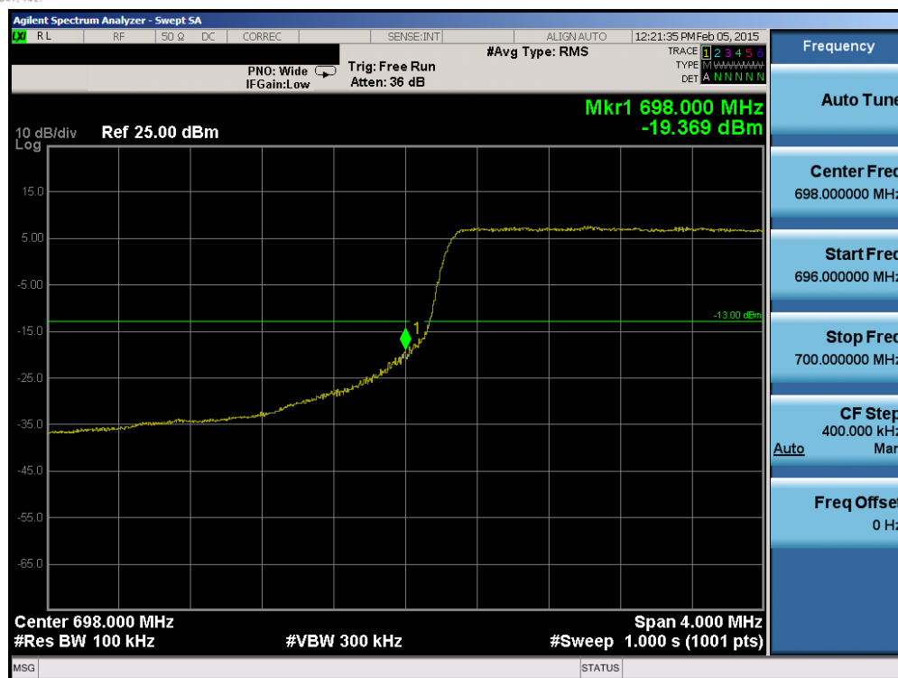
Plot 6-83. Lower Band Edge Plot (Band 12 – 5.0MHz QPSK – RB Size 25)
