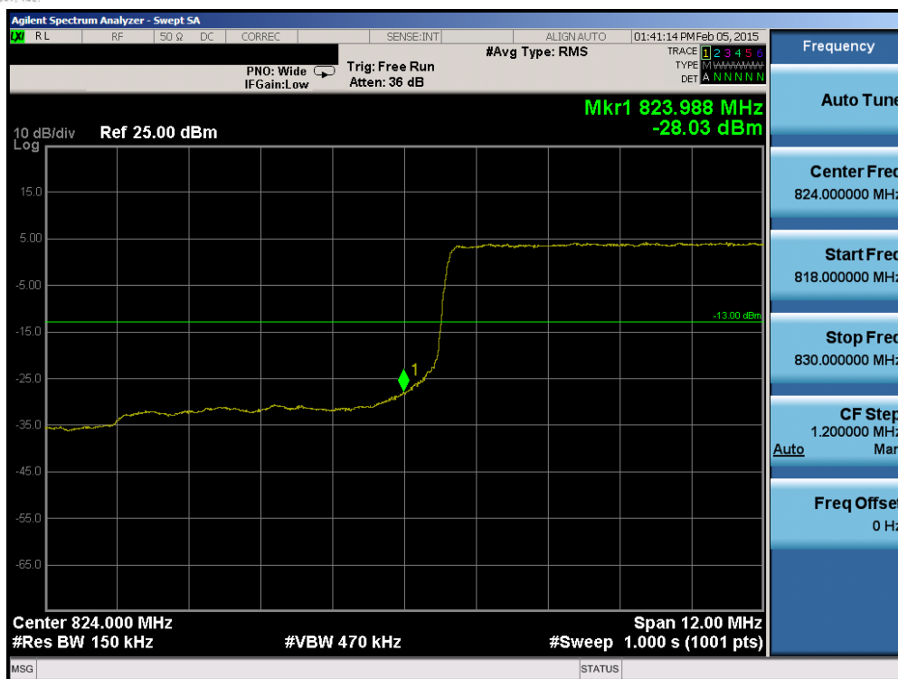
Plot 6-97. Lower Band Edge Plot (Band 26 – 15.0MHz QPSK – RB Size 75)
