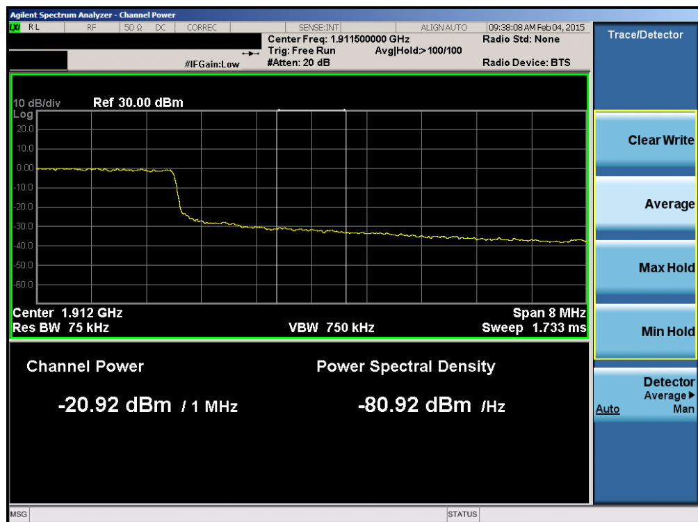
Plot 6-138. Upper Extended Band Edge Plot (Band 2 – 10.0MHz QPSK – RB Size 50)
