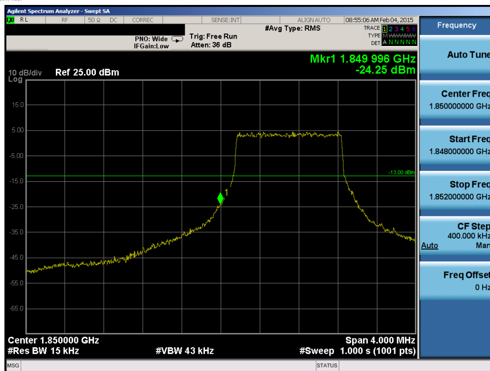
Plot 6-123. Lower Band Edge Plot (Band 2 – 1.4MHz QPSK – RB Size 6)
