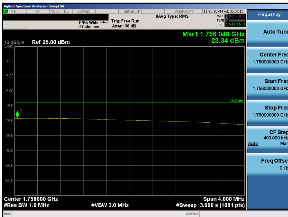
Plot 6-118. Upper Extended Band Edge Plot (Band 4 – 15.0MHz QPSK – RB Size 75)
