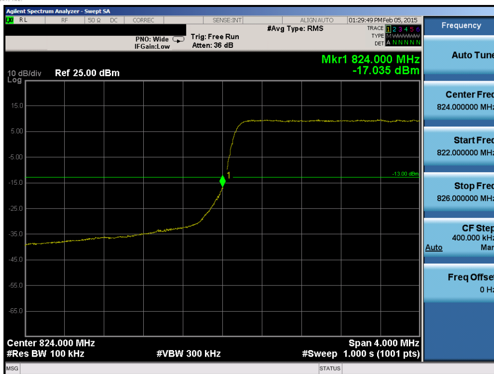
Plot 6-91. Lower Band Edge Plot (Band 5/26 – 3.0MHz QPSK – RB Size 15)
