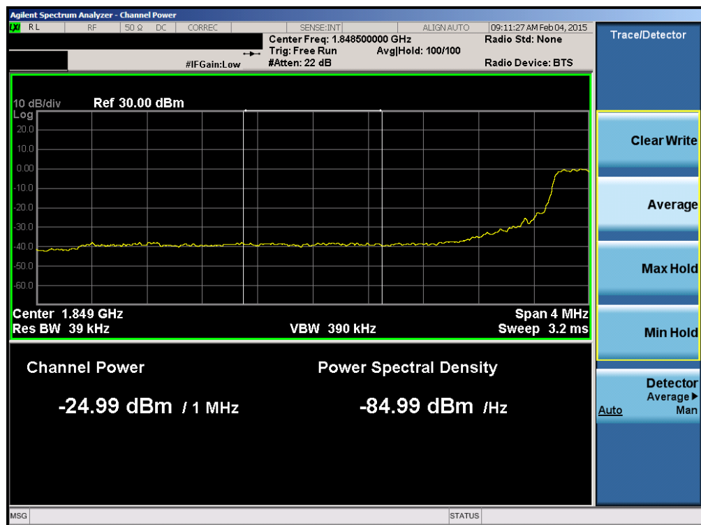
Plot 6-132. Lower Extended Band Edge Plot (Band 2 – 5.0MHz QPSK – RB Size 25)
