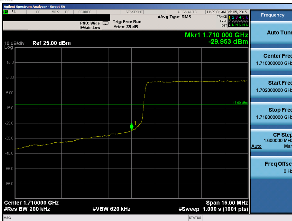
Plot 6-119. Lower Band Edge Plot (Band 4 – 20.0MHz QPSK – RB Size 100)
