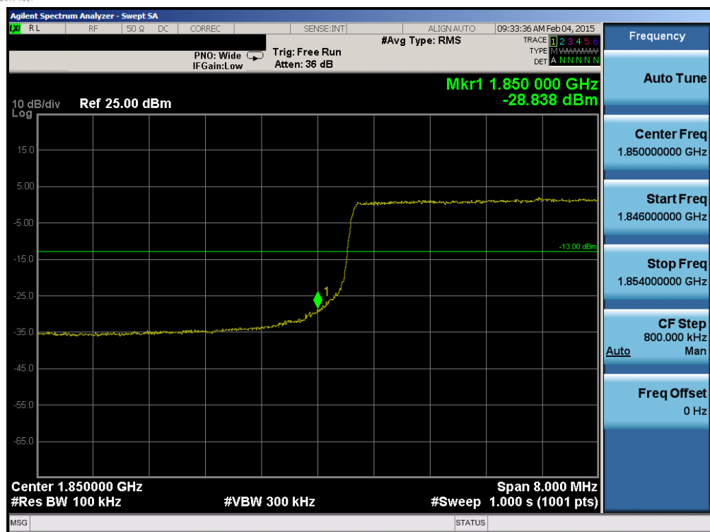
Plot 6-135. Lower Band Edge Plot (Band 2 – 10.0MHz QPSK – RB Size 50)
