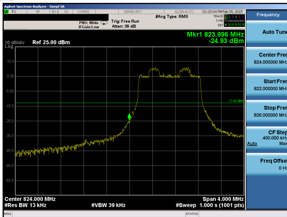
Plot 6-87. Lower Band Edge Plot (Band 5/26 – 1.4MHz QPSK – RB Size 6)
