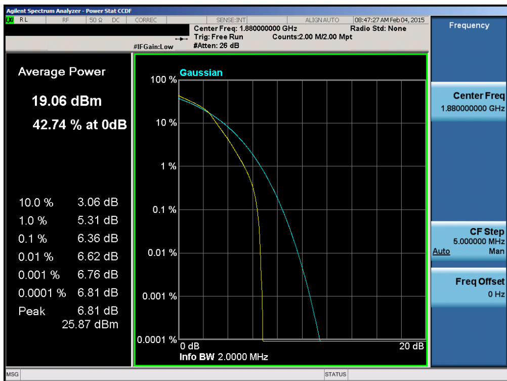
Plot 6-148. PAR Plot (Band 2 – 1.4MHz 16-QAM – RB Size 6)
