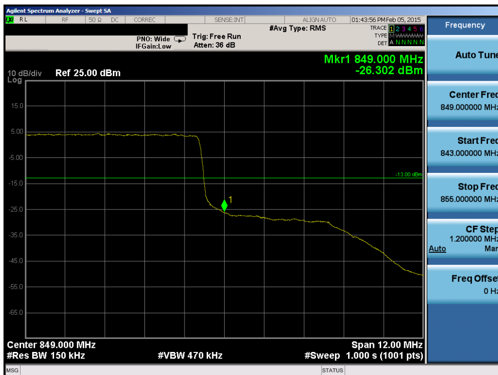
Plot 6-98. Upper Band Edge Plot (Band 26 – 15.0MHz QPSK – RB Size 75)
