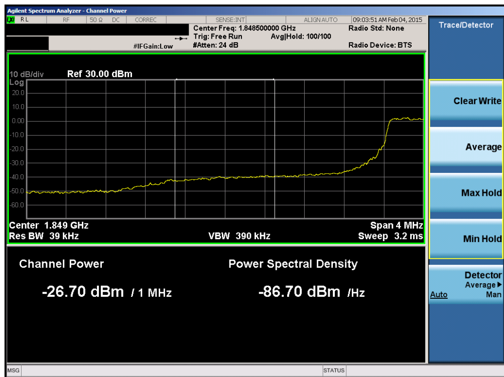
Plot 6-128. Lower Extended Band Edge Plot (Band 2 – 3.0MHz QPSK – RB Size 15)
