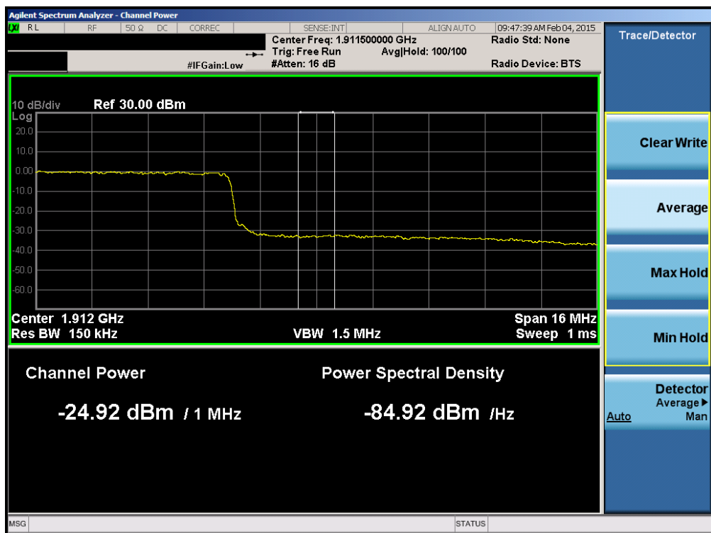
Plot 6-146. Upper Extended Band Edge Plot (Band 2 – 20.0MHz QPSK – RB Size 100)
