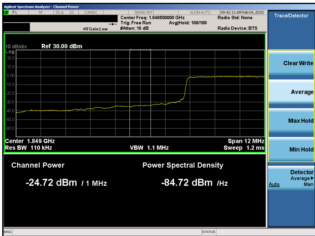
Plot 6-140. Lower Extended Band Edge Plot (Band 2 – 15.0MHz QPSK – RB Size 75)
