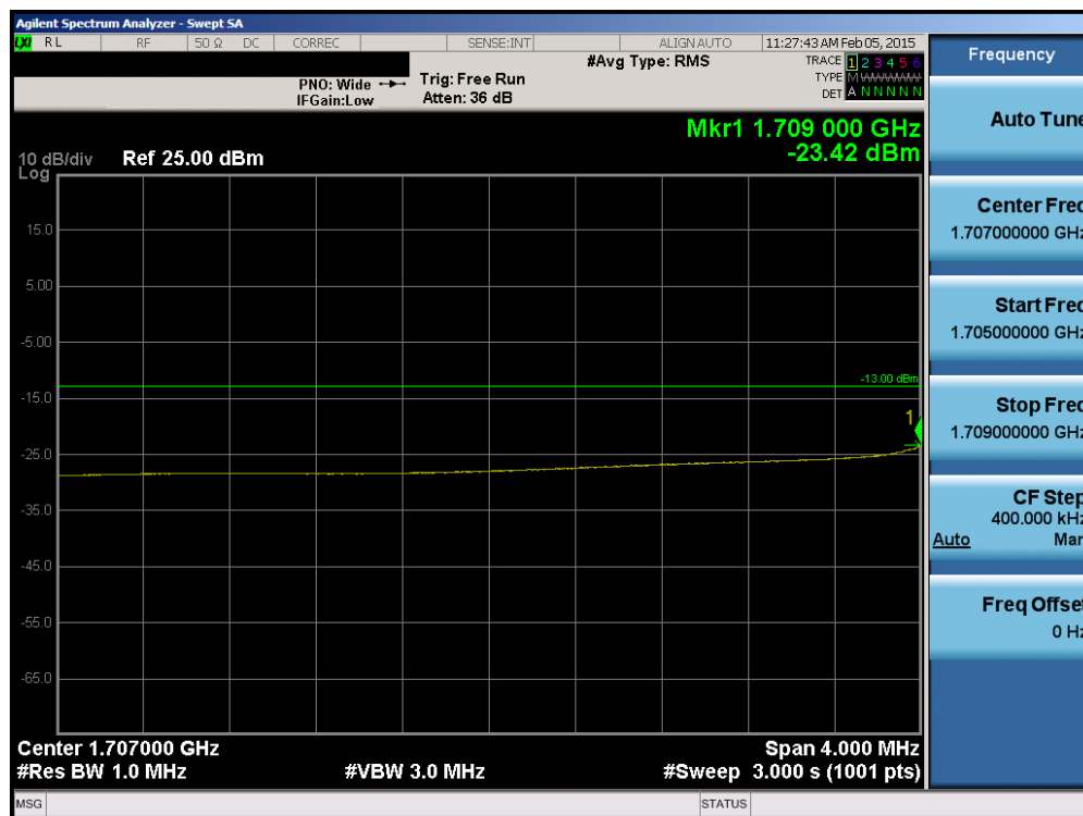
Plot 6-112. Lower Extended Band Edge Plot (Band 4 – 10.0MHz QPSK – RB Size 50)
