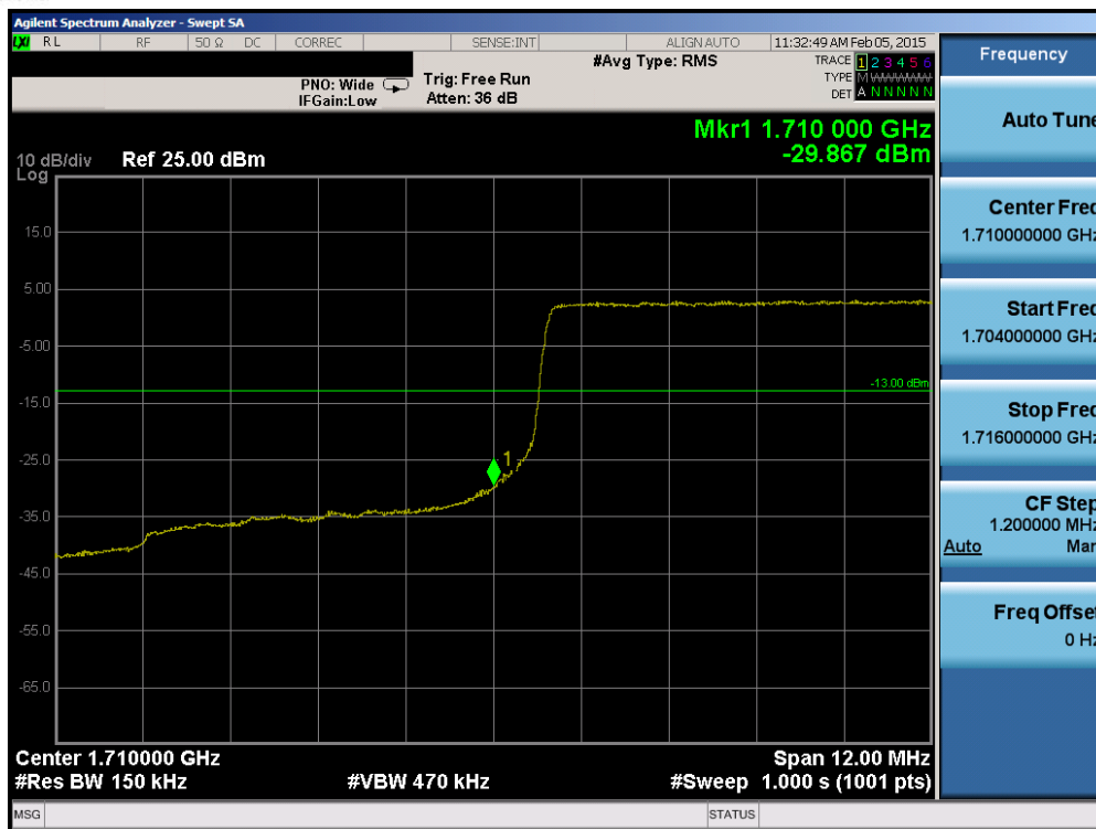
Plot 6-115. Lower Band Edge Plot (Band 4 – 15.0MHz QPSK – RB Size 75)
