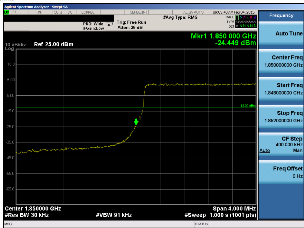
Plot 6-127. Lower Band Edge Plot (Band 2 – 3.0MHz QPSK – RB Size 15)
