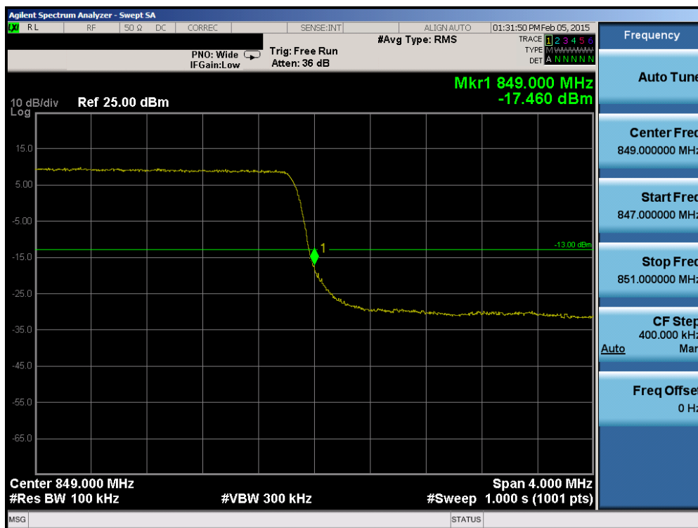
Plot 6-92. Upper Band Edge Plot (Band 5/26 – 3.0MHz QPSK – RB Size 15)
