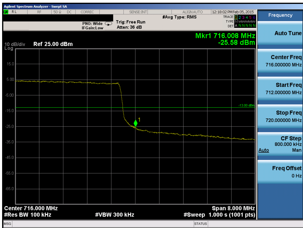
Plot 6-86. Upper Band Edge Plot (Band 12 – 10.0MHz QPSK – RB Size 50)
