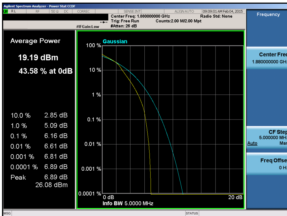
Plot 6-152. PAR Plot (Band 2 – 5.0MHz 16-QAM – RB Size 25)
