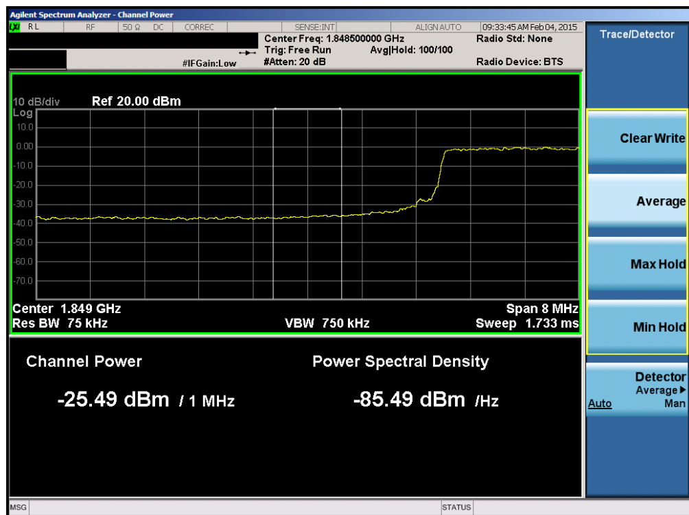
Plot 6-136. Lower Extended Band Edge Plot (Band 2 – 10.0MHz QPSK – RB Size 50)
