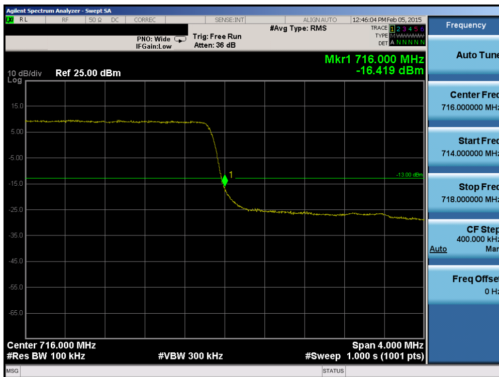
Plot 6-82. Upper Band Edge Plot (Band 12 – 3.0MHz QPSK – RB Size 15)
