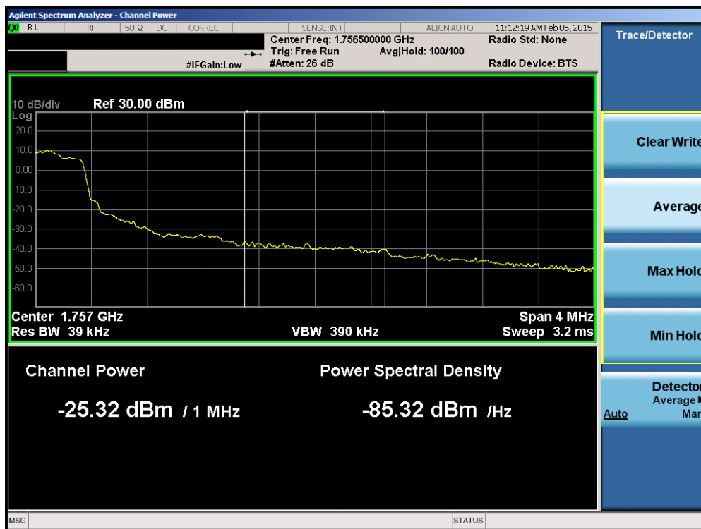
Plot 6-102. Upper Extended Band Edge Plot (Band 4 – 1.4MHz QPSK – RB Size 6)
