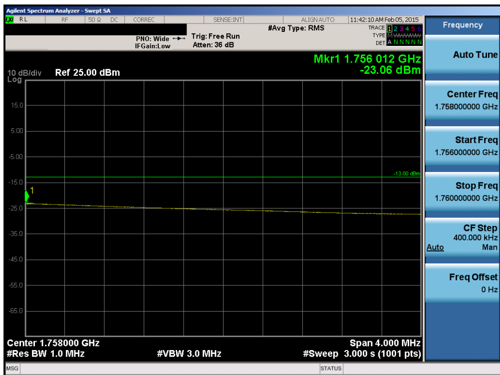
Plot 6-122. Upper Extended Band Edge Plot (Band 4 - 20.0MHz QPSK - RB Size 100)
