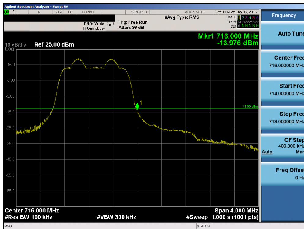
Plot 6-80. Upper Band Edge Plot (Band 12 – 1.4MHz QPSK – RB Size 6)
