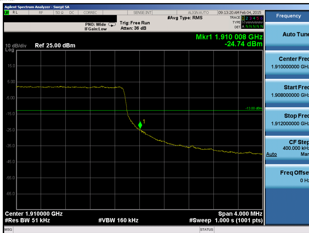
Plot 6-133. Upper Band Edge Plot (Band 2 – 5.0MHz QPSK – RB Size 25)
