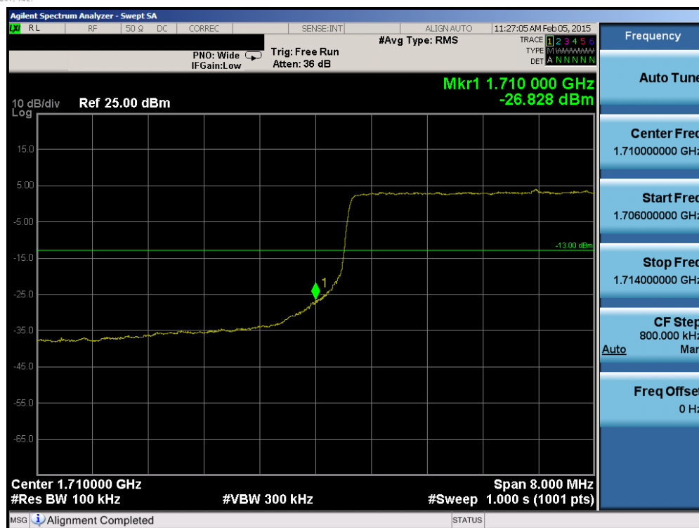
Plot 6-111. Lower Band Edge Plot (Band 4 – 10.0MHz QPSK – RB Size 50)
