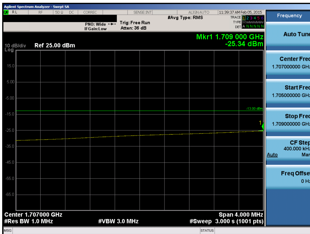
Plot 6-120. Lower Extended Band Edge Plot (Band 4 – 20.0MHz QPSK – RB Size 100)
