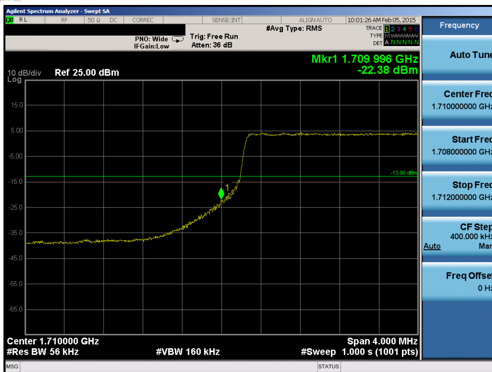
Plot 6-107. Lower Band Edge Plot (Band 4 – 5.0MHz QPSK – RB Size 25)
