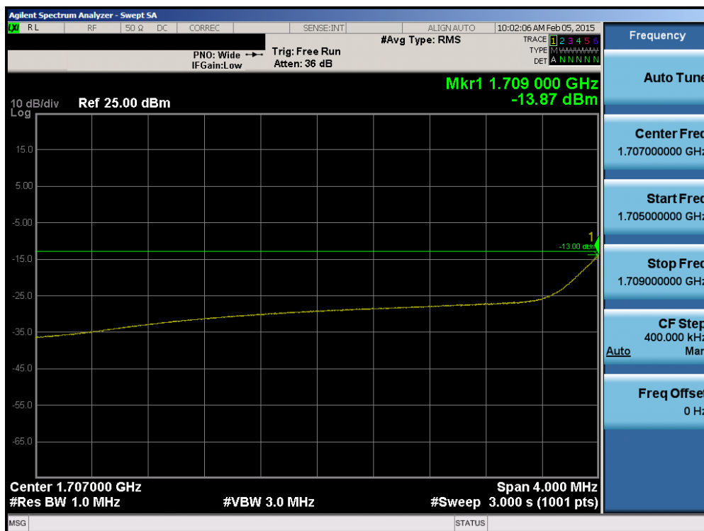
Plot 6-108. Lower Extended Band Edge Plot (Band 4 – 5.0MHz QPSK – RB Size 25)
