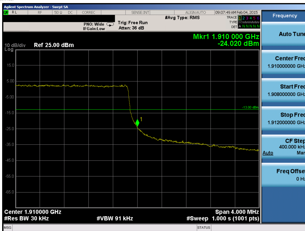
Plot 6-129. Upper Band Edge Plot (Band 2 – 3.0MHz QPSK – RB Size 15)
