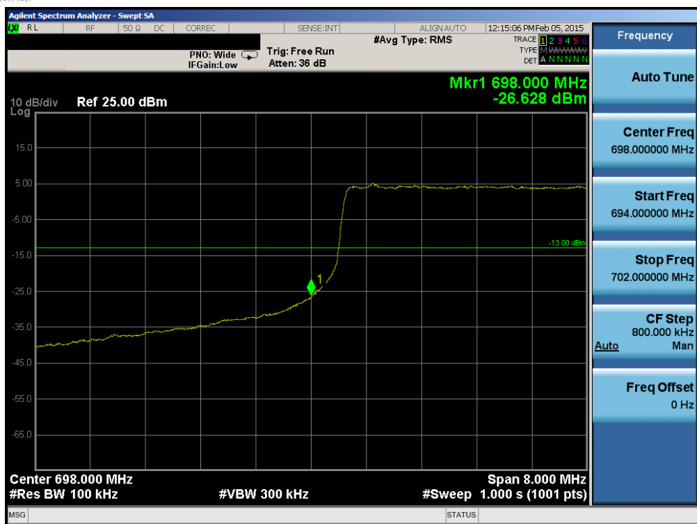
Plot 6-85. Lower Band Edge Plot (Band 12 – 10.0MHz QPSK – RB Size 50)
