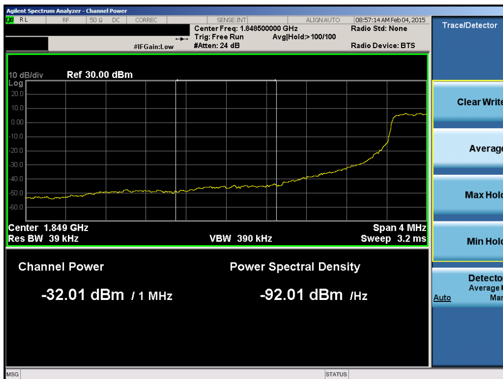
Plot 6-124. Lower Extended Band Edge Plot (Band 2 – 1.4MHz QPSK – RB Size 6)
