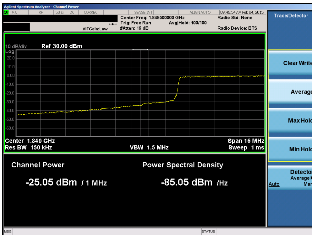
Plot 6-144. Lower Extended Band Edge Plot (Band 2 – 20.0MHz QPSK – RB Size 100)
