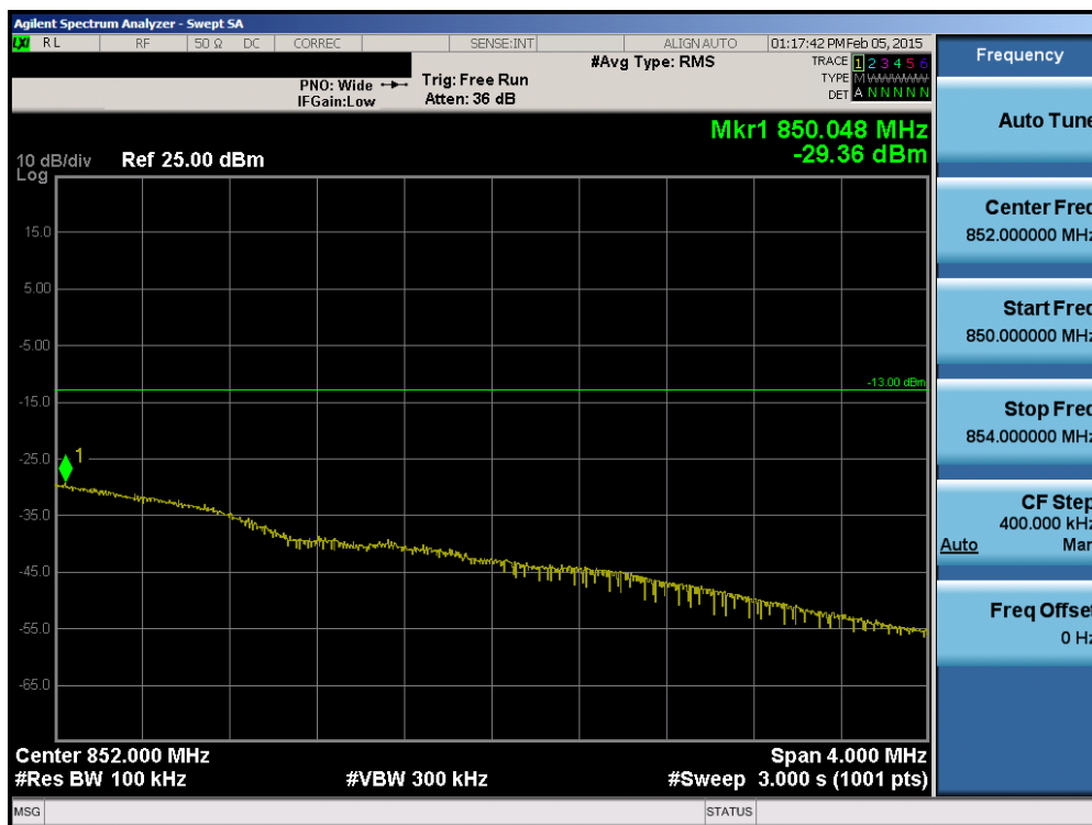
Plot 6-90. Upper Extended Band Edge Plot (Band 5/26 – 1.4MHz QPSK – RB Size 6)
