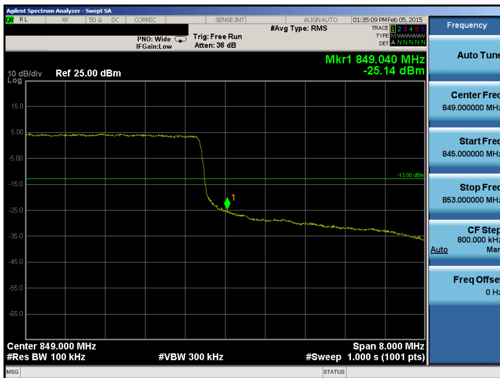
Plot 6-96. Upper Band Edge Plot (Band 5/26 – 10.0MHz QPSK – RB Size 50)
