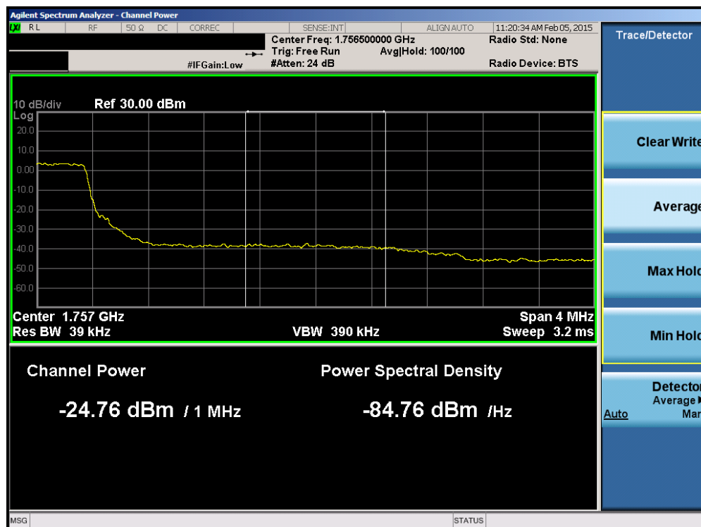
Plot 6-106. Upper Extended Band Edge Plot (Band 4 – 3.0MHz QPSK – RB Size 15)
