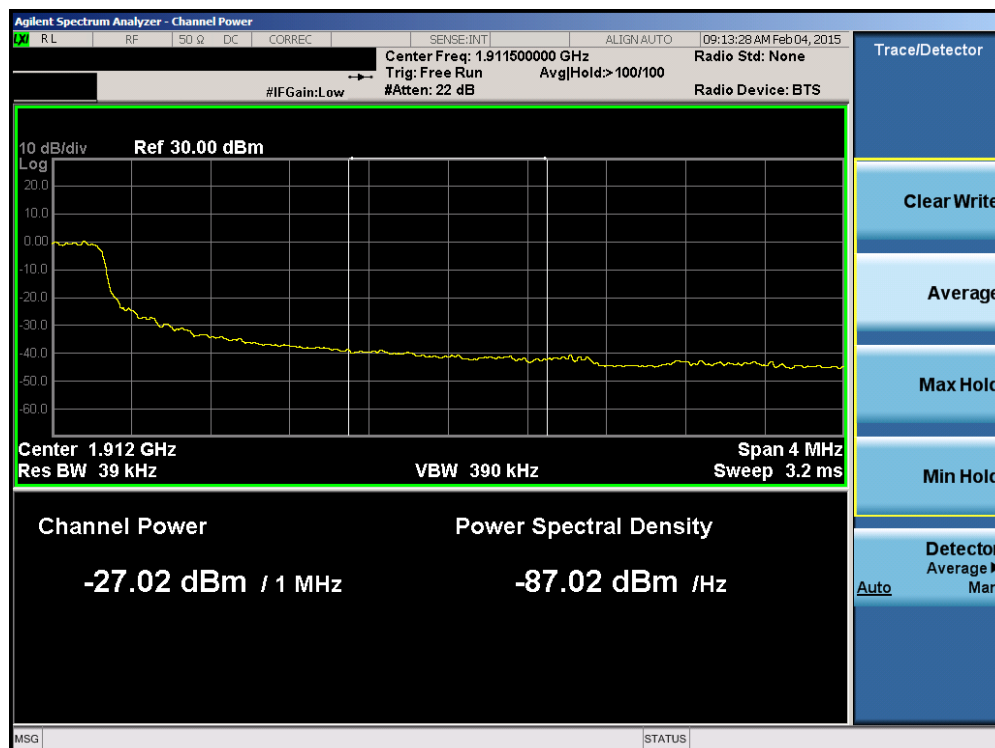
Plot 6-134. Upper Extended Band Edge Plot (Band 2 – 5.0MHz QPSK – RB Size 25)
