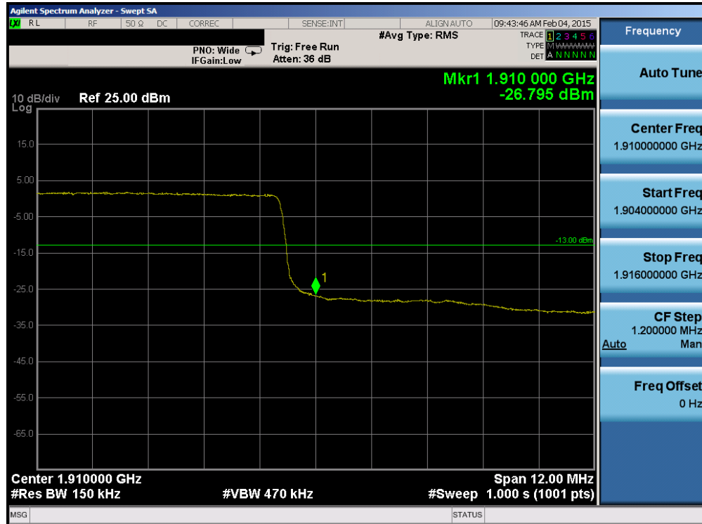
Plot 6-141. Upper Band Edge Plot (Band 2 – 15.0MHz QPSK – RB Size 75)
