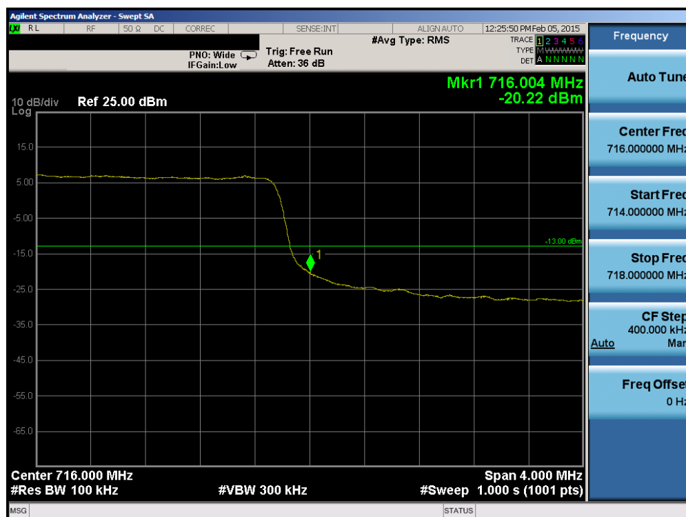
Plot 6-84. Upper Band Edge Plot (Band 12 – 5.0MHz QPSK – RB Size 25)
