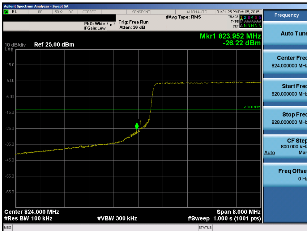
Plot 6-95. Lower Band Edge Plot (Band 5/26 – 10.0MHz QPSK – RB Size 50)
