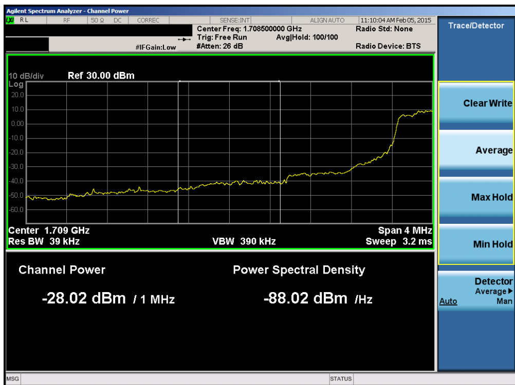
Plot 6-100. Lower Extended Band Edge Plot (Band 4 – 1.4MHz QPSK – RB Size 6)
