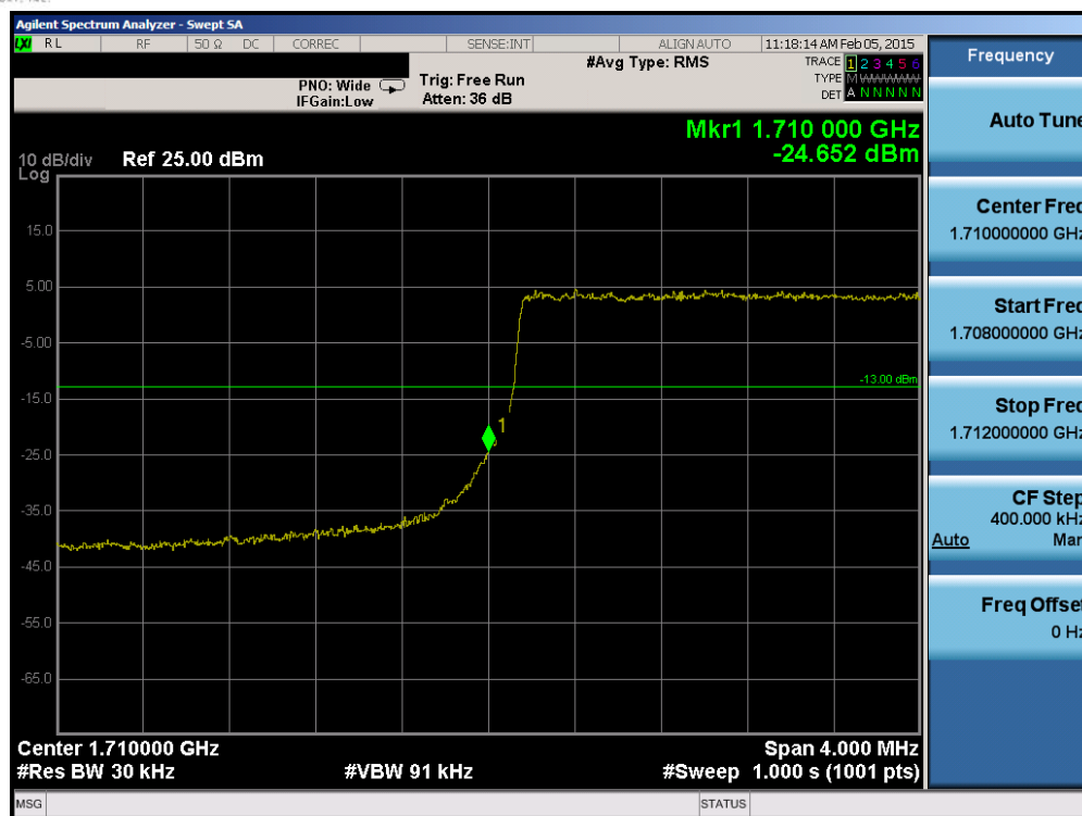
Plot 6-103. Lower Band Edge Plot (Band 4 – 3.0MHz QPSK – RB Size 15)
