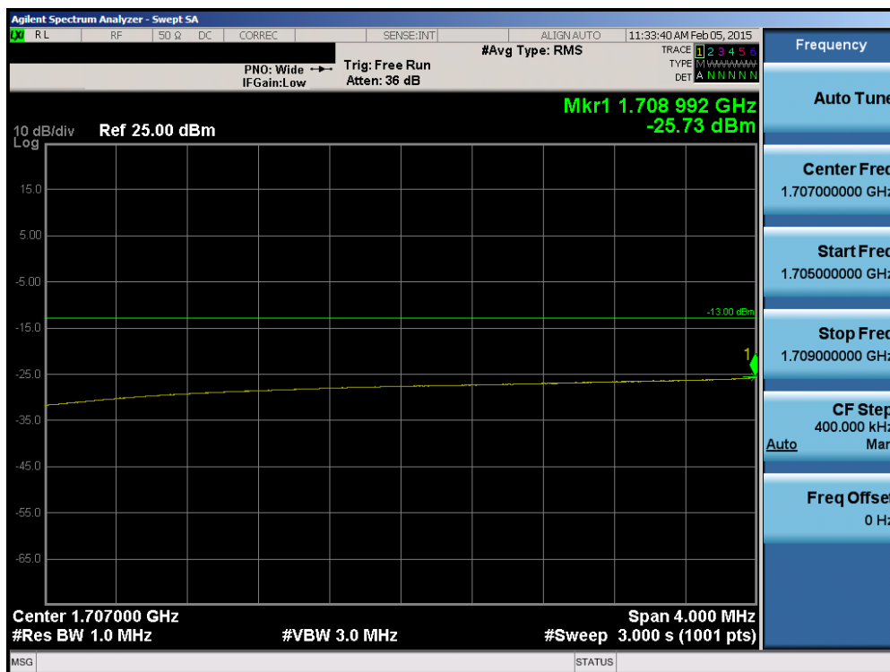
Plot 6-116. Lower Extended Band Edge Plot (Band 4 – 15.0MHz QPSK – RB Size 75)
