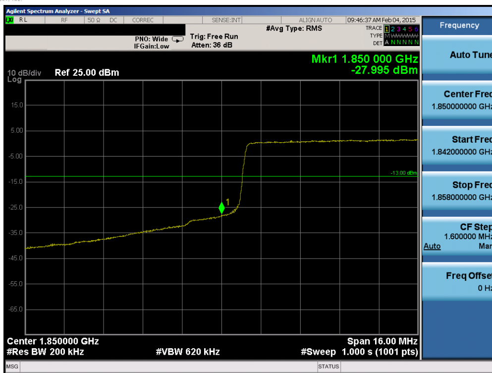
Plot 6-143. Lower Band Edge Plot (Band 2 – 20.0MHz QPSK – RB Size 100)
