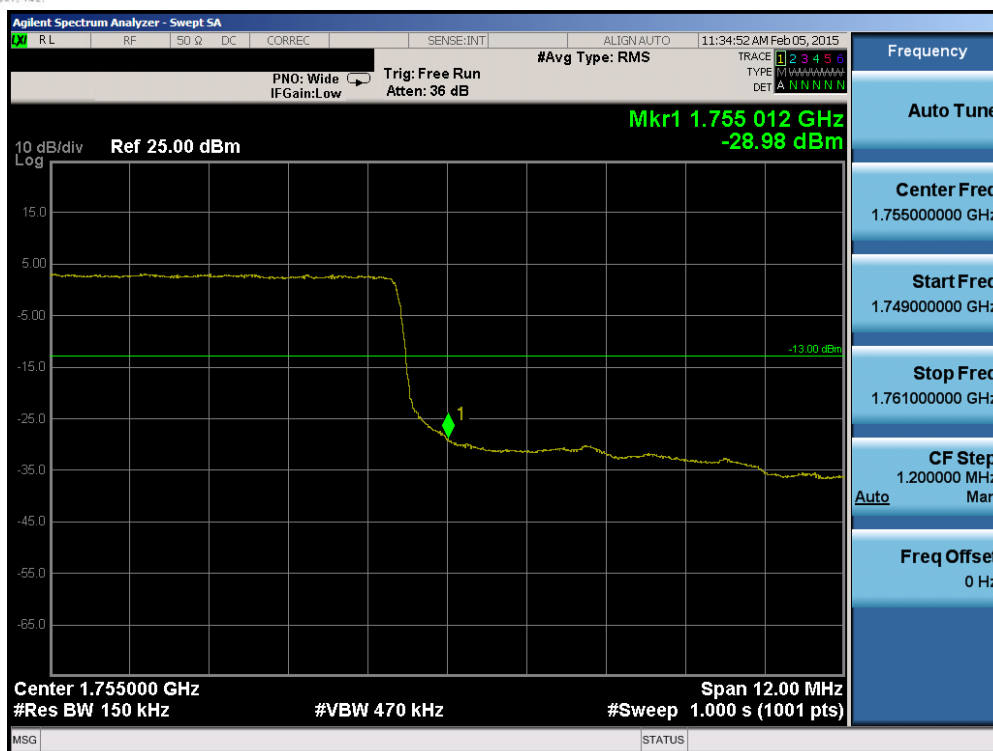
Plot 6-117. Upper Band Edge Plot (Band 4 – 15.0MHz QPSK – RB Size 75)
