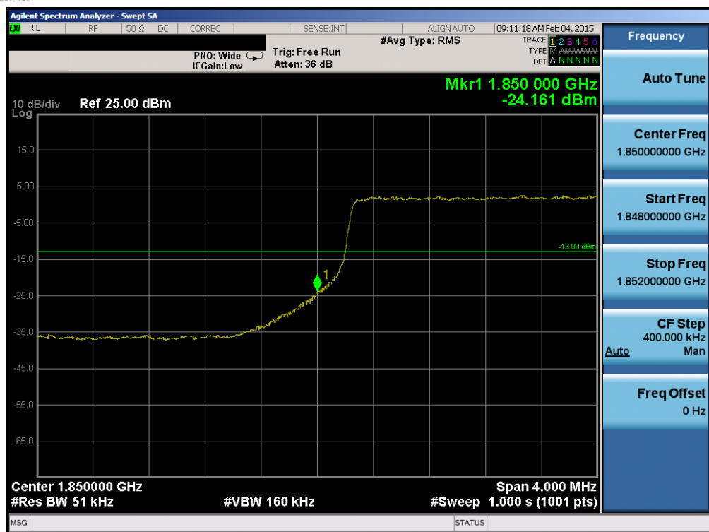
Plot 6-131. Lower Band Edge Plot (Band 2 – 5.0MHz QPSK – RB Size 25)
