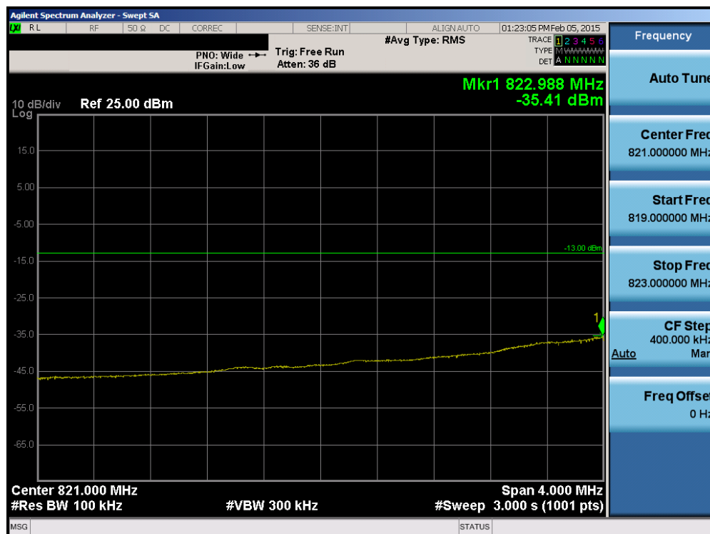
Plot 6-88. Lower Extended Band Edge Plot (Band 5/26 – 1.4MHz QPSK – RB Size 6)
