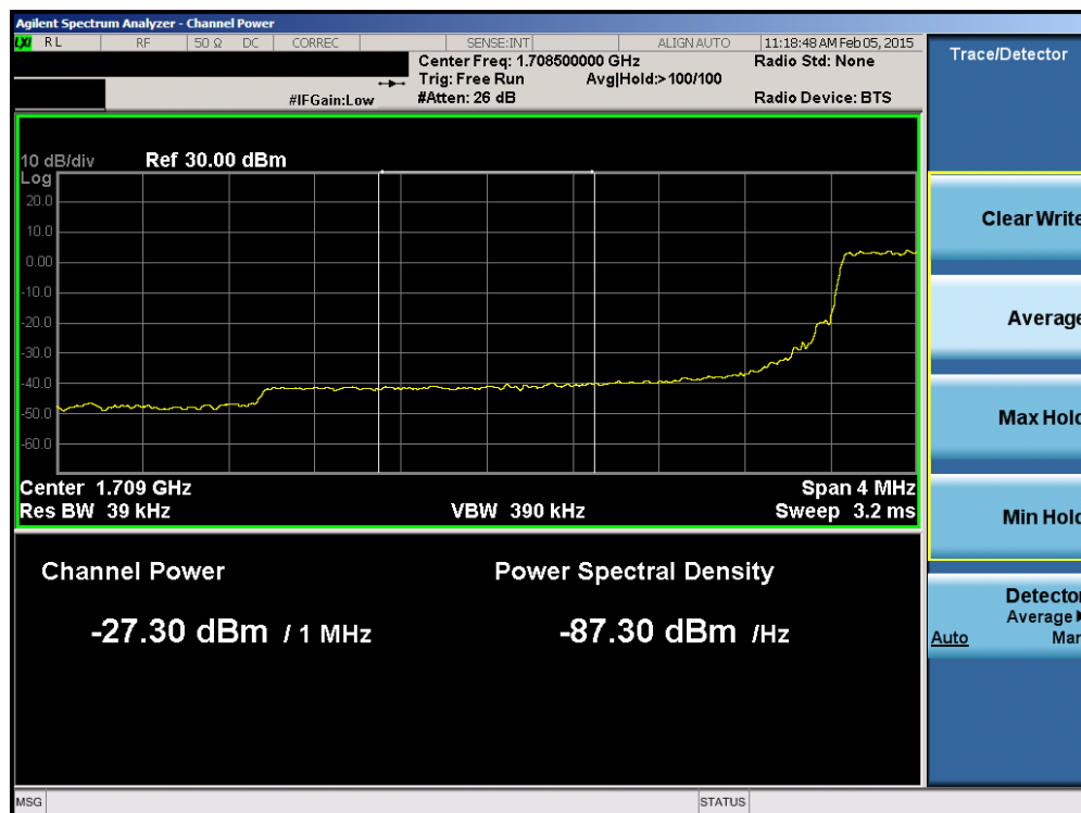
Plot 6-104. Lower Extended Band Edge Plot (Band 4 – 3.0MHz QPSK – RB Size 15)
