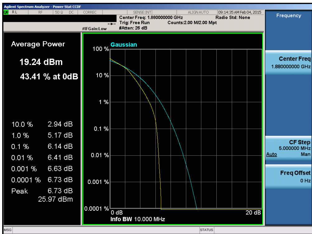
Plot 6-154. PAR Plot (Band 2 – 10.0MHz 16-QAM – RB Size 50)
