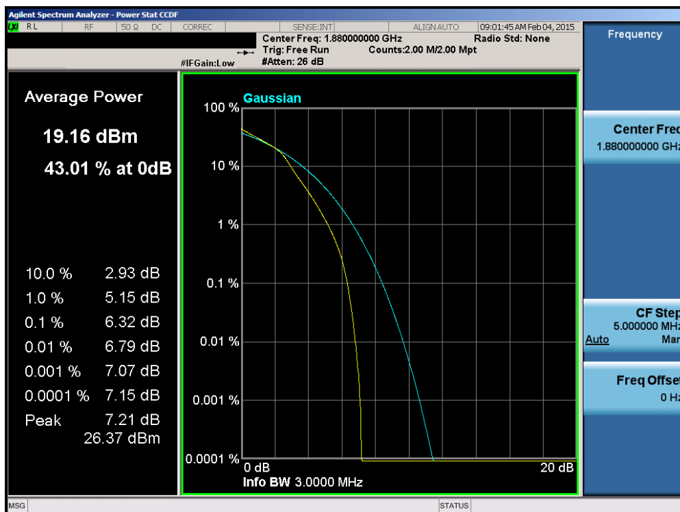
Plot 6-150. PAR Plot (Band 2 – 3.0MHz 16-QAM – RB Size 15)
