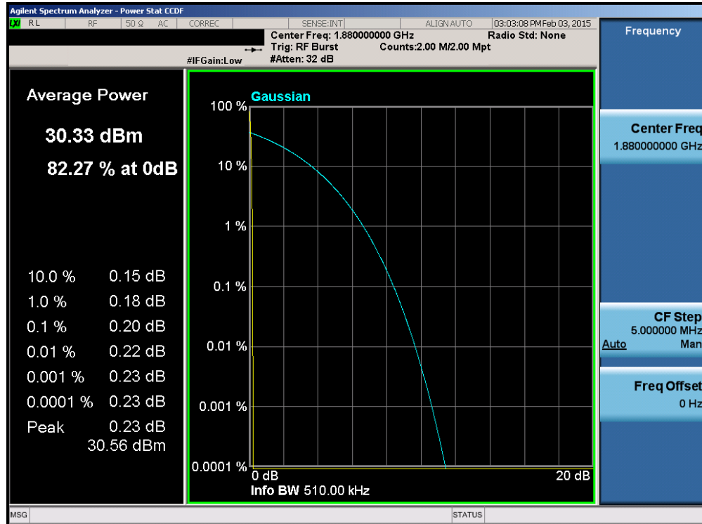
Plot 6-63. Peak-Average Ratio Plot (PCS GSM Mode – Ch. 661)
