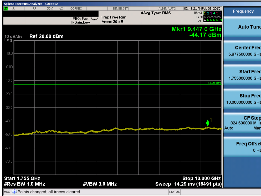
Plot 6-36. Conducted Spurious Plot (AWS WCDMA Mode – Ch. 1412)
