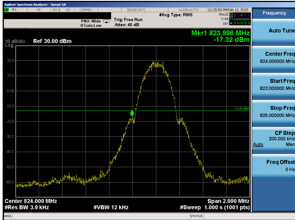
Plot 6-47. Band Edge Plot (Cellular GSM Mode – Ch. 128)
