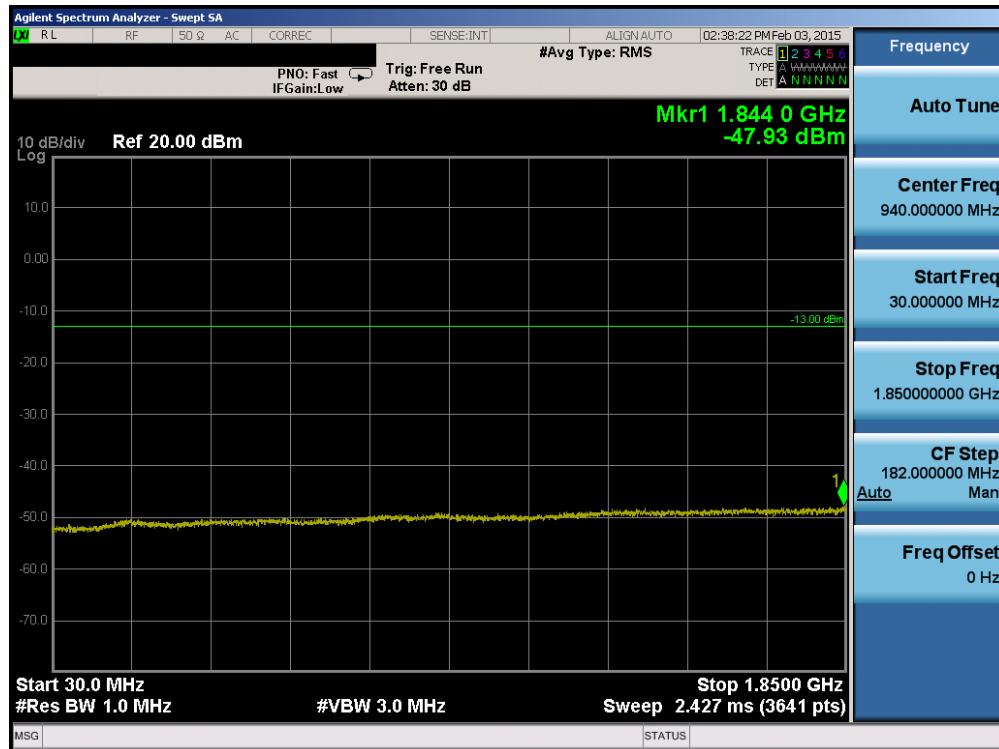
Plot 6-45. Conducted Spurious Plot (PCS WCDMA Mode – Ch. 9538)
