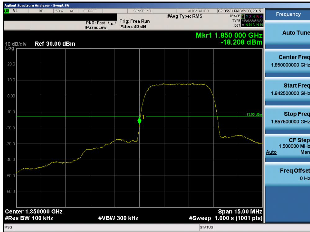
Plot 6-59. Band Edge Plot (PCS WCDMA Mode – Ch. 9262)
