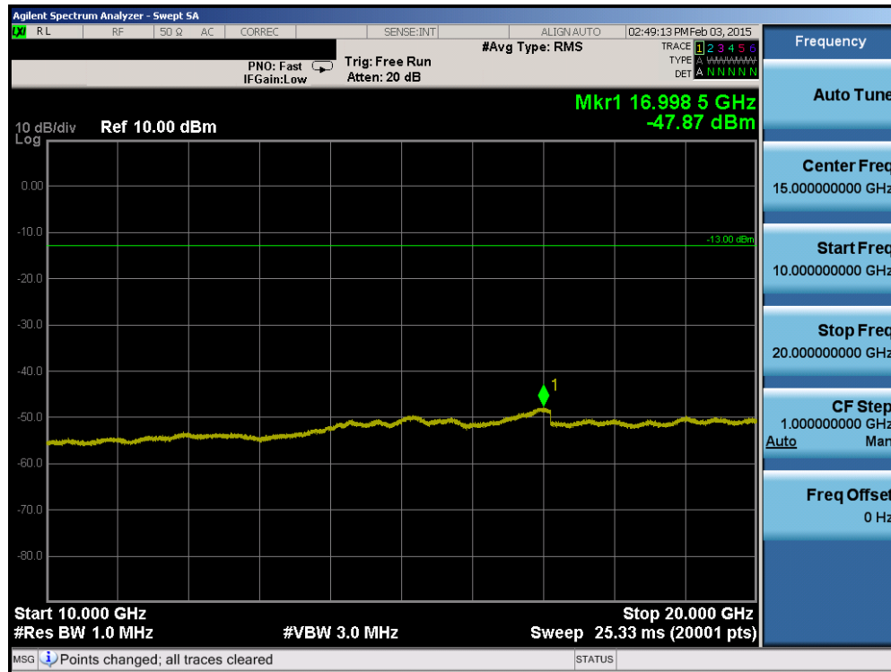
Plot 6-37. Conducted Spurious Plot (AWS WCDMA Mode – Ch. 1412)
