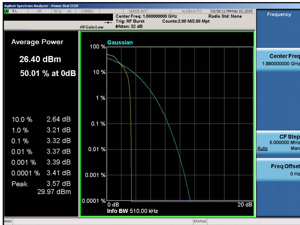
Plot 6-64. Peak-Average Ratio Plot (EDGE1900 Mode – Ch. 661)
