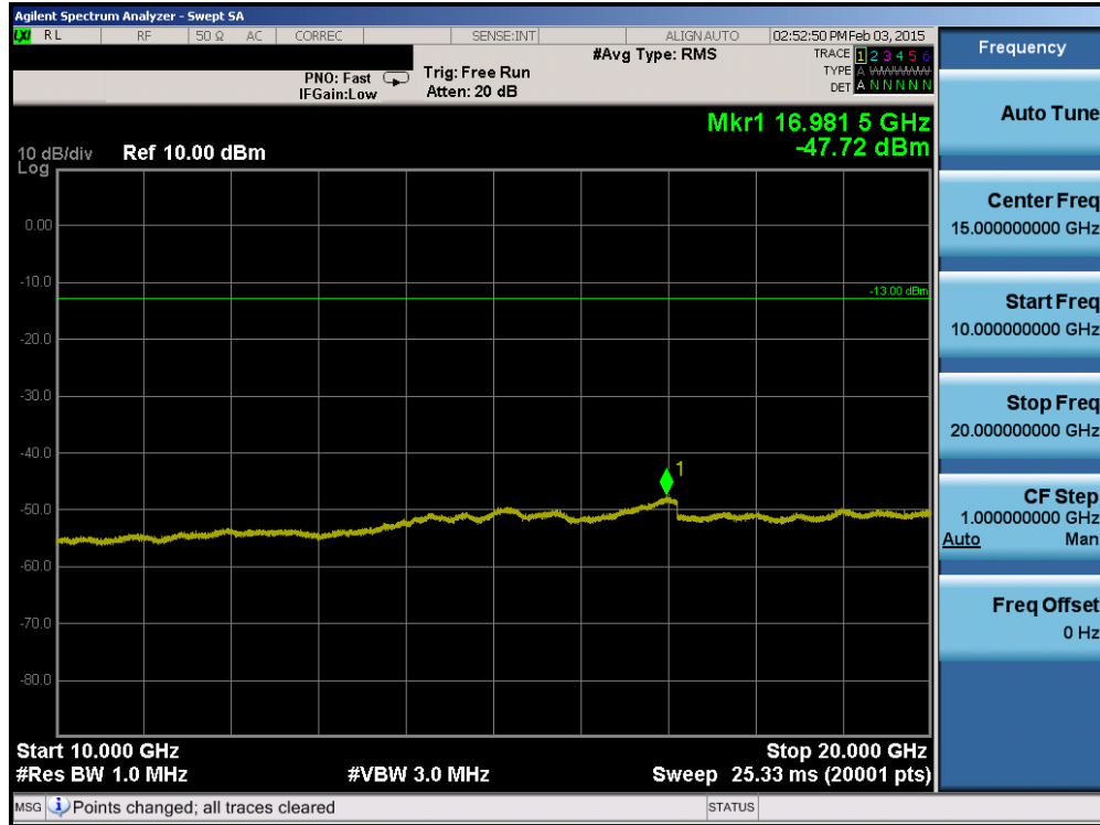
Plot 6-34. Conducted Spurious Plot (AWS WCDMA Mode – Ch. 1312)
