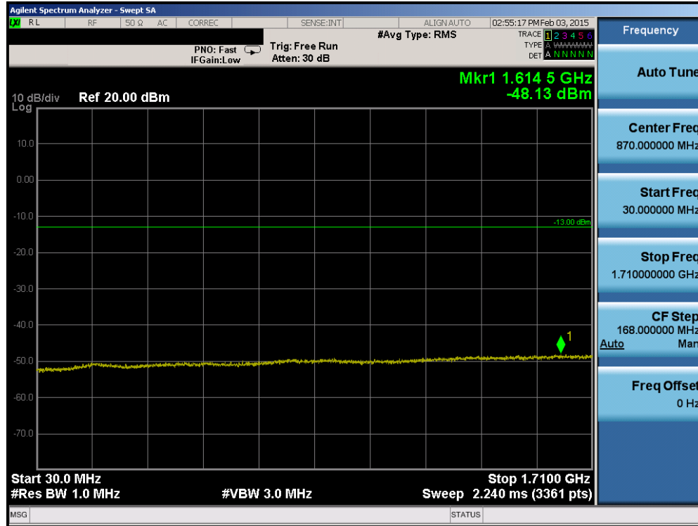
Plot 6-38. Conducted Spurious Plot (AWS WCDMA Mode – Ch. 1862)
