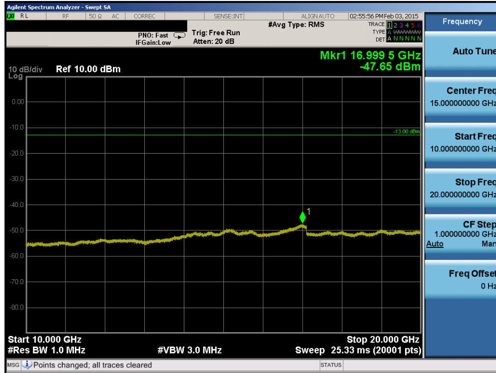
Plot 6-40. Conducted Spurious Plot (AWS WCDMA Mode – Ch. 1862)
