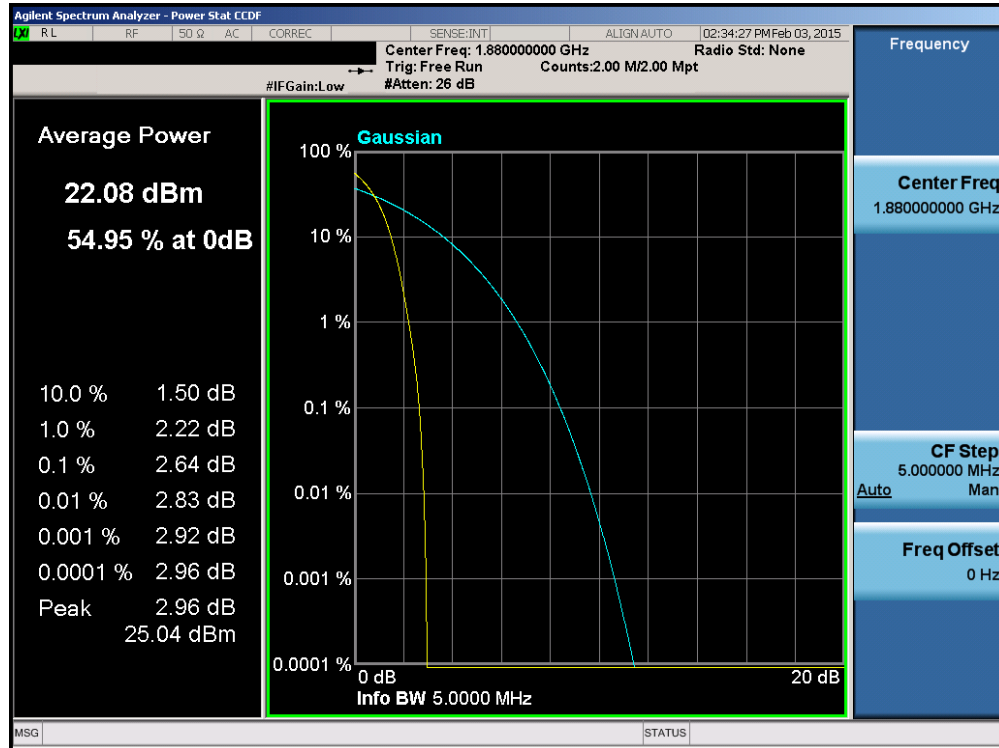
Plot 6-65. Peak-Average Ratio Plot (PCS WCDMA Mode – Ch. 9400)
