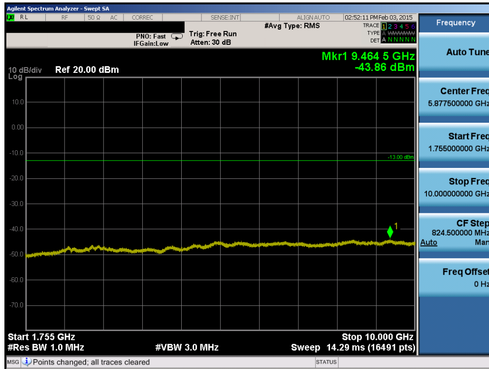
Plot 6-33. Conducted Spurious Plot (AWS WCDMA Mode – Ch. 1312)
