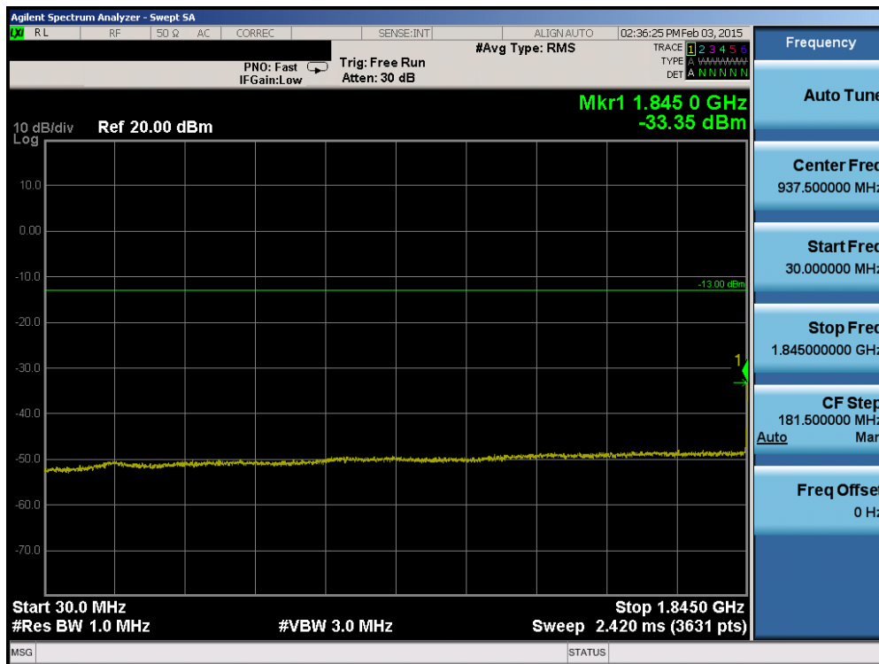
Plot 6-41. Conducted Spurious Plot (PCS WCDMA Mode – Ch. 9262)
