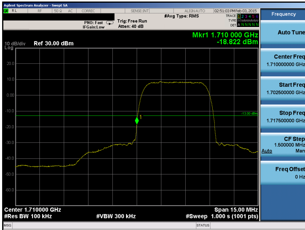
Plot 6-55. Band Edge Plot (AWS WCDMA Mode – Ch. 1312)
