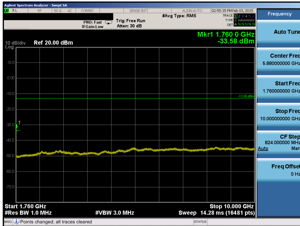
Plot 6-39. Conducted Spurious Plot (AWS WCDMA Mode – Ch. 1862)
