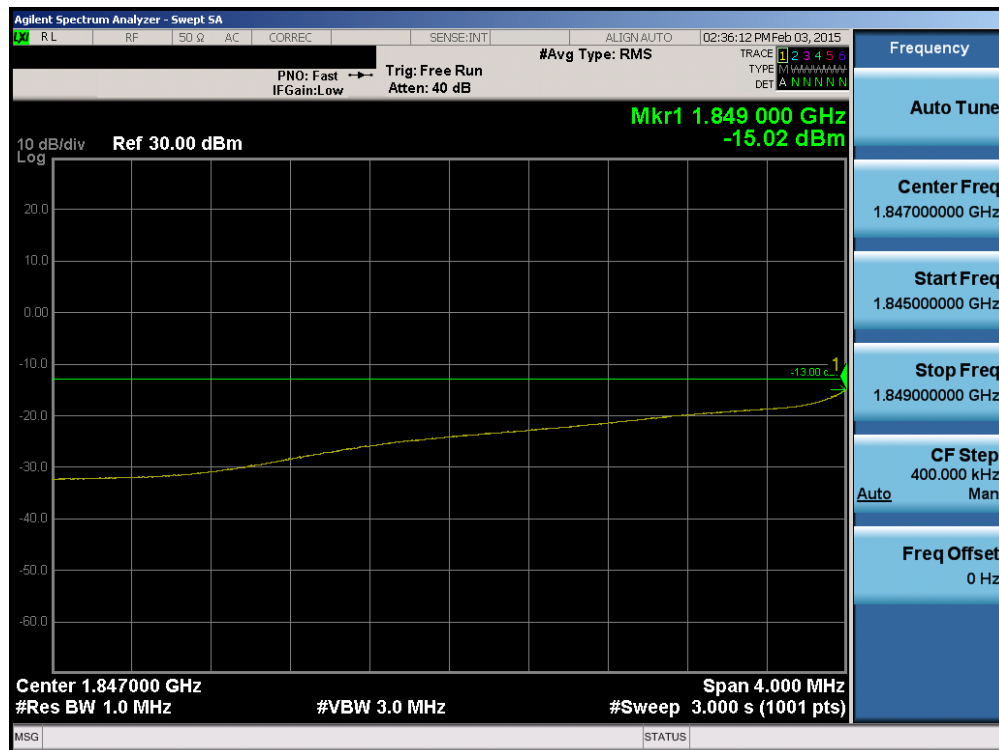
Plot 6-60. 4MHz Span Plot (PCS WCDMA Mode – Ch. 9262)
