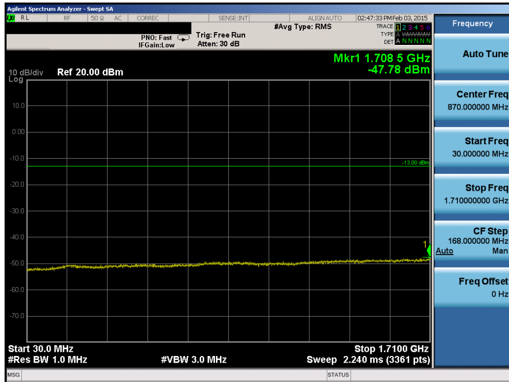
Plot 6-35. Conducted Spurious Plot (AWS WCDMA Mode – Ch. 1412)
