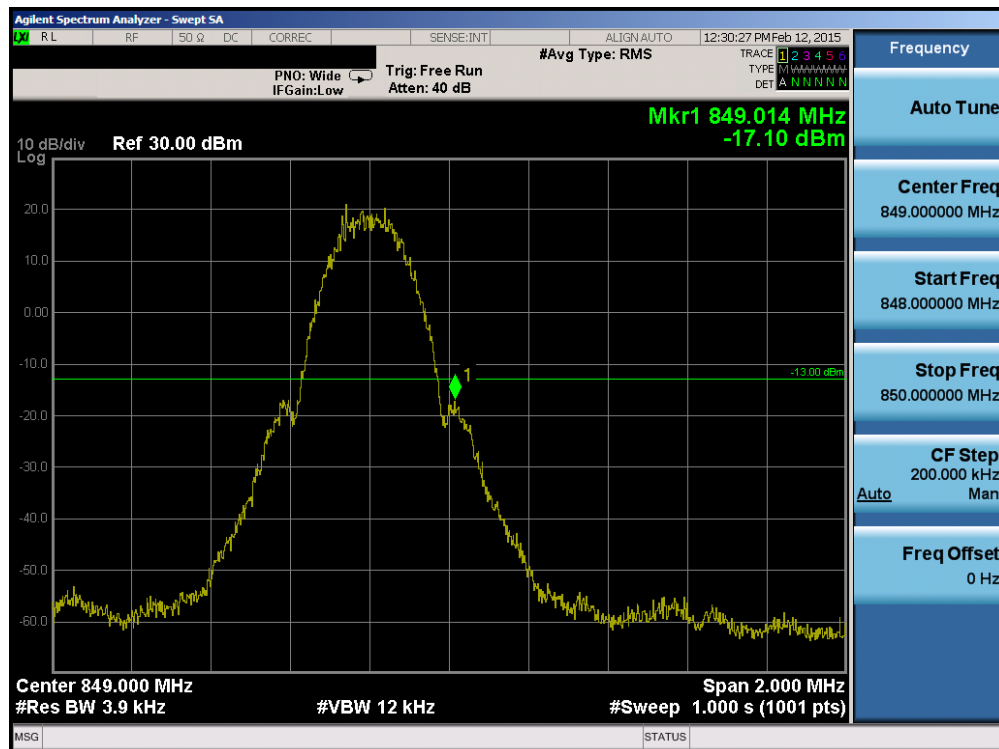
Plot 6-48. Band Edge Plot (Cellular GSM Mode – Ch. 251)
