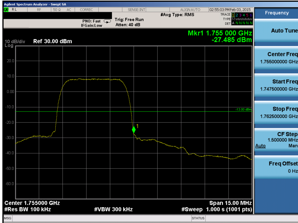
Plot 6-57. Band Edge Plot (AWS WCDMA Mode – Ch. 1862)
