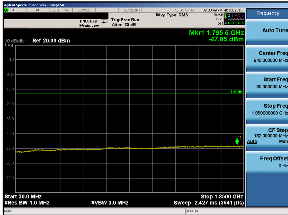
Plot 6-43. Conducted Spurious Plot (PCS WCDMA Mode – Ch. 9400)
