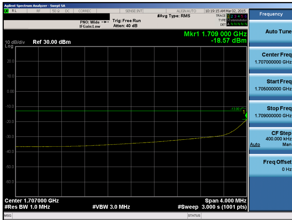
Plot 6-56. 4MHz Span Plot (AWS WCDMA Mode – Ch. 1312)
