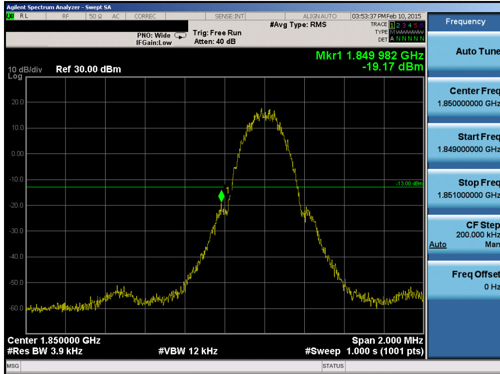
Plot 6-49. Band Edge Plot (PCS GSM Mode – Ch. 512)
