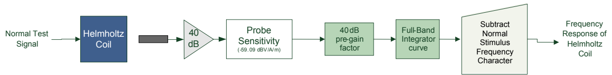
Figure 4-12 Frequency Response Block Diagram
