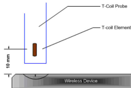
Figure 4-10 Measurement Distance
