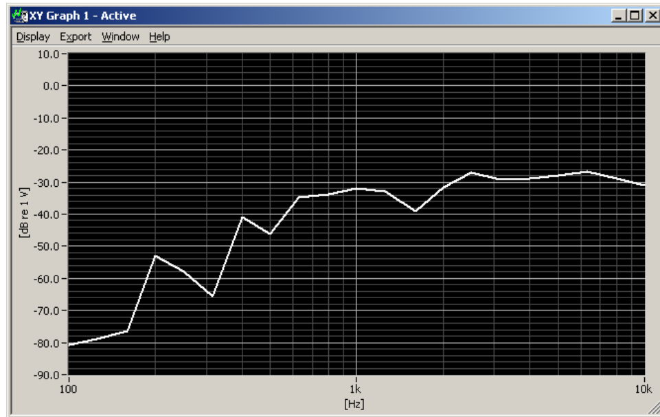
Figure 6-2 Worst-case ABM2 Plot for GSM
