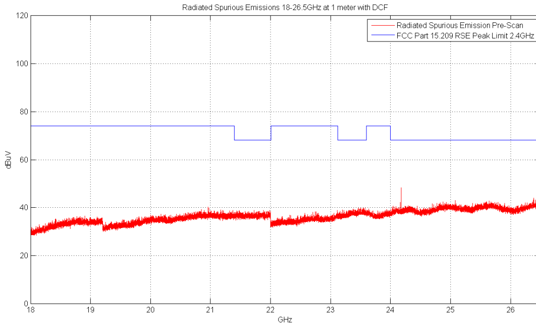
Plot 6-69. Radiated Spurious Plot above 18GHz (Pol. H)
