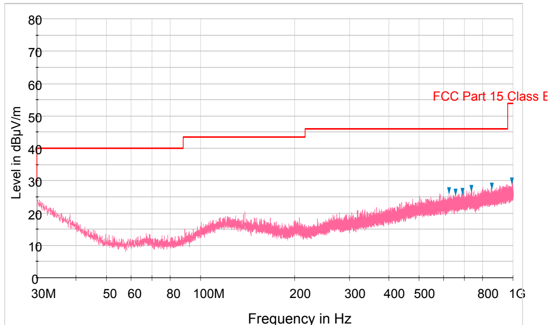
Plot 6-85. Radiated Spurious Plot below 1GHz (Pol. H)
