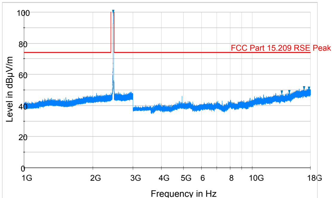
Plot 6-60. Radiated Spurious Plot above 1GHz (802.11b – Ch. 11, Ant. Pol. V)
