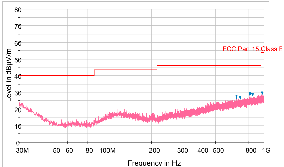
Plot 6-83. Radiated Spurious Plot below 1GHz (Pol. H)
