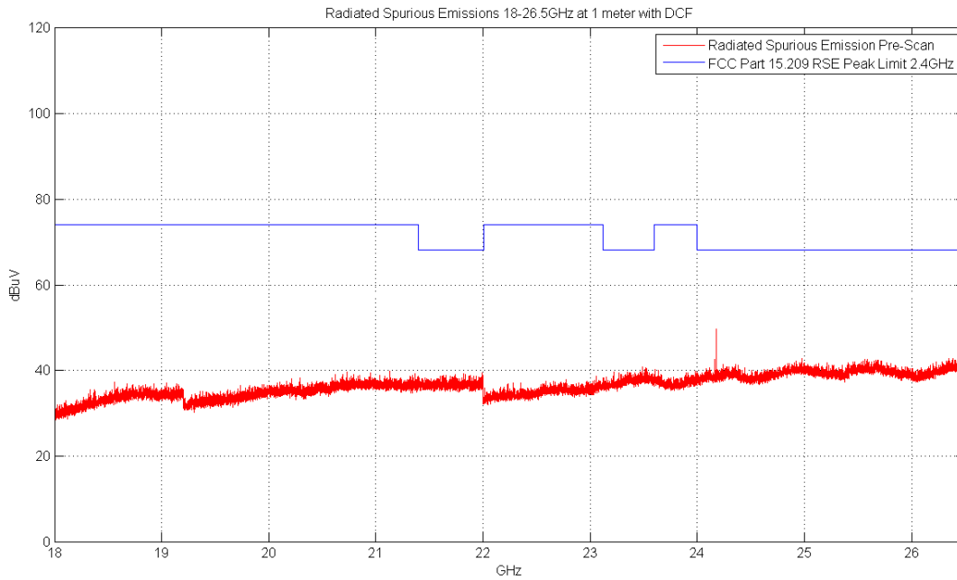
Plot 6-61. Radiated Spurious Plot above 18GHz (Pol. H)
