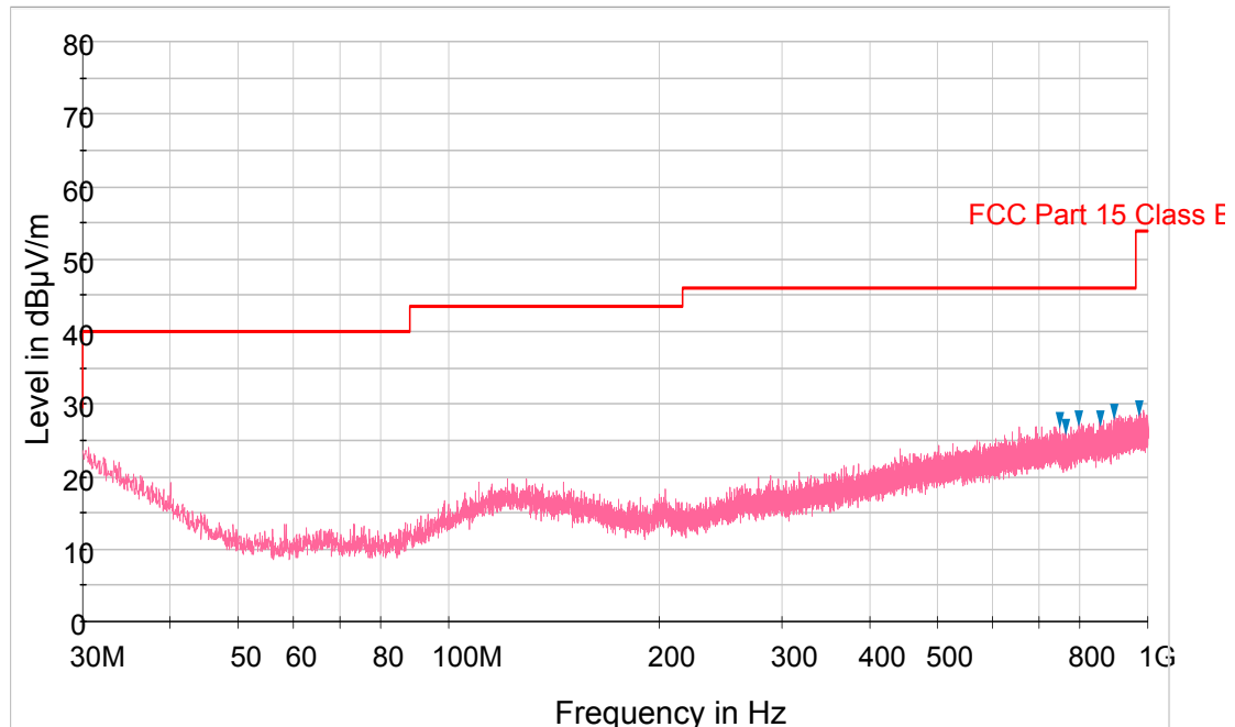
Plot 6-84. Radiated Spurious Plot below 1GHz (Pol. V)
