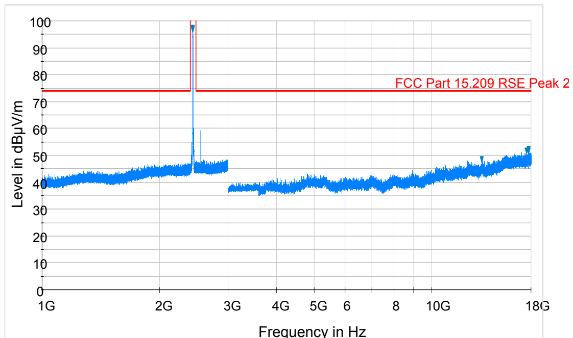
Plot 6-57. Radiated Spurious Plot above 1GHz (802.11b – Ch. 6, Ant. Pol. H)
