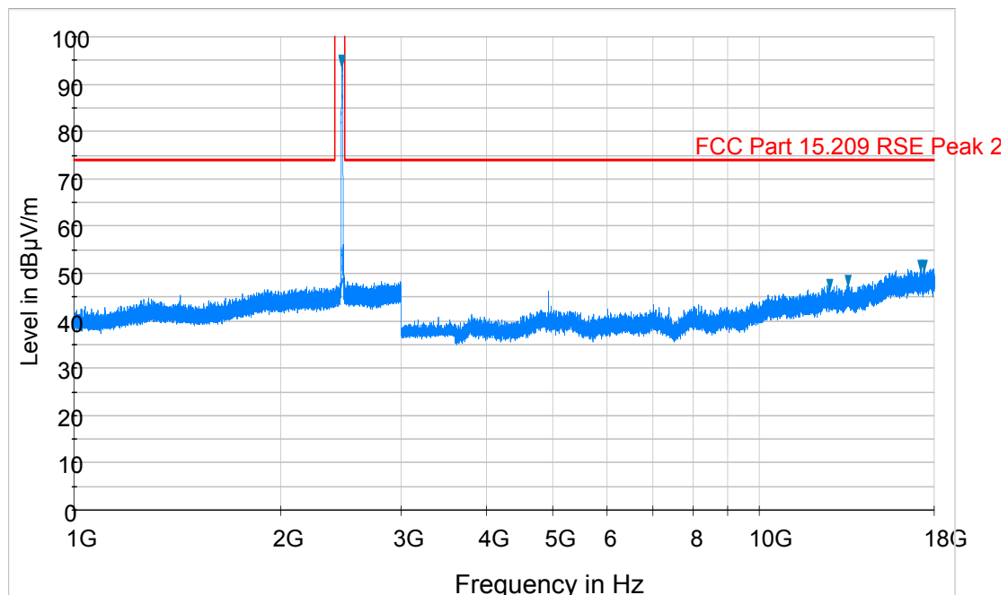
Plot 6-67. Radiated Spurious Plot above 1GHz (802.11b – Ch. 11, Ant. Pol. H)
