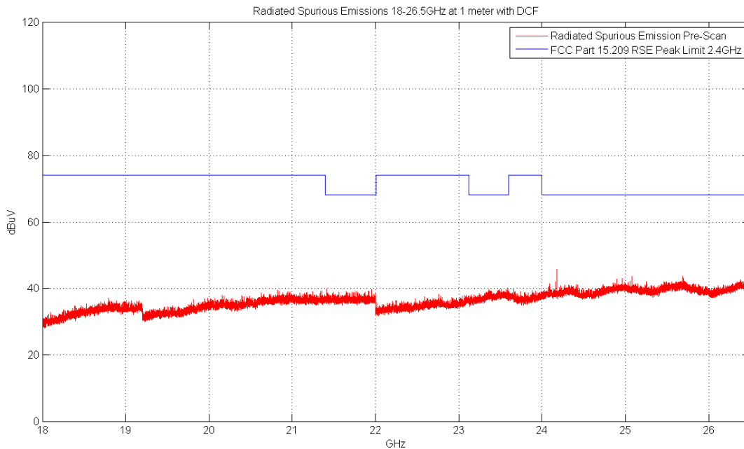
Plot 6-70. Radiated Spurious Plot above 18GHz (Pol. V)
