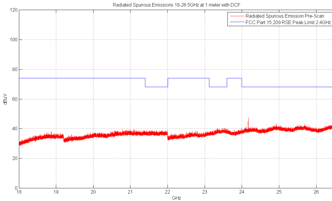
Plot 6-62. Radiated Spurious Plot above 18GHz (Pol. V)
