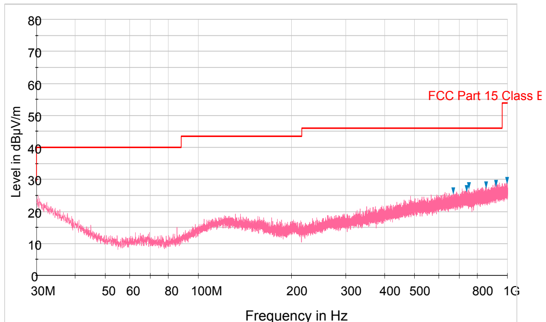
Plot 6-86. Radiated Spurious Plot below 1GHz (Pol. V)
