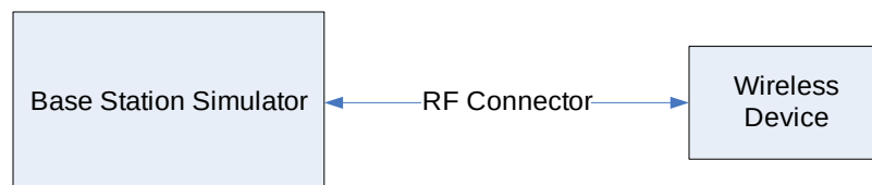
Figure 9-1 Power Measurement Setup
