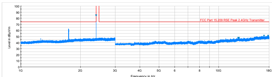
Plot 6-19. Radiated Spurious Plot above 1GHz (BTLE – Ch. 0, Ant. Pol. V)
