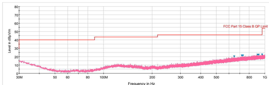
Plot 6-28. Radiated Spurious Plot below 1GHz (Pol. H)
