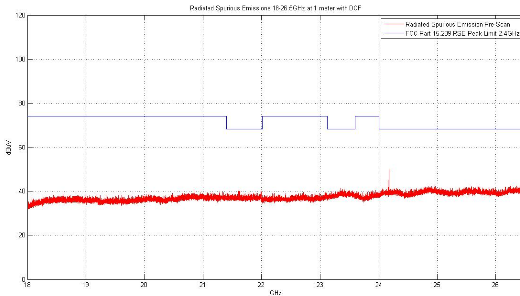
Plot 6-25. Radiated Spurious Plot above 18GHz (Pol. V)
