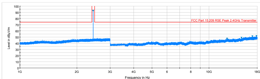
Plot 6-20. Radiated Spurious Plot above 1GHz (BTLE – Ch. 19, Ant. Pol. H)
