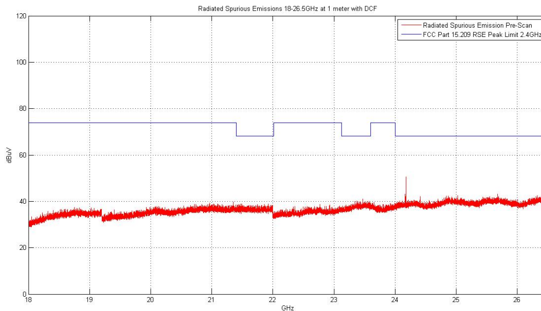
Plot 6-24. Radiated Spurious Plot above 18GHz (Pol. H)
