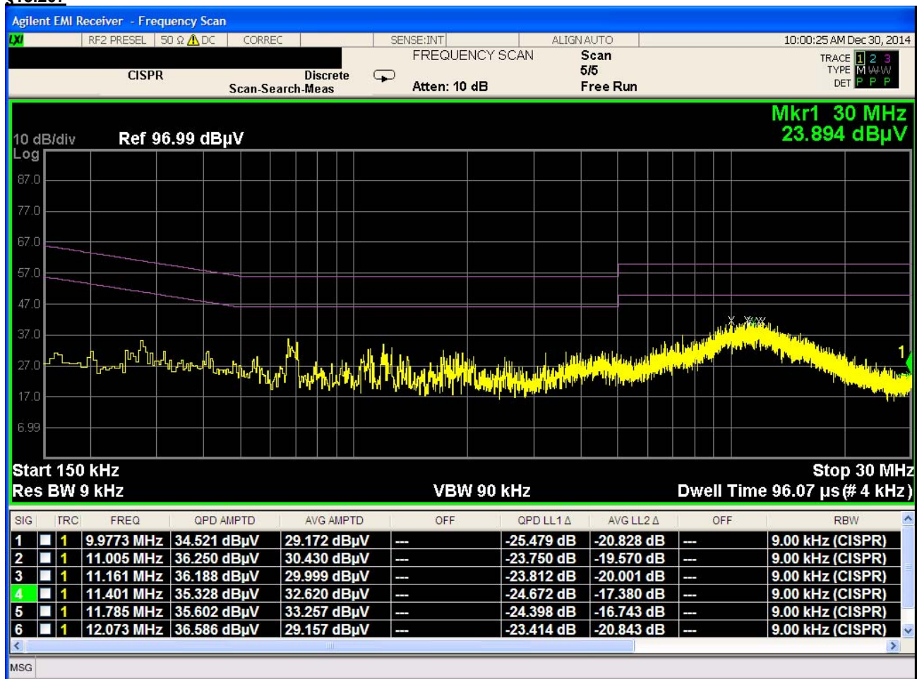
Plot 6-31. Line Conducted Plot with Bluetooth LE (N)
