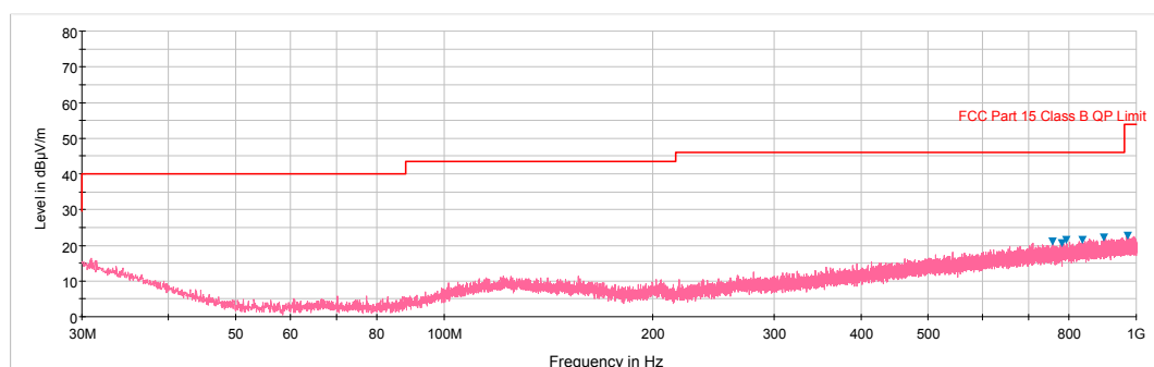
Plot 6-29. Radiated Spurious Plot below 1GHz (Pol. V)
