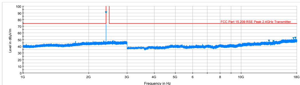
Plot 6-18. Radiated Spurious Plot above 1GHz (BTLE – Ch. 0, Ant. Pol. H)
