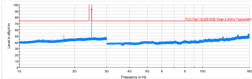
Plot 6-23. Radiated Spurious Plot above 1GHz (BTLE – Ch. 39, Ant. Pol. V)
