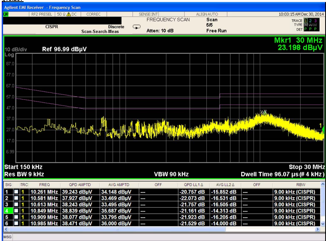
Plot 6-30. Line Conducted Plot with Bluetooth LE (L1)
