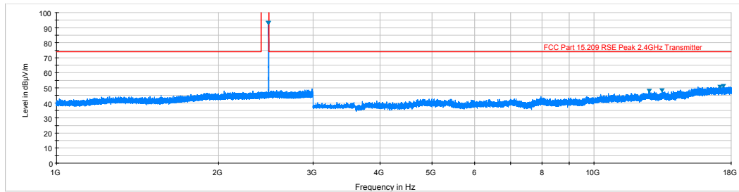
Plot 6-22. Radiated Spurious Plot above 1GHz (BTLE – Ch. 39, Ant. Pol. H)
