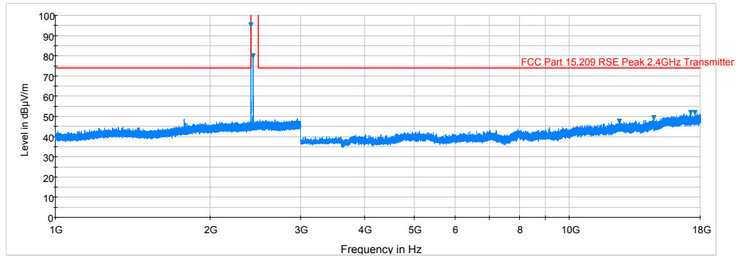
Plot 6-42. Radiated Spurious Plot above 1GHz (BT – Ch. 0, Ant. Pol. H)
