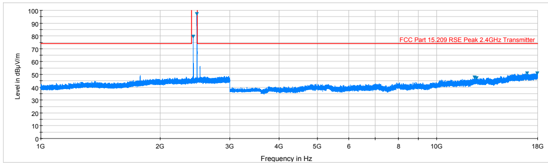
Plot 6-46. Radiated Spurious Plot above 1GHz (BT – Ch. 78, Ant. Pol. H)
