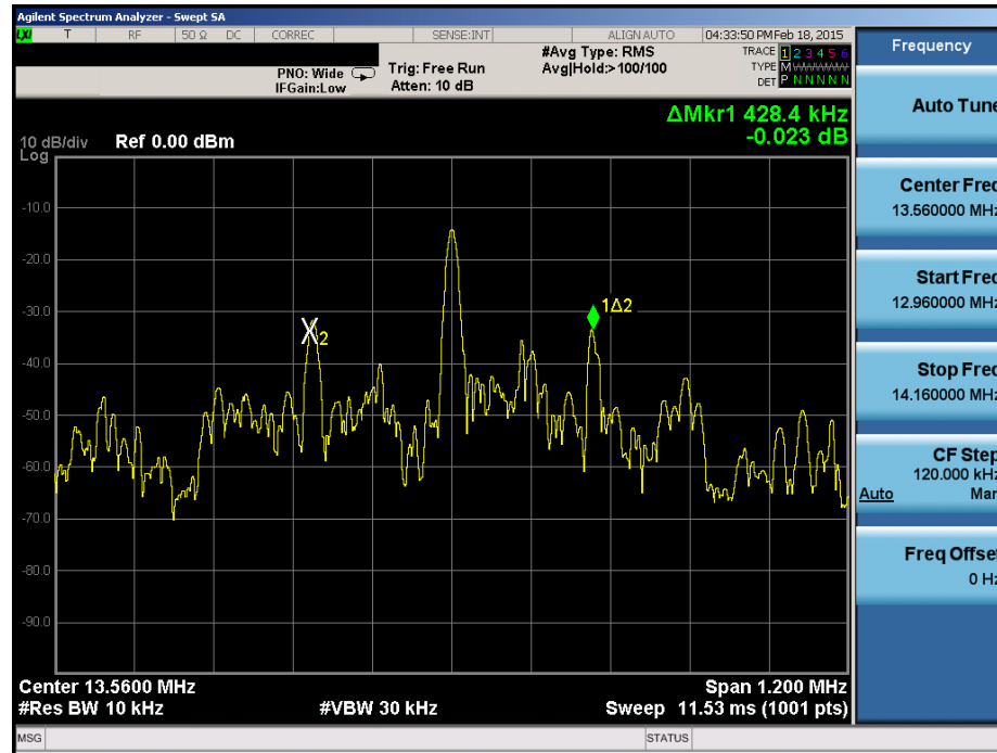
Figure 7-3. 20dB Bandwidth Plot with WCP
