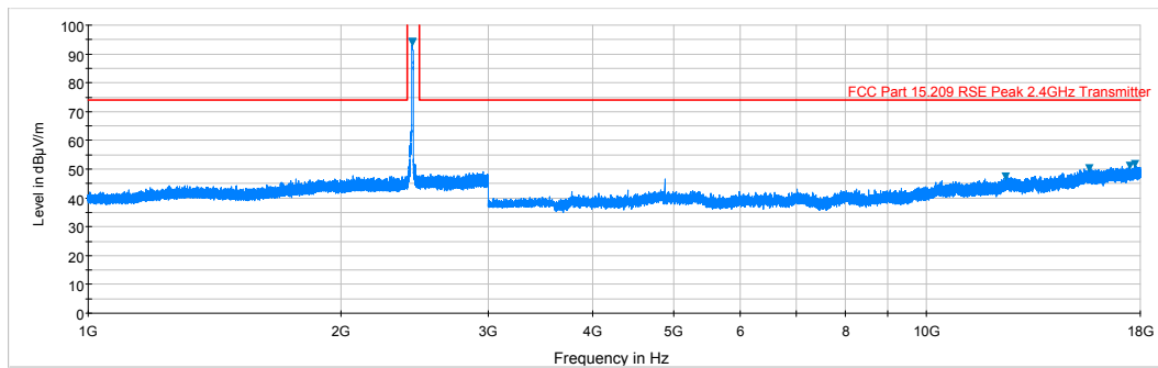
Plot 6-57. Radiated Spurious Plot above 1GHz (802.11b – Ch. 6, Ant. Pol. H)
