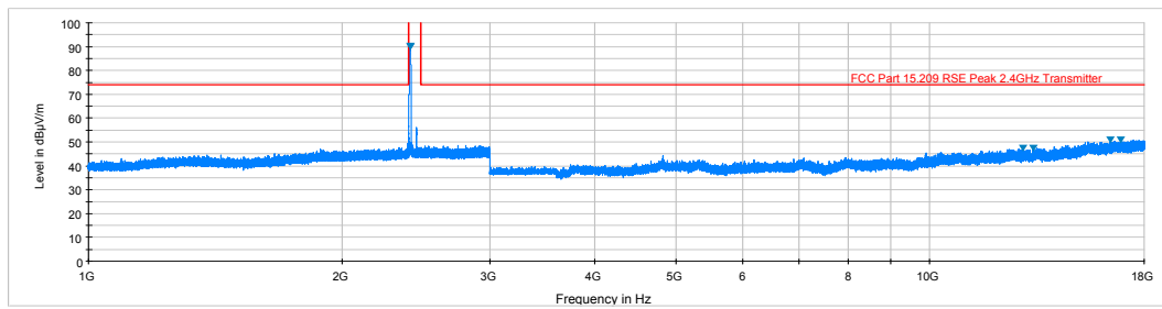
Plot 6-64. Radiated Spurious Plot above 1GHz (802.11b – Ch. 1, Ant. Pol. V)
