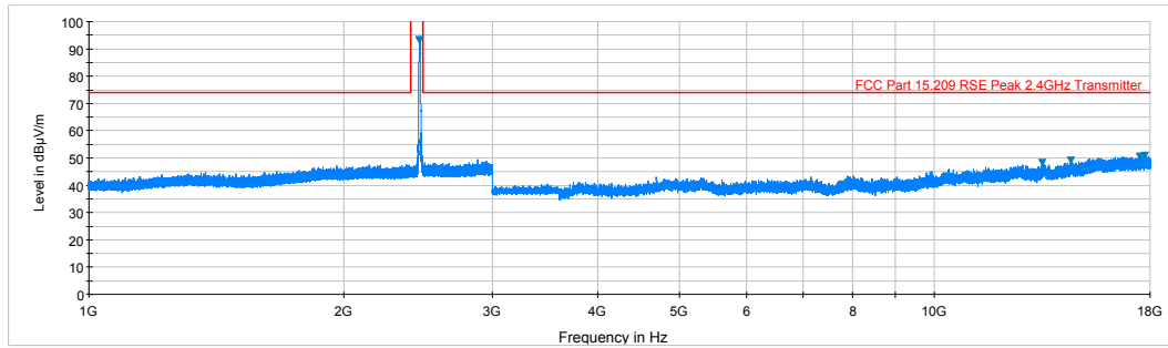
Plot 6-60. Radiated Spurious Plot above 1GHz (802.11b – Ch. 11, Ant. Pol. V)
