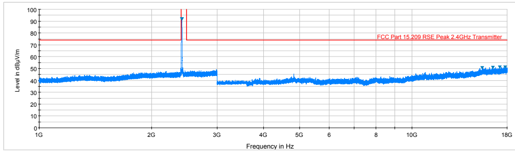
Plot 6-56. Radiated Spurious Plot above 1GHz (802.11b – Ch. 1, Ant. Pol. V)
