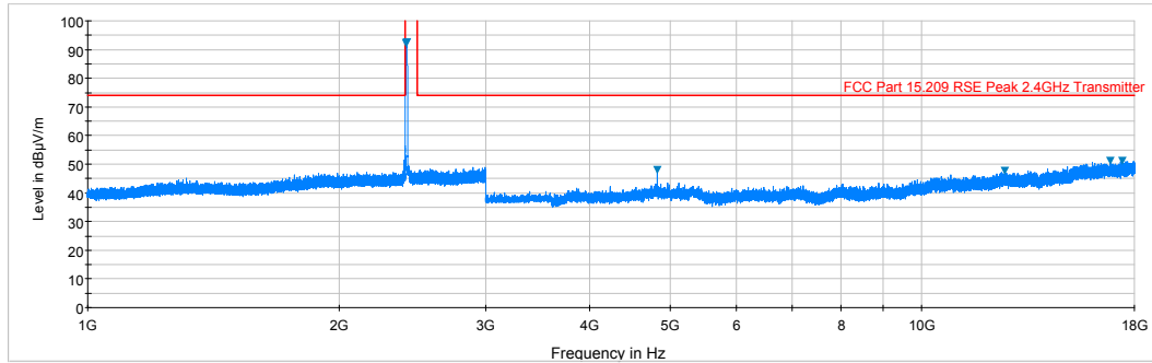
Plot 6-55. Radiated Spurious Plot above 1GHz (802.11b – Ch. 1, Ant. Pol. H)
