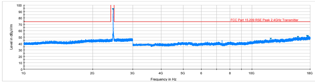
Plot 6-59. Radiated Spurious Plot above 1GHz (802.11b – Ch. 11, Ant. Pol. H)
