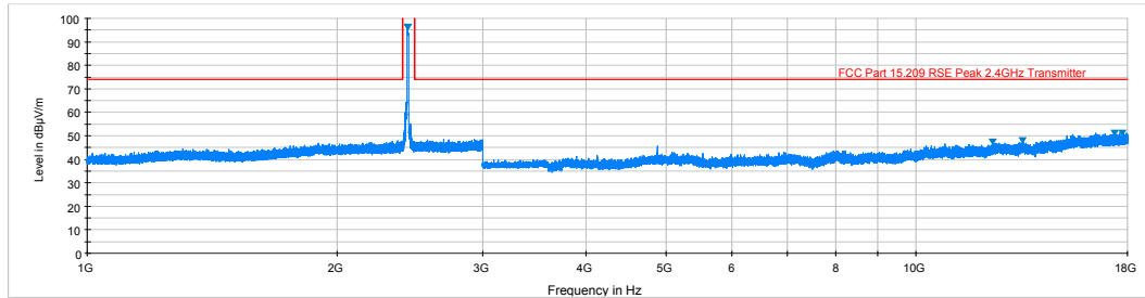
Plot 6-65. Radiated Spurious Plot above 1GHz (802.11b – Ch. 6, Ant. Pol. H)
