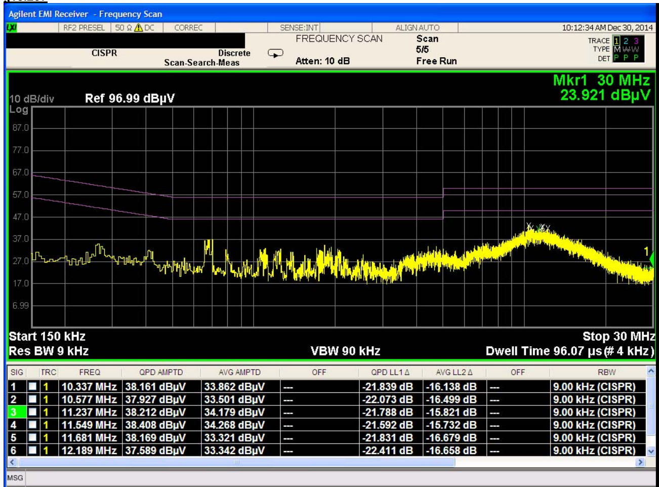
Plot 6-88. Line Conducted Plot with 802.11b (N)
