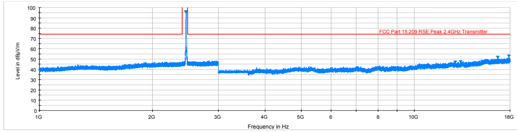
Plot 6-67. Radiated Spurious Plot above 1GHz (802.11b – Ch. 11, Ant. Pol. H)
