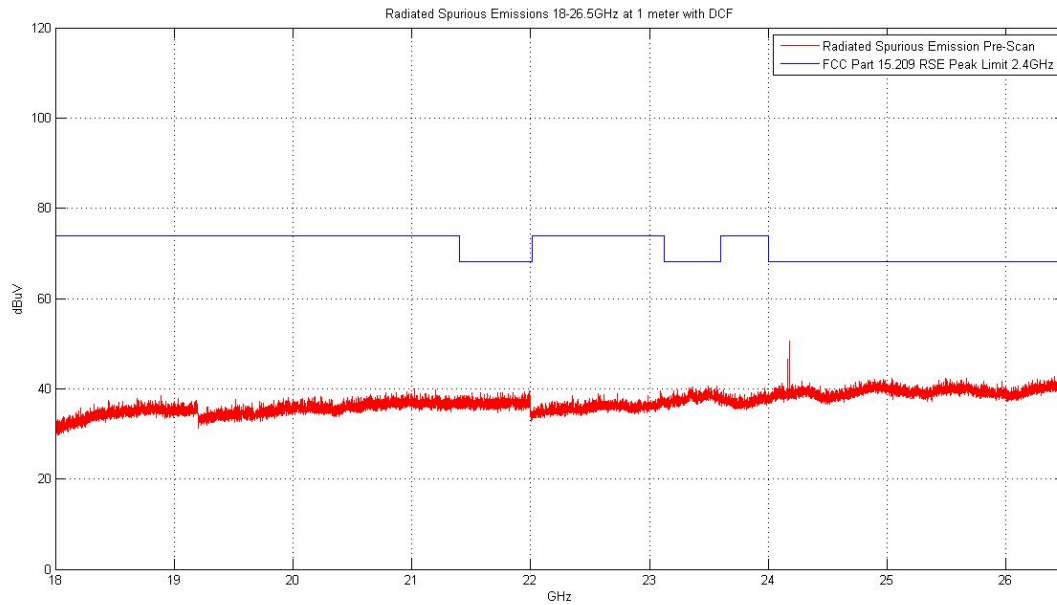
Plot 6-61. Radiated Spurious Plot above 18GHz (Pol. H)
