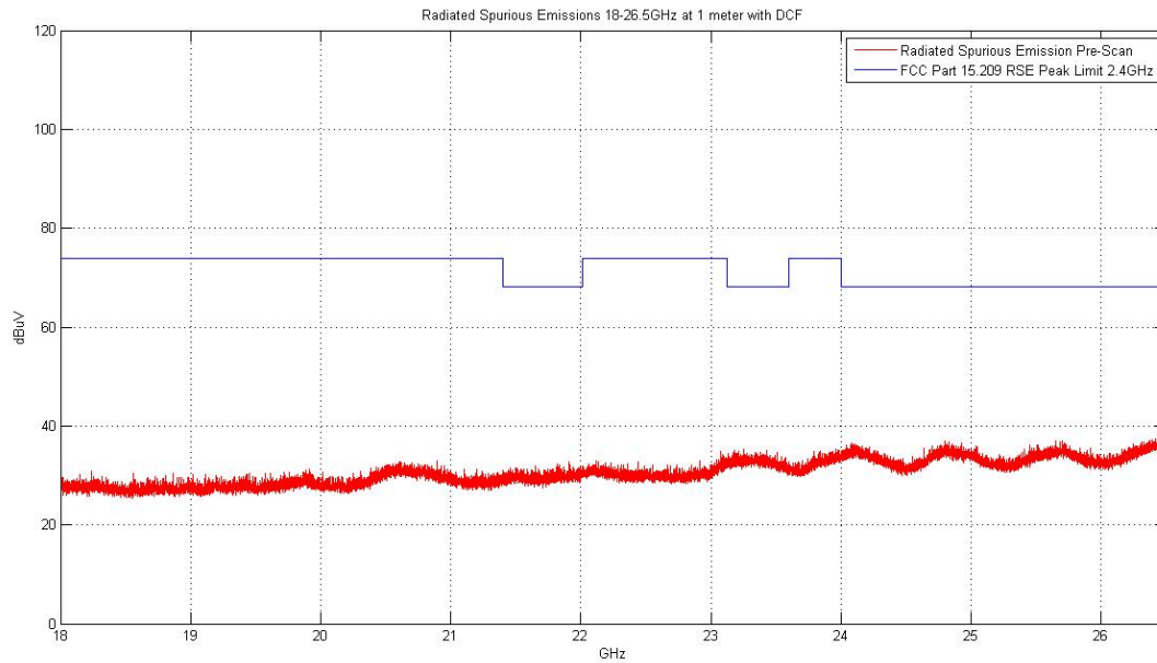
Plot 6-70. Radiated Spurious Plot above 18GHz (Pol. V)
