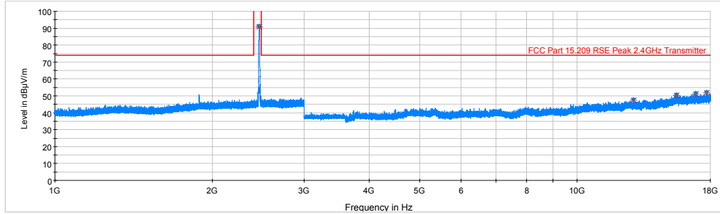
Plot 6-68. Radiated Spurious Plot above 1GHz (802.11b – Ch. 11, Ant. Pol. V)
