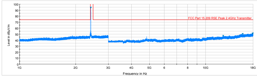
Plot 6-63. Radiated Spurious Plot above 1GHz (802.11b – Ch. 1, Ant. Pol. H)
