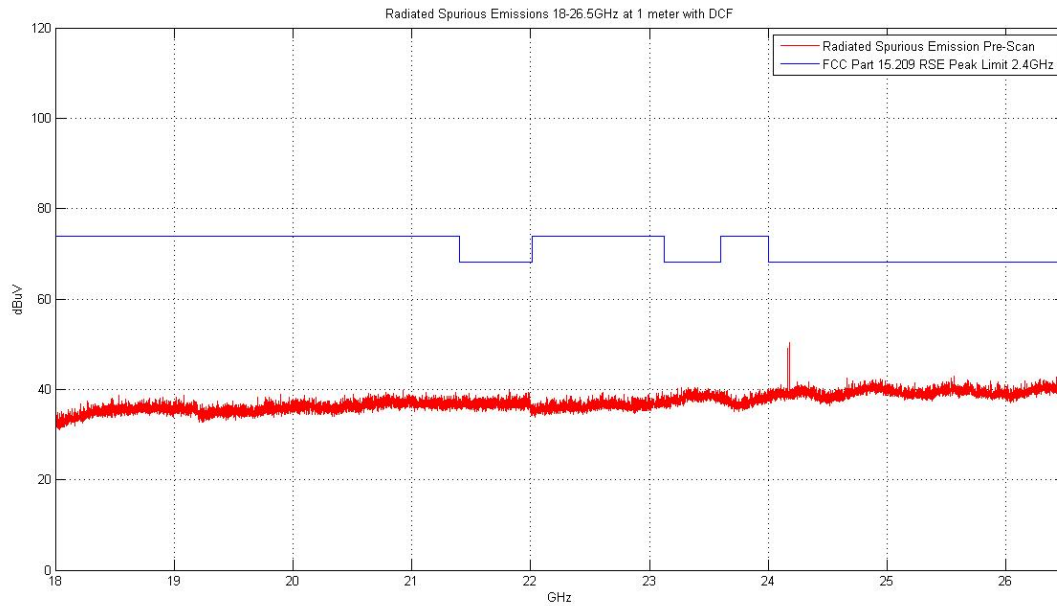
Plot 6-62. Radiated Spurious Plot above 18GHz (Pol. V)
