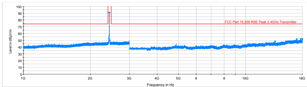
Plot 6-66. Radiated Spurious Plot above 1GHz (802.11b – Ch. 6, Ant. Pol. V)
