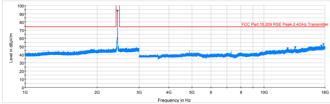
Plot 6-58. Radiated Spurious Plot above 1GHz (802.11b – Ch. 6, Ant. Pol. V)
