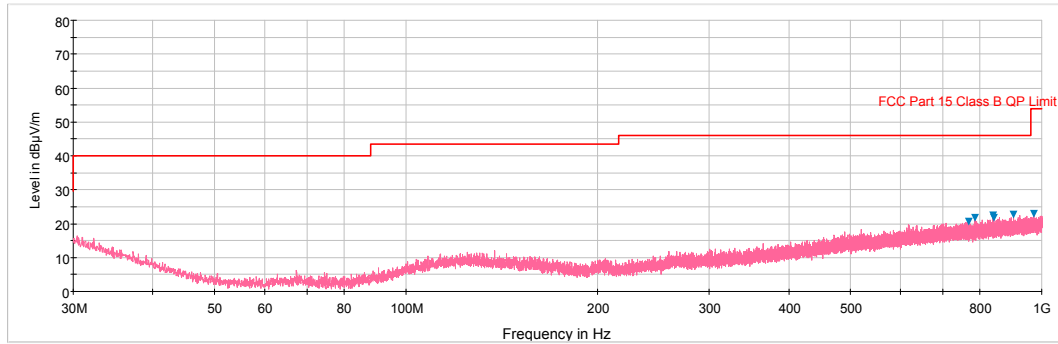
Plot 6-85. Radiated Spurious Plot below 1GHz (Pol. H)
