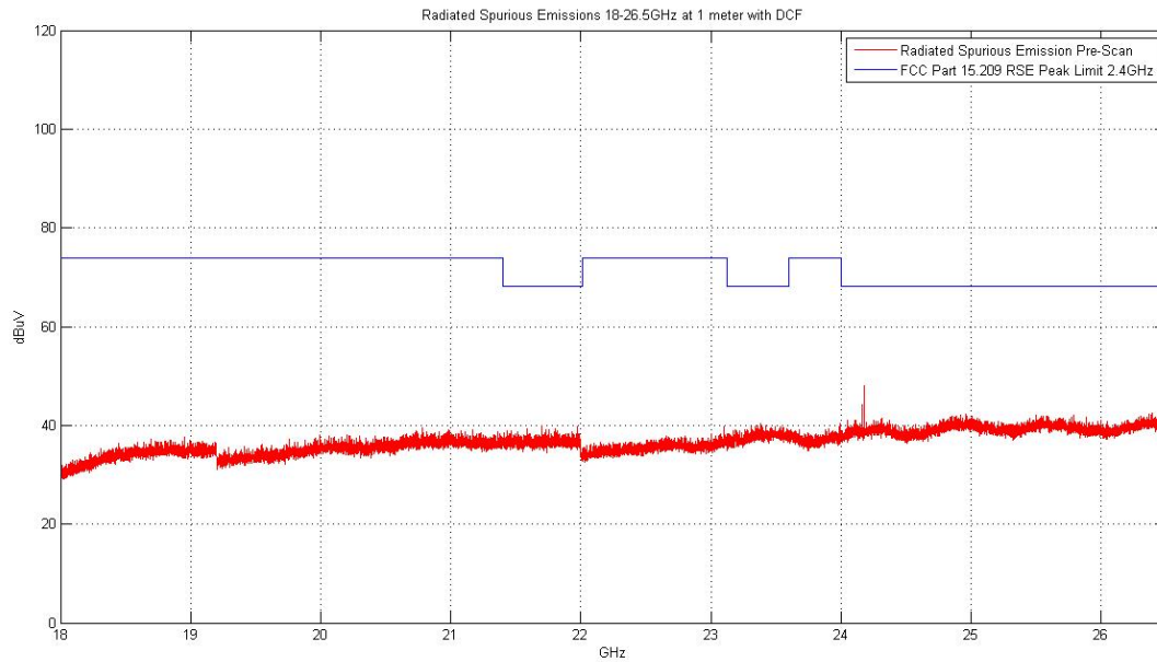
Plot 6-69. Radiated Spurious Plot above 18GHz (Pol. H)
