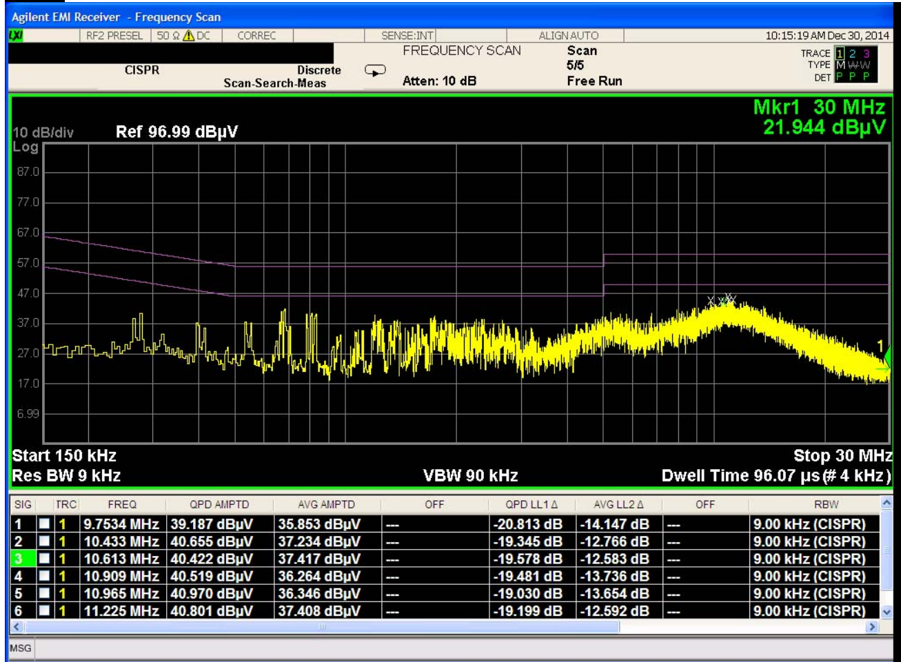
Plot 6-87. Line Conducted Plot with 802.11b (L1)
