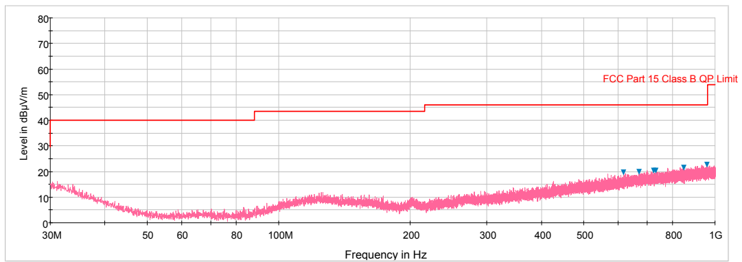
Plot 6-86. Radiated Spurious Plot below 1GHz (Pol. V)
