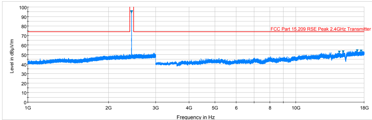
Plot 6-21. Radiated Spurious Plot above 1GHz (BTLE – Ch. 19, Ant. Pol. V)
