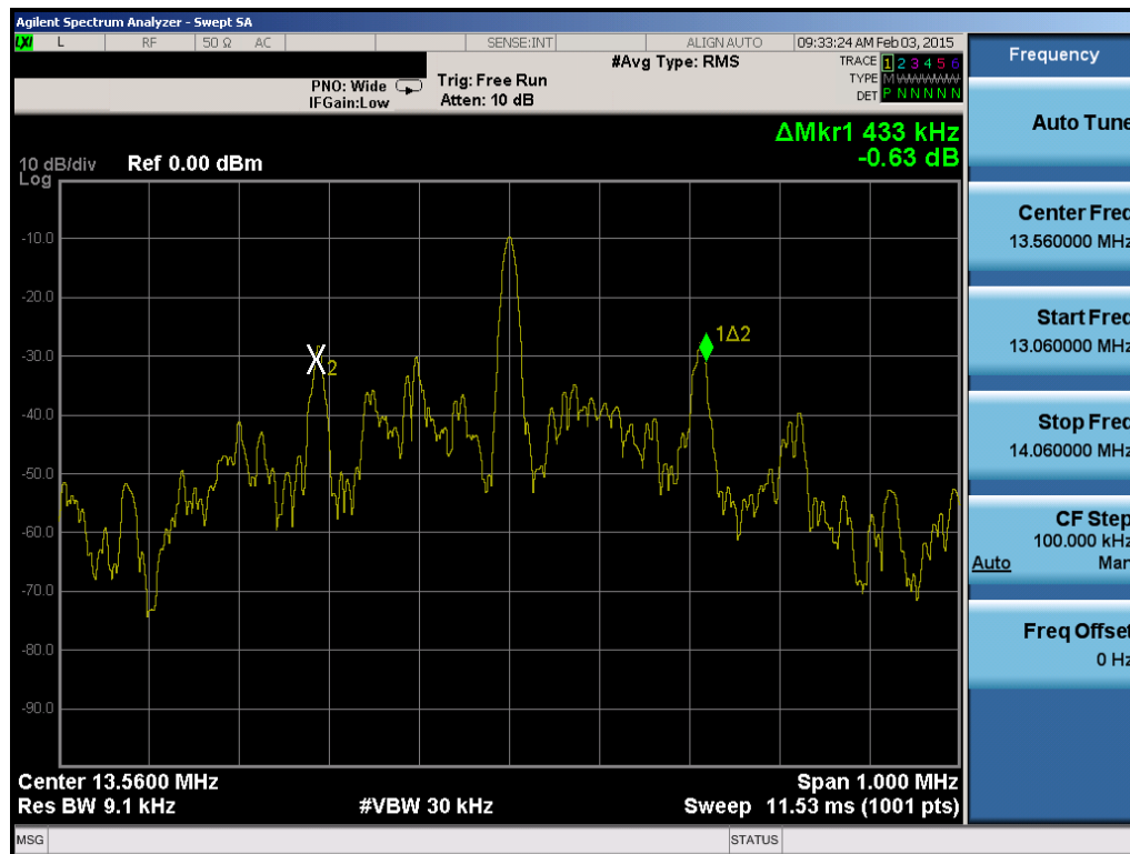
Figure 7-2. 20dB Bandwidth Plot
