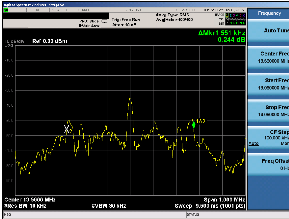
Figure 7-3. 20dB Bandwidth Plot w/ WCP
