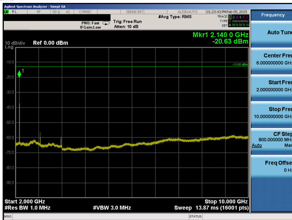
Plot 6-59. Conducted Spurious Plot (Band 12 – 3.0MHz QPSK – RB Size 1, RB Offset 0 – High Channel)
