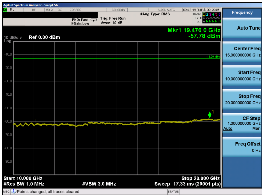
Plot 6-80. Conducted Spurious Plot (Band 25 – 5.0MHz QPSK – RB Size 1, RB Offset 0 – Low Channel)
