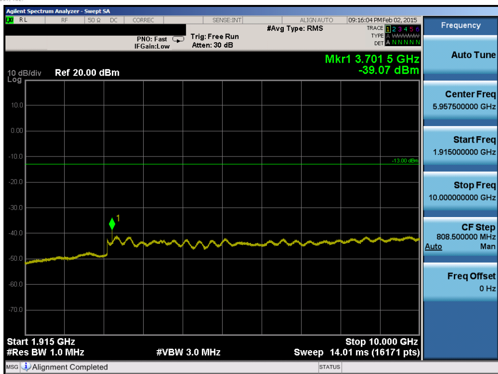
Plot 6-79. Conducted Spurious Plot (Band 25 – 5.0MHz QPSK – RB Size 1, RB Offset 0 – Low Channel)
