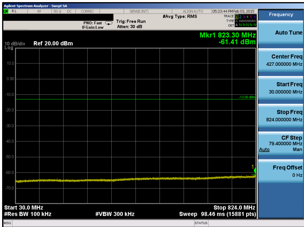
Plot 6-66. Conducted Spurious Plot (Band 26 – 1.4MHz QPSK – RB Size 1, RB Offset 0 – High Channel)
