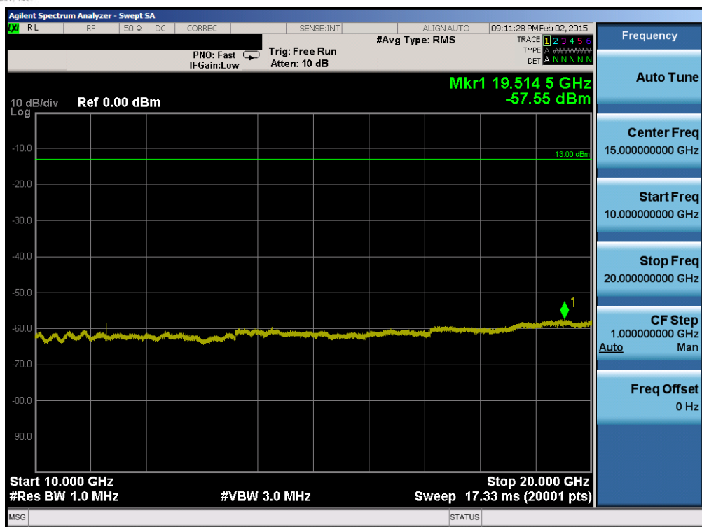
Plot 6-83. Conducted Spurious Plot (Band 25 – 5.0MHz QPSK – RB Size 1, RB Offset 0 – Mid Channel)
