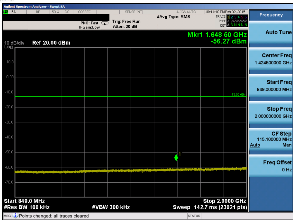
Plot 6-61. Conducted Spurious Plot (Band 26 – 1.4MHz QPSK – RB Size 1, RB Offset 0 – Low Channel)
