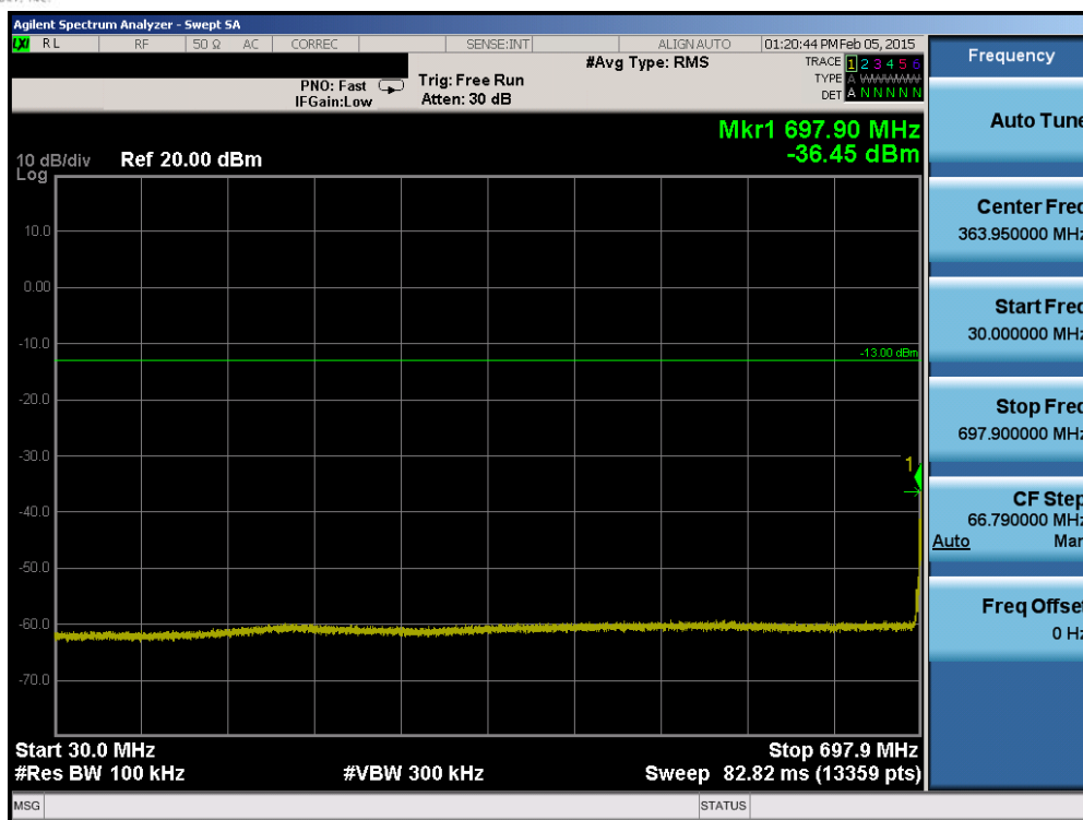
Plot 6-51. Conducted Spurious Plot (Band 12 – 3.0MHz QPSK – RB Size 1, RB Offset 0 – Low Channel)
