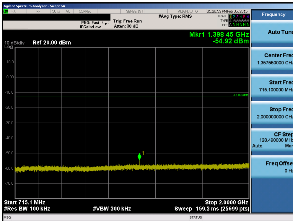
Plot 6-52. Conducted Spurious Plot (Band 12 – 3.0MHz QPSK – RB Size 1, RB Offset 0 – Low Channel)
