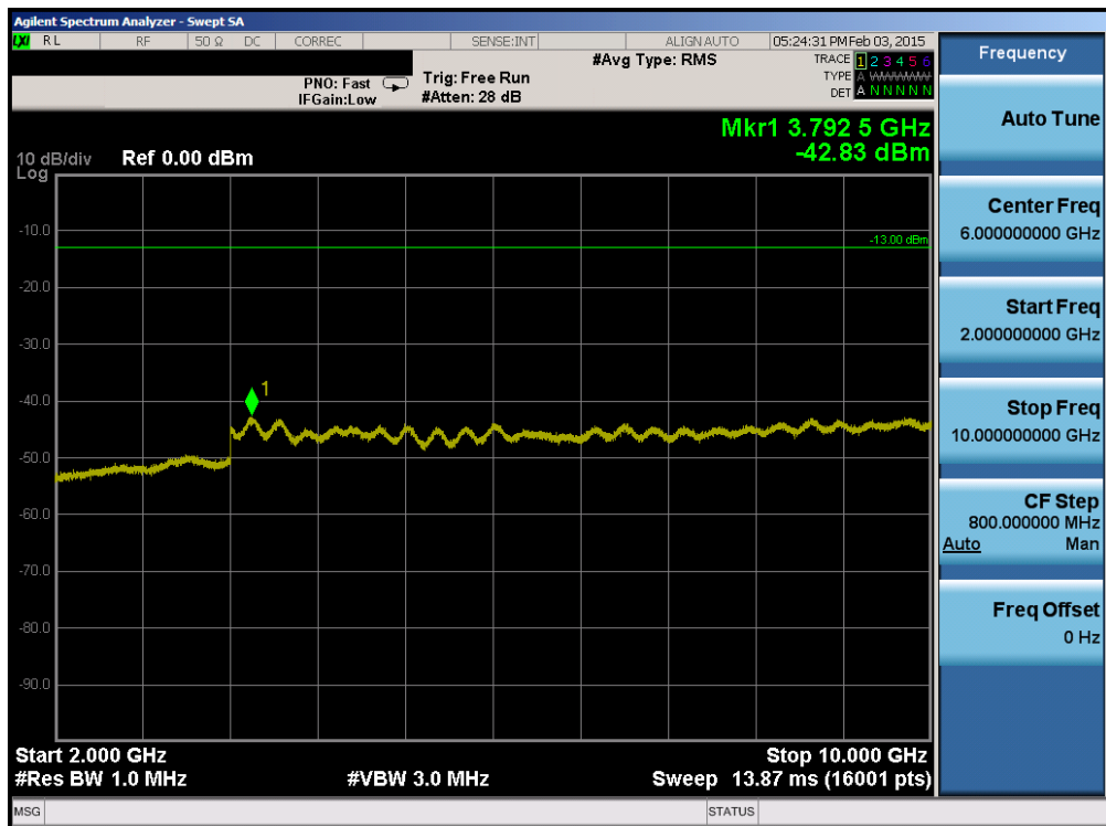
Plot 6-68. Conducted Spurious Plot (Band 26 – 1.4MHz QPSK – RB Size 1, RB Offset 0 – High Channel)
