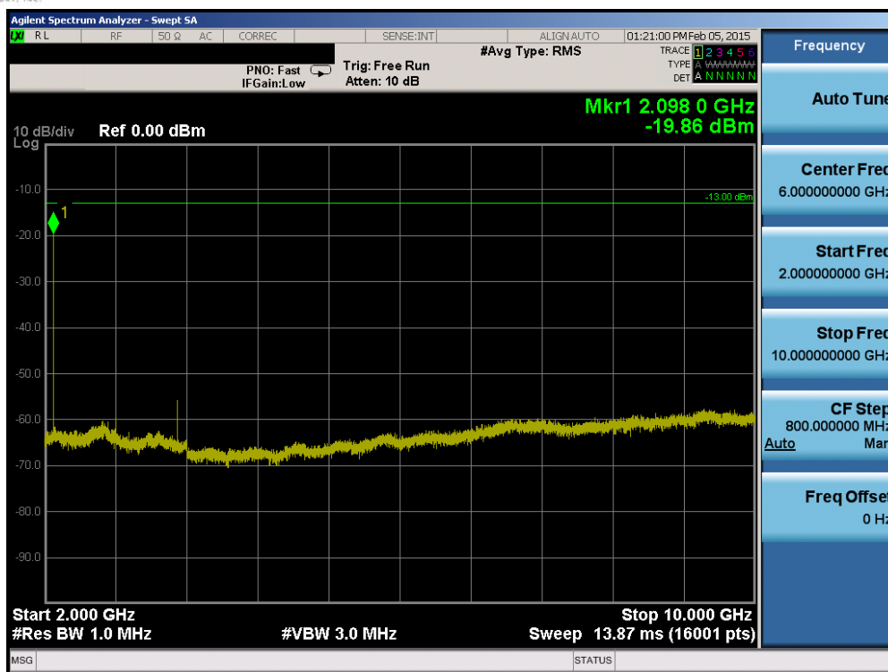
Plot 6-53. Conducted Spurious Plot (Band 12 – 3.0MHz QPSK – RB Size 1, RB Offset 0 – Low Channel)
