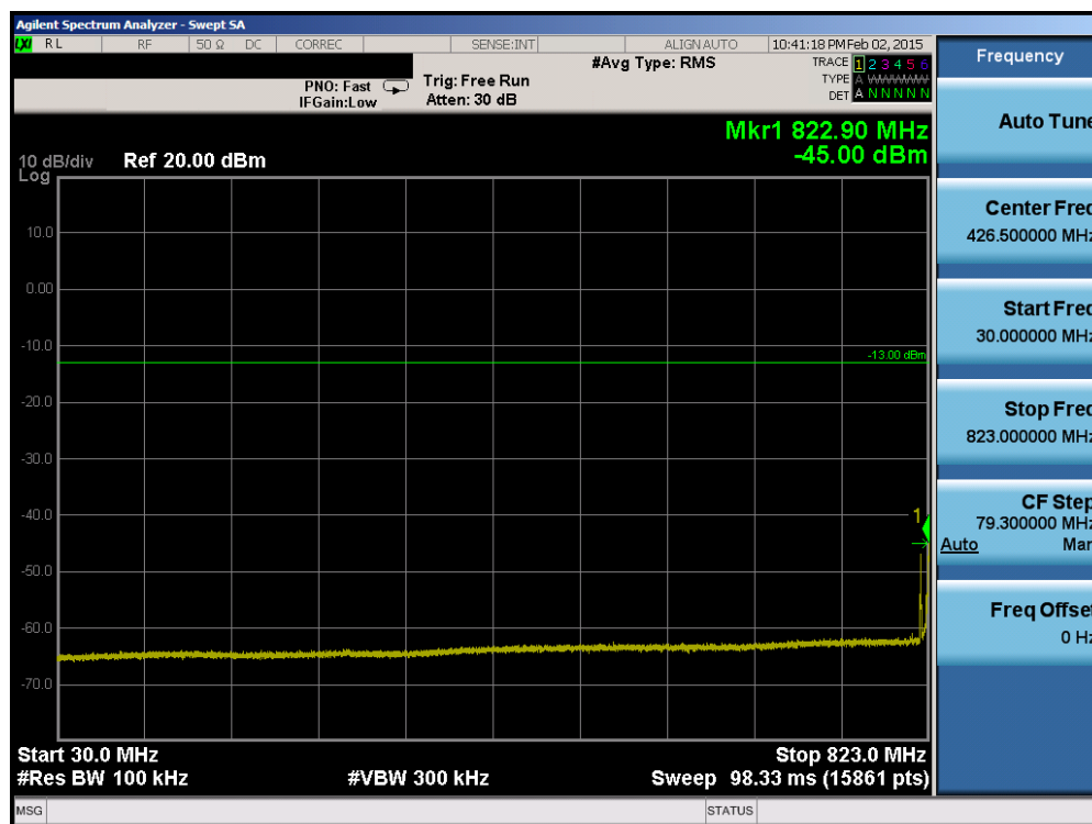
Plot 6-60. Conducted Spurious Plot (Band 26 – 1.4MHz QPSK – RB Size 1, RB Offset 0 – Low Channel)
