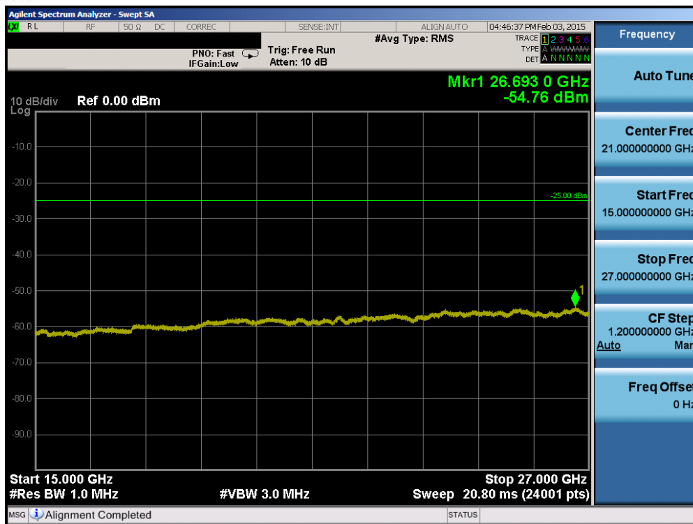
Plot 6-95. Conducted Spurious Plot (Band 41 – 5.0MHz QPSK – RB Size 1, RB Offset 0 – High Channel)
