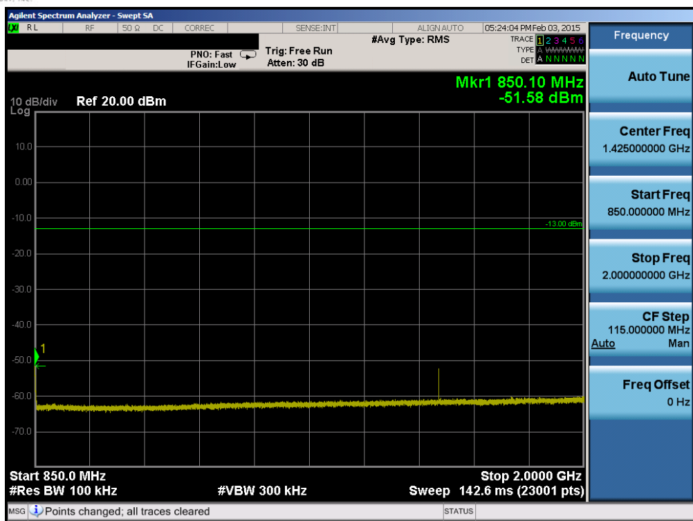
Plot 6-67. Conducted Spurious Plot (Band 26 – 1.4MHz QPSK – RB Size 1, RB Offset 0 – High Channel)
