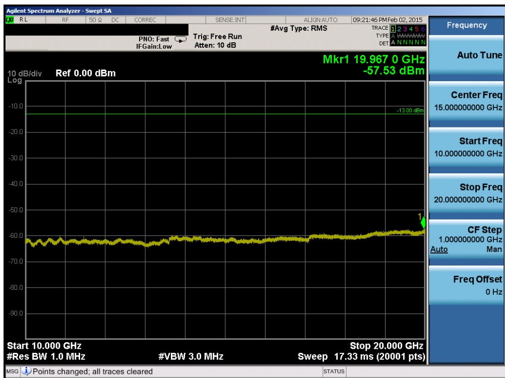
Plot 6-86. Conducted Spurious Plot (Band 25 – 5.0MHz QPSK – RB Size 1, RB Offset 0 – High Channel)
