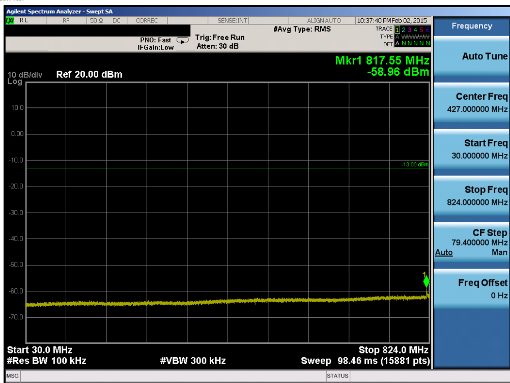
Plot 6-63. Conducted Spurious Plot (Band 26 – 1.4MHz QPSK – RB Size 1, RB Offset 0 – Mid Channel)
