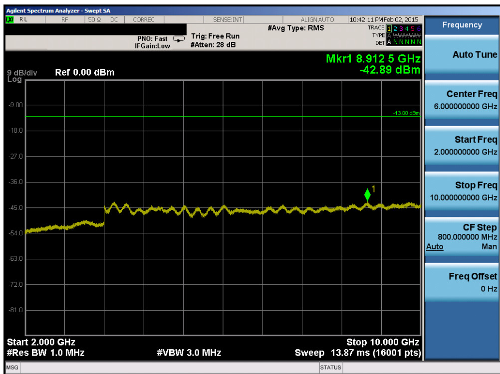
Plot 6-62. Conducted Spurious Plot (Band 26 – 1.4MHz QPSK – RB Size 1, RB Offset 0 – Low Channel)
