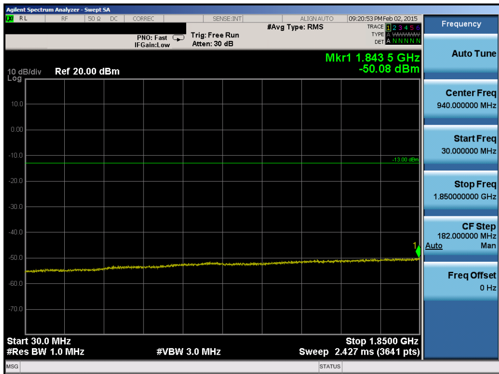
Plot 6-84. Conducted Spurious Plot (Band 25 – 5.0MHz QPSK – RB Size 1, RB Offset 0 – High Channel)
