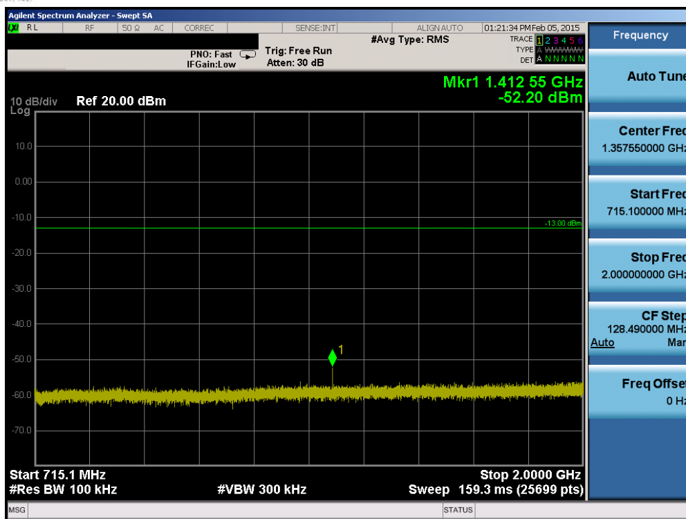
Plot 6-55. Conducted Spurious Plot (Band 12 – 3.0MHz QPSK – RB Size 1, RB Offset 0 – Mid Channel)
