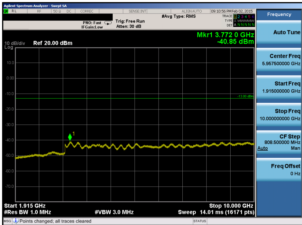
Plot 6-82. Conducted Spurious Plot (Band 25 – 5.0MHz QPSK – RB Size 1, RB Offset 0 – Mid Channel)
