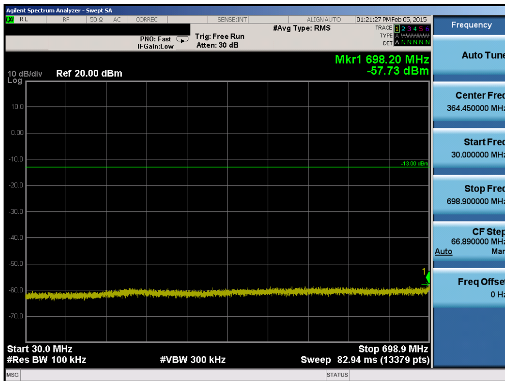
Plot 6-54. Conducted Spurious Plot (Band 12 – 3.0MHz QPSK – RB Size 1, RB Offset 0 – Mid Channel)
