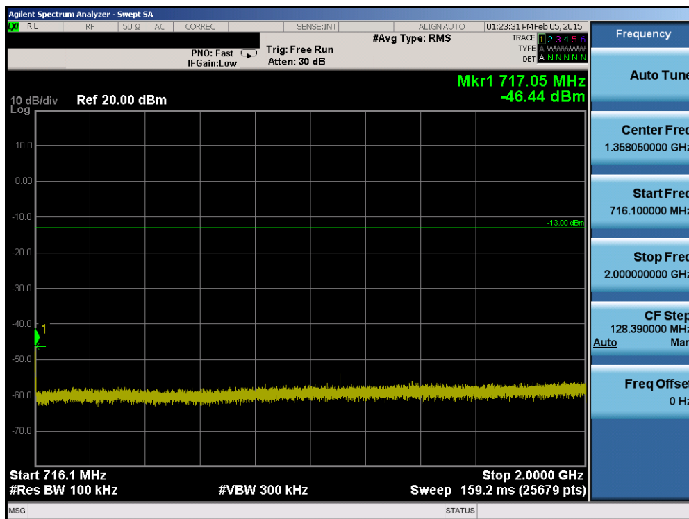
Plot 6-58. Conducted Spurious Plot (Band 12 – 3.0MHz QPSK – RB Size 1, RB Offset 0 – High Channel)
