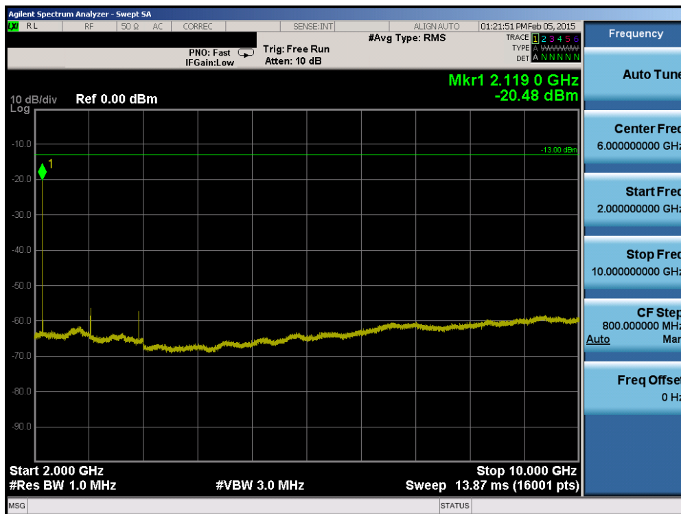
Plot 6-56. Conducted Spurious Plot (Band 12 – 3.0MHz QPSK – RB Size 1, RB Offset 0 – Mid Channel)
