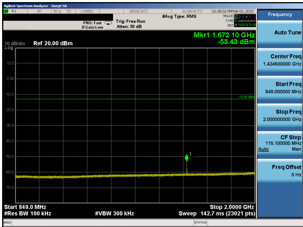
Plot 6-64. Conducted Spurious Plot (Band 26 – 1.4MHz QPSK – RB Size 1, RB Offset 0 – Mid Channel)
