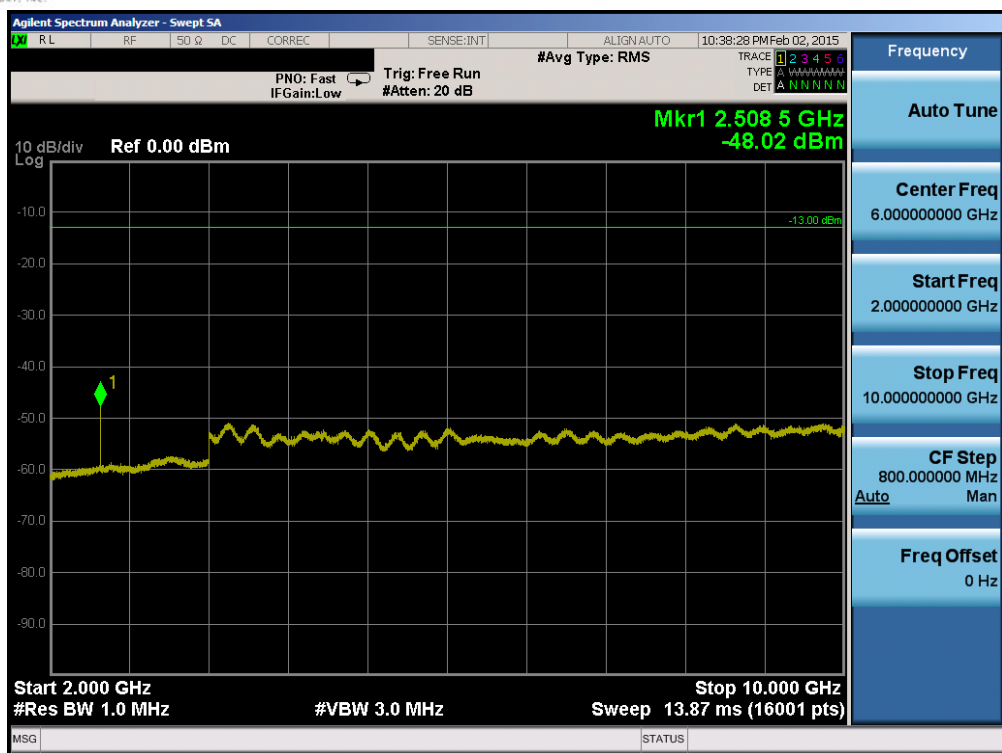
Plot 6-65. Conducted Spurious Plot (Band 26 – 1.4MHz QPSK – RB Size 1, RB Offset 0 – Mid Channel)
