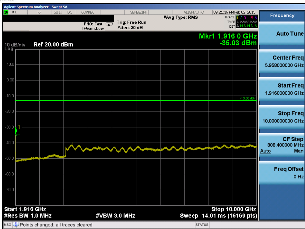
Plot 6-85. Conducted Spurious Plot (Band 25 – 5.0MHz QPSK – RB Size 1, RB Offset 0 – High Channel)
