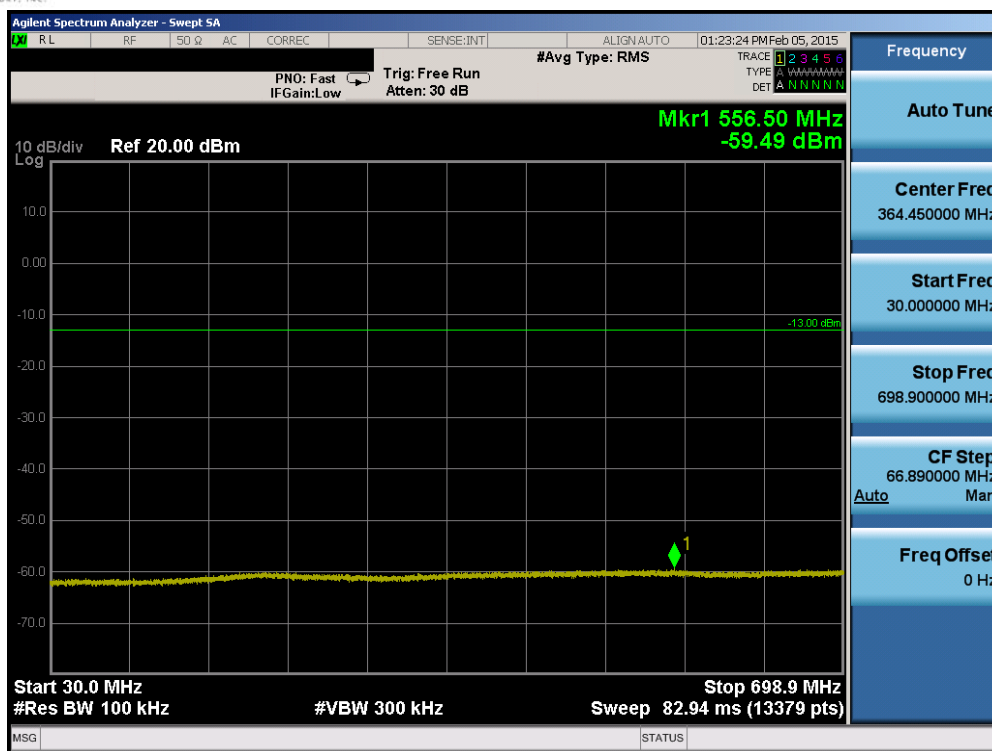
Plot 6-57. Conducted Spurious Plot (Band 12 – 3.0MHz QPSK – RB Size 1, RB Offset 0 – High Channel)
