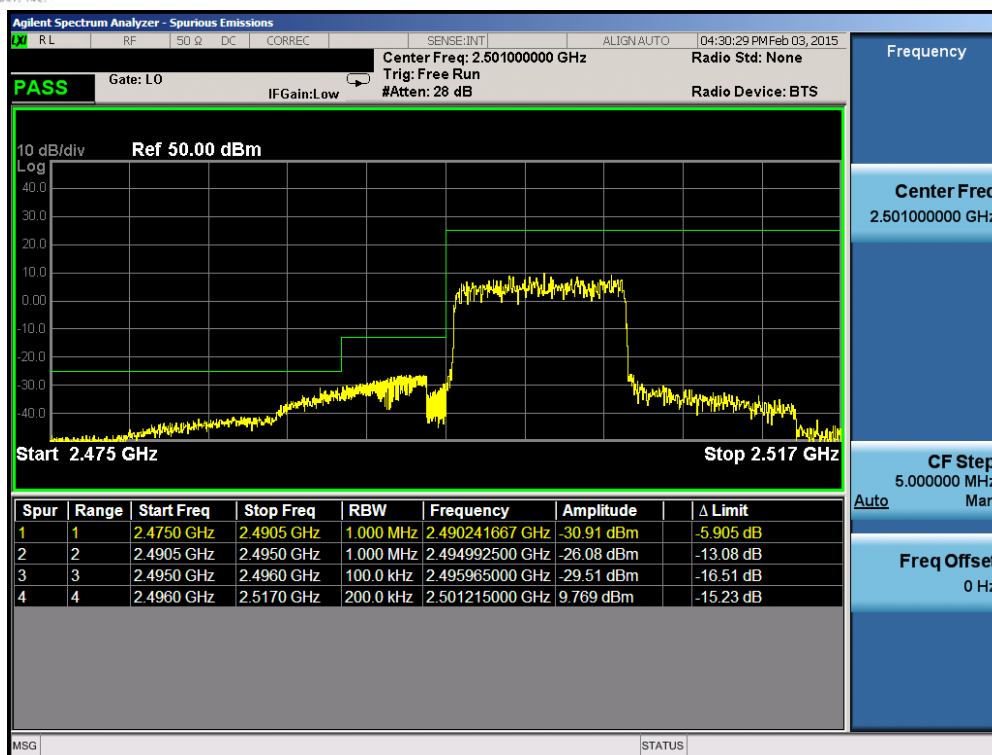
Plot 6-178. Lower ACP Plot (Band 41 – 10.0MHz QPSK – RB Size 50)
