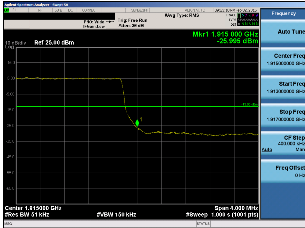
Plot 6-162. Upper Band Edge Plot (Band 25 – 5.0MHz QPSK – RB Size 25)
