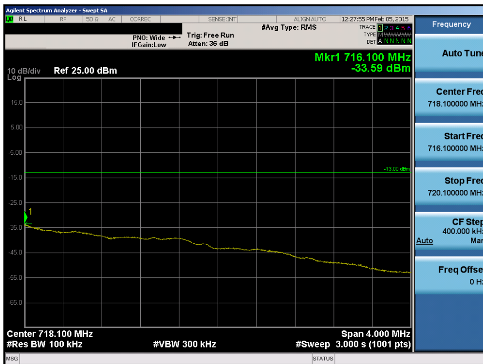
Plot 6-99. Upper Extended Band Edge Plot (Band 12 – 1.4MHz QPSK – RB Size 6)
