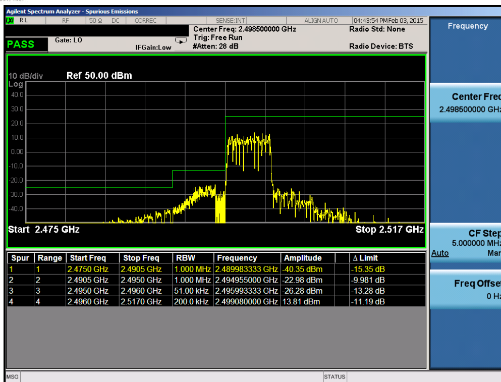
Plot 6-176. Lower ACP Plot (Band 41 – 5.0MHz QPSK – RB Size 25)
