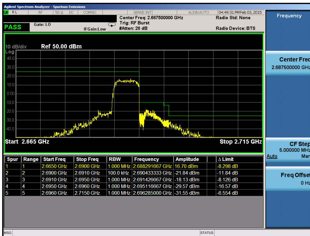
Plot 6-177. Upper ACP Plot (Band 41 – 5.0MHz QPSK – RB Size 25)
