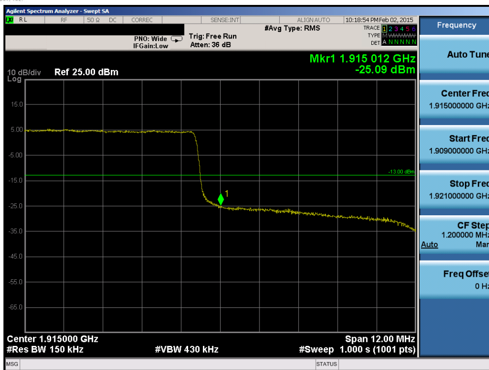
Plot 6-170. Upper Band Edge Plot (Band 25 – 15.0MHz QPSK – RB Size 75)
