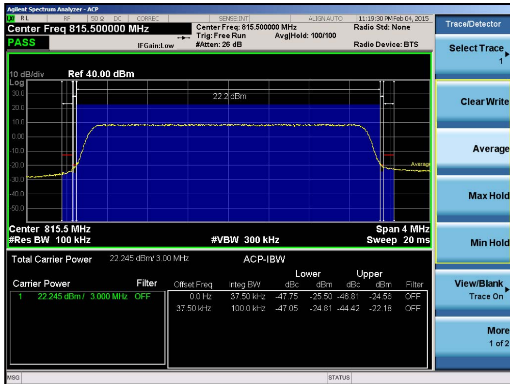
Plot 8-10. Channel Edge Plot (3MHz QPSK – RB Size 15– Low Channel)
