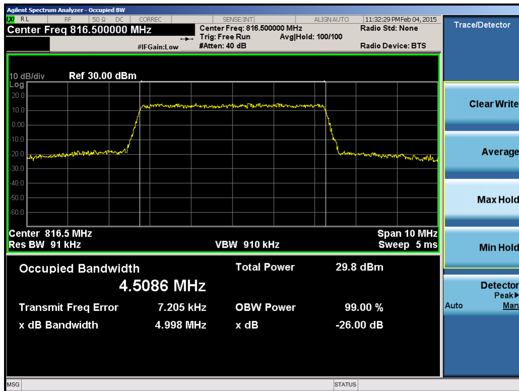
Plot 8-16. Occupied Bandwidth Plot (5MHz 16-QAM – RB Size 25– Low Channel))
