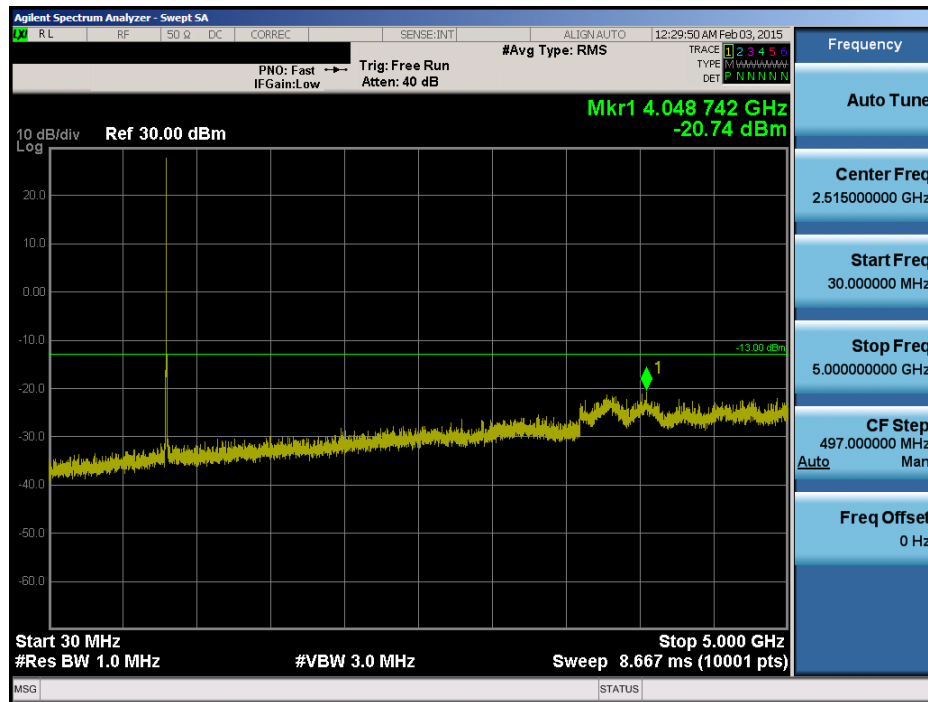
Plot 7-1. Conducted Spurious Plot (Ch. 476)
