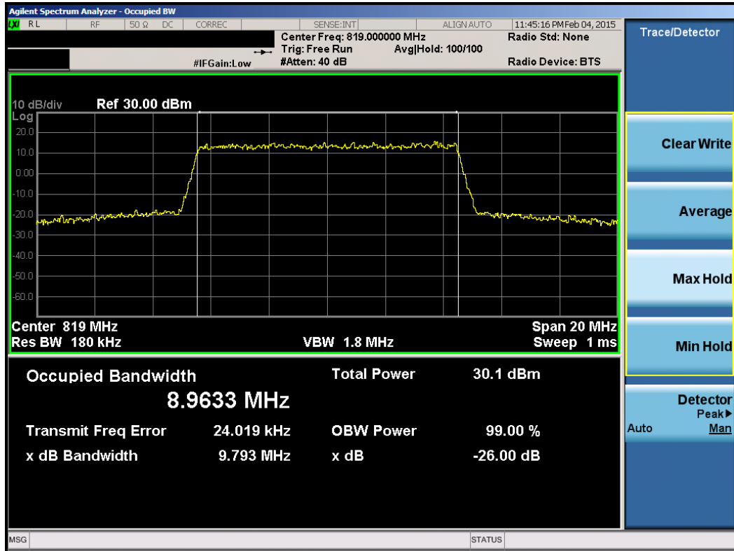
Plot 8-19. Occupied Bandwidth Plot (10MHz 16-QAM – RB Size 50)
