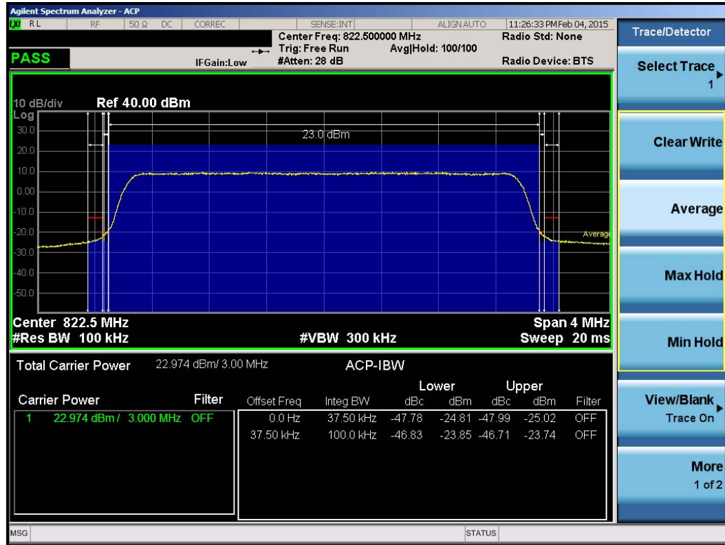
Plot 8-13. Channel Edge Plot (3MHz QPSK – RB Size 15 – High Channel)
