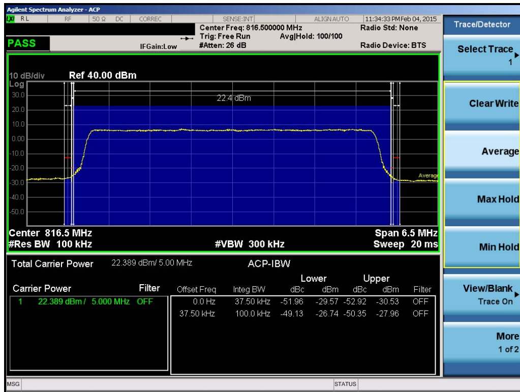
Plot 8-14. Channel Edge Plot (5MHz QPSK – RB Size 25– Low Channel)
