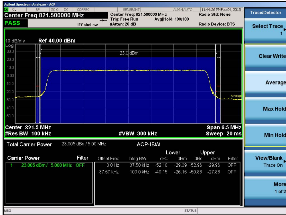
Plot 8-17. Channel Edge Plot (5MHz QPSK – RB Size 25 – High Channel)
