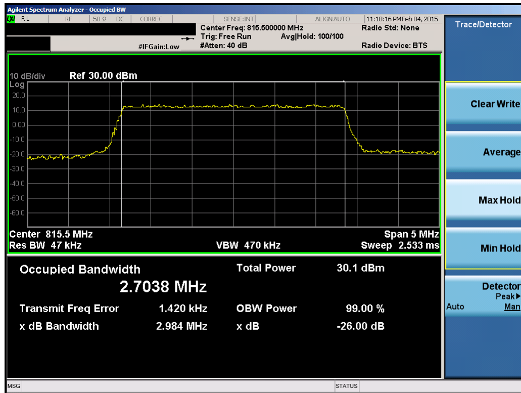
Plot 8-12. Occupied Bandwidth Plot (3MHz 16-QAM – RB Size 15– Low Channel))
