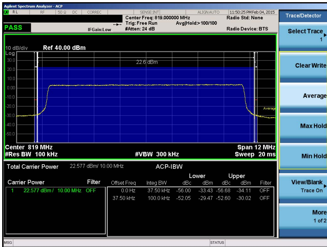
Plot 8-20. Channel Edge Plot (10MHz QPSK – RB Size 50)
