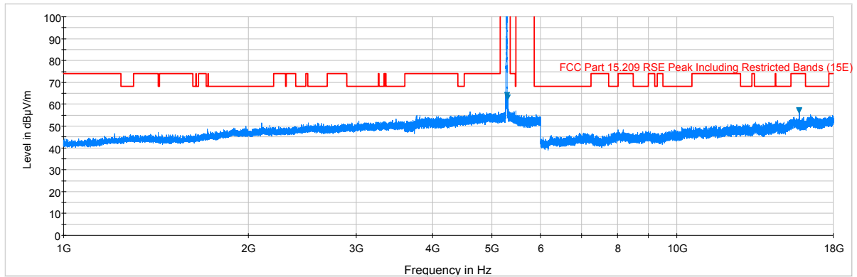
Plot 6-155. Radiated Spurious Plot above 1GHz (802.11a – U2A, Ant. Pol. H)
