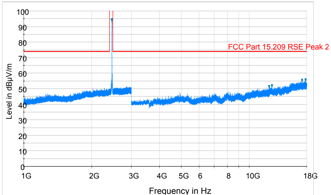
Plot 6-68. Radiated Spurious Plot above 1GHz (802.11b – Ch. 11, Ant. Pol. V)
